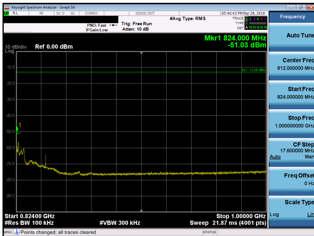
Plot 7-27. Conducted Spurious Plot (LTE Band 26 - 5 MHz QPSK – RB Size 1, RB Offset 0 – High Channel)
