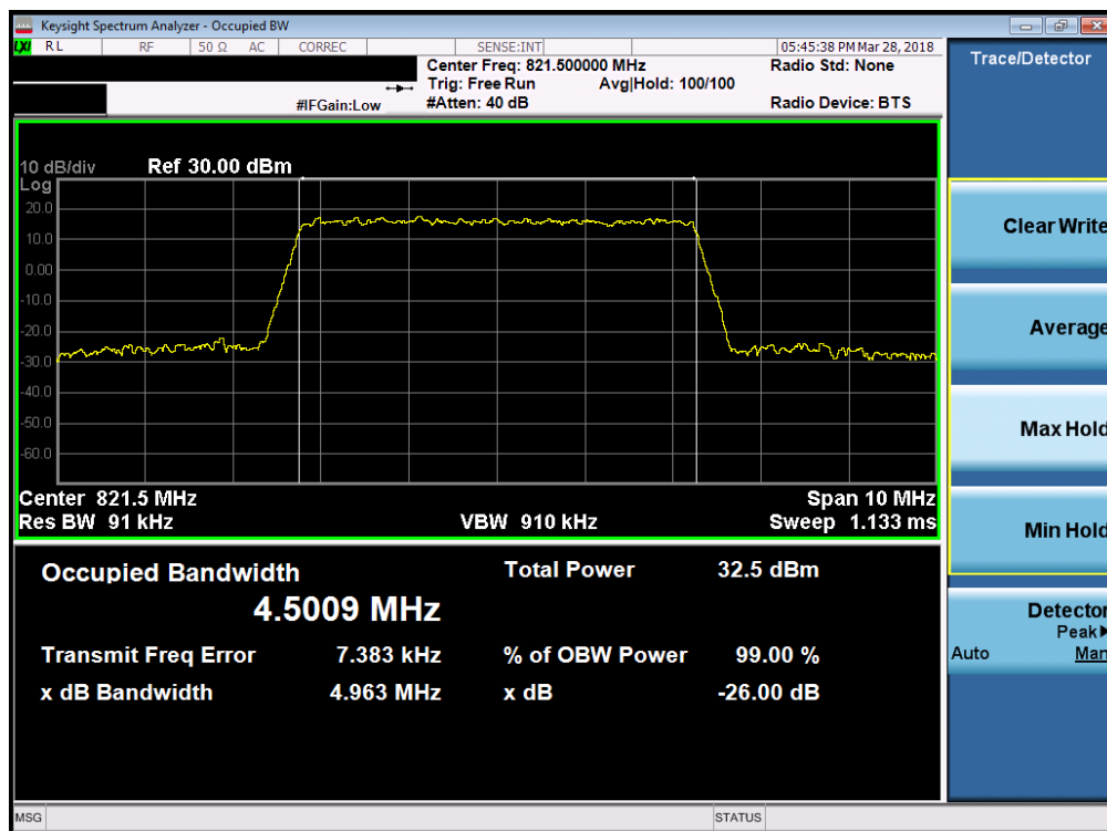
Plot 7-9. Occupied Bandwidth Plot (LTE Band 26 - 5MHz 16-QAM – RB Size 25– Low Channel)
