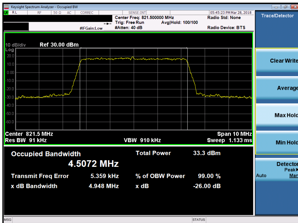
Plot 7-8. Occupied Bandwidth Plot (LTE Band 26 - 5MHz QPSK – RB Size 25– Low Channel)
