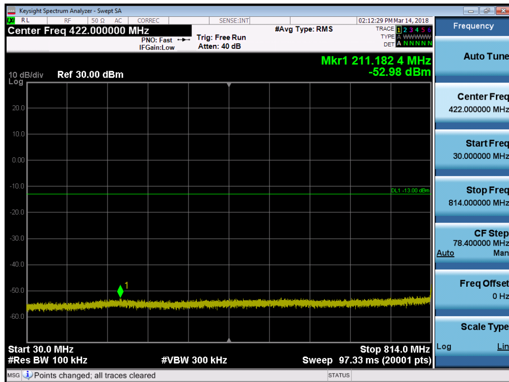
Plot 7-17. Conducted Spurious Plot (CDMA - Ch. 476)
