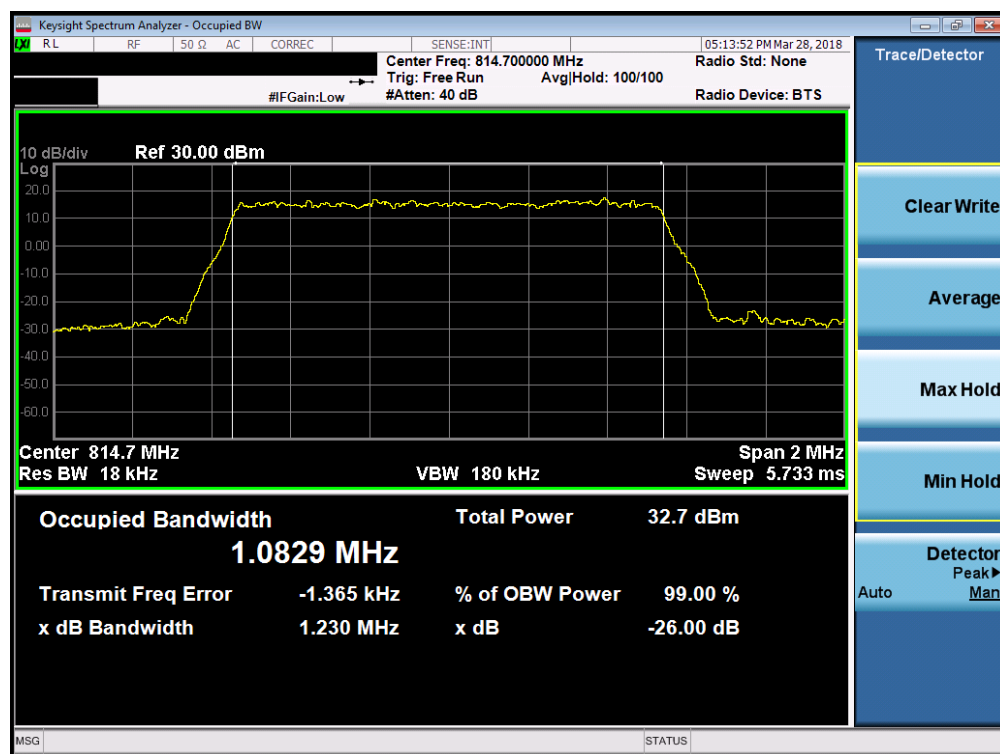
Plot 7-2. Occupied Bandwidth Plot (LTE Band 26 - 1.4MHz QPSK - RB Size 6- Low Channel)
