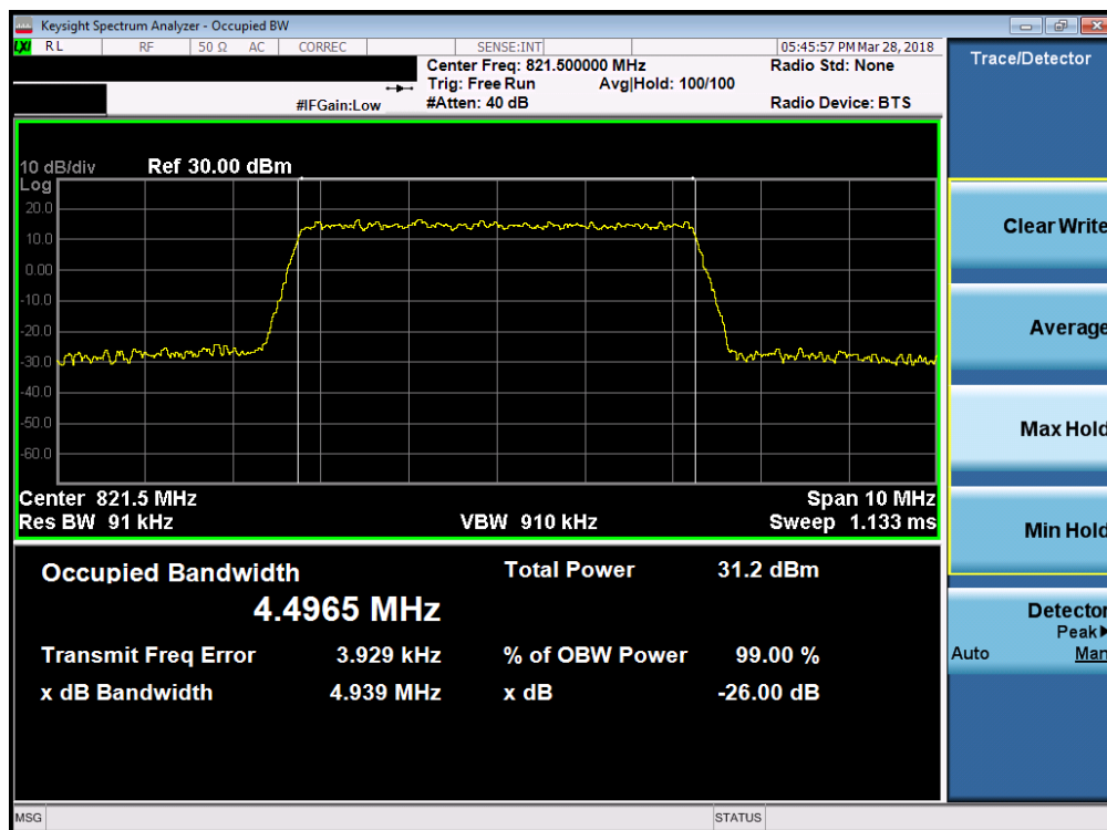
Plot 7-10. Occupied Bandwidth Plot (LTE Band 26 - 5MHz 64-QAM – RB Size 25– Low Channel)
