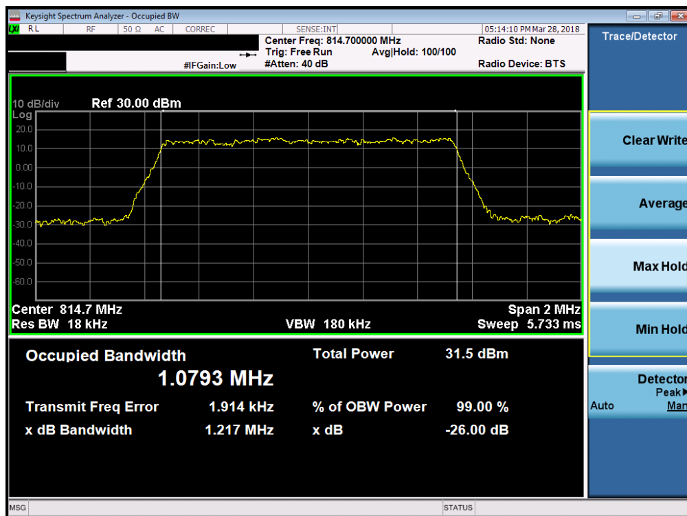
Plot 7-3. Occupied Bandwidth Plot (LTE Band 26 - 1.4MHz 16-QAM – RB Size 6– Low Channel)
