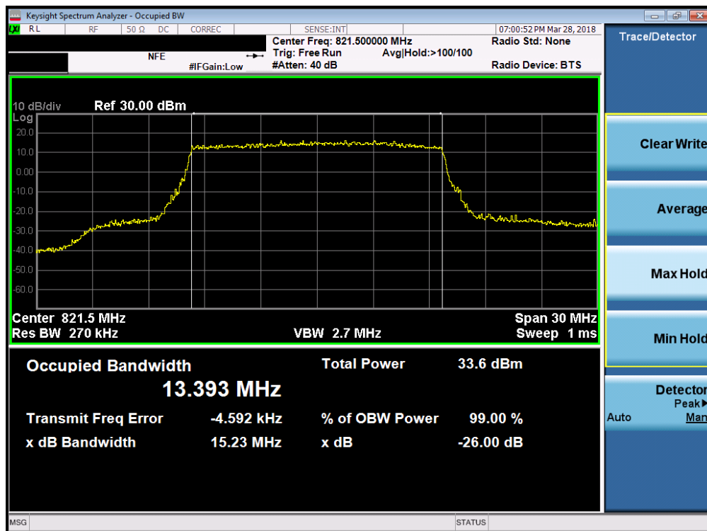
Plot 7-14. Occupied Bandwidth Plot (LTE Band 26 - 15MHz QPSK – RB Size 75)
