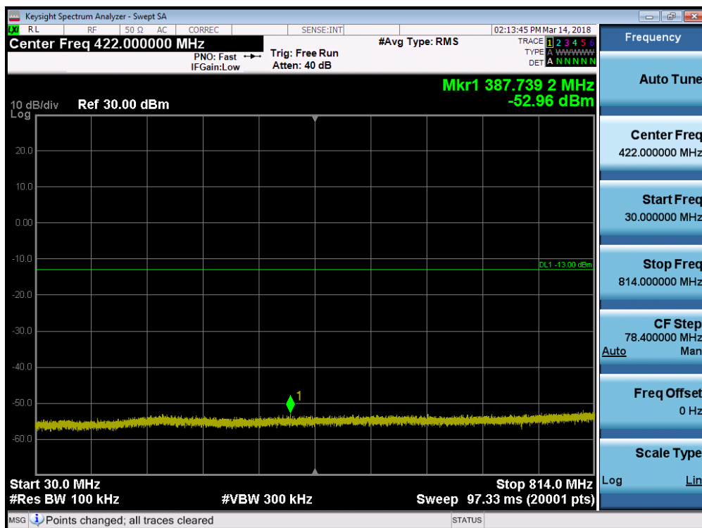
Plot 7-20. Conducted Spurious Plot (CDMA - Ch. 684)
