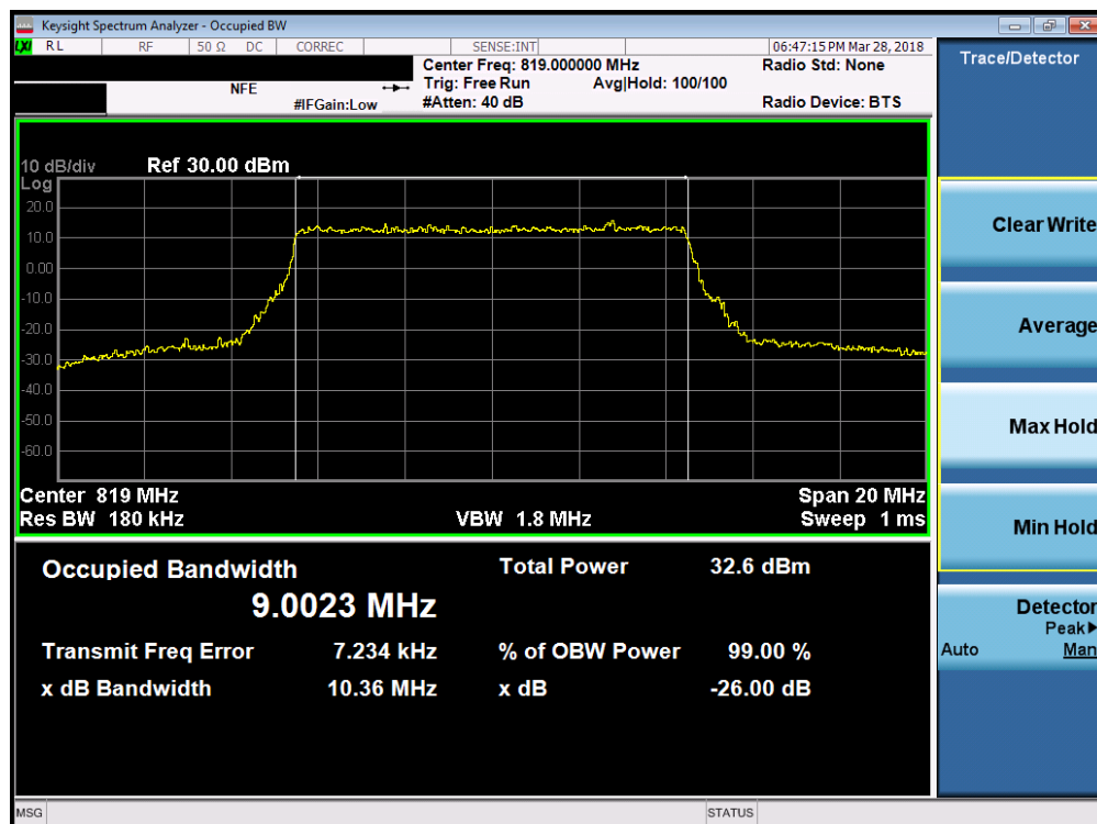
Plot 7-12. Occupied Bandwidth Plot (LTE Band 26 - 10MHz 16-QAM – RB Size 50)
