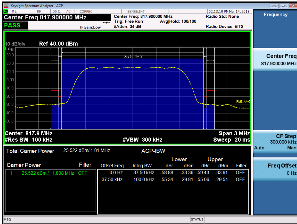
Plot 7-29. Channel Edge Plot (CDMA - Ch. 476)
