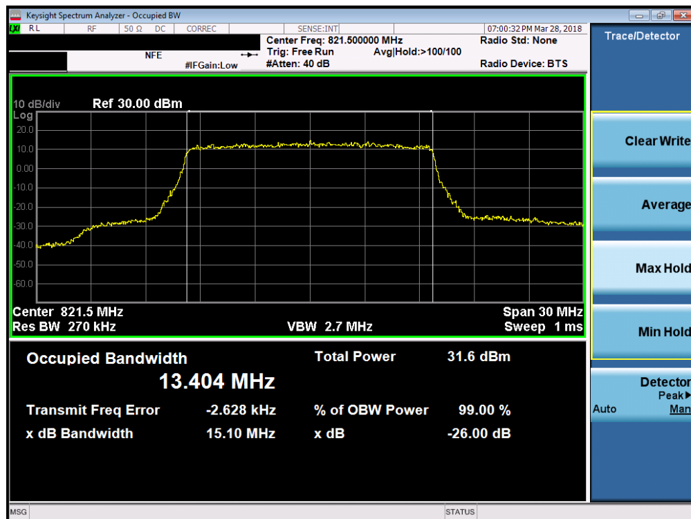
Plot 7-16. Occupied Bandwidth Plot (LTE Band 26 - 15MHz 64-QAM – RB Size 75)
