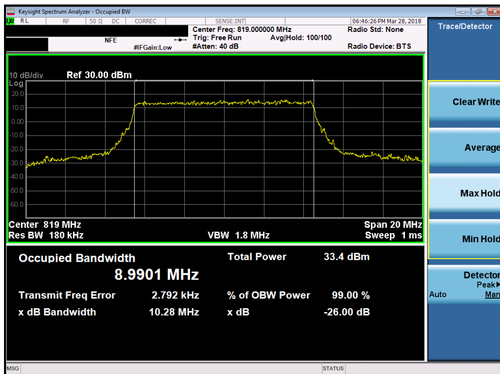
Plot 7-11. Occupied Bandwidth Plot (LTE Band 26 - 10MHz QPSK – RB Size 50)
