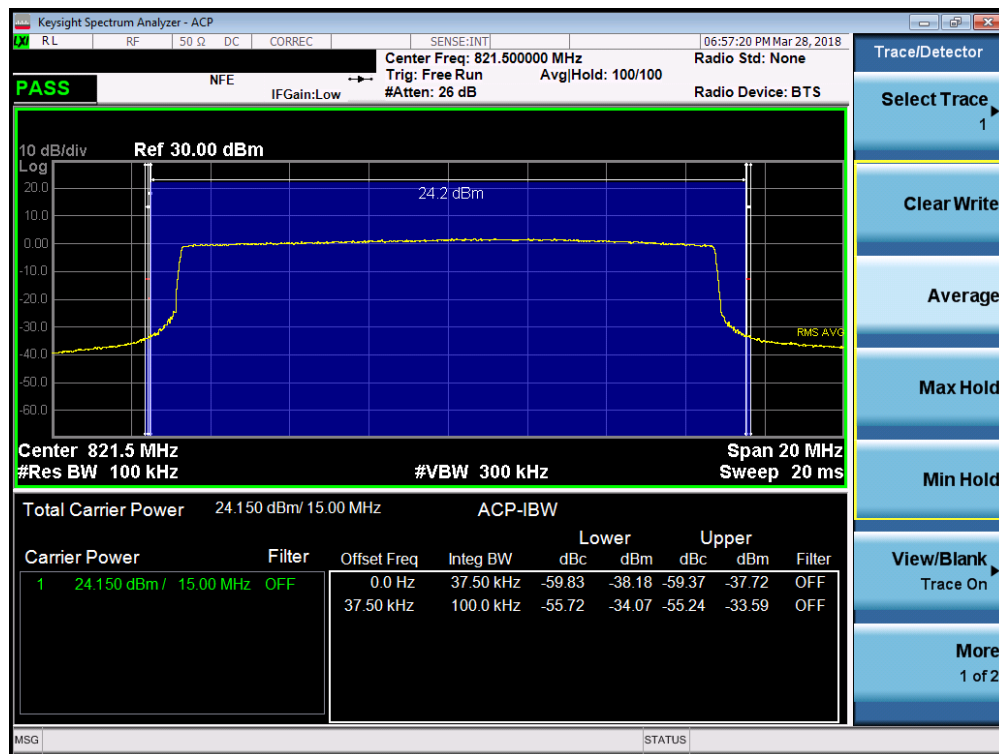
Plot 7-38. Channel Edge Plot (LTE Band 26 - 15MHz QPSK – RB Size 75)
