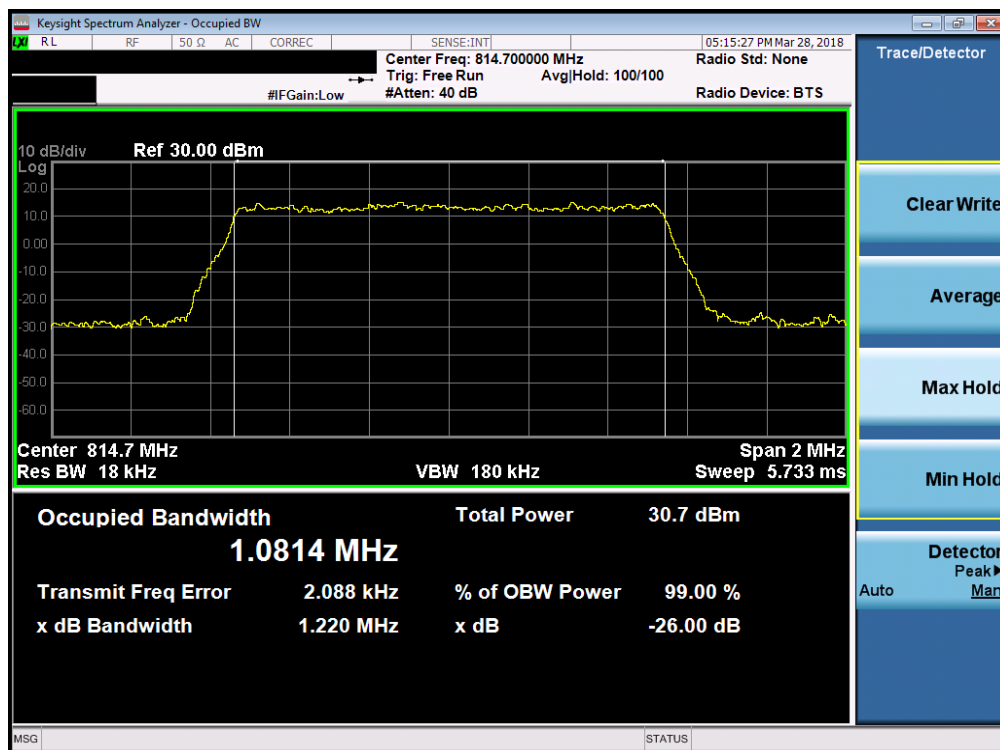
Plot 7-4. Occupied Bandwidth Plot (LTE Band 26 - 1.4MHz 64-QAM – RB Size 6– Low Channel)
