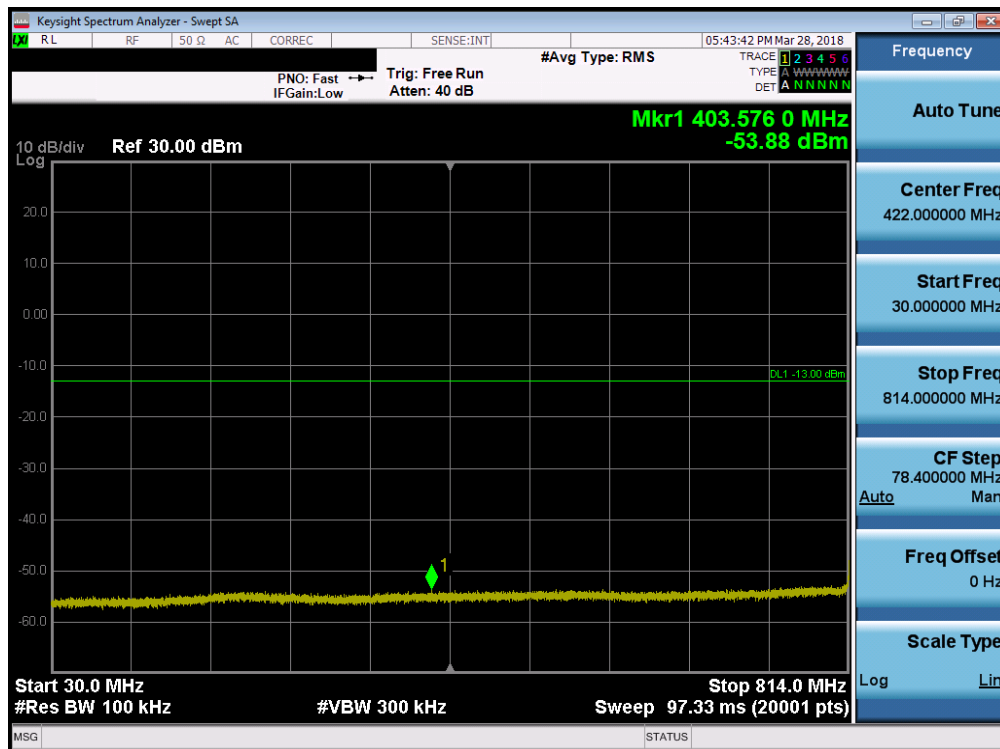
Plot 7-23. Conducted Spurious Plot (LTE Band 26 - 5 MHz QPSK – RB Size 1, RB Offset 0 – Low Channel)
