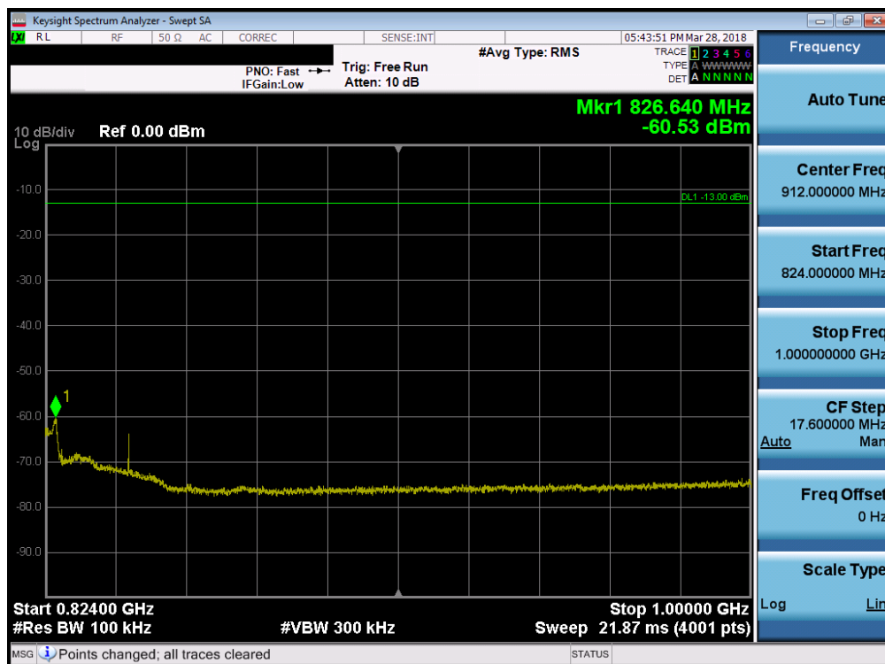
Plot 7-24. Conducted Spurious Plot (LTE Band 26 - 5 MHz QPSK – RB Size 1, RB Offset 0 – Low Channel)
