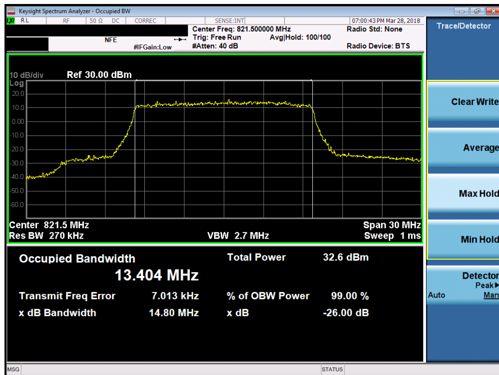
Plot 7-15. Occupied Bandwidth Plot (LTE Band 26 - 15MHz 16-QAM – RB Size 75)
