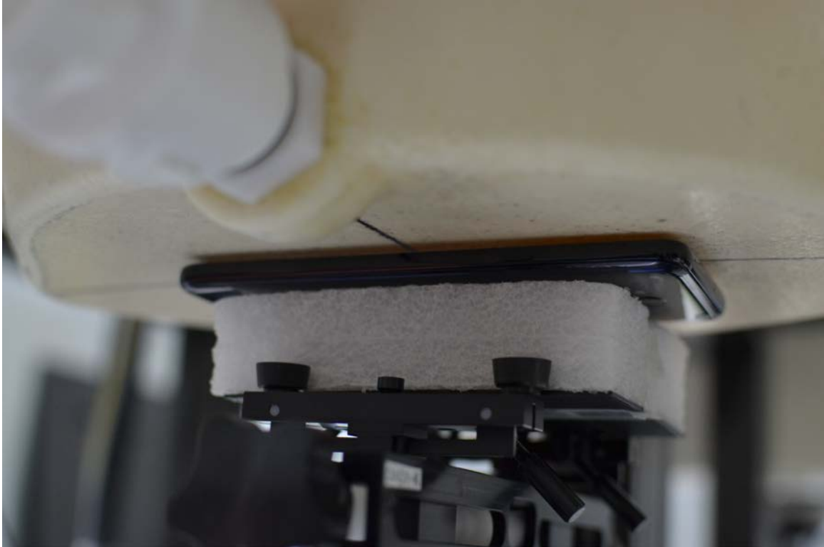
SAR Test Setup Photo 9: Front at 0.2 cm
