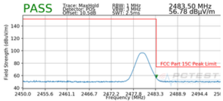
Plot 7-36. Radiated Restricted Upper Band Edge Measurement (Peak)
