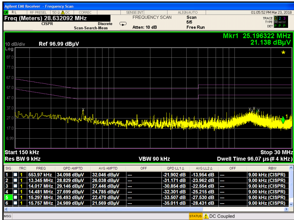
Plot 7-45. Line Conducted Plot with Bluetooth LE (L1) with WCP
