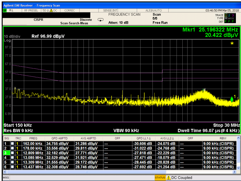
Plot 7-43. Line Conducted Plot with Bluetooth LE (L1)
