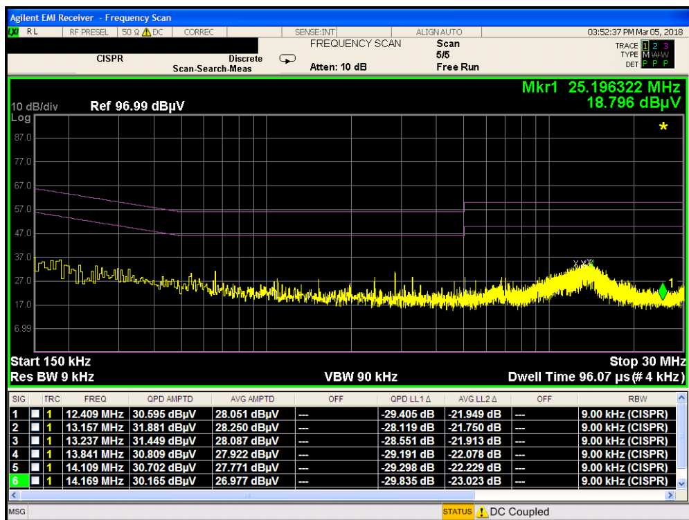
Plot 7-44. Line Conducted Plot with Bluetooth LE (N)
