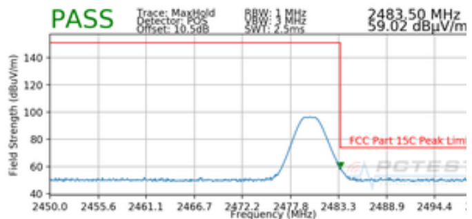
Plot 7-42. Radiated Restricted Upper Band Edge Measurement with WCP (Peak)
