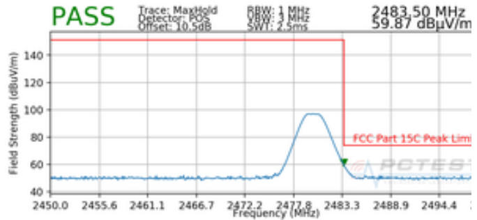
Plot 7-40. Radiated Restricted Upper Band Edge Measurement (Peak)
