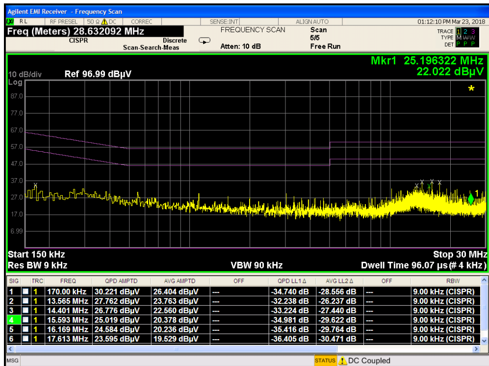
Plot 7-46. Line Conducted Plot with Bluetooth LE (N) with WCP
