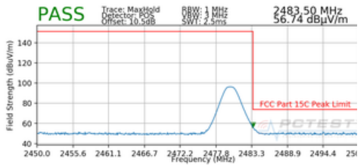
Plot 7-38. Radiated Restricted Upper Band Edge Measurement with WCP (Peak)
