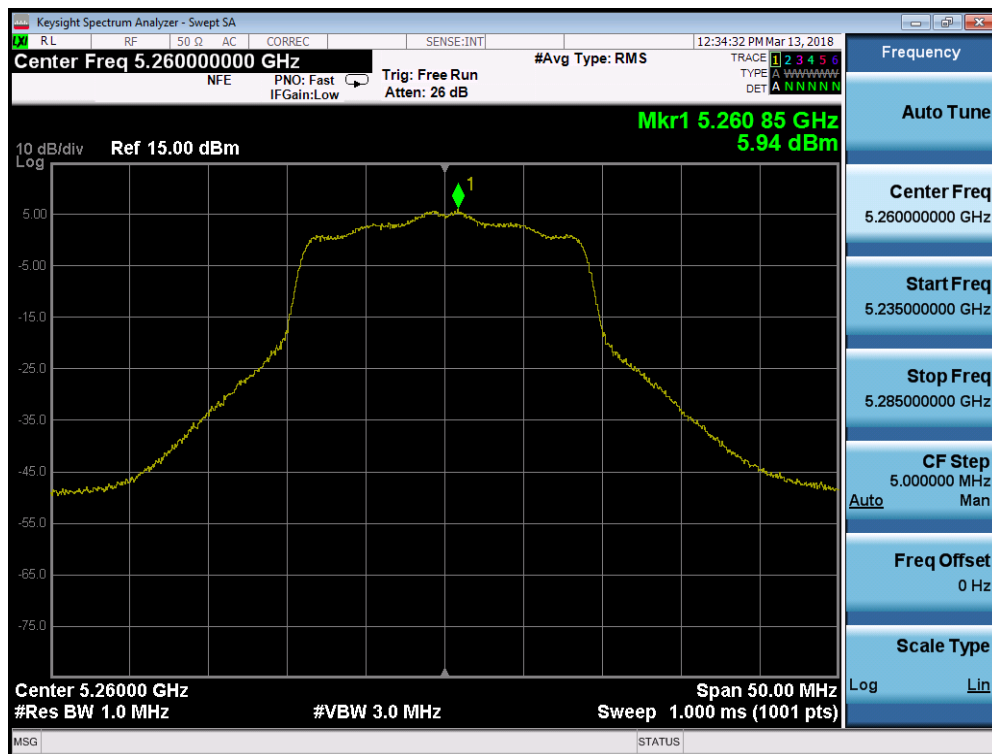
Plot 7-89. Power Spectral Density Plot (20MHz BW 802.11n (UNII Band 2A) – Ch. 52)
