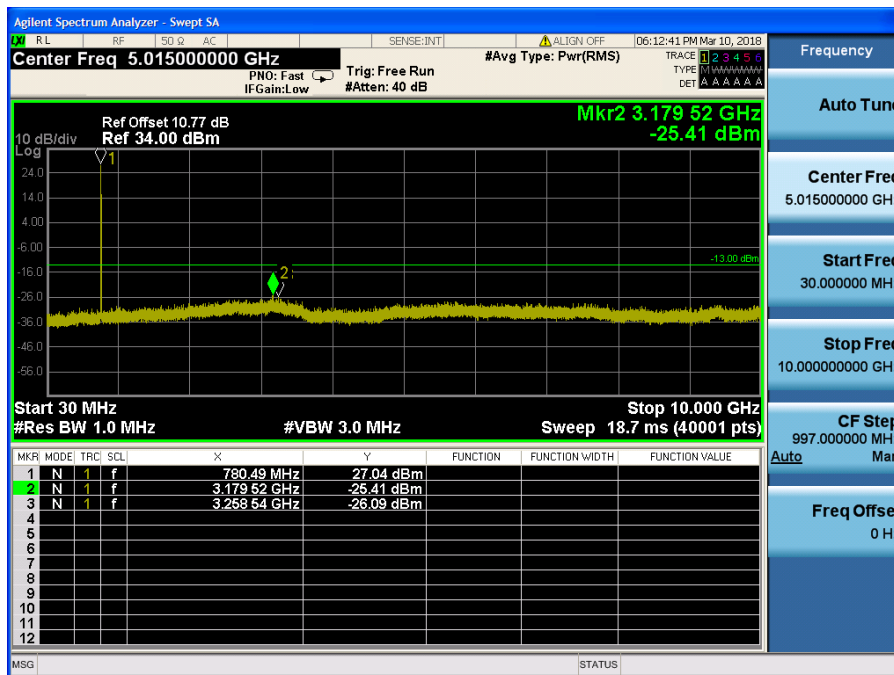
LTE Band 13 / 10MHz / 64QAM - RB Size/Offset (25/12) – Low Channel
