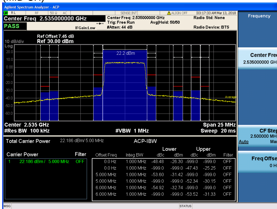
LTE Band 7 / 5MHz / 64QAM - RB Size/Offset (25/0)
