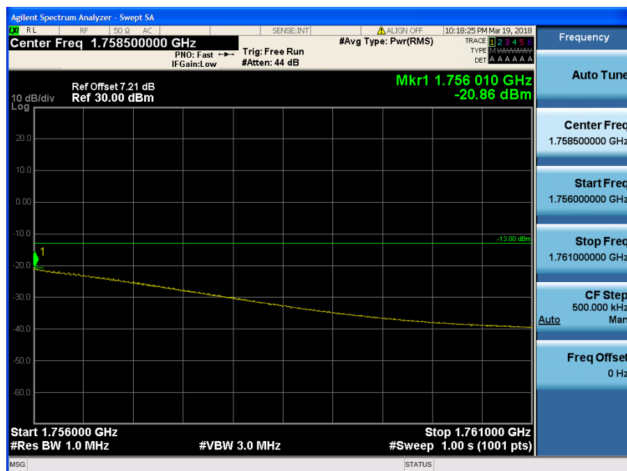
LTE Band 4 / 3MHz / 64QAM - RB Size/Offset (8/4)
