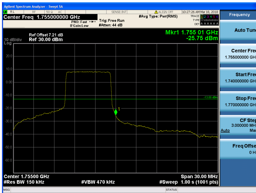
LTE Band 4 / 15MHz / QPSK - RB Size/Offset (36/39)
