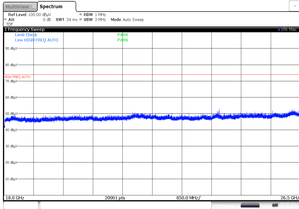
Plot 7-7. Radiated Spurious Plot above 18GHz (Pol. H)
