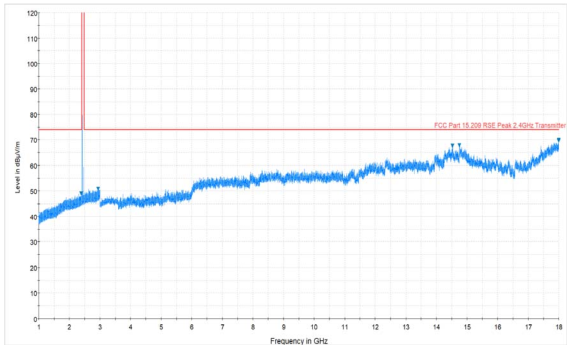
Plot 7-2. Radiated Spurious Plot above 1GHz (BT – Ch. 0, Ant. Pol. V)
