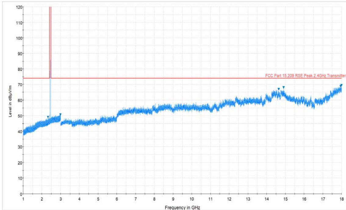
Plot 7-1. Radiated Spurious Plot above 1GHz (BT – Ch. 0, Ant. Pol. H)
