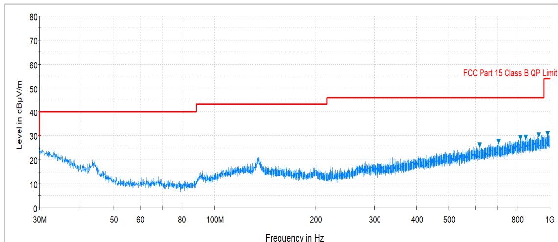
Plot 7-12. Radiated Spurious Plot below 1GHz (Pol. V)
