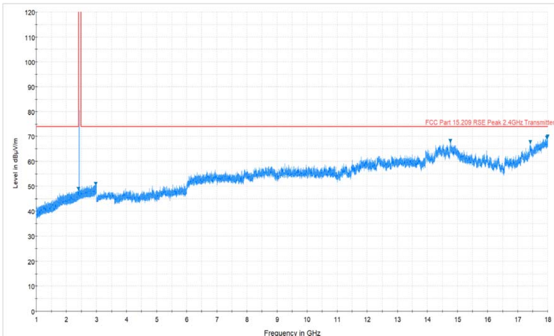
Plot 7-4. Radiated Spurious Plot above 1GHz (BT – Ch. 39, Ant. Pol. V)
