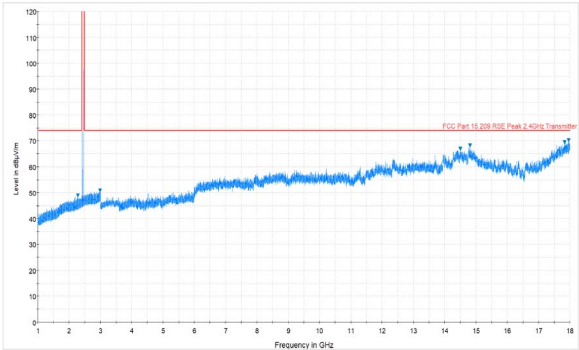
Plot 7-5. Radiated Spurious Plot above 1GHz (BT – Ch. 78, Ant. Pol. H)
