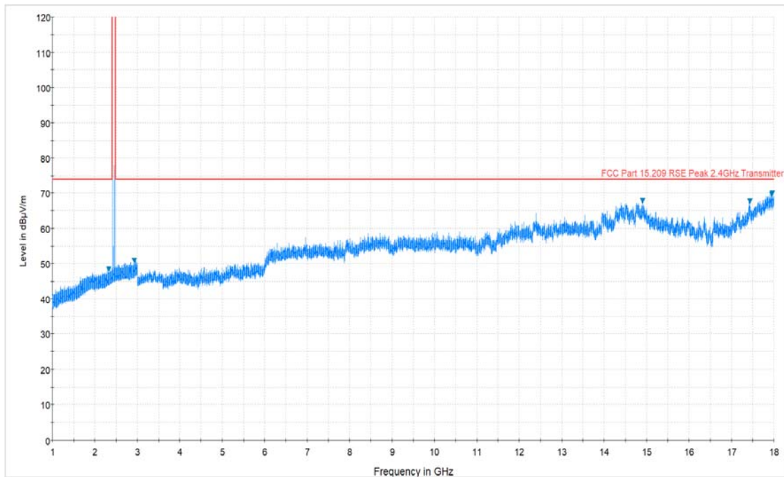
Plot 7-3. Radiated Spurious Plot above 1GHz (BT – Ch. 39, Ant. Pol. H)
