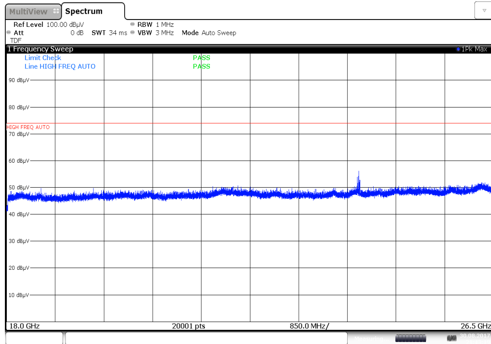
Plot 7-8. Radiated Spurious Plot above 18GHz (Pol. V)
