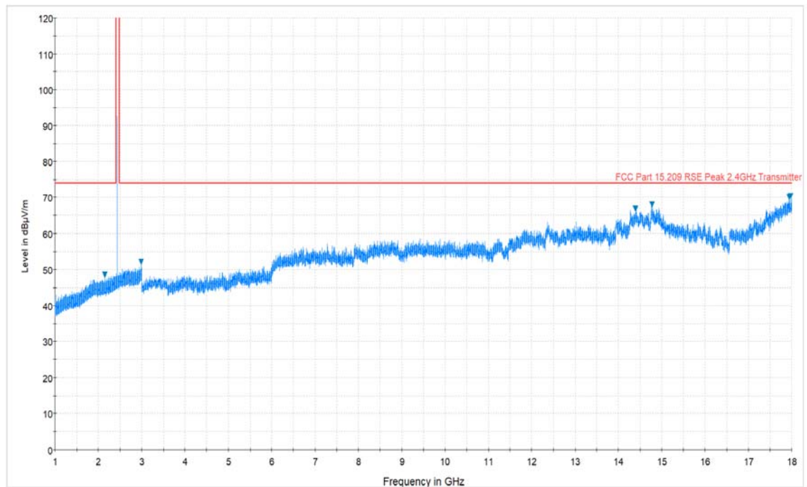
Plot 7-6. Radiated Spurious Plot above 1GHz (BT – Ch. 78, Ant. Pol. V)
