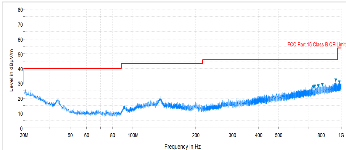
Plot 7-11. Radiated Spurious Plot below 1GHz (Pol. H)
