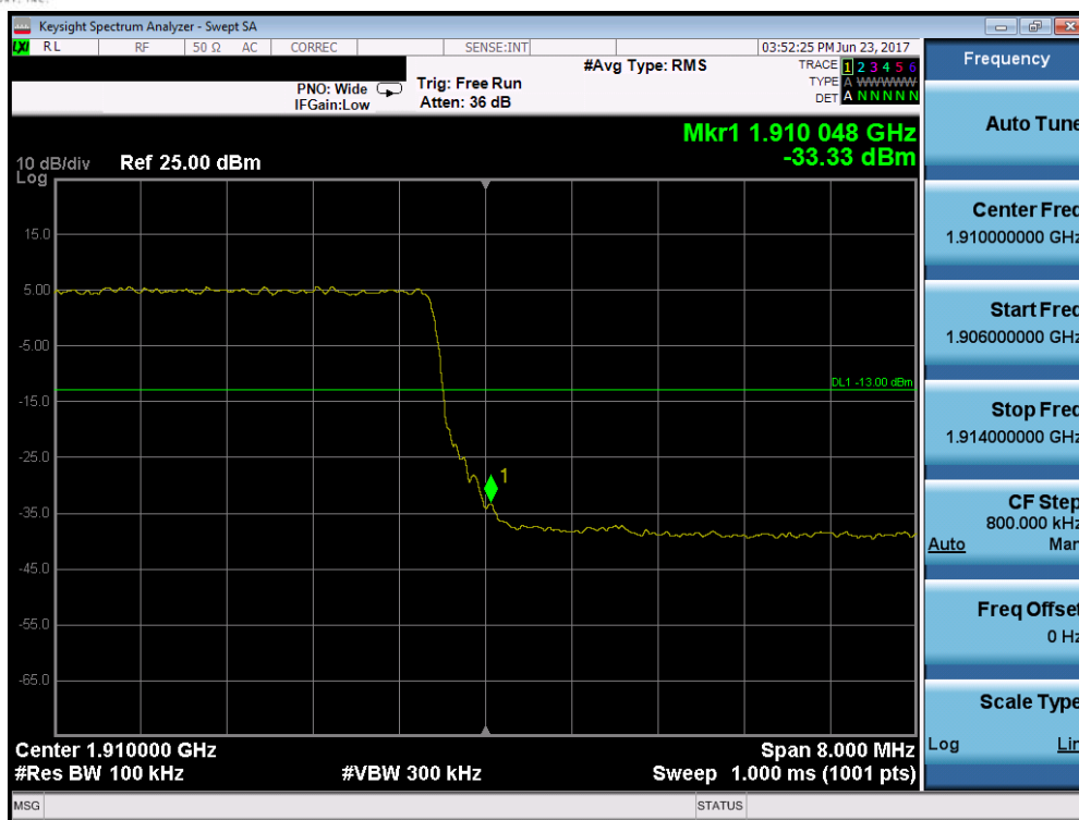
Plot 7-260. Upper Band Edge Plot (Band 2 – 10.0MHz QPSK – RB Size 50)
