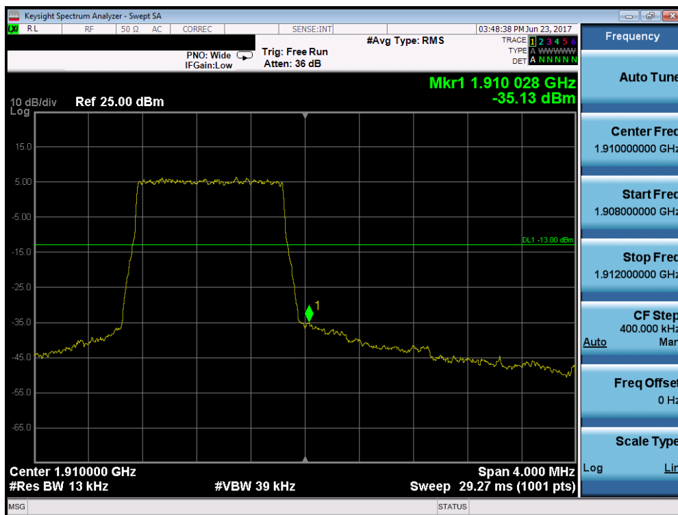
Plot 7-254. Upper Band Edge Plot (Band 2 – 1.4MHz QPSK – RB Size 6)
