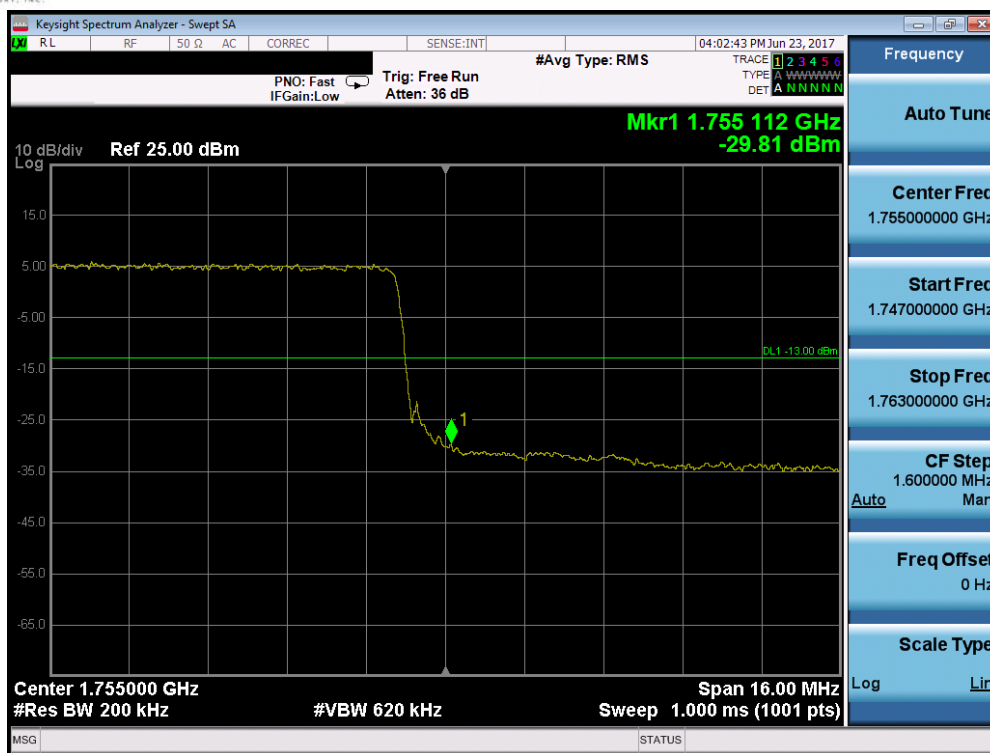
Plot 7-228. Upper Band Edge Plot (Band 4 – 20.0MHz QPSK – RB Size 100)
