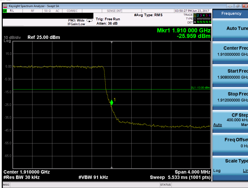
Plot 7-256. Upper Band Edge Plot (Band 2 – 3.0MHz QPSK – RB Size 15)
