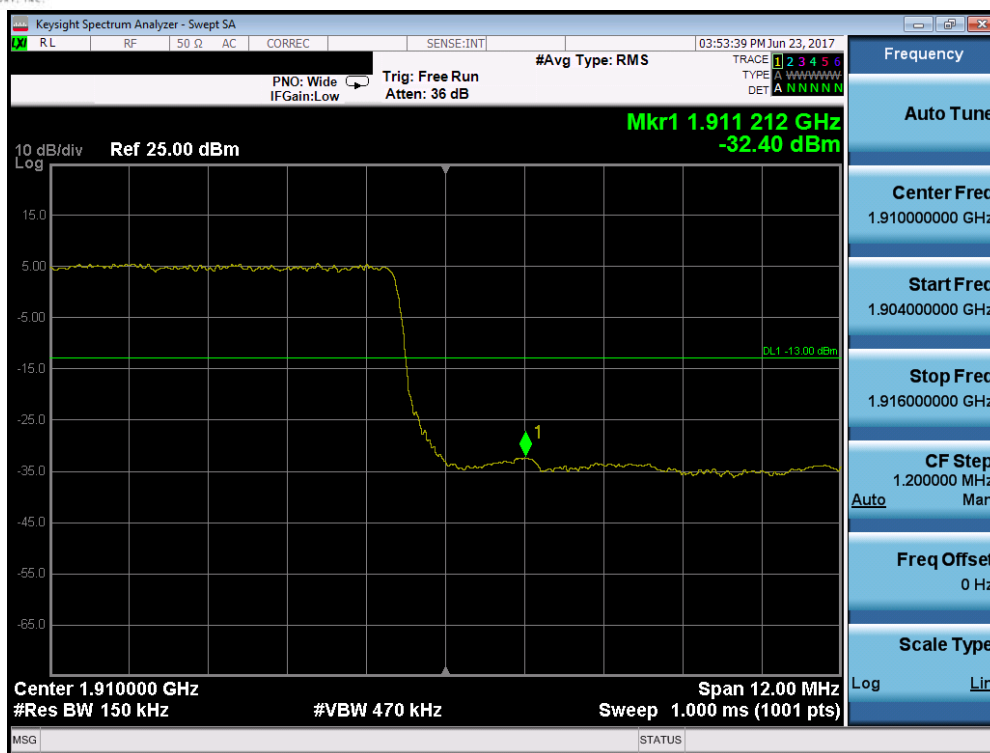
Plot 7-262. Upper Band Edge Plot (Band 2 – 15.0MHz QPSK – RB Size 75)
