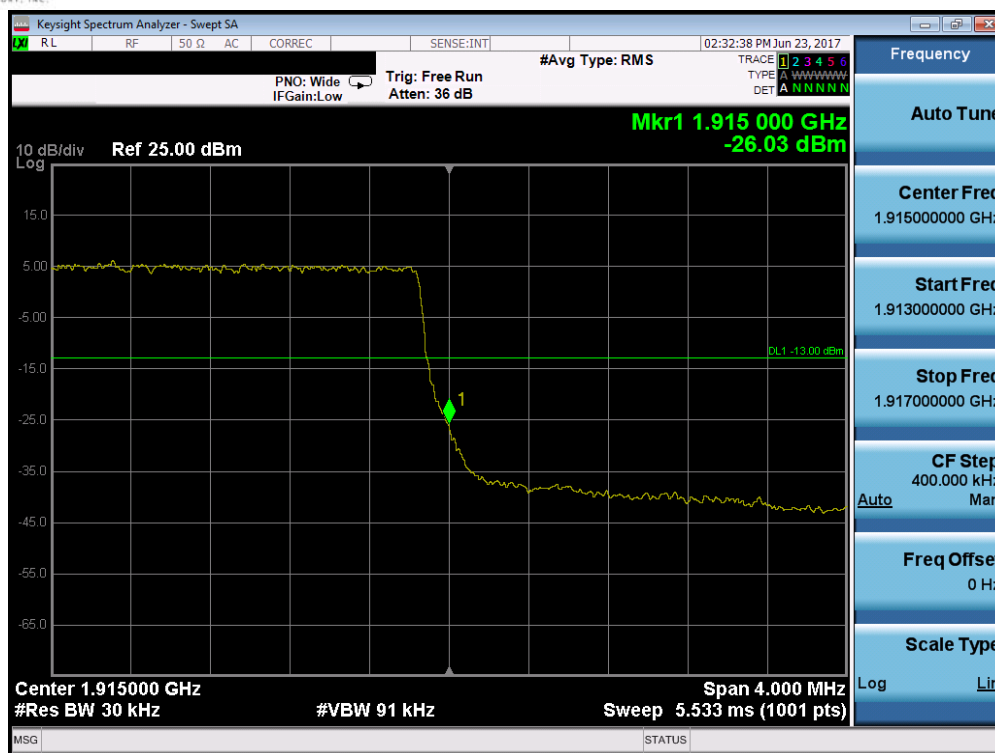
Plot 7-236. Upper Band Edge Plot (Band 25 – 3.0MHz QPSK – RB Size 15)
