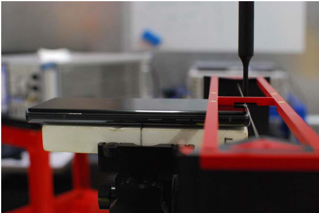
Figure 18-2 HAC Phantom Plane Alignment – Normal Mode
