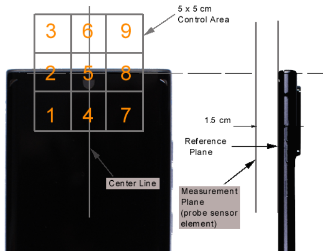
Figure 18-5 5x5 Scan grid above WD
