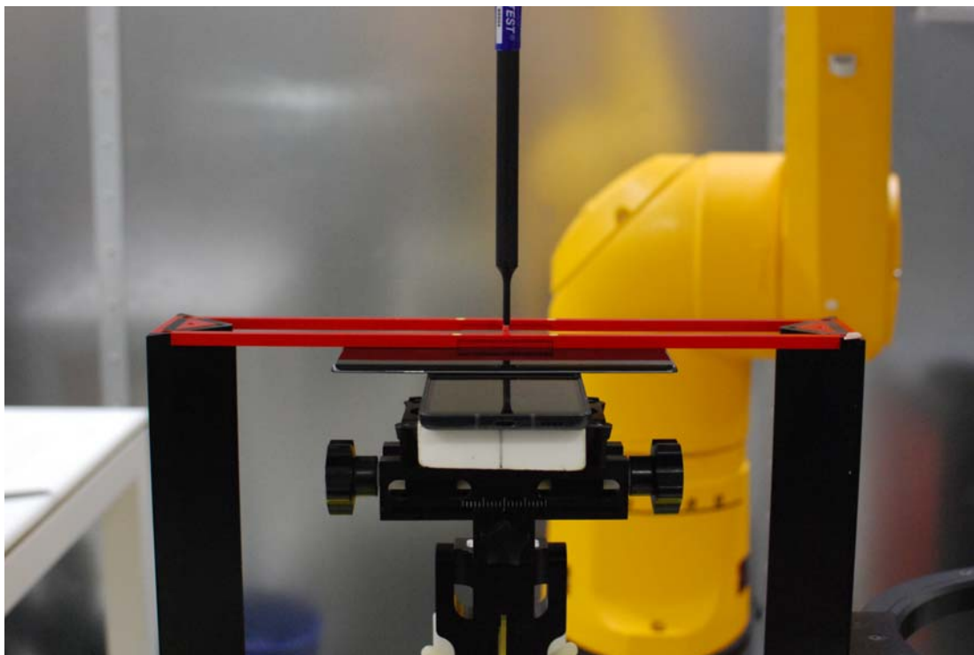
Figure 18-3 Ear Reference Point HAC Phantom Alignment – Swivel Mode
