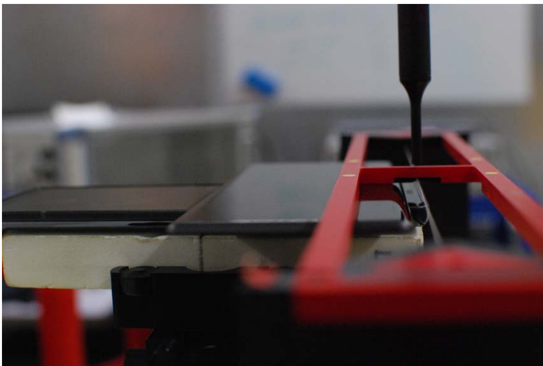
Figure 18-4 HAC Phantom Plane Alignment – Swivel Mode
