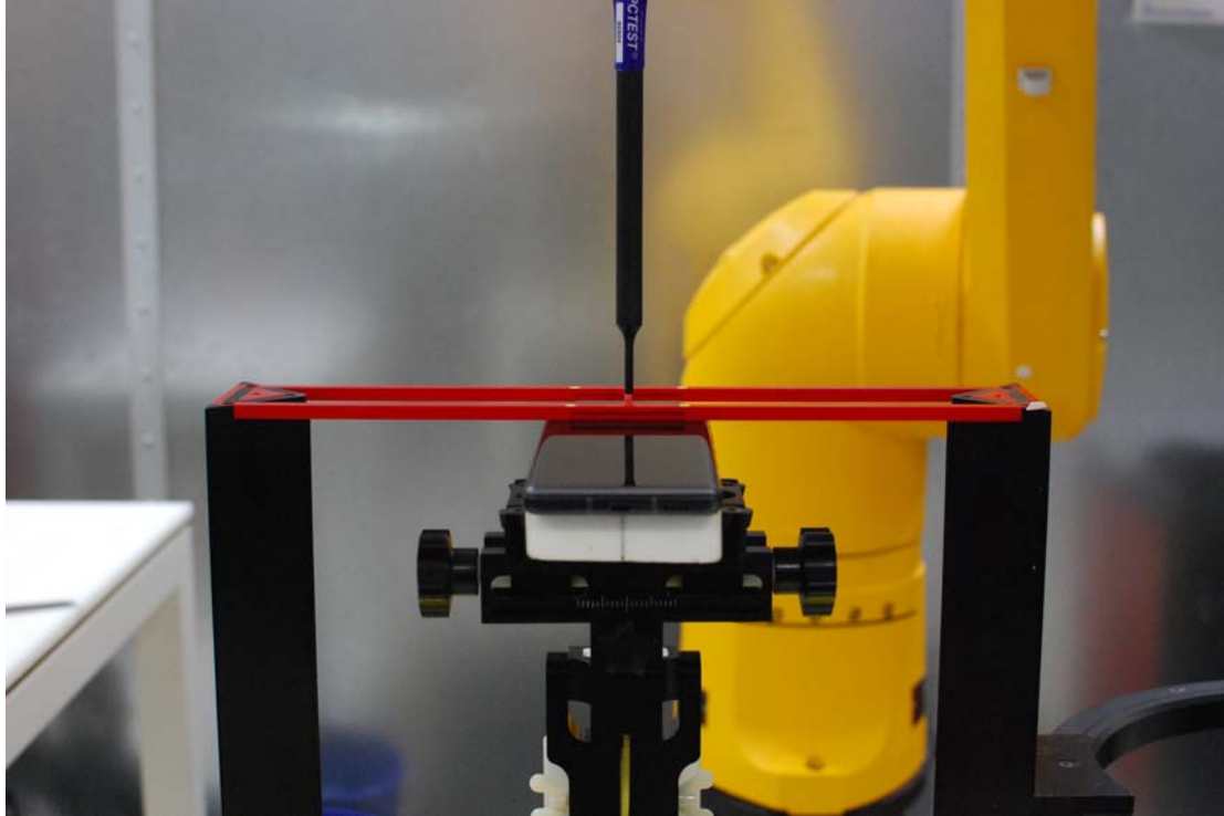
Figure 18-1 Ear Reference Point HAC Phantom Alignment – Normal Mode
