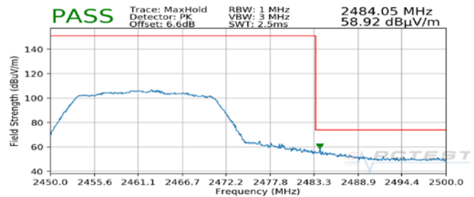
Plot 7-14. Radiated Restricted Band Edge Measurement MIMO with WCP (Peak)
