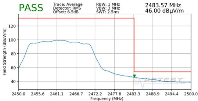
Plot 7-3. Radiated Restricted Upper Band Edge Measurement SISO ANT1 (Average)
