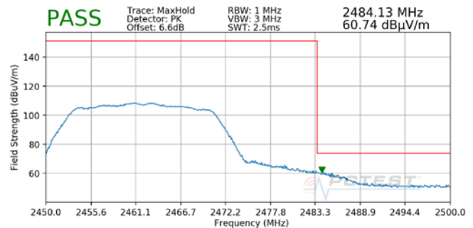
Plot 7-12. Radiated Restricted Upper Band Edge Measurement MIMO (Peak)
