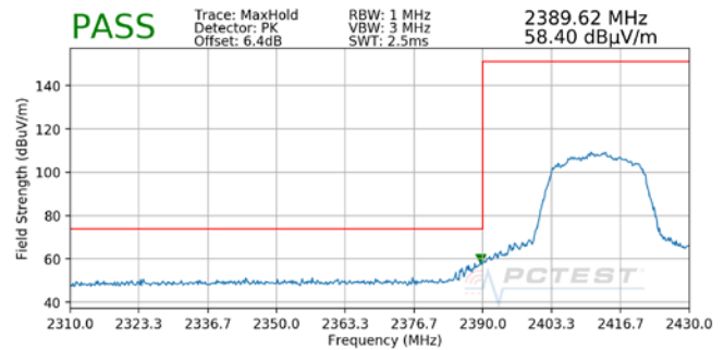
Plot 7-10. Radiated Restricted Lower Band Edge Measurement MIMO (Peak)
