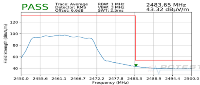
Plot 7-13. Radiated Restricted Band Edge Measurement MIMO with WCP (Average)
