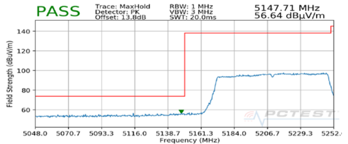
Plot 7-37. Radiated Lower Band Edge Plot SISO ANT2 (Peak – UNII Band 1)
