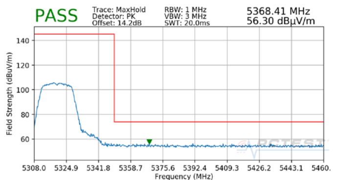
Plot 7-4. Radiated Upper Band Edge Plot SISO ANT1 (Peak – UNII Band 2A)
