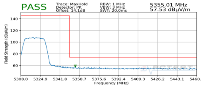
Plot 7-25. Radiated Upper Band Edge Plot SISO ANT2 (Peak – UNII Band 2A)
