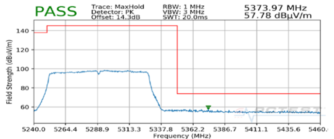
Plot 7-39. Radiated Upper Band Edge Plot SISO ANT2 (Peak – UNII Band 2A)
