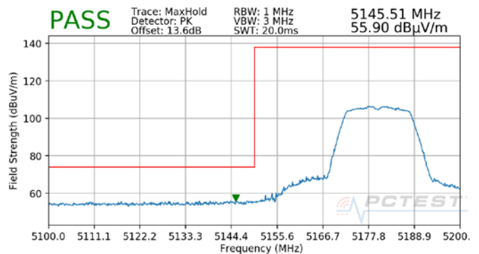
Plot 7-2. Radiated Lower Band Edge Plot SISO ANT1 (Peak – UNII Band 1)
