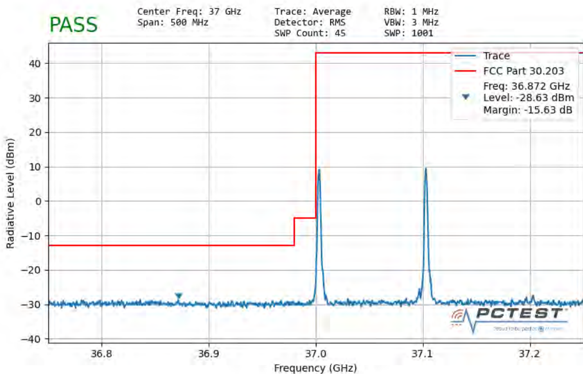
Plot 7-76. Ant 3 Lower Band Edge (100MHz-2CC – \pi/2 BPSK 1 RB)
