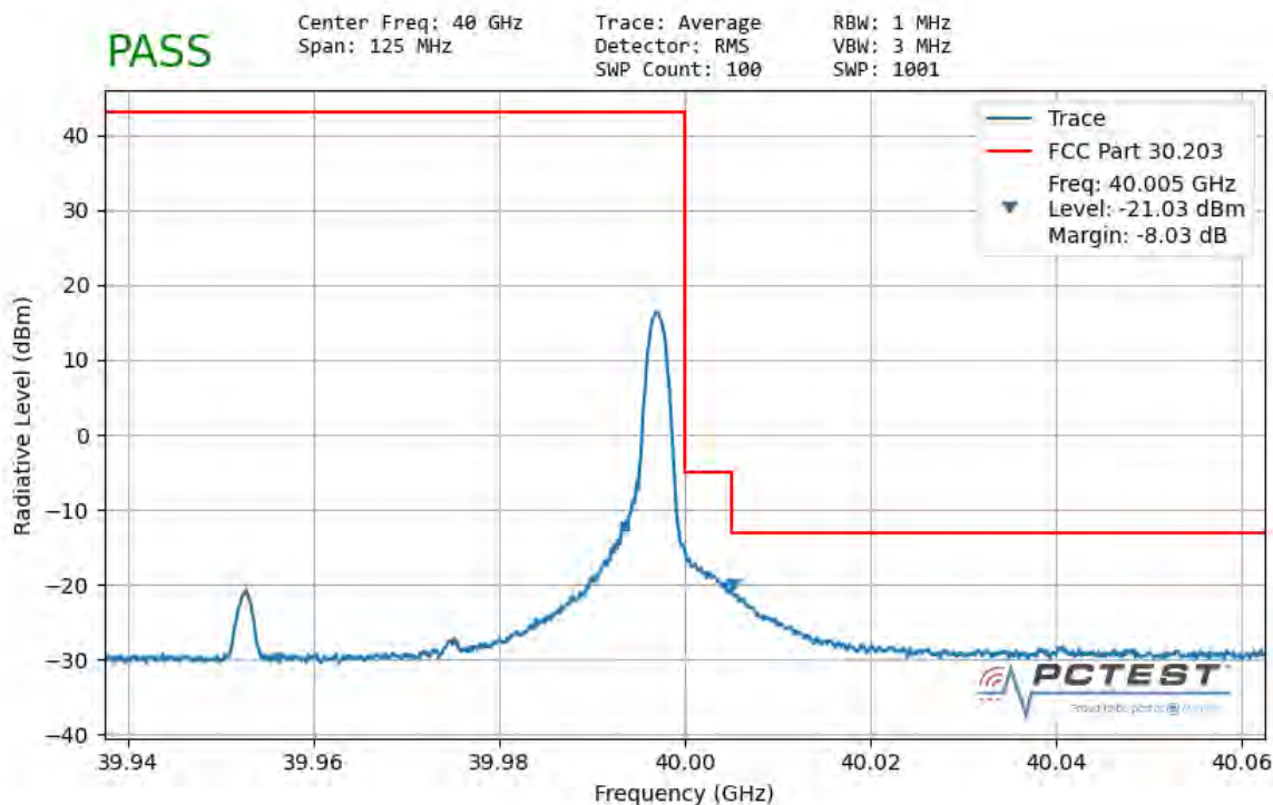
Plot 7-89. Ant 2 Upper Band Edge (50MHz-1CC – \pi/2 BPSK 1 RB)
