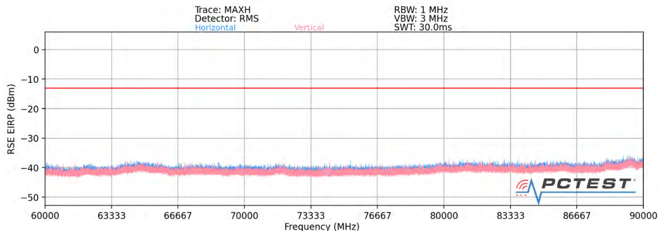
Plot 7-38. Ant 2-n261 Radiated Spurious Plot (1CC \pi/2 BPSK Mid Channel MIMO)
