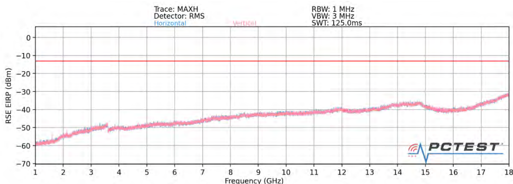
Plot 7-48. Ant 3 - n260 Radiated Spurious Plot (1CC \pi/2 BPSK Mid Channel MIMO)
