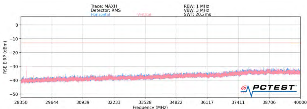
Plot 7-36. Ant 2 - n261 Radiated Spurious Plot (1CC \pi/2 BPSK Mid Channel MIMO)
