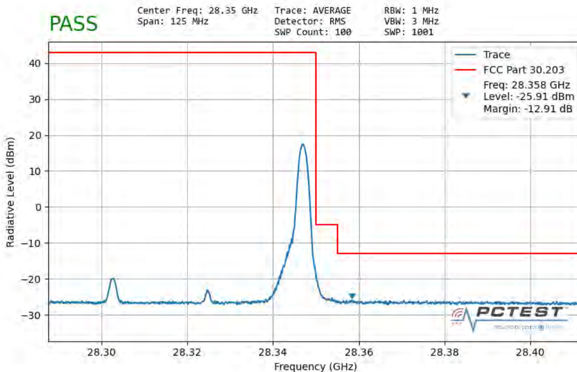
Plot 7-73. Ant 3 Upper Band Edge (50MHz-1CC – \pi/2 BPSK 1 RB)
