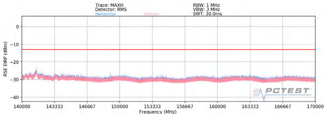
Plot 7-53. Ant 3 - n260 Radiated Spurious Plot (1CC \pi/2 BPSK Mid Channel MIMO)
