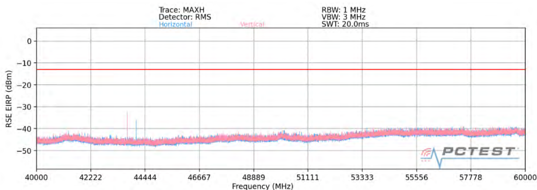
Plot 7-50. Ant 1-n260 Radiated Spurious Plot (1CC \pi/2 BPSK Mid Channel MIMO)
