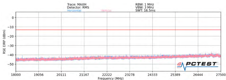
Plot 7-35. Ant 1-n261 Radiated Spurious Plot (1CC \pi/2 BPSK Mid Channel MIMO)
