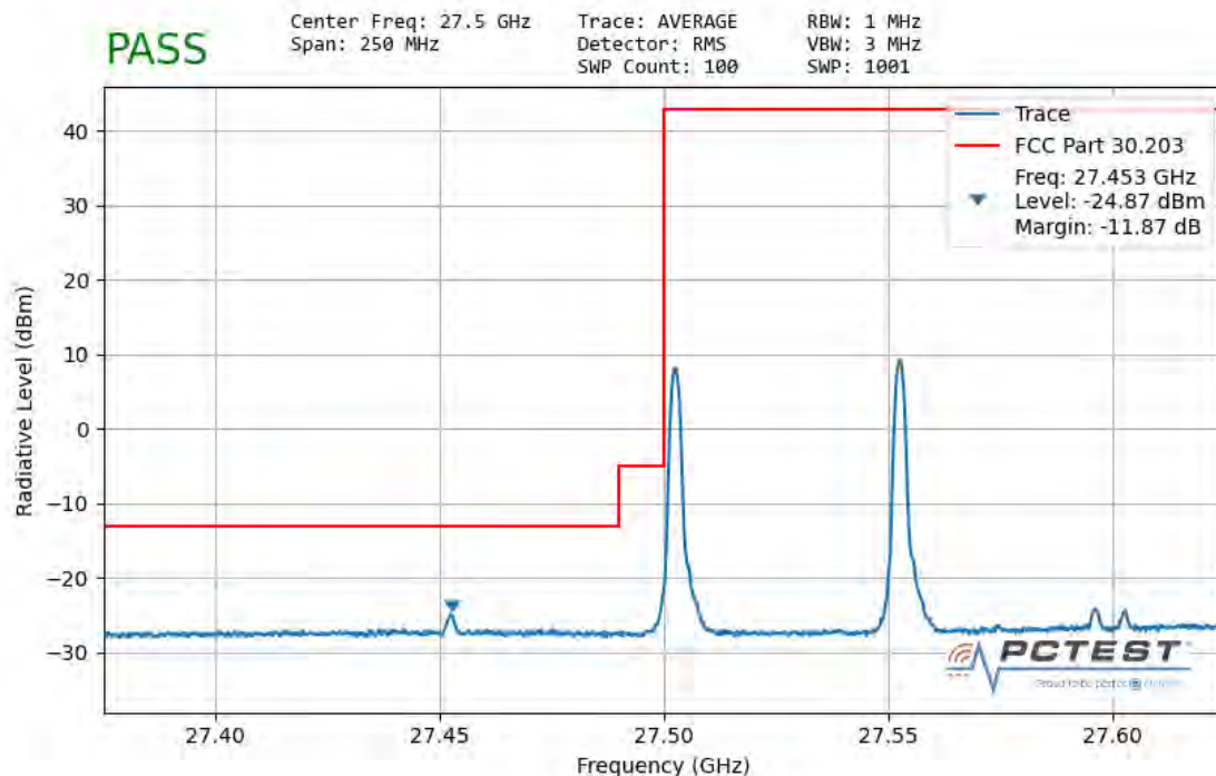
Plot 7-64. Ant 1 Lower Band Edge (50MHz-2CC – \pi/2 BPSK 1 RB)
