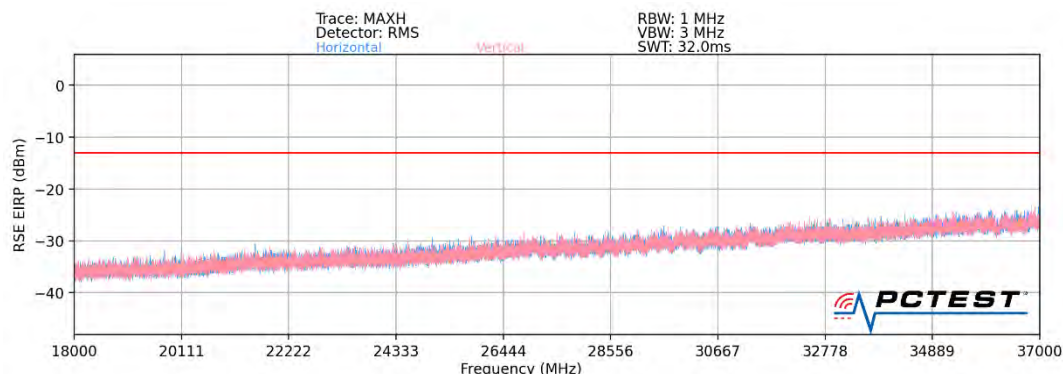
Plot 7-49. Ant 3 - n260 Radiated Spurious Plot (1CC \pi/2 BPSK Mid Channel MIMO)
