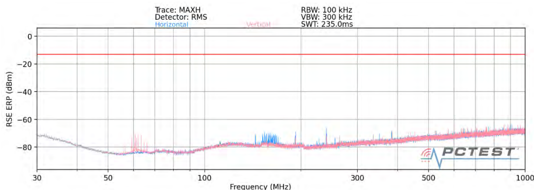
Plot 7-47. Ant 1-n260 Radiated Spurious Plot (1CC \pi/2 BPSK Mid Channel MIMO)
