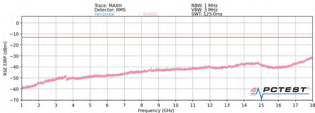
Plot 7-34. Ant 3 - n261 Radiated Spurious Plot (1CC \pi/2 BPSK Mid Channel MIMO)
