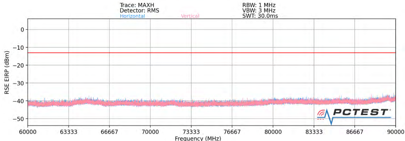
Plot 7-4. Ant 1-n260 Radiated Spurious Plot (1CC \pi/2 BPSK Mid Channel MIMO)
