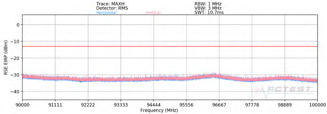
Plot 7-39. Ant 1-n261 Radiated Spurious Plot (1CC \pi/2 BPSK Mid Channel MIMO)
