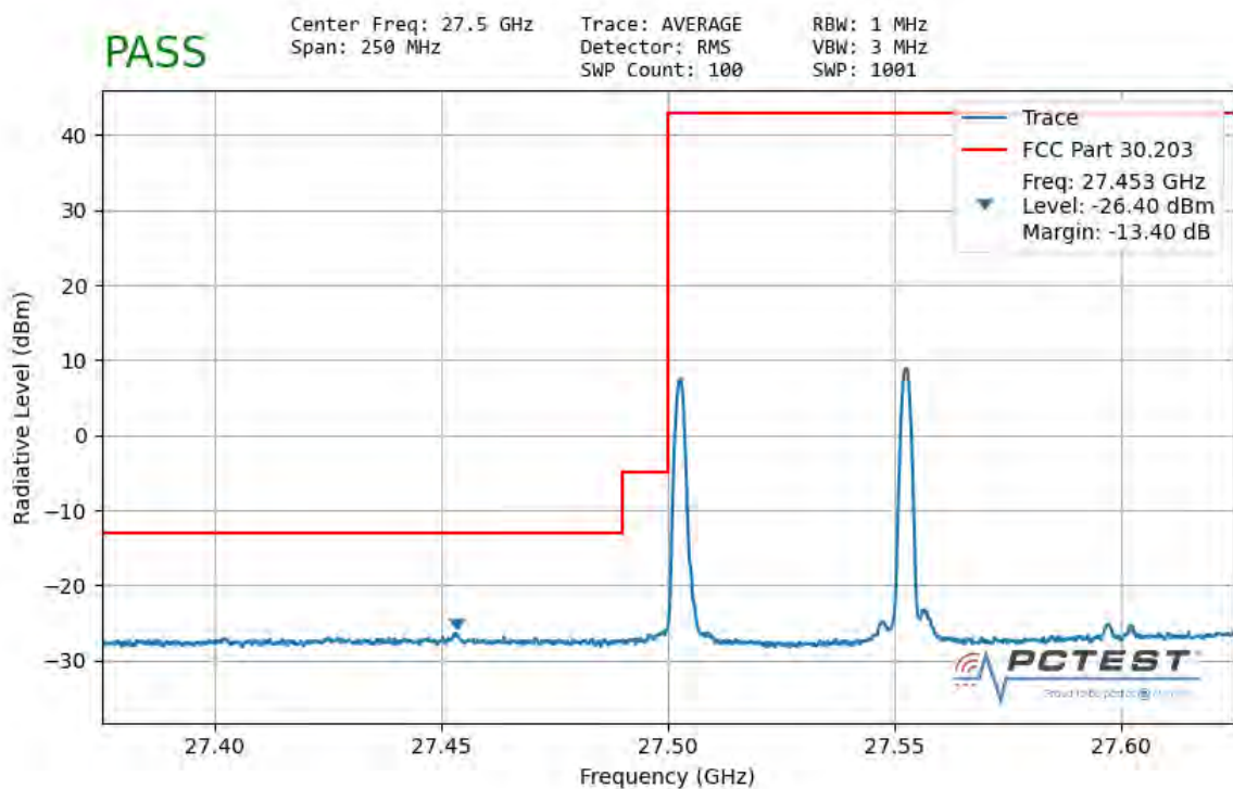
Plot 7-72. Ant 2 Lower Band Edge (50MHz-2CC – \pi/2 BPSK 1 RB)
