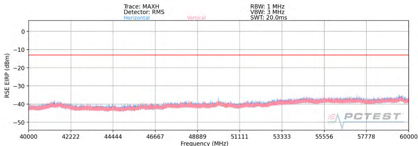
Plot 7-44. Ant 2-n261 Radiated Spurious Plot (1CC \pi/2 BPSK Mid Channel MIMO)
