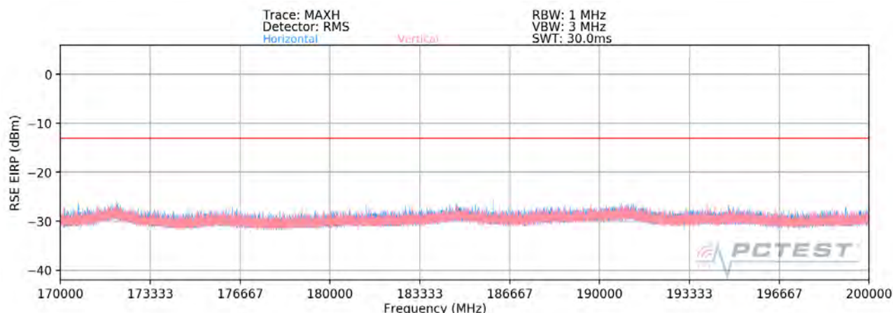
Plot 7-54. Ant 2 - n260 Radiated Spurious Plot (1CC \pi/2 BPSK Mid Channel MIMO)
