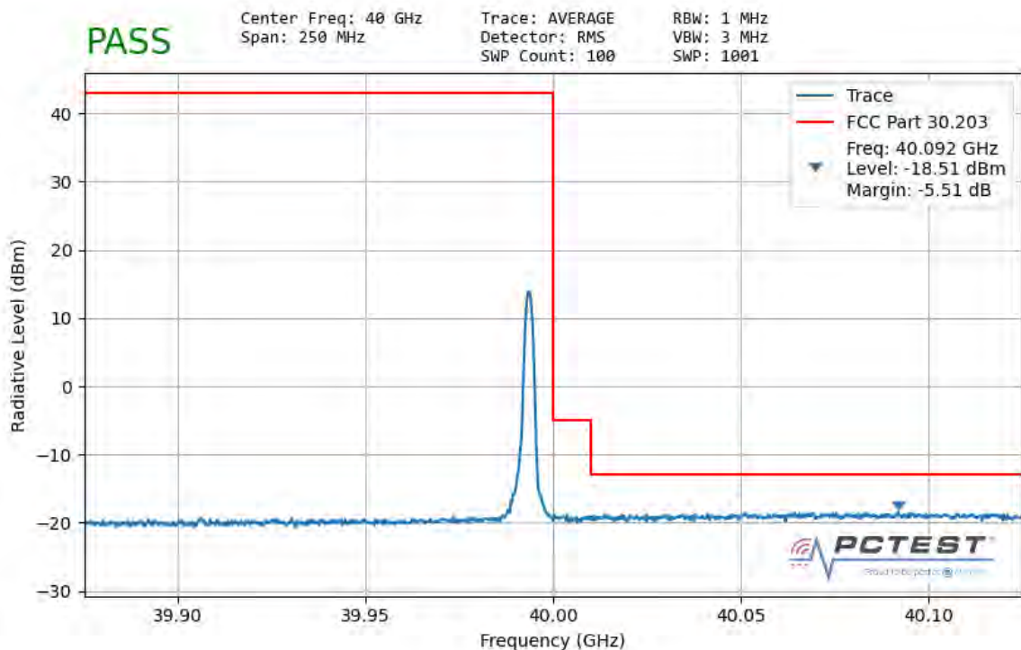
Plot 7-85. Ant 1 Upper Band Edge (100MHz-1CC – \pi/2 BPSK 1 RB)
