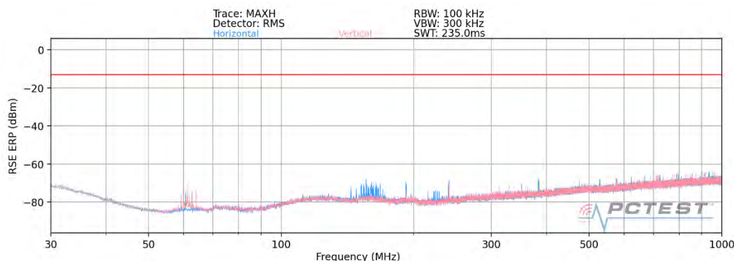
Plot 7-2. Ant 2 - n261 Radiated Spurious Plot (1CC \pi/2 BPSK Mid Channel MIMO)
