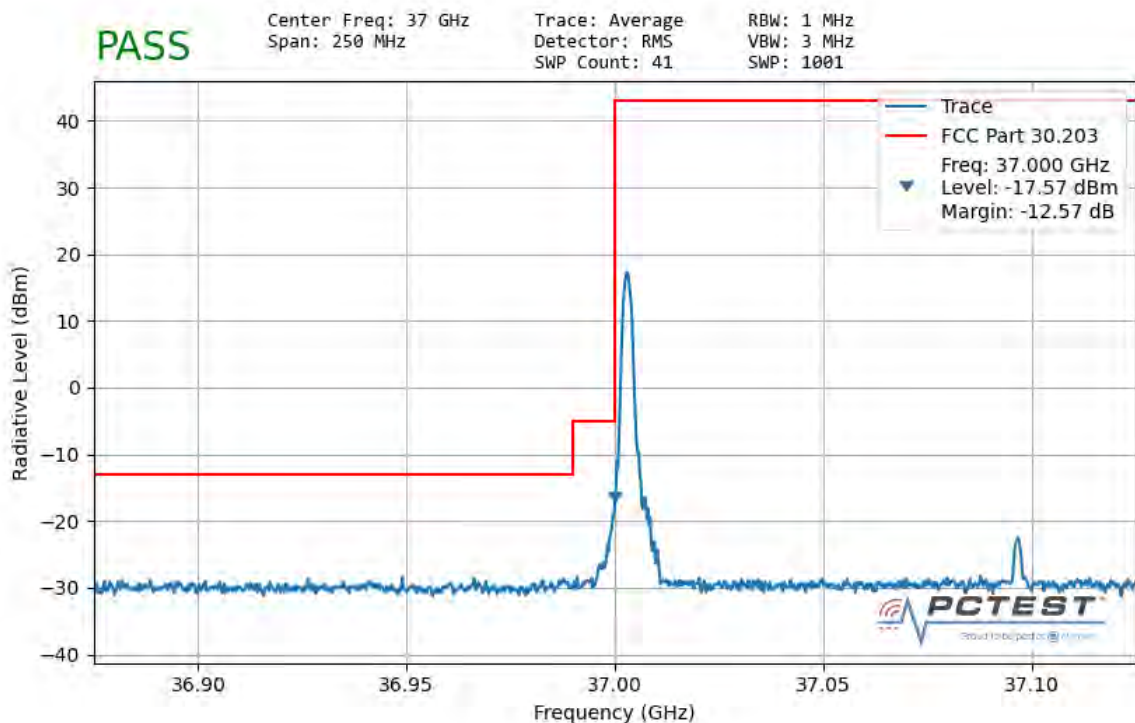
Plot 7-75. Ant 3 Lower Band Edge (100MHz-1CC – \pi/2 BPSK 1 RB)
