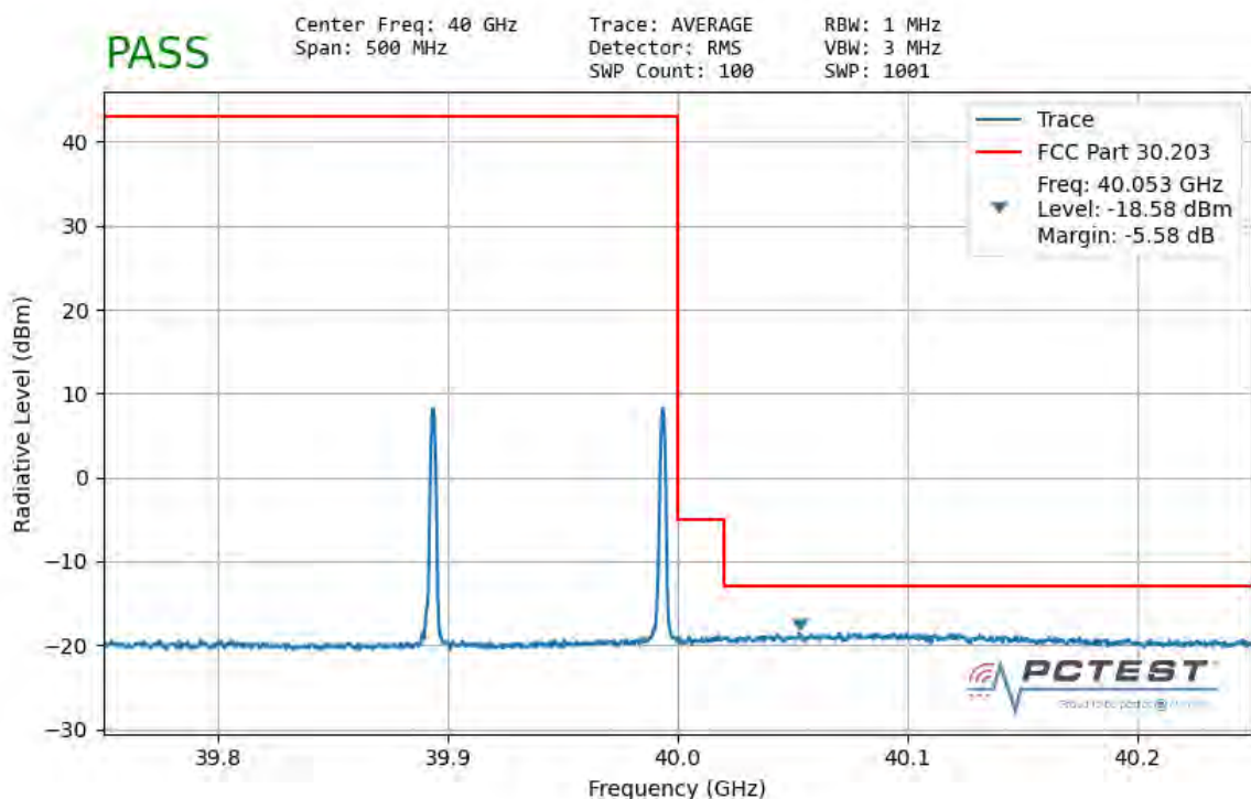
Plot 7-86. Ant 1 Upper Band Edge (100MHz-2CC – \pi/2 BPSK 1 RB)
