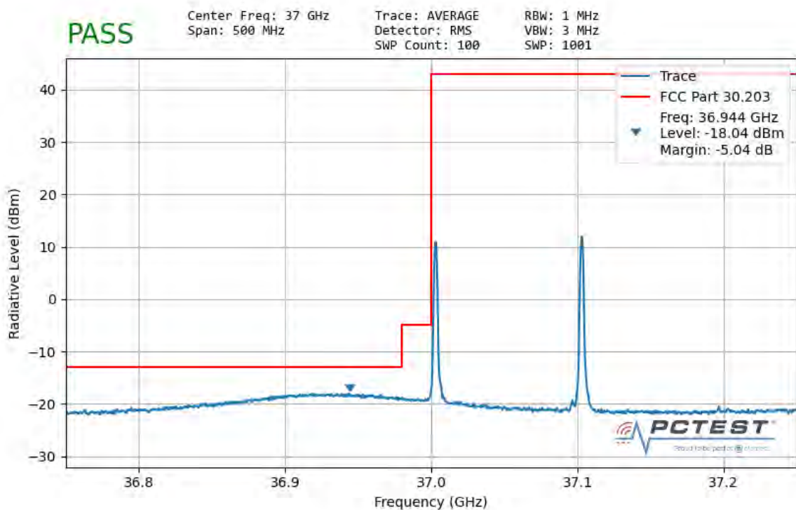
Plot 7-84. Ant 1 Lower Band Edge (100MHz-2CC – \pi/2 BPSK 1 RB)
