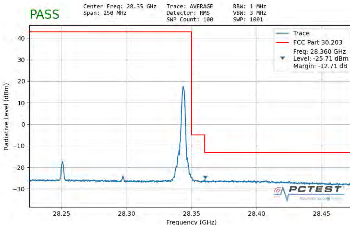
Plot 7-77. Ant 3 Upper Band Edge (100MHz-1CC – \pi/2 BPSK 1 RB)
