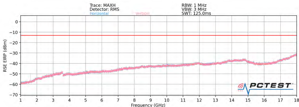
Plot 7-34. Ant 2 - n261 Radiated Spurious Plot (1CC \pi/2 BPSK Mid Channel MIMO)
