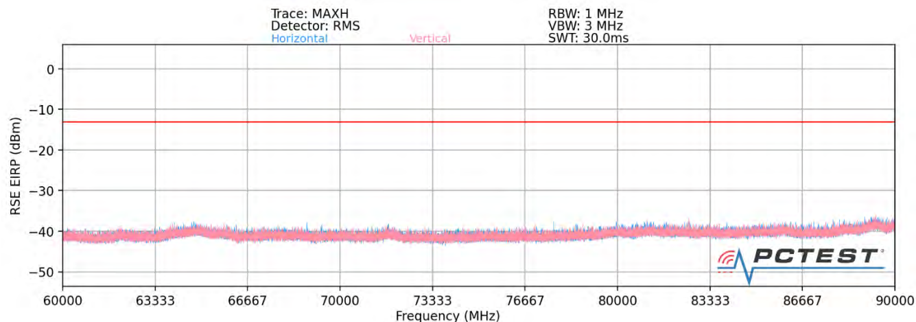
Plot 7-38. Ant 3-n261 Radiated Spurious Plot (1CC \pi/2 BPSK Mid Channel MIMO)
