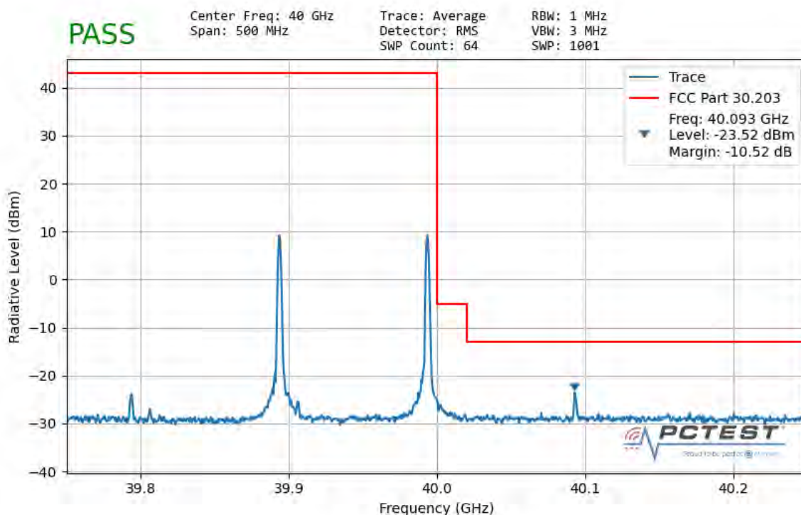
Plot 7-94. Ant 2 Upper Band Edge (100MHz-2CC – \pi/2 BPSK 1 RB)
