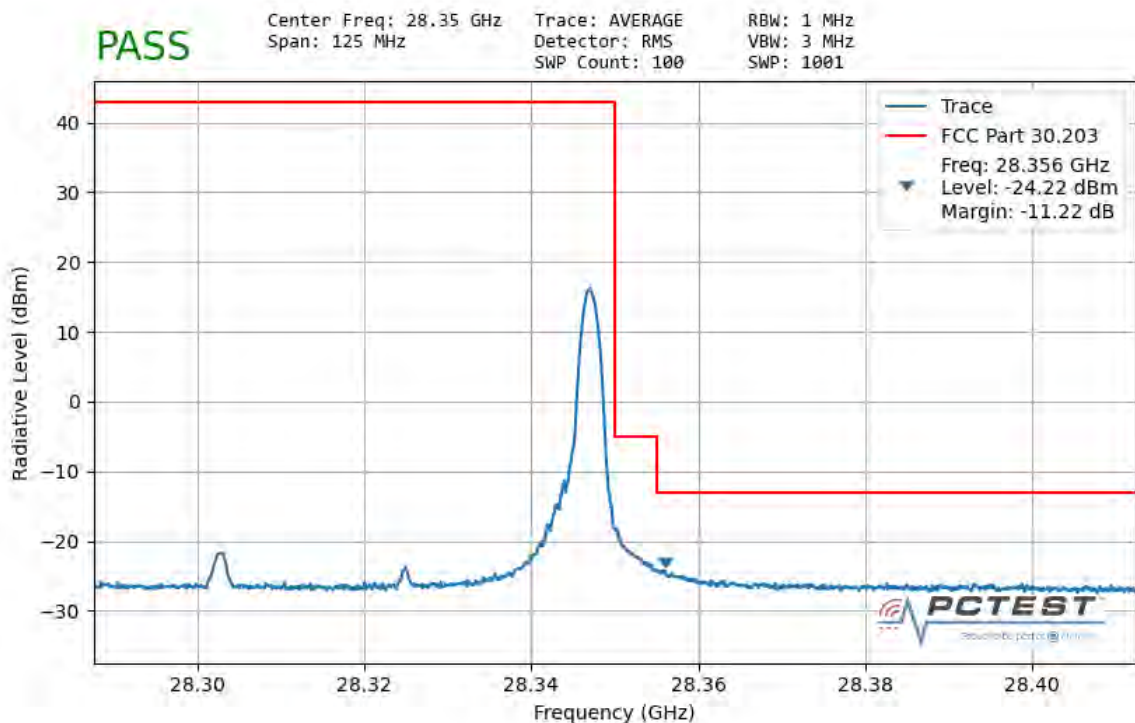
Plot 7-73. Ant 2 Upper Band Edge (50MHz-1CC – \pi/2 BPSK 1 RB)
