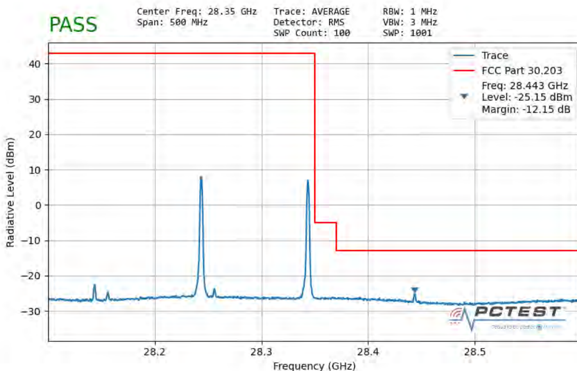
Plot 7-70. Ant 1 Upper Band Edge (100MHz-2CC – \pi/2 BPSK 1 RB)
