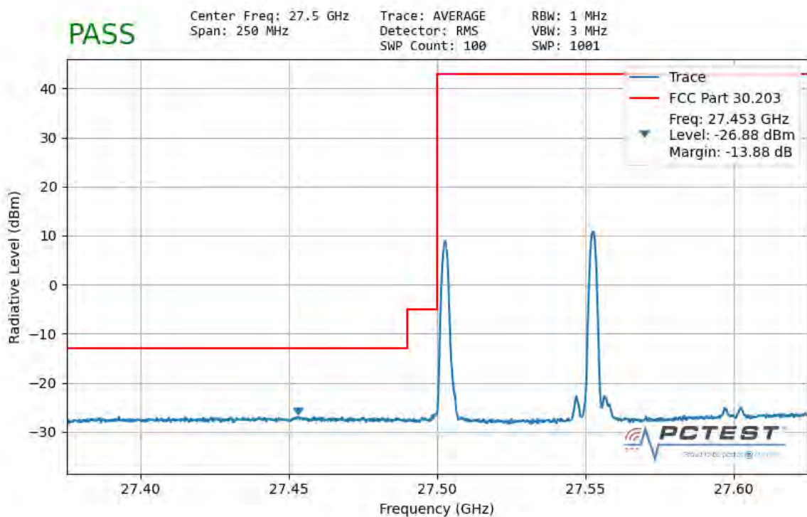
Plot 7-72. Ant 3 Lower Band Edge (50MHz-2CC – \pi/2 BPSK 1 RB)
