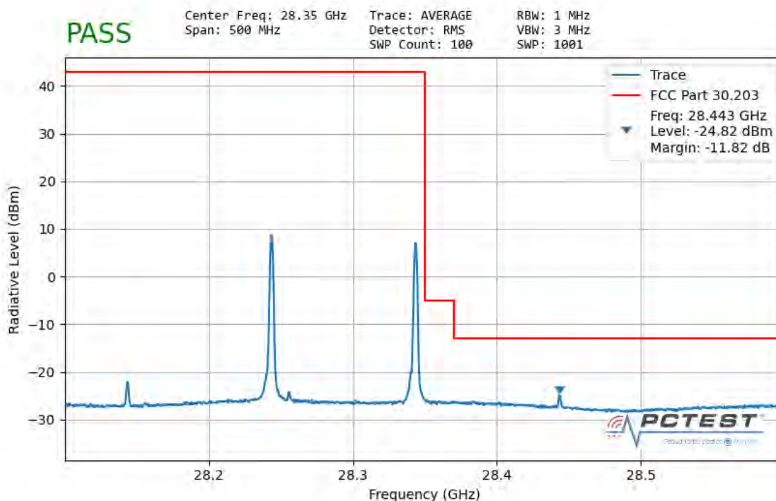
Plot 7-78. Ant 2 Upper Band Edge (100MHz-2CC – \pi/2 BPSK 1 RB)
