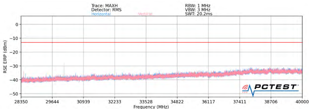
Plot 7-36. Ant 3 - n261 Radiated Spurious Plot (1CC \pi/2 BPSK Mid Channel MIMO)
