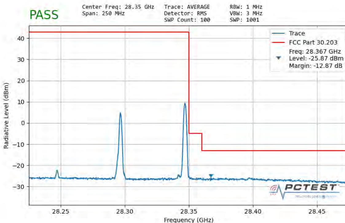
Plot 7-74. Ant 3 Upper Band Edge (50MHz-2CC – \pi/2 BPSK 1 RB)
