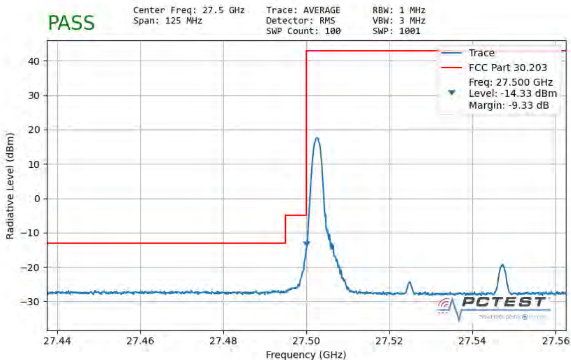
Plot 7-71. Ant 3 Lower Band Edge (50MHz-1CC – \pi/2 BPSK 1 RB)
