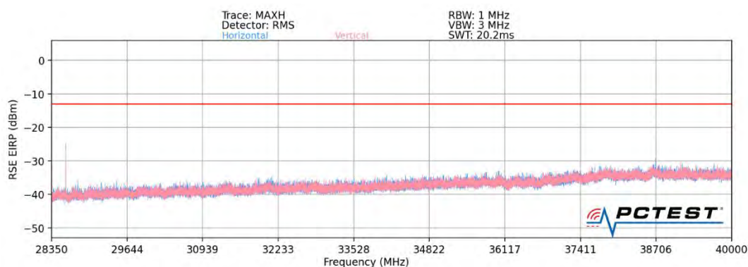
Plot 7-36. Ant 1-n261 Radiated Spurious Plot (1CC \pi/2 BPSK Mid Channel MIMO)
