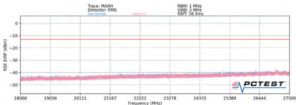
Plot 7-35. Ant 2 - n261 Radiated Spurious Plot (1CC \pi/2 BPSK Mid Channel MIMO)
