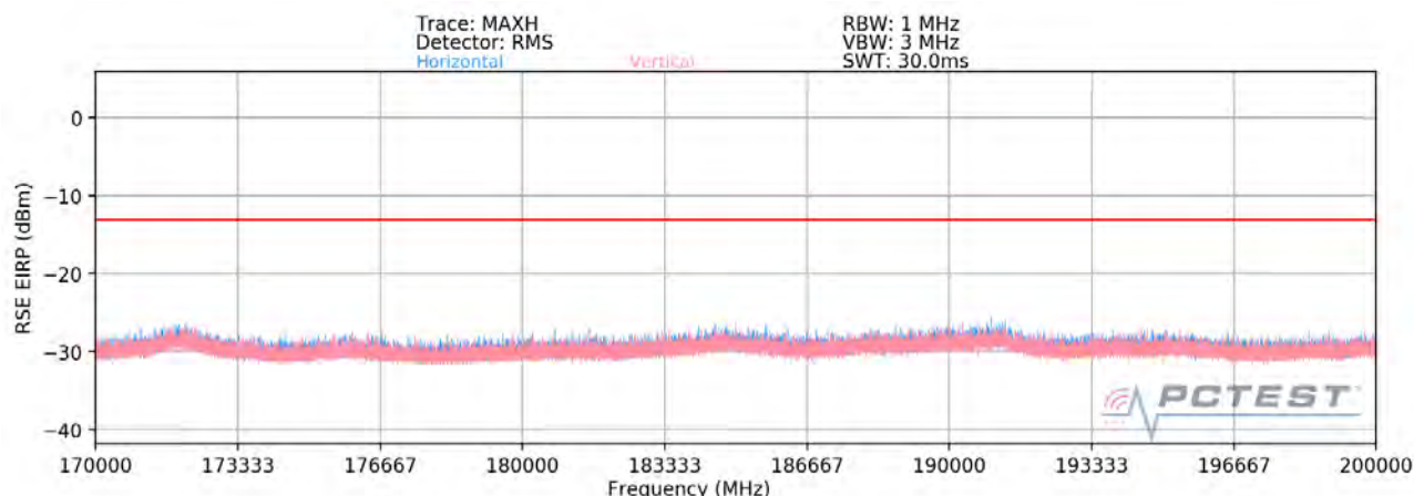
Plot 7-54. Ant 3 - n260 Radiated Spurious Plot (1CC \pi/2 BPSK Mid Channel MIMO)
