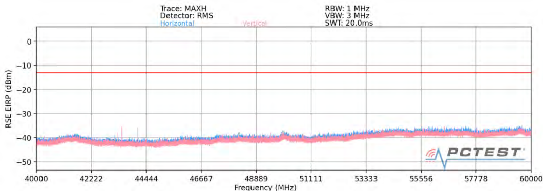
Plot 7-50. Ant 2 - n260 Radiated Spurious Plot (1CC \pi/2 BPSK Mid Channel MIMO)
