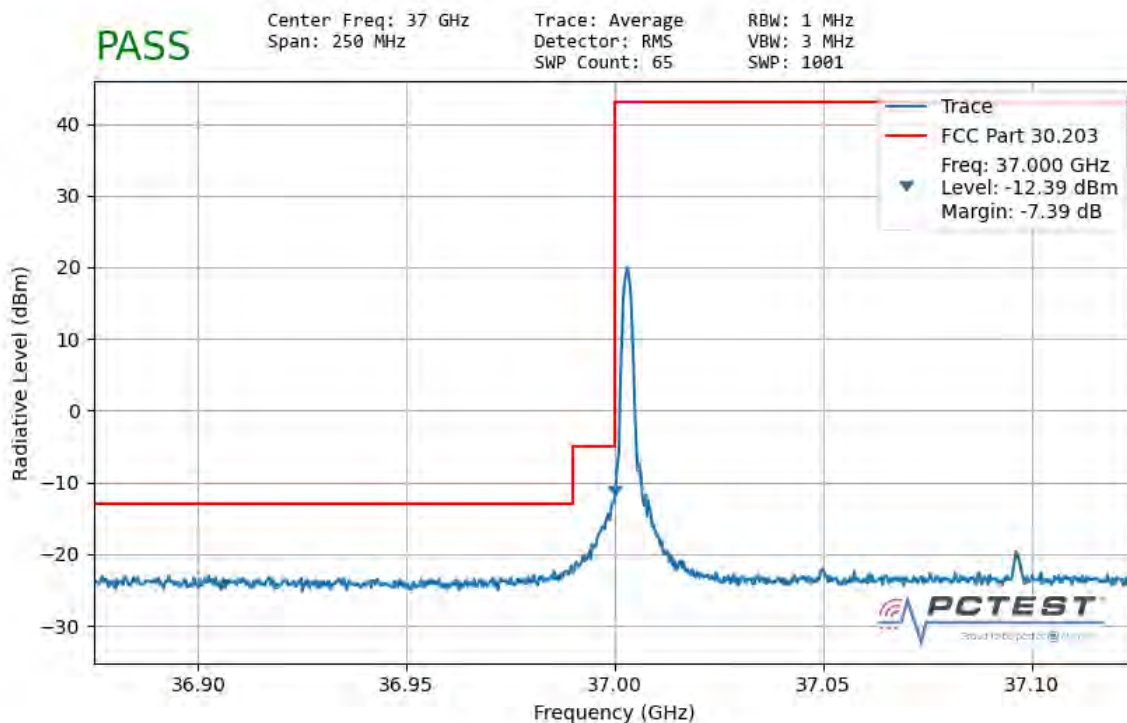
Plot 7-91. Ant 2 Lower Band Edge (100MHz-1CC – \pi/2 BPSK 1 RB)
