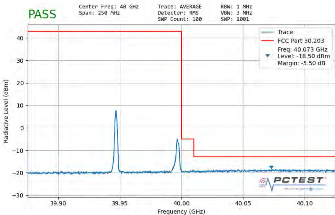
Plot 7-82. Ant 1 Upper Band Edge (50MHz-2CC – \pi/2 BPSK 1 RB)
