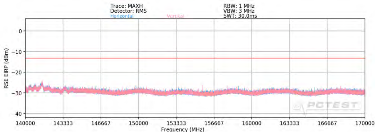
Plot 7-53. Ant 1-n260 Radiated Spurious Plot (1CC \pi/2 BPSK Mid Channel MIMO)
