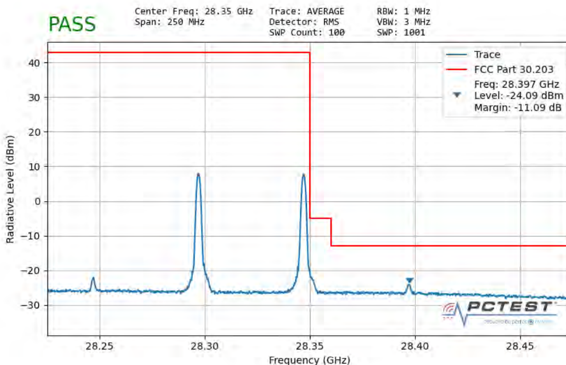
Plot 7-66. Ant 1 Upper Band Edge (50MHz-2CC – \pi/2 BPSK 1 RB)
