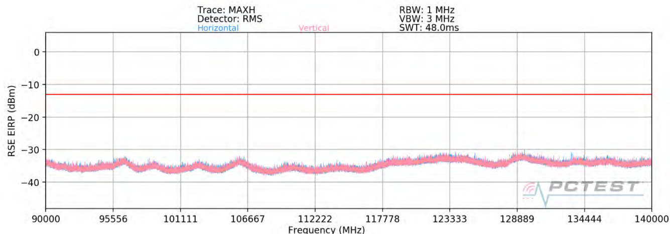
Plot 7-60. Ant 2-n260 Radiated Spurious Plot (1CC \pi/2 BPSK Mid Channel MIMO)
