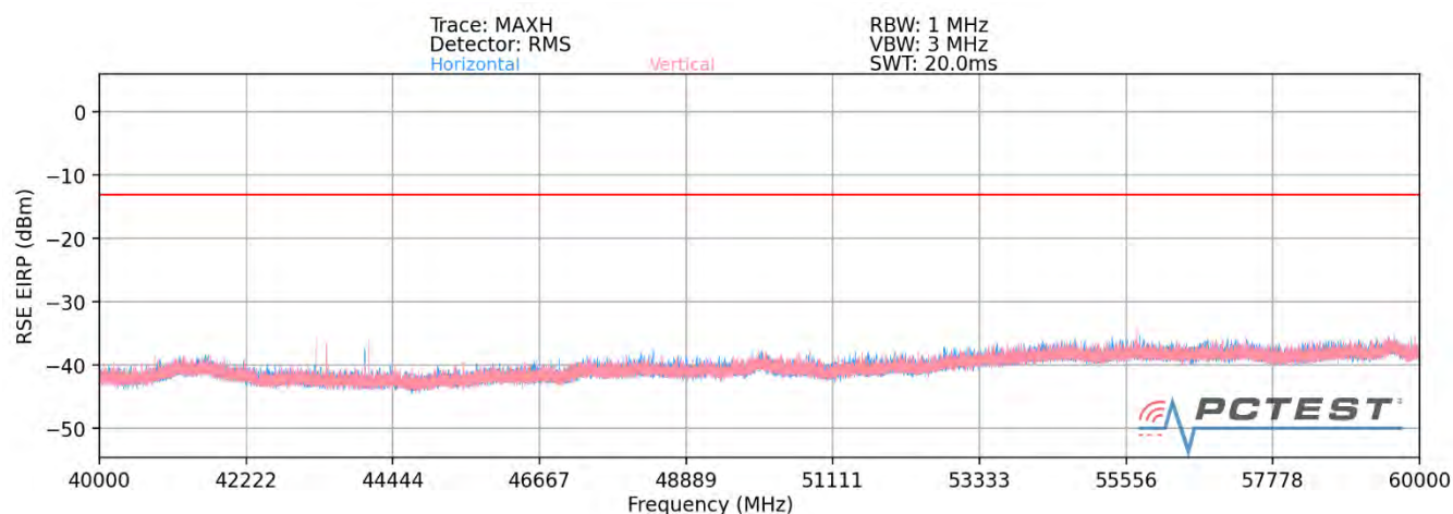
Plot 7-50. Ant 3 - n260 Radiated Spurious Plot (1CC \pi/2 BPSK Mid Channel MIMO)
