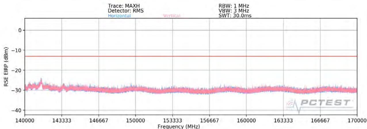
Plot 7-53. Ant 2 - n260 Radiated Spurious Plot (1CC \pi/2 BPSK Mid Channel MIMO)
