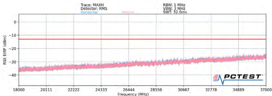
Plot 7-49. Ant 1-n260 Radiated Spurious Plot (1CC \pi/2 BPSK Mid Channel MIMO)
