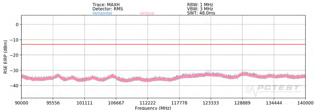
Plot 7-60. Ant 1-n260 Radiated Spurious Plot (1CC \pi/2 BPSK Mid Channel MIMO)
