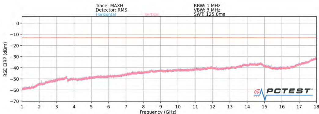
Plot 7-48. Ant 2 - n260 Radiated Spurious Plot (1CC \pi/2 BPSK Mid Channel MIMO)
