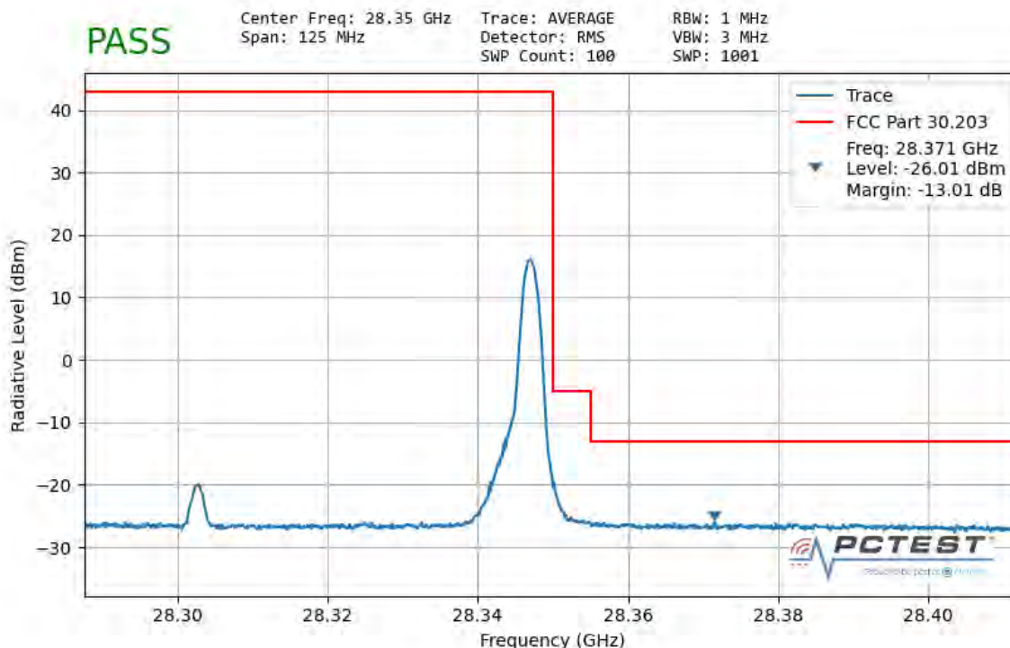
Plot 7-65. Ant 1 Upper Band Edge (50MHz-1CC – \pi/2 BPSK 1 RB)
