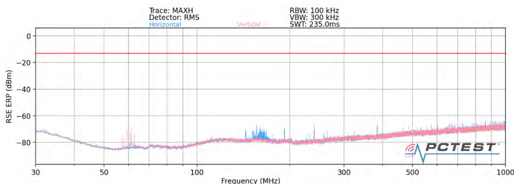
Plot 7-47. Ant 3 - n260 Radiated Spurious Plot (1CC \pi/2 BPSK Mid Channel MIMO)
