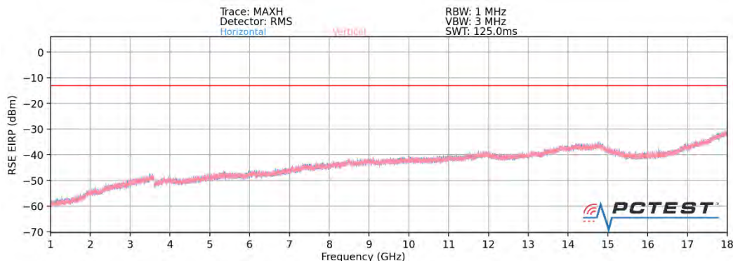
Plot 7-48. Ant 1-n260 Radiated Spurious Plot (1CC \pi/2 BPSK Mid Channel MIMO)
