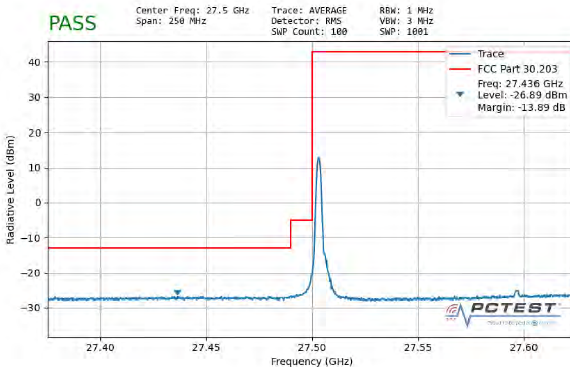
Plot 7-75. Ant 2 Lower Band Edge (100MHz-1CC – \pi/2 BPSK 1 RB)
