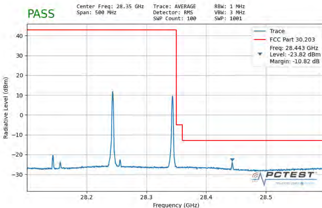
Plot 7-78. Ant 3 Upper Band Edge (100MHz-2CC – \pi/2 BPSK 1 RB)
