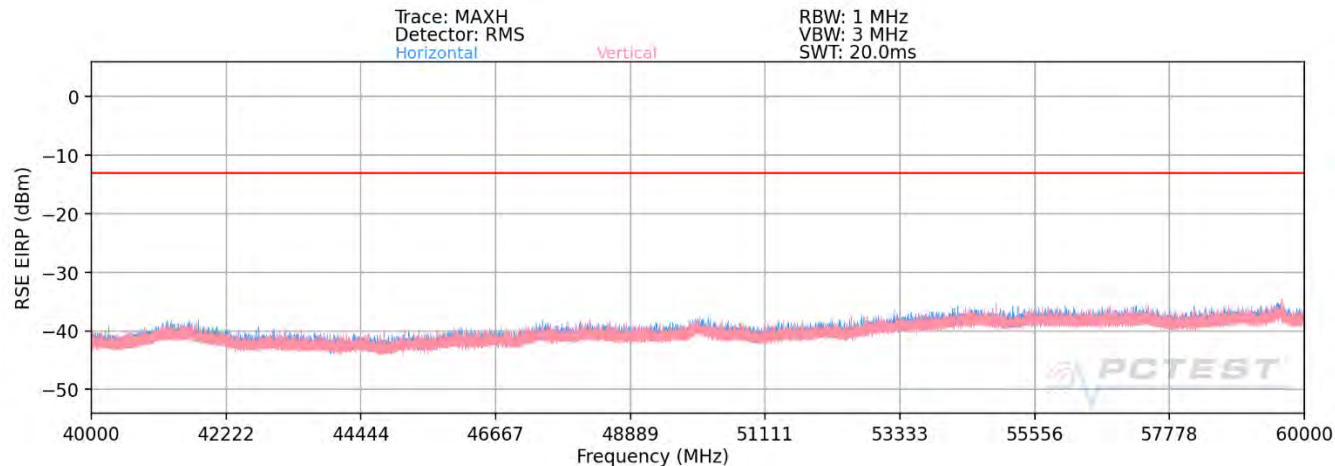
Plot 7-44. Ant 1-n261 Radiated Spurious Plot (1CC \pi/2 BPSK Mid Channel MIMO)
