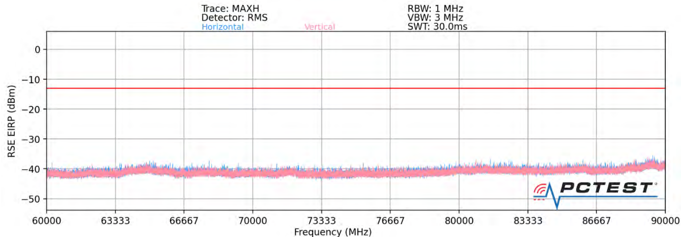
Plot 7-51. Ant 3-n260 Radiated Spurious Plot (1CC \pi/2 BPSK Mid Channel MIMO)
