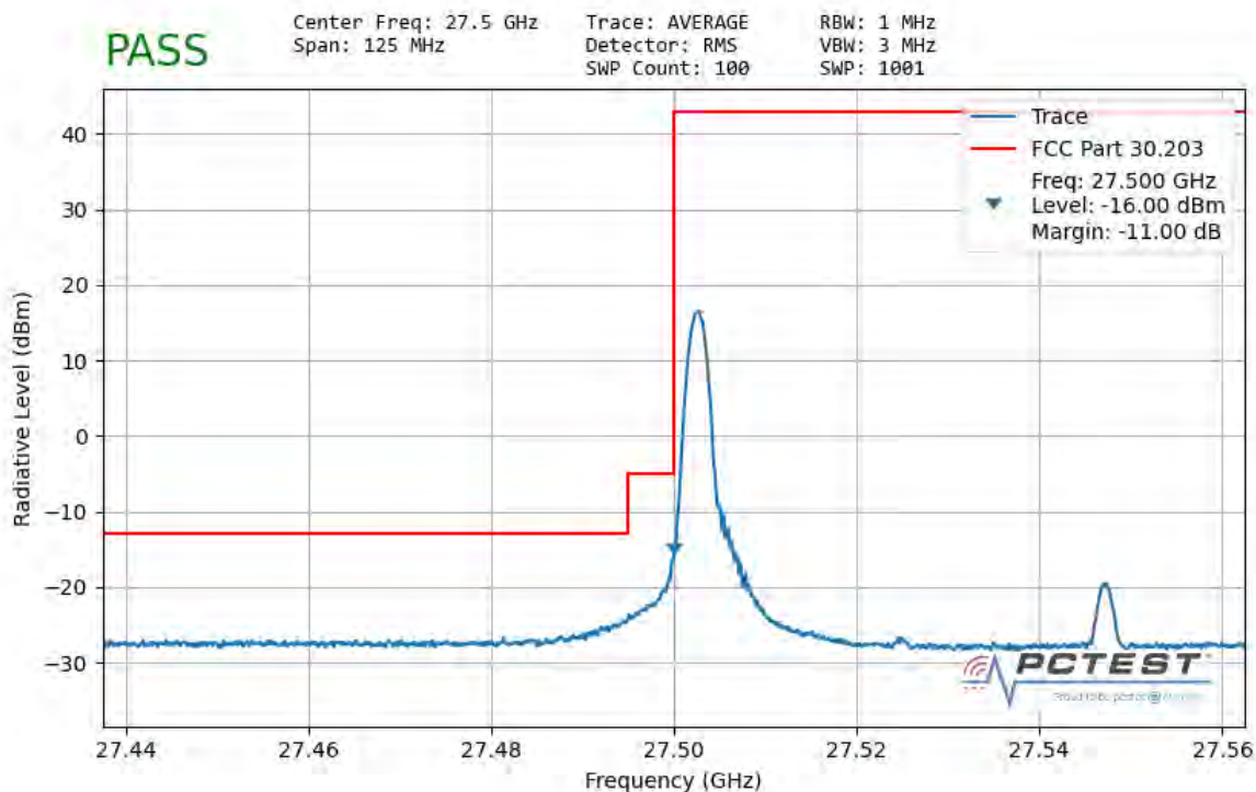
Plot 7-71. Ant 2 Lower Band Edge (50MHz-1CC – \pi/2 BPSK 1 RB)
