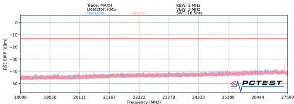
Plot 7-35. Ant 3 - n261 Radiated Spurious Plot (1CC \pi/2 BPSK Mid Channel MIMO)
