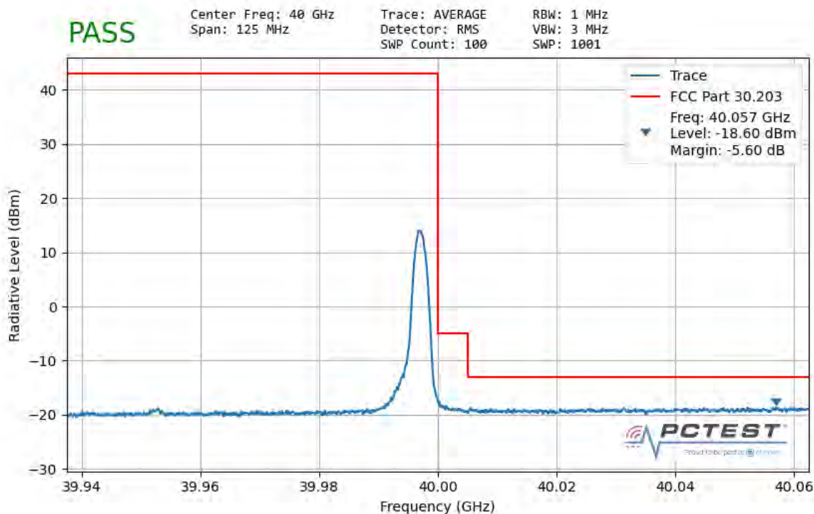
Plot 7-81. Ant 1 Upper Band Edge (50MHz-1CC – \pi/2 BPSK 1 RB)
