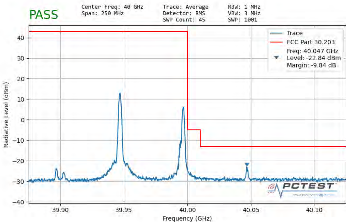
Plot 7-90. Ant 2 Upper Band Edge (50MHz-2CC – \pi/2 BPSK 1 RB)
