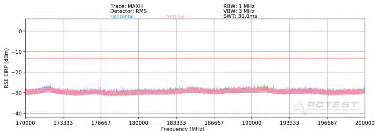
Plot 7-54. Ant 1-n260 Radiated Spurious Plot (1CC \pi/2 BPSK Mid Channel MIMO)
