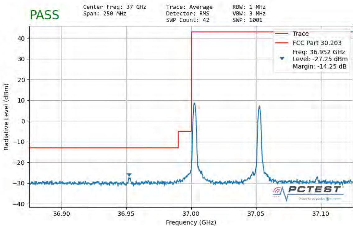
Plot 7-88. Ant 2 Lower Band Edge (50MHz-2CC – \pi/2 BPSK 1 RB)
