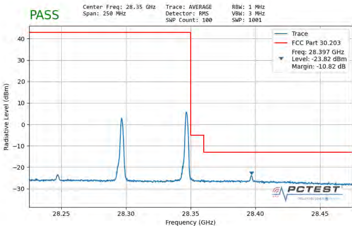
Plot 7-74. Ant 2 Upper Band Edge (50MHz-2CC – \pi/2 BPSK 1 RB)
