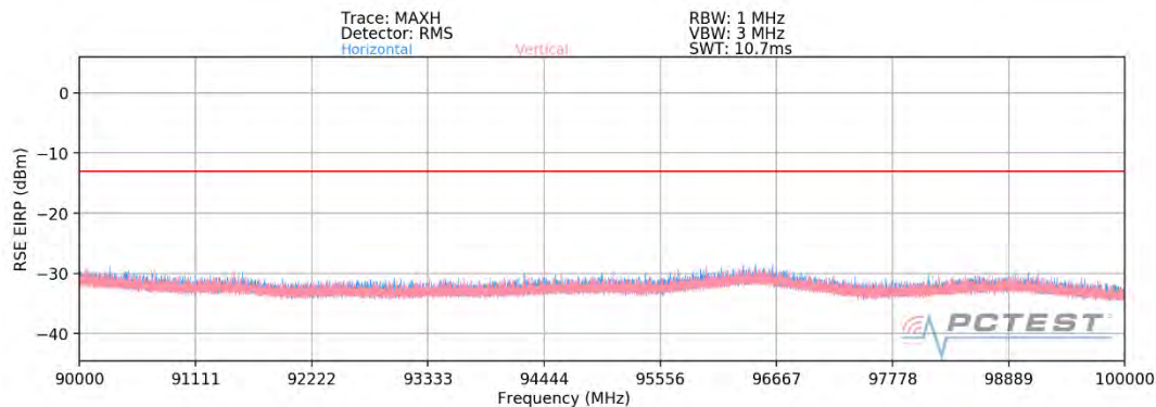
Plot 7-39. Ant 3 - n261 Radiated Spurious Plot (1CC \pi/2 BPSK Mid Channel MIMO)
