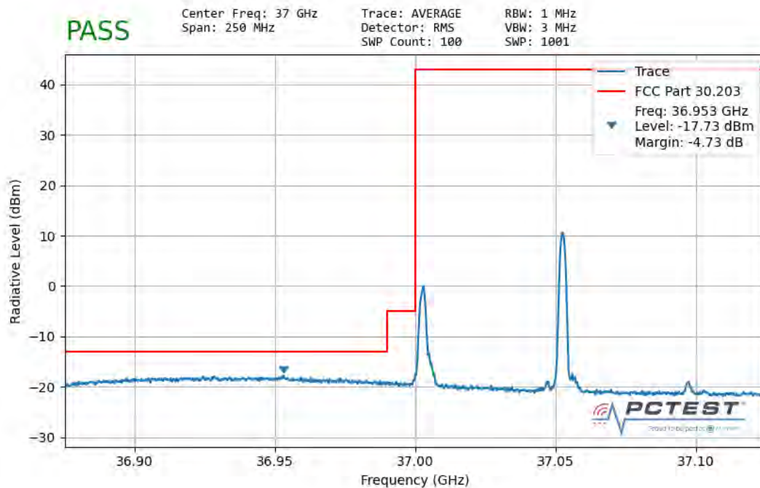
Plot 7-80. Ant 1 Lower Band Edge (50MHz-2CC – \pi/2 BPSK 1 RB)
