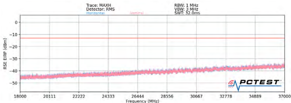
Plot 7-49. Ant 2 - n260 Radiated Spurious Plot (1CC \pi/2 BPSK Mid Channel MIMO)
