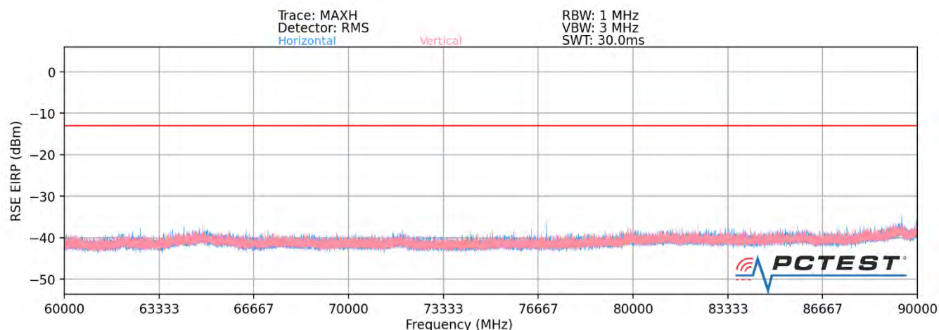
Plot 7-5. Ant 2-n260 Radiated Spurious Plot (1CC \pi/2 BPSK Mid Channel MIMO)
