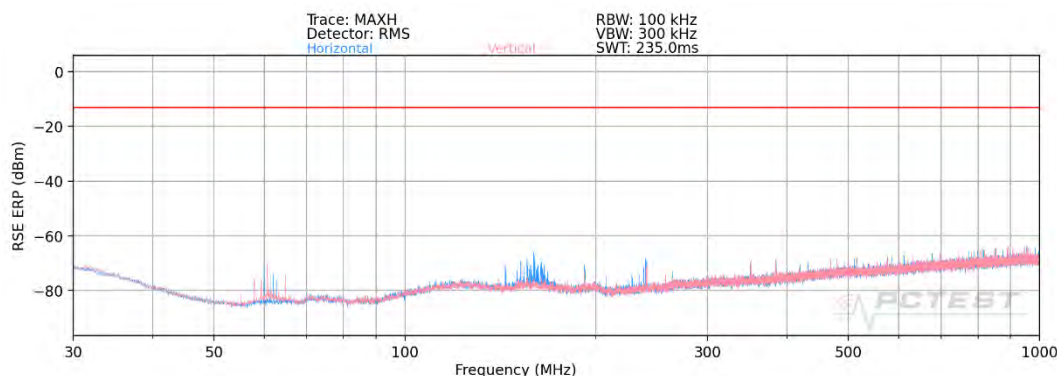
Plot 7-3. Ant 3 - n261 Radiated Spurious Plot (1CC \pi/2 BPSK Mid Channel MIMO)
