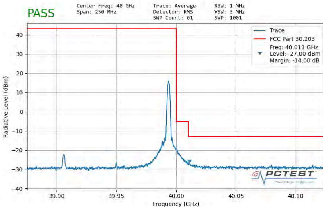
Plot 7-93. Ant 2 Upper Band Edge (100MHz-1CC – \pi/2 BPSK 1 RB)
