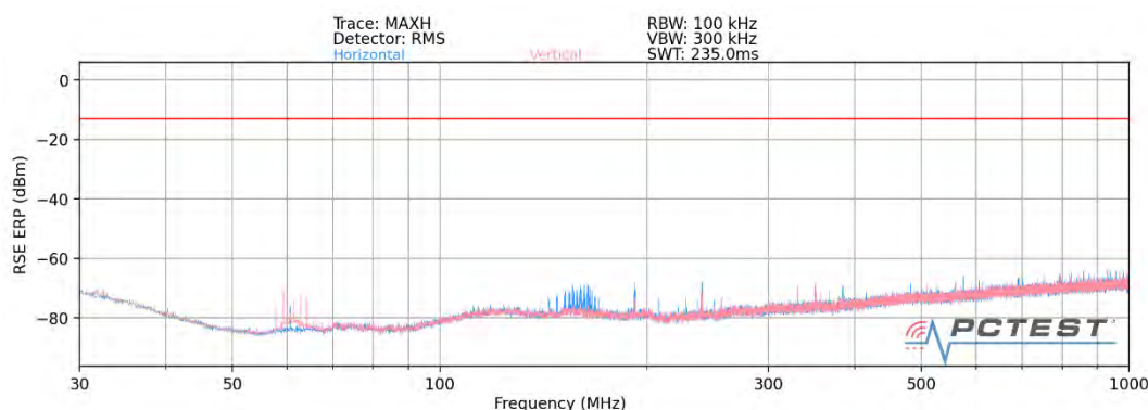
Plot 7-47. Ant 2 - n260 Radiated Spurious Plot (1CC \pi/2 BPSK Mid Channel MIMO)
