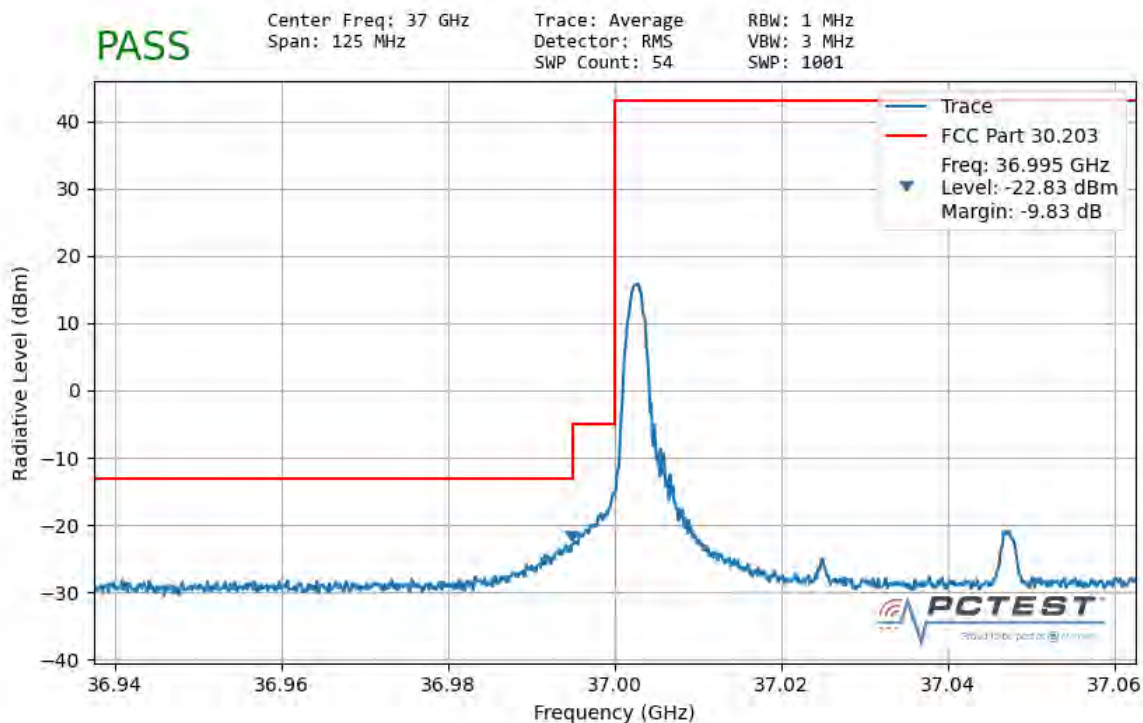
Plot 7-87. Ant 2 Lower Band Edge (50MHz-1CC – \pi/2 BPSK 1 RB)
