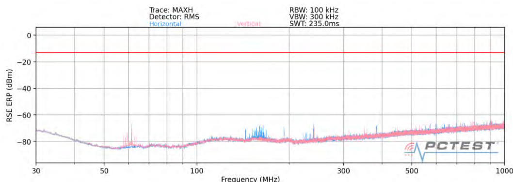
Plot 7-1. Ant 1- n261 Radiated Spurious Plot (1CC \pi/2 BPSK Mid Channel MIMO)
