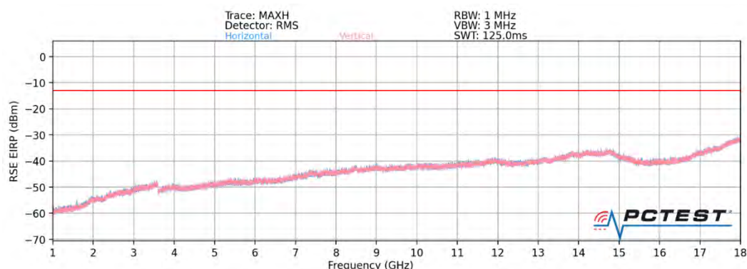
Plot 7-34. Ant 1-n261 Radiated Spurious Plot (1CC \pi/2 BPSK Mid Channel MIMO)
