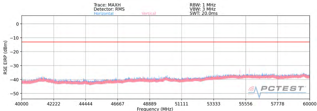
Plot 7-37. Ant 3-n261 Radiated Spurious Plot (1CC \pi/2 BPSK Mid Channel MIMO)
