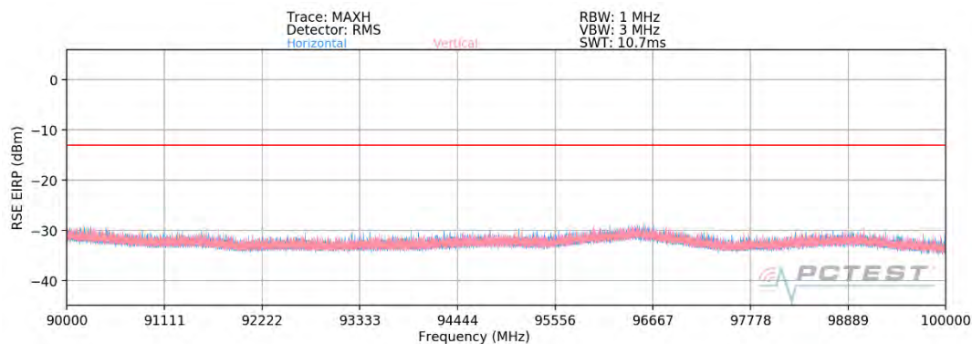
Plot 7-39. Ant 2 - n261 Radiated Spurious Plot (1CC \pi/2 BPSK Mid Channel MIMO)
