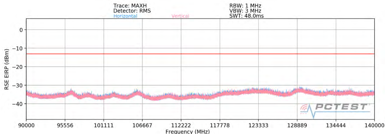
Plot 7-52. Ant 3-n260 Radiated Spurious Plot (1CC \pi/2 BPSK Mid Channel MIMO)
