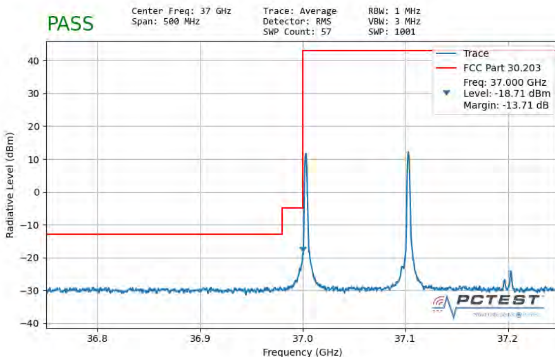
Plot 7-92. Ant 2 Lower Band Edge (100MHz-2CC – \pi/2 BPSK 1 RB)
