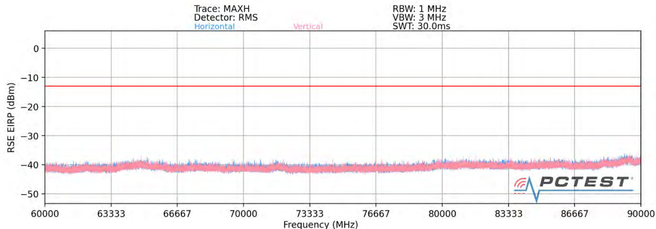
Plot 7-38. Ant 1-n261 Radiated Spurious Plot (1CC \pi/2 BPSK Mid Channel MIMO)
