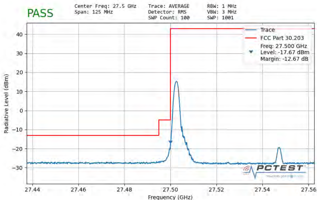
Plot 7-63. Ant 1 Lower Band Edge (50MHz-1CC – \pi/2 BPSK 1 RB)
