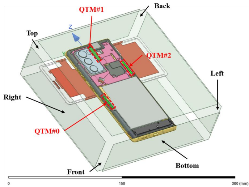
Figure 3-2. PD evaluation Surfaces with swivel up
