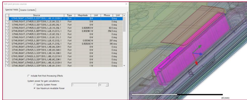
Figure 5. An example of port excitation (QTM#0)
