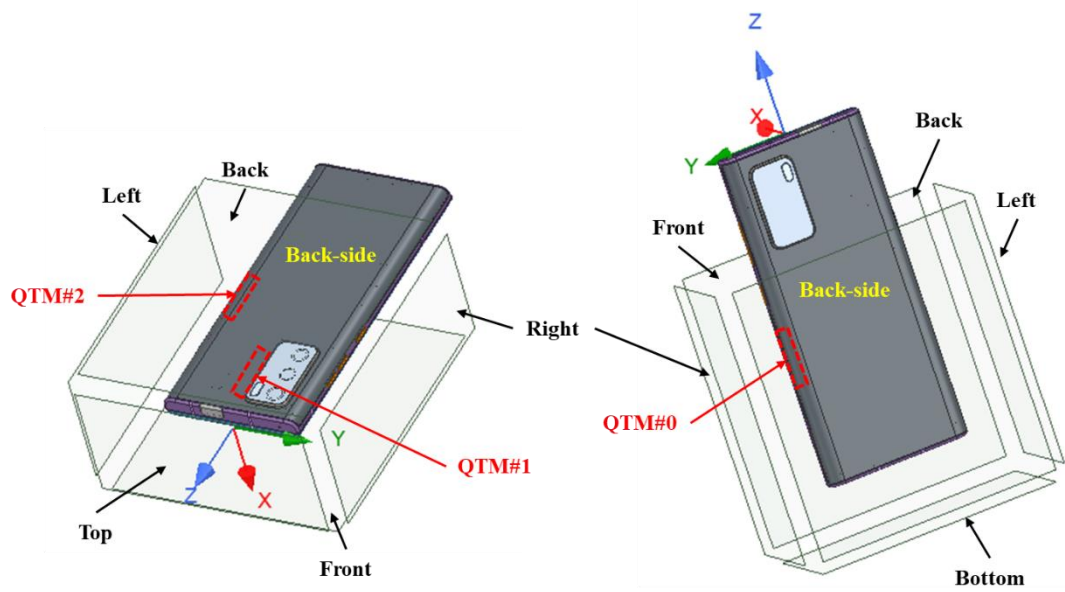
Figure 3-1. PD evaluation Surfaces
