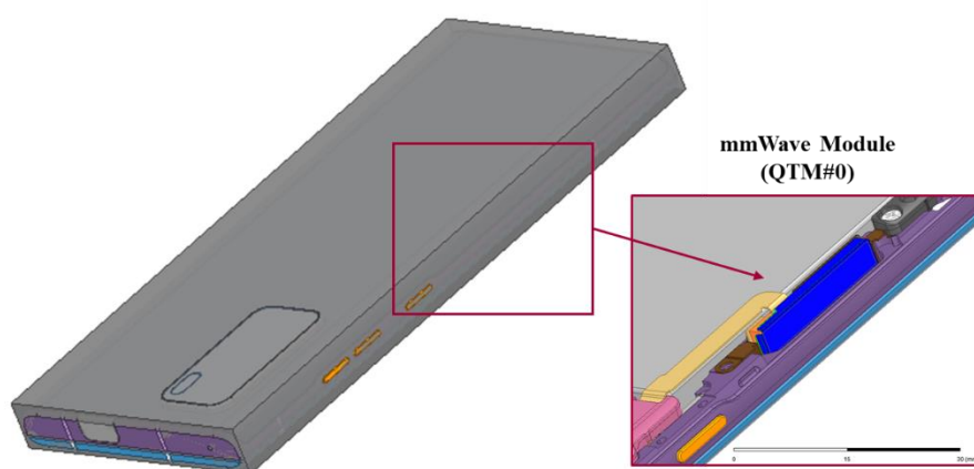
Figure 4. mmWave module (QTM#0)
