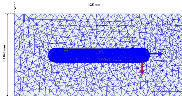
Figure 1-1. Example of HFSS mesh in a model of the device (Top view)
