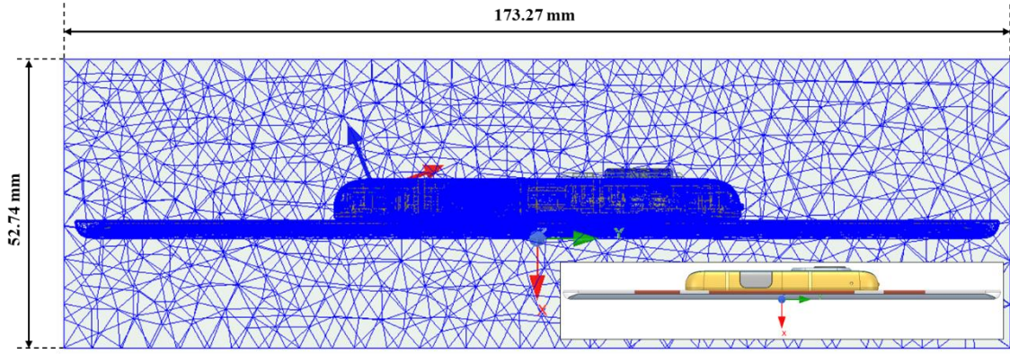
Figure 1-2. Example of HFSS mesh in a model of the device with swivel up (Top view)
