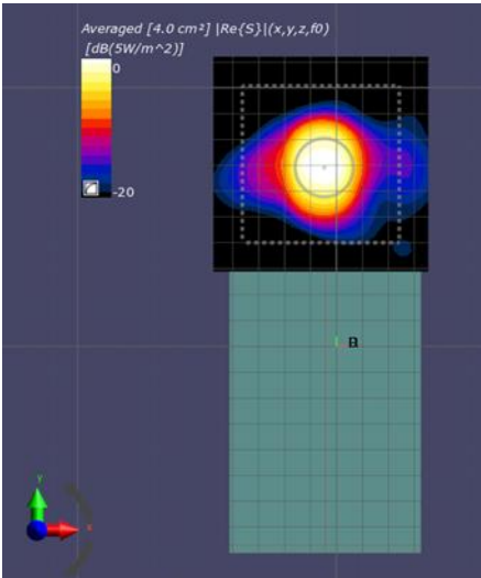
Figure 12-1 4cm 2 psPD distribution measured at input.power.limit of 4.5 dBm on the back surface for n261 beam 20
