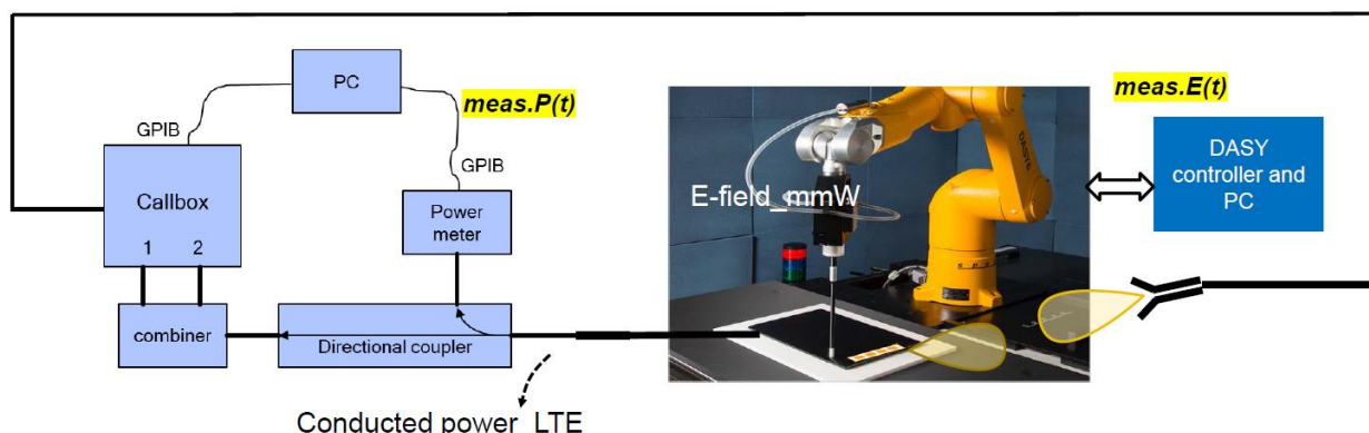
Figure 7-2 Power Density Measurement Setup – Test Setup Photo 4
