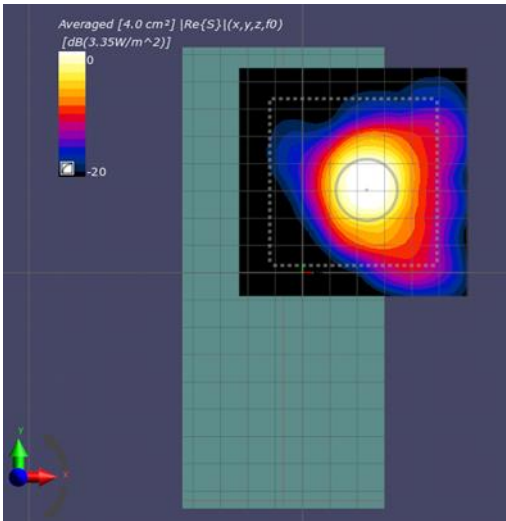
Figure 12-2 4cm 2 psPD distribution measured at input.power.limit of 4.3 dBm on the back surface for n260 beam 44
