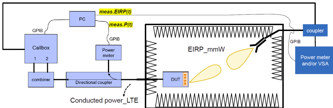
Figure 7-1 mmW NR radiated power measurement setup – Test Setup Photo 5
