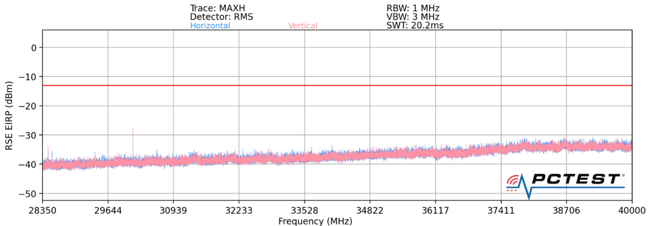
Plot 7-36. Ant 3 - n261 Radiated Spurious Plot (1CC QPSK Mid Channel MIMO)
