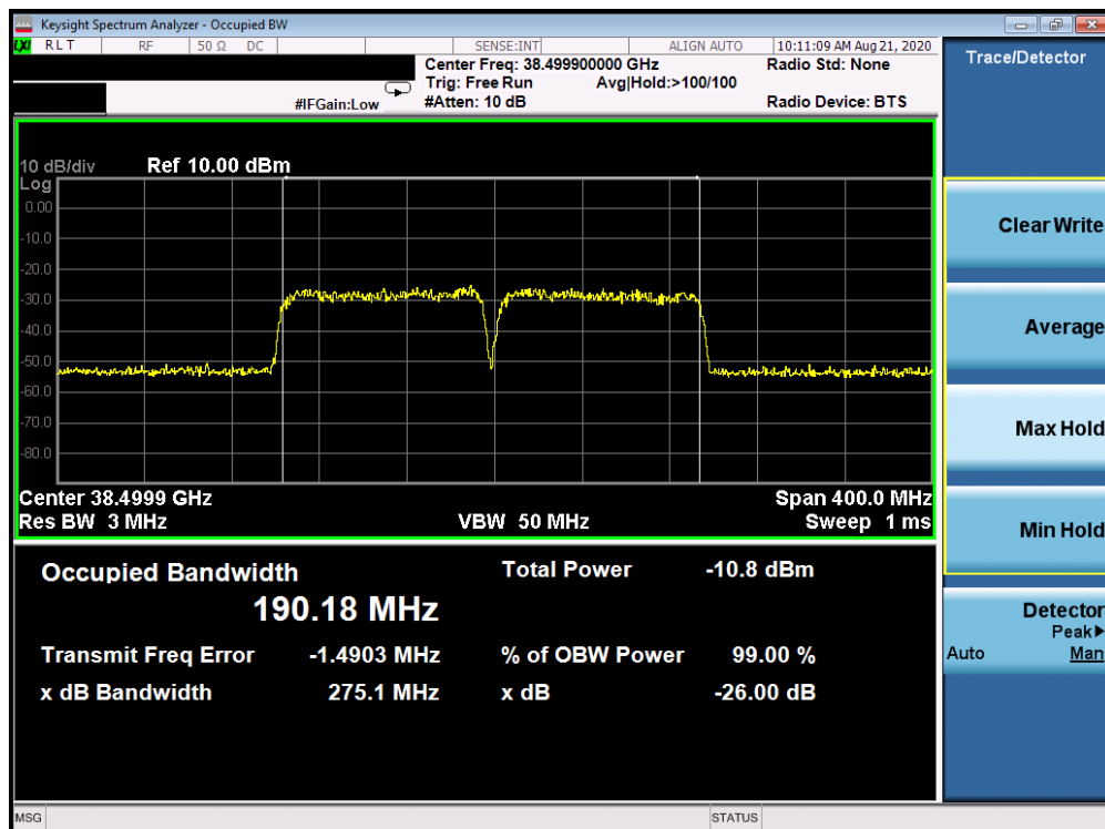
Plot 7-30. Ant 3 Occupied Bandwidth Plot (100MHz-2CC – 16QAM – Mid Channel)
