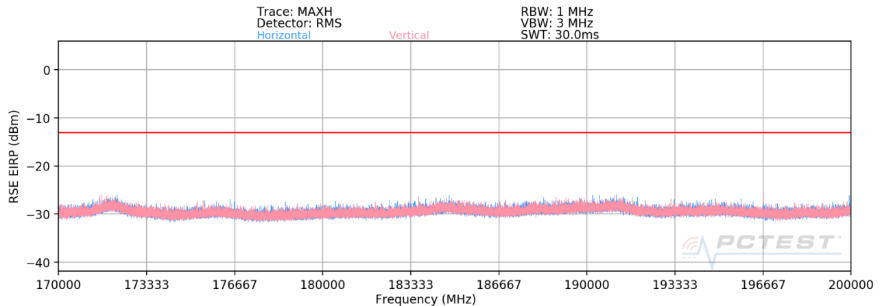
Plot 7-54. Ant 1-n260 Radiated Spurious Plot (1CC QPSK Mid Channel MIMO)
