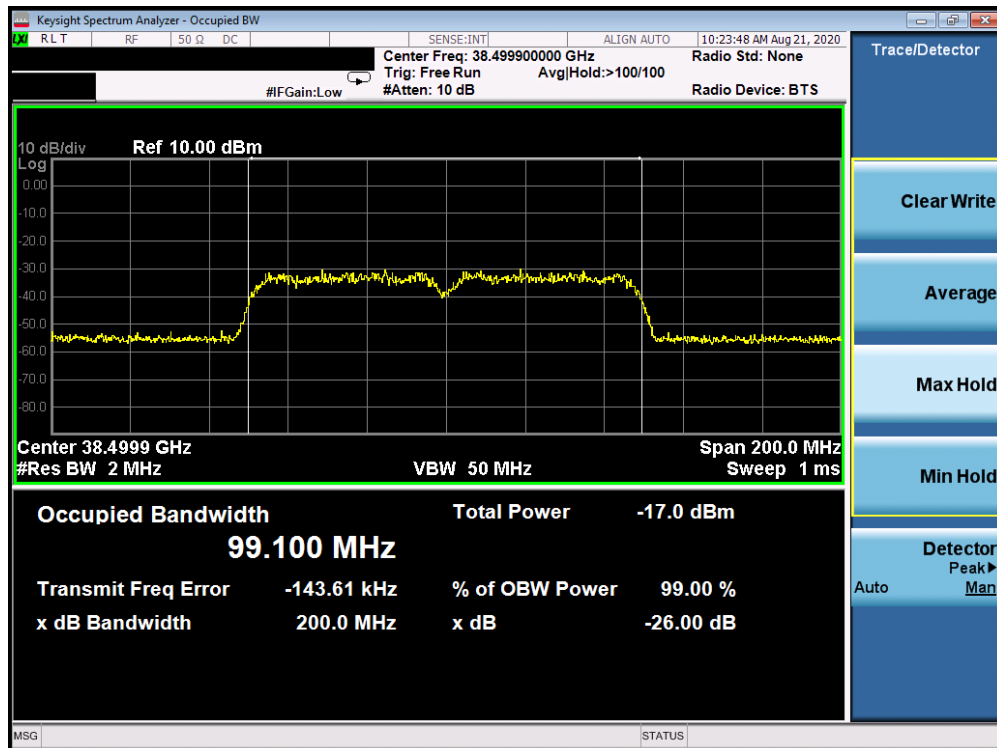
Plot 7-22. Ant 3 Occupied Bandwidth Plot (50MHz-2CC – 16QAM – Mid Channel)
