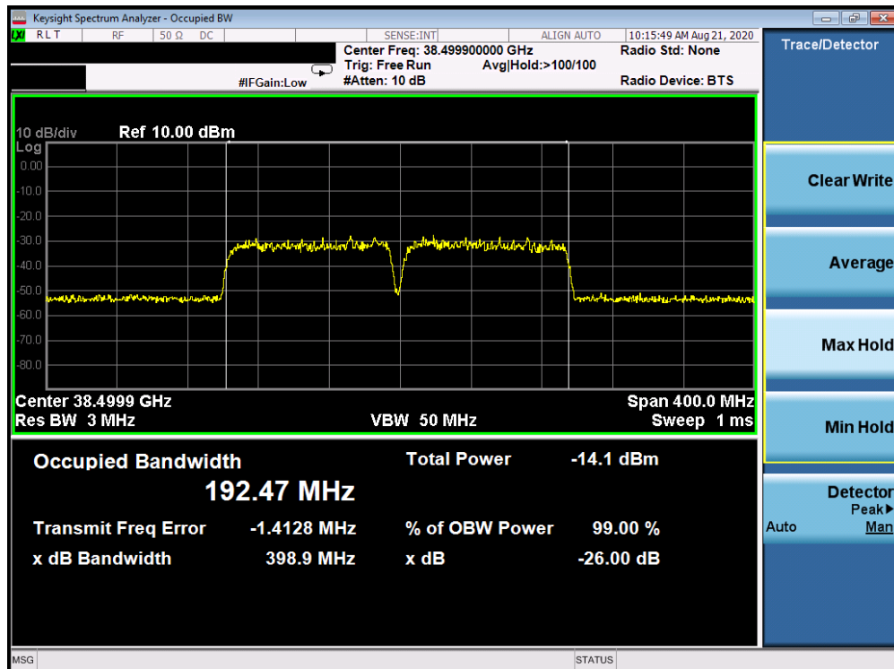
Plot 7-32. Ant 3 Occupied Bandwidth Plot (100MHz-2CC – \pi/2 -BPSK – Mid Channel)
