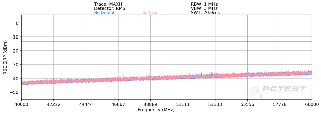
Plot 7-44. Ant 1-n261 Radiated Spurious Plot (1CC QPSK Mid Channel MIMO)
