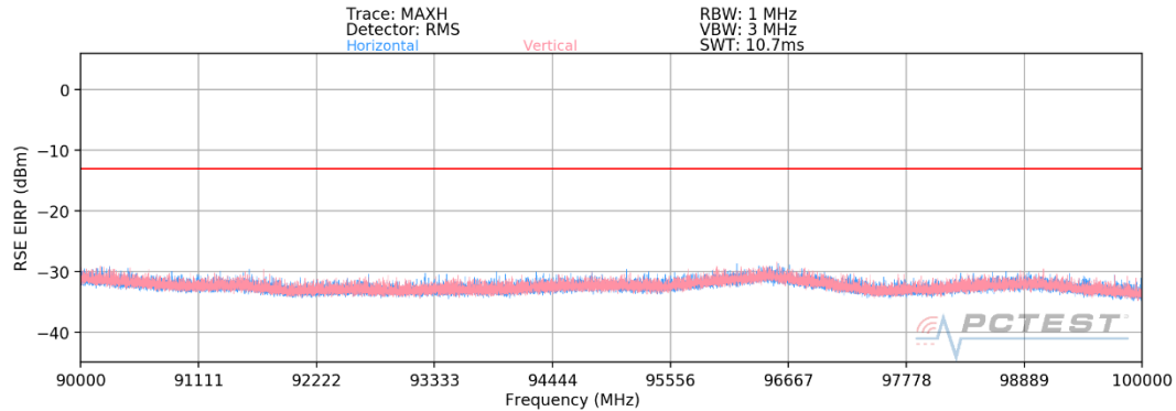
Plot 7-39. Ant 2 - n261 Radiated Spurious Plot (1CC QPSK Mid Channel MIMO)
