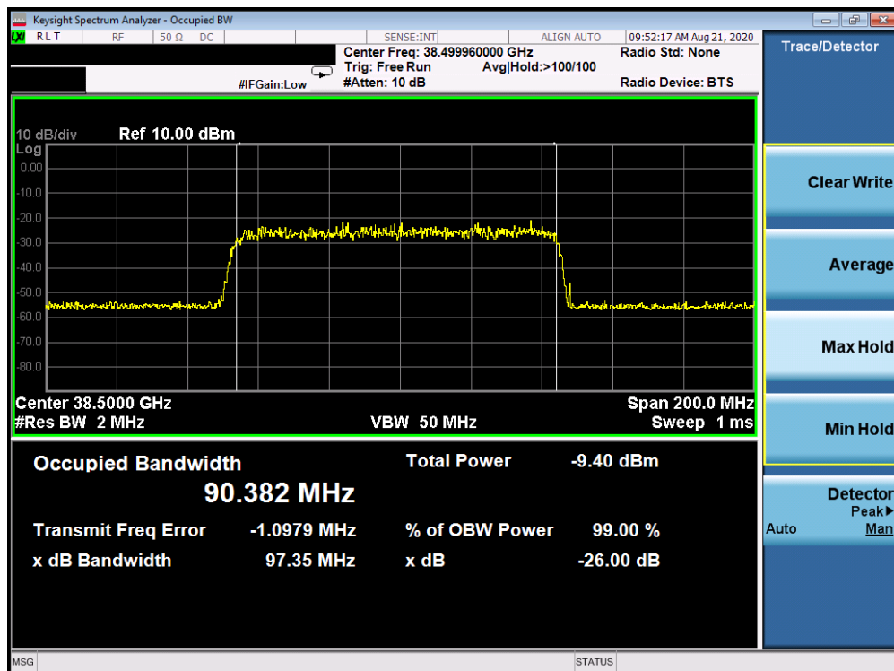
Plot 7-28. Ant 3 Occupied Bandwidth Plot (100MHz-1CC – pi/2-BPSK – Mid Channel)
