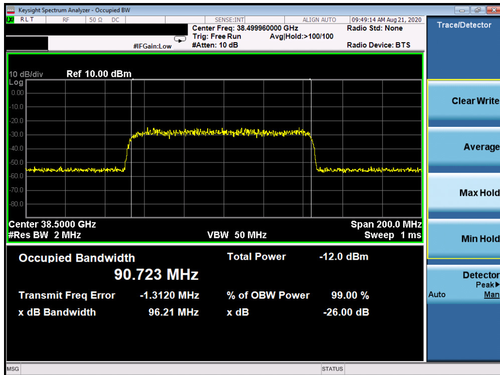
Plot 7-26. Ant 3 Occupied Bandwidth Plot (100MHz-1CC – 16QAM – Mid Channel)
