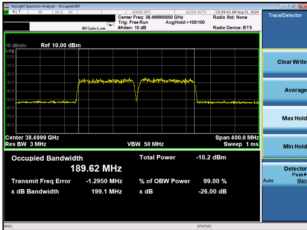
Plot 7-29. Ant 3 Occupied Bandwidth Plot (100MHz-2CC – QPSK – Mid Channel)
