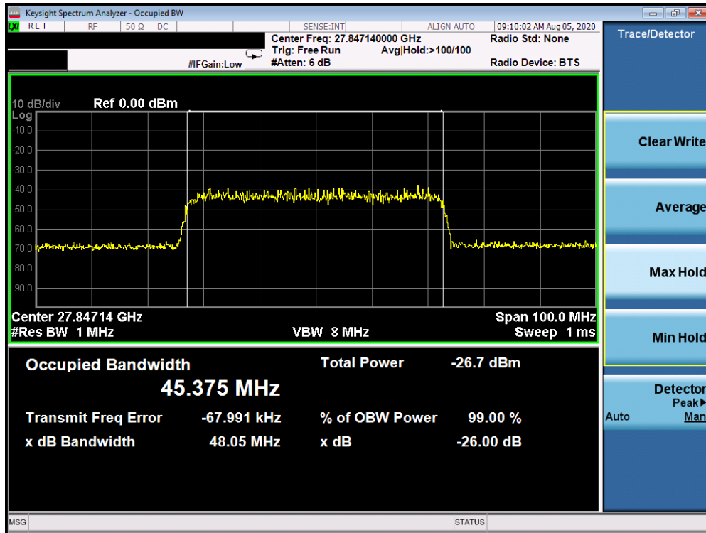
Plot 7-1. Ant 3 Occupied Bandwidth Plot (50MHz-1CC – QPSK – Mid Channel)
