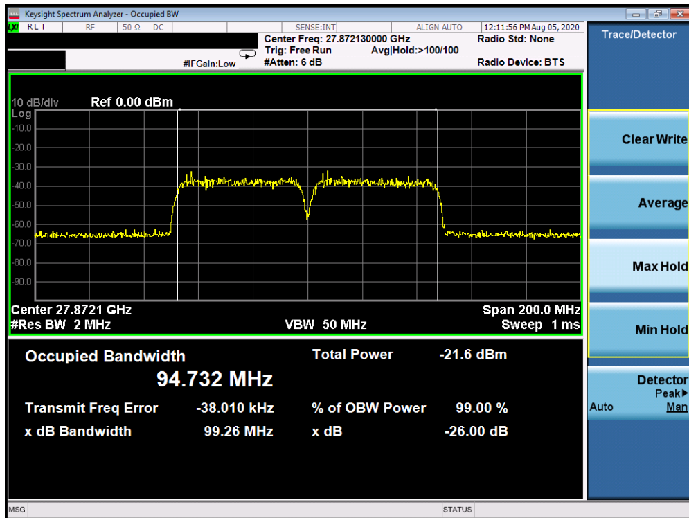
Plot 7-6. Ant 3 Occupied Bandwidth Plot (50MHz-2CC – 16QAM – Mid Channel)
