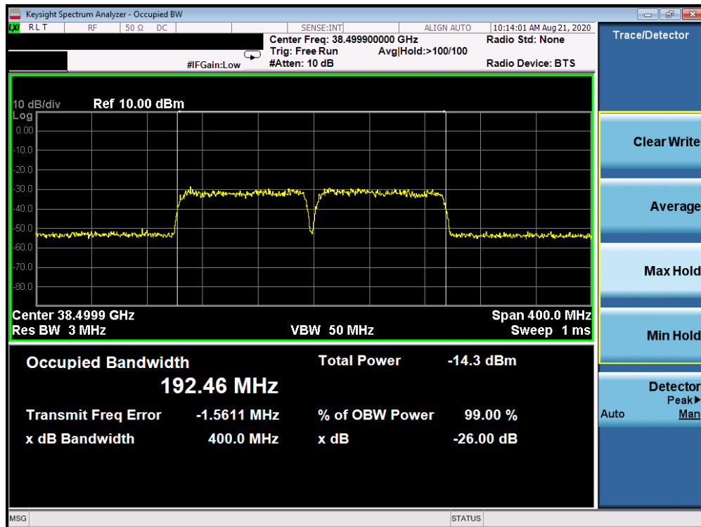
Plot 7-31. Ant 3 Occupied Bandwidth Plot (100MHz-2CC – 64QAM – Mid Channel)
