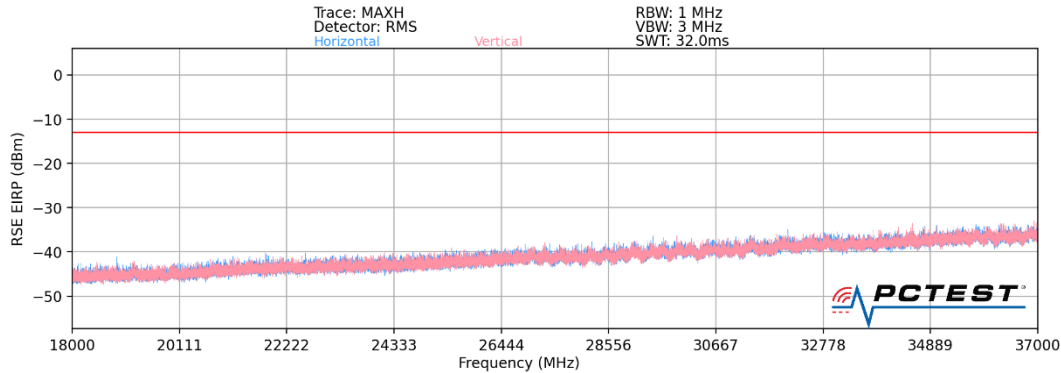
Plot 7-49. Ant 2 - n260 Radiated Spurious Plot (1CC QPSK Mid Channel MIMO)
