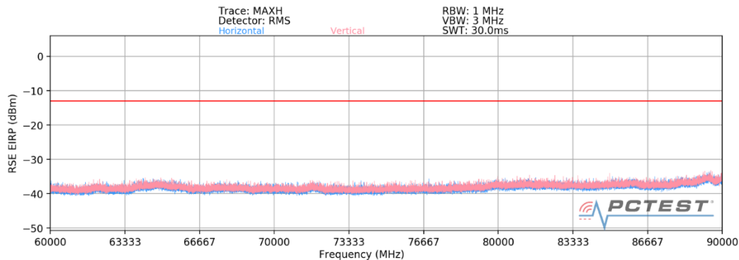
Plot 7-38. Ant 2-n261 Radiated Spurious Plot (1CC QPSK Mid Channel MIMO)
