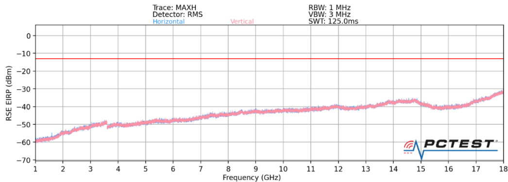
Plot 7-34. Ant 1-n261 Radiated Spurious Plot (1CC QPSK Mid Channel MIMO)
