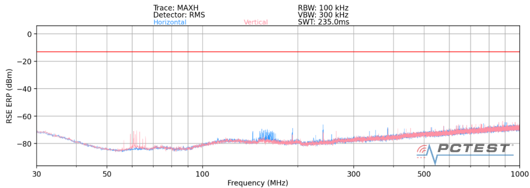
Plot 7-47. Ant 1-n260 Radiated Spurious Plot (1CC QPSK Mid Channel MIMO)
