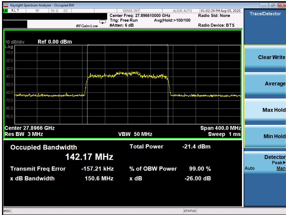
Plot 7-15. Ant 3 Occupied Bandwidth Plot (100MHz-2CC – 64QAM – Mid Channel)
