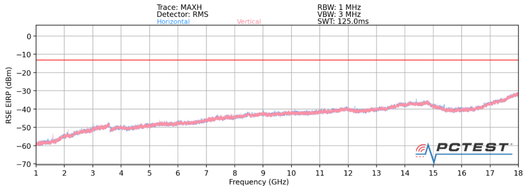
Plot 7-48. Ant 2 - n260 Radiated Spurious Plot (1CC QPSK Mid Channel MIMO)
