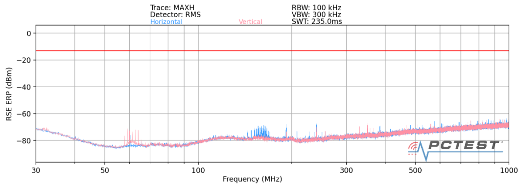
Plot 7-47. Ant 2 - n260 Radiated Spurious Plot (1CC QPSK Mid Channel MIMO)
