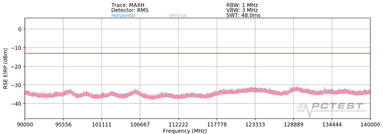
Plot 7-60. Ant 2-n260 Radiated Spurious Plot (1CC QPSK Mid Channel MIMO)
