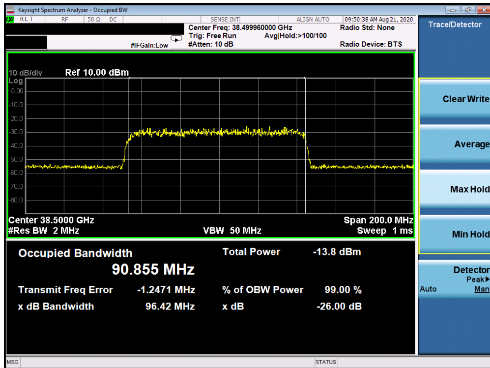
Plot 7-27. Ant 3 Occupied Bandwidth Plot (100MHz-1CC – 64QAM – Mid Channel)
