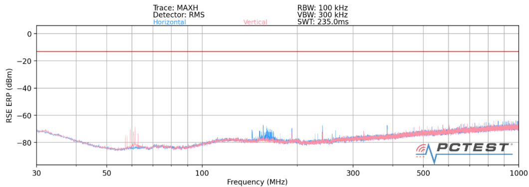
Plot 7-47. Ant 3 - n260 Radiated Spurious Plot (1CC QPSK Mid Channel MIMO)
