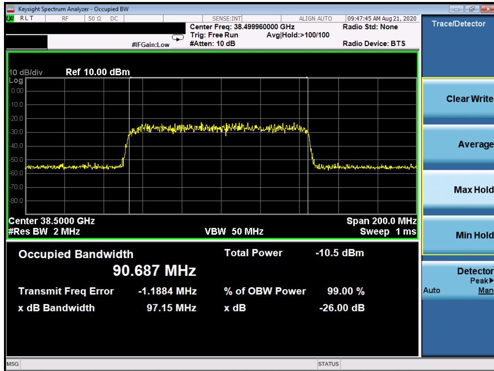
Plot 7-25. Ant 3 Occupied Bandwidth Plot (100MHz-1CC – QPSK – Mid Channel)
