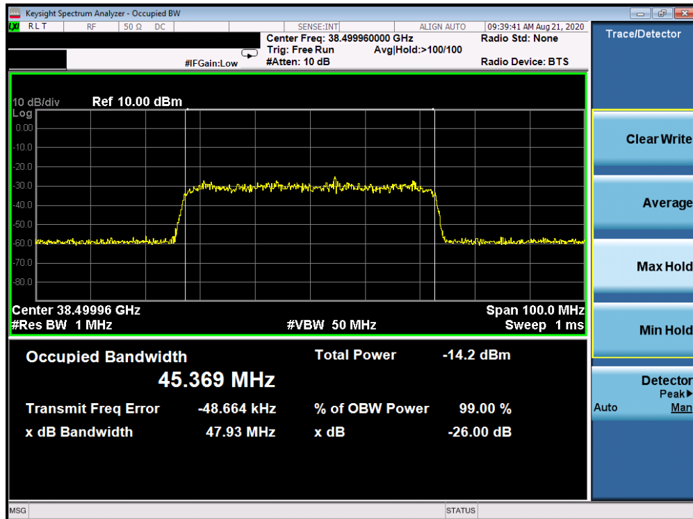
Plot 7-19. Ant 3 Occupied Bandwidth Plot (50MHz-1CC – 64QAM – Mid Channel)
