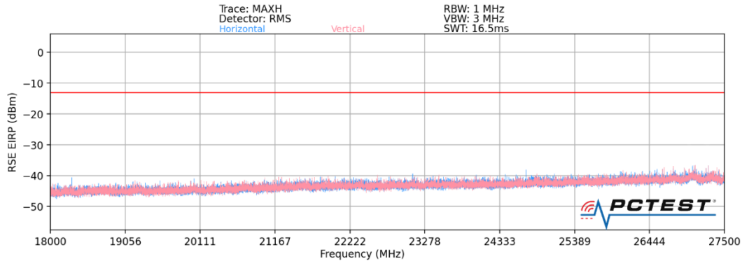
Plot 7-35. Ant 1-n261 Radiated Spurious Plot (1CC QPSK Mid Channel MIMO)
