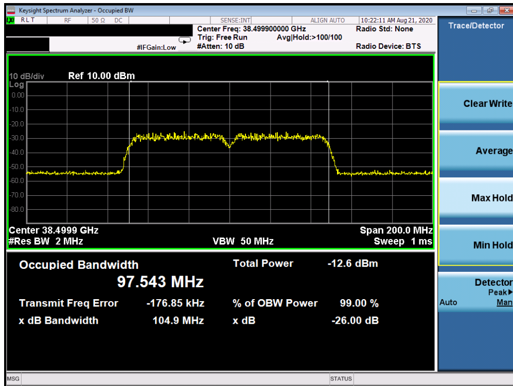
Plot 7-21. Ant 3 Occupied Bandwidth Plot (50MHz-2CC – QPSK – Mid Channel)
