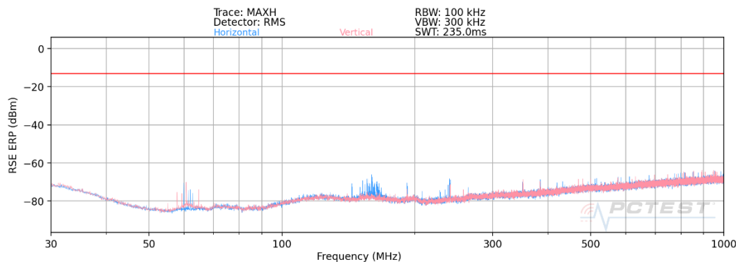
Plot 7-35. Ant 3 - n261 Radiated Spurious Plot (1CC QPSK Mid Channel MIMO)
