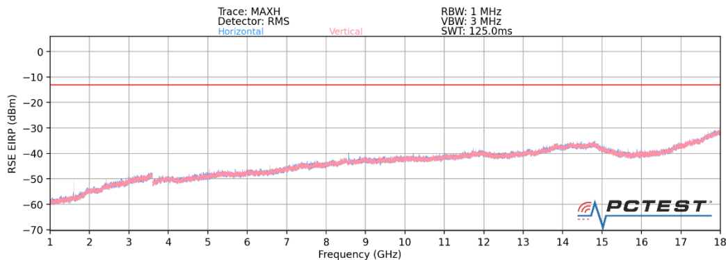
Plot 7-34. Ant 3 - n261 Radiated Spurious Plot (1CC QPSK Mid Channel MIMO)
