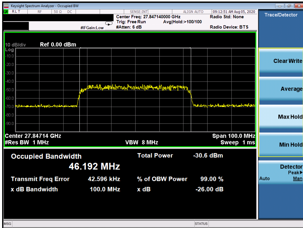
Plot 7-3. Ant 3 Occupied Bandwidth Plot (50MHz-1CC – 64QAM – Mid Channel)
