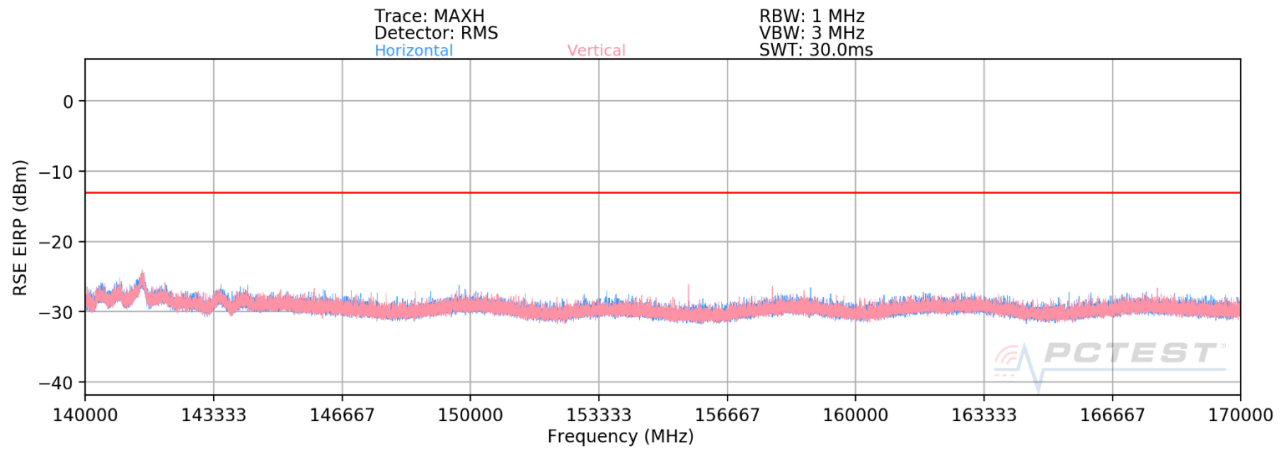
Plot 7-53. Ant 1-n260 Radiated Spurious Plot (1CC QPSK Mid Channel MIMO)
