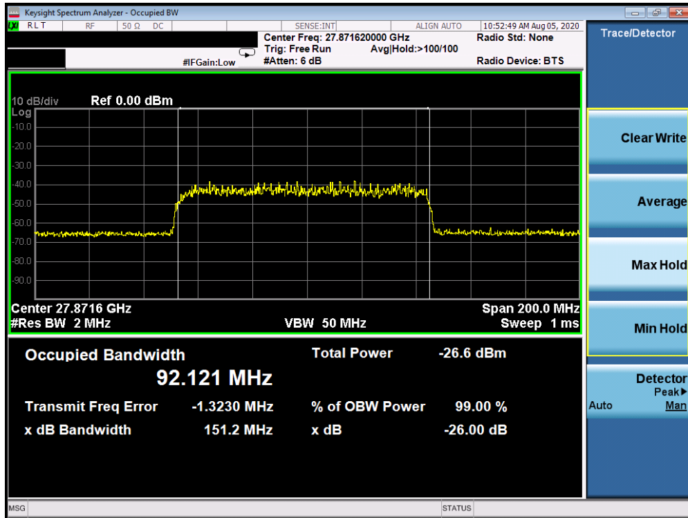
Plot 7-11. Ant 3 Occupied Bandwidth Plot (100MHz-1CC – 64QAM – Mid Channel)
