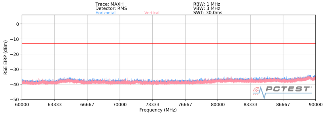
Plot 7-38. Ant 1-n261 Radiated Spurious Plot (1CC QPSK Mid Channel MIMO)
