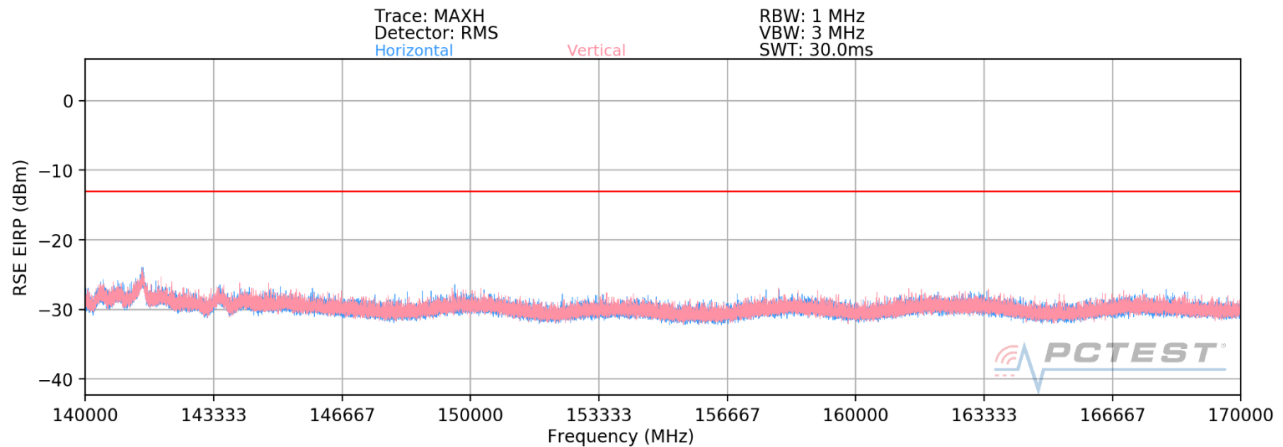
Plot 7-53. Ant 2 - n260 Radiated Spurious Plot (1CC QPSK Mid Channel MIMO)
