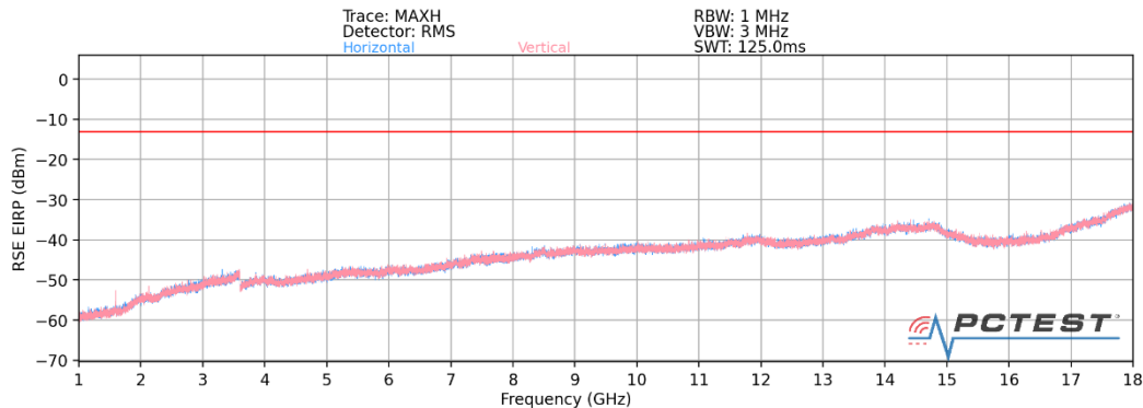
Plot 7-48. Ant 3 - n260 Radiated Spurious Plot (1CC QPSK Mid Channel MIMO)
