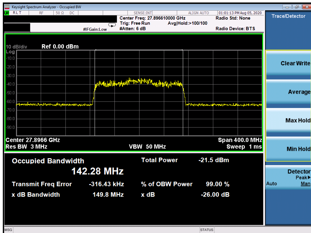
Plot 7-14. Ant 3 Occupied Bandwidth Plot (100MHz-2CC – 16QAM – Mid Channel)
