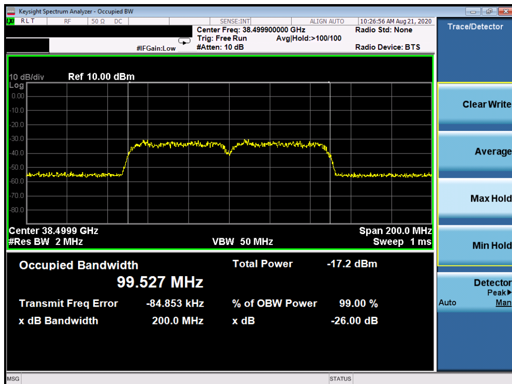
Plot 7-24. Ant 3 Occupied Bandwidth Plot (50MHz-2CC – pi/2-BPSK – Mid Channel)
