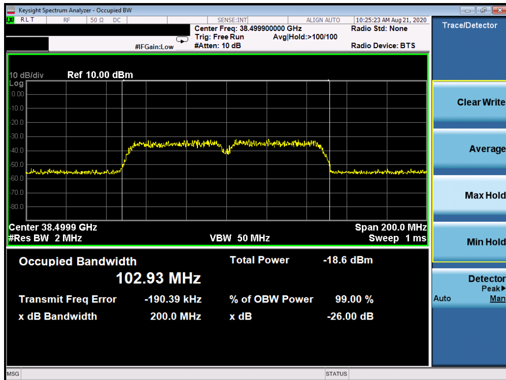
Plot 7-23. Ant 3 Occupied Bandwidth Plot (50MHz-2CC – 64QAM – Mid Channel)
