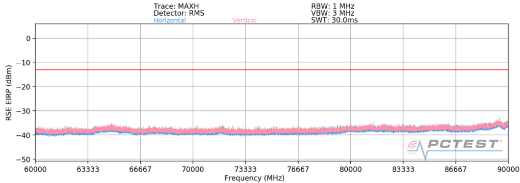
Plot 7-36. Ant 1-n260 Radiated Spurious Plot (1CC QPSK Mid Channel MIMO)
