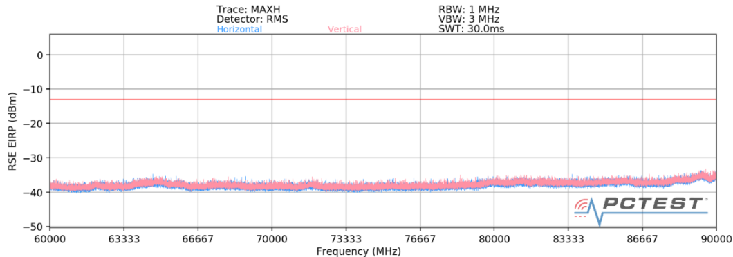
Plot 7-38. Ant 3-n261 Radiated Spurious Plot (1CC QPSK Mid Channel MIMO)
