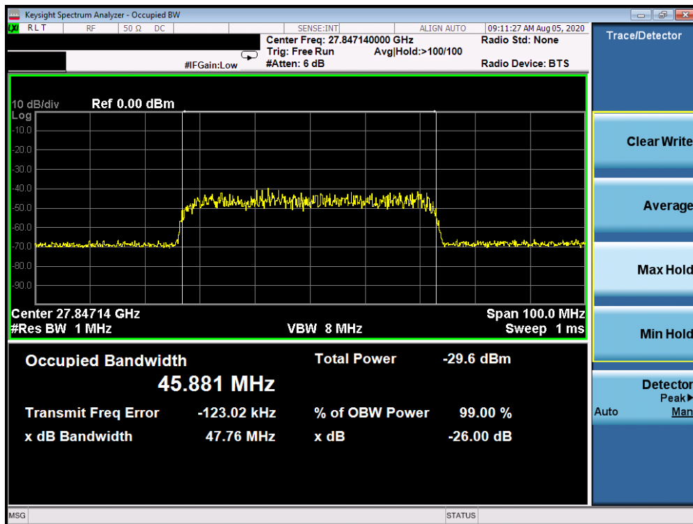
Plot 7-2. Ant 3 Occupied Bandwidth Plot (50MHz-1CC – 16QAM – Mid Channel)
