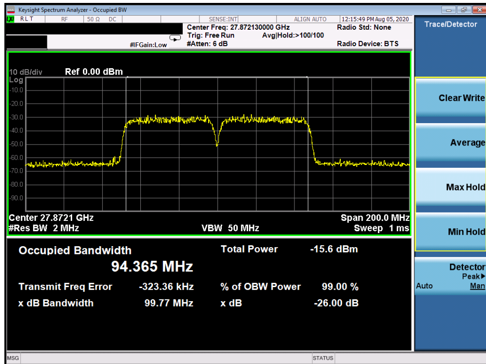
Plot 7-8. Ant 3 Occupied Bandwidth Plot (50MHz-2CC – pi/2-BPSK – Mid Channel)
