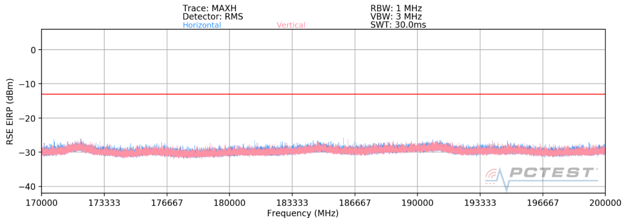
Plot 7-54. Ant 2 - n260 Radiated Spurious Plot (1CC QPSK Mid Channel MIMO)
