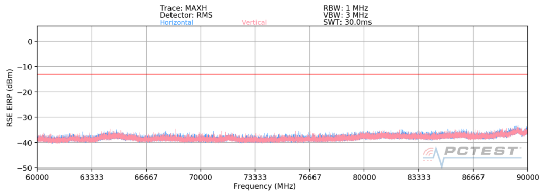
Plot 7-37. Ant 2-n260 Radiated Spurious Plot (1CC QPSK Mid Channel MIMO)
