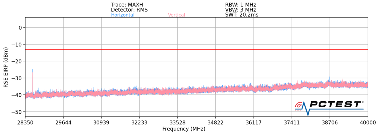
Plot 7-36. Ant 1-n261 Radiated Spurious Plot (1CC QPSK Mid Channel MIMO)
