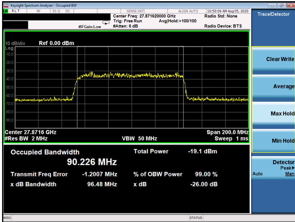
Plot 7-9. Ant 3 Occupied Bandwidth Plot (100MHz-1CC – QPSK – Mid Channel)
