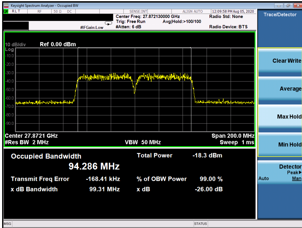
Plot 7-5. Ant 3 Occupied Bandwidth Plot (50MHz-2CC – QPSK – Mid Channel)
