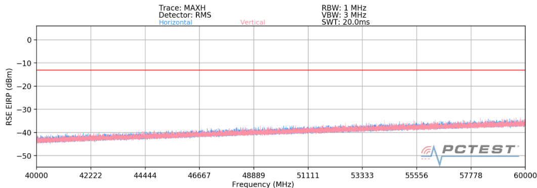
Plot 7-50. Ant 1-n260 Radiated Spurious Plot (1CC QPSK Mid Channel MIMO)
