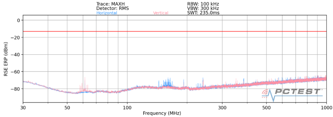
Plot 7-33. Ant 1- n261 Radiated Spurious Plot (1CC QPSK Mid Channel MIMO)
