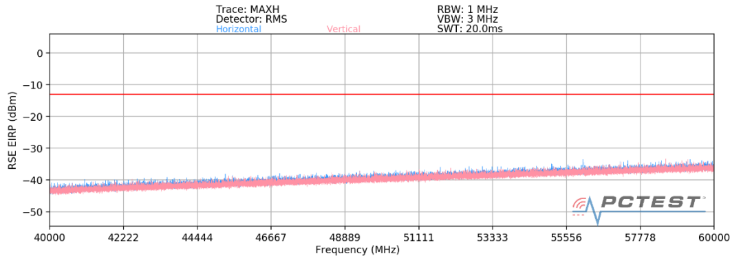
Plot 7-50. Ant 2 - n260 Radiated Spurious Plot (1CC QPSK Mid Channel MIMO)
