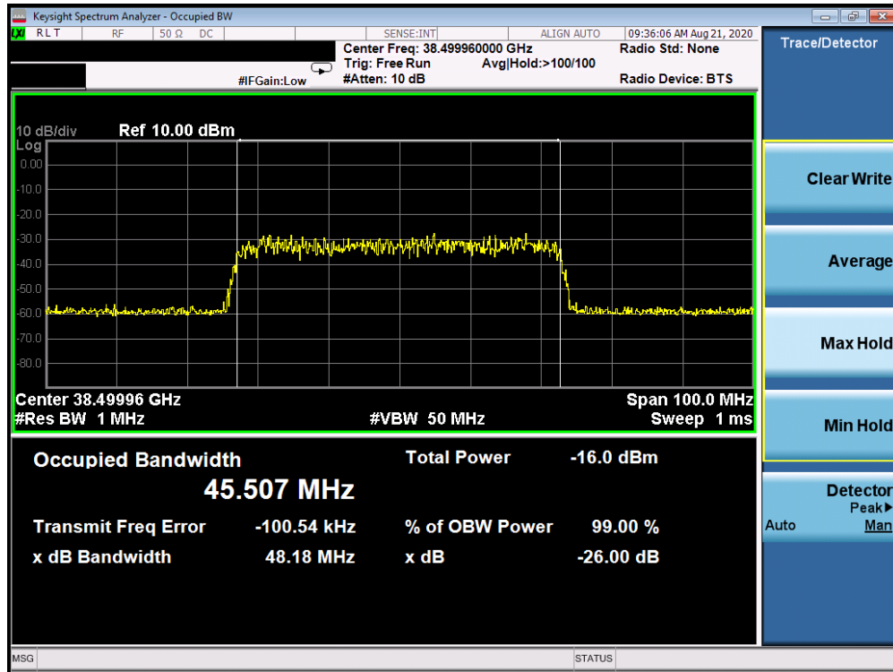
Plot 7-17. Ant 3 Occupied Bandwidth Plot (50MHz-1CC – QPSK – Mid Channel)
