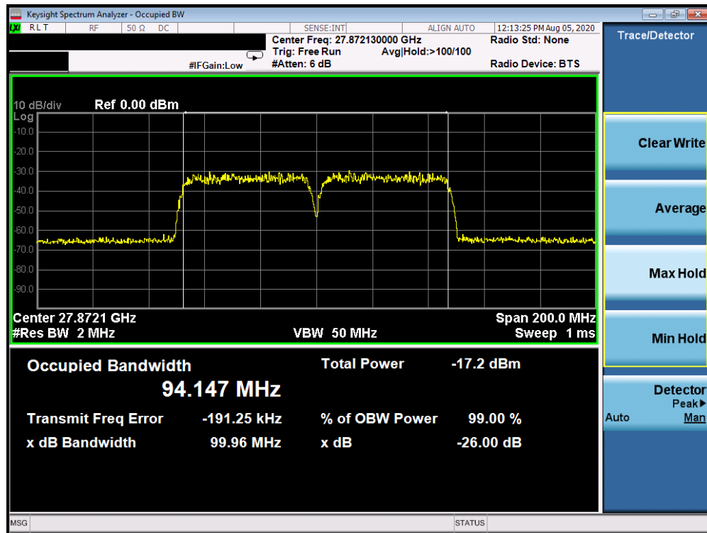
Plot 7-7. Ant 3 Occupied Bandwidth Plot (50MHz-2CC – 64QAM – Mid Channel)
