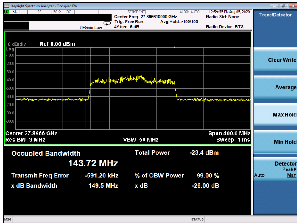
Plot 7-13. Ant 3 Occupied Bandwidth Plot (100MHz-2CC – QPSK – Mid Channel)
