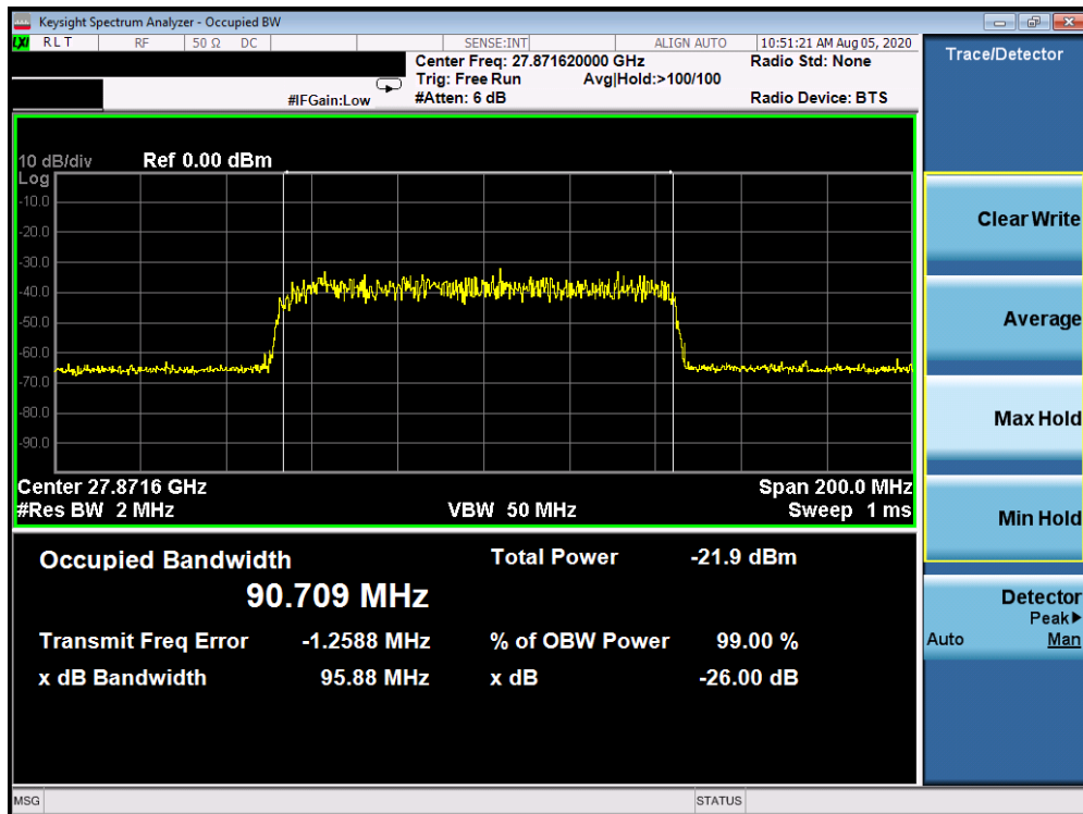
Plot 7-10. Ant 3 Occupied Bandwidth Plot (100MHz-1CC – 16QAM – Mid Channel)
