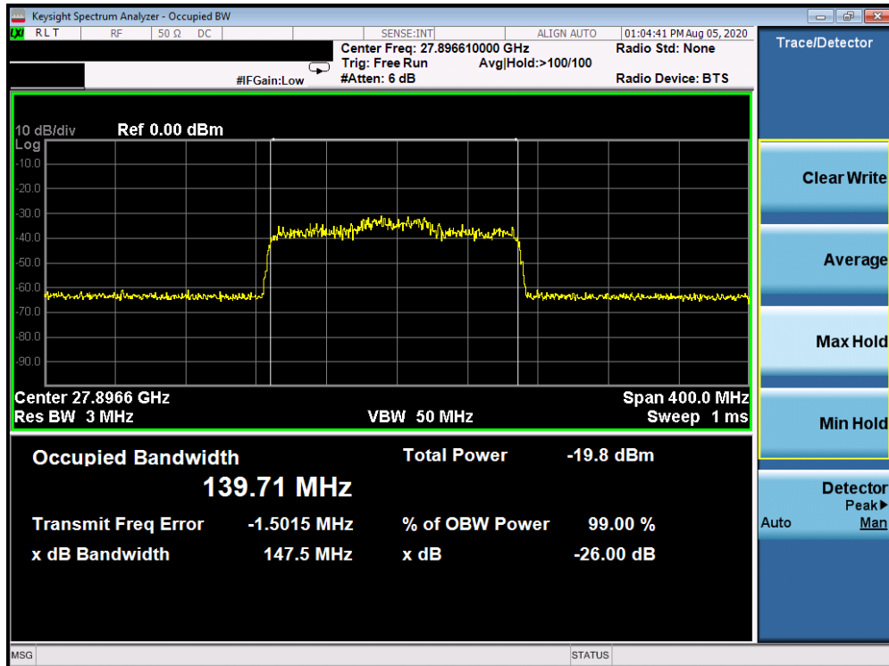
Plot 7-16. Ant 3 Occupied Bandwidth Plot (100MHz-2CC – pi/2-BPSK – Mid Channel)
