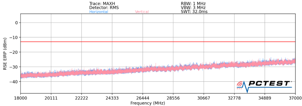
Plot 7-49. Ant 1-n260 Radiated Spurious Plot (1CC QPSK Mid Channel MIMO)
