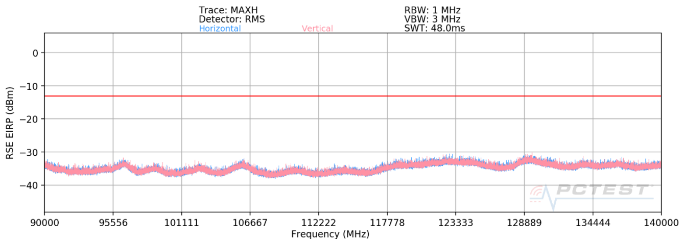
Plot 7-60. Ant 1-n260 Radiated Spurious Plot (1CC QPSK Mid Channel MIMO)
