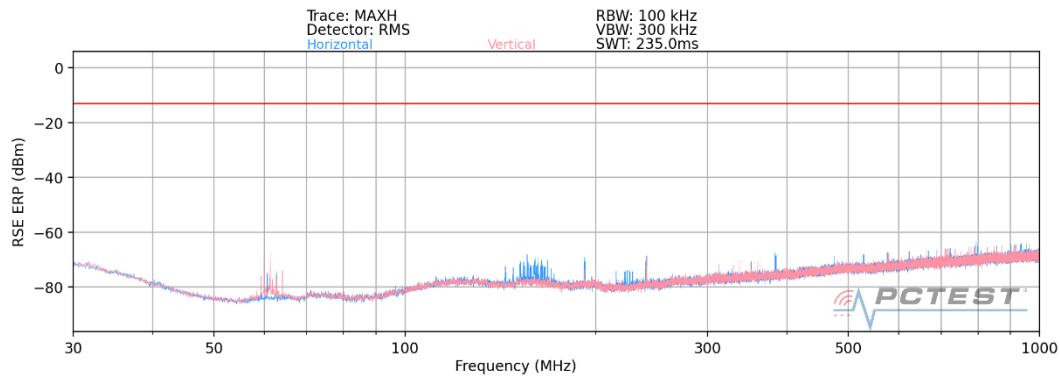
Plot 7-34. Ant 2 - n261 Radiated Spurious Plot (1CC QPSK Mid Channel MIMO)
