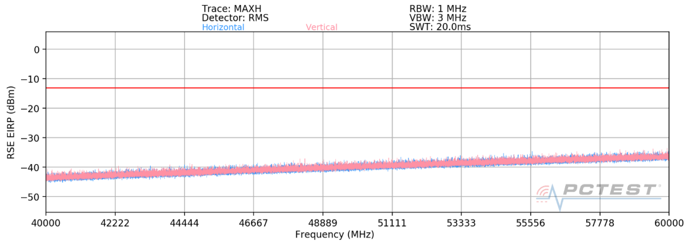
Plot 7-44. Ant 2-n261 Radiated Spurious Plot (1CC QPSK Mid Channel MIMO)
