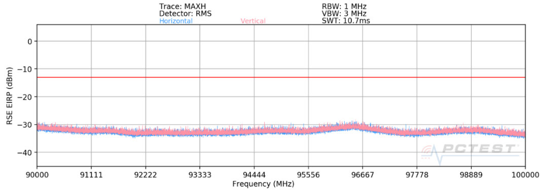
Plot 7-39. Ant 1-n261 Radiated Spurious Plot (1CC QPSK Mid Channel MIMO)
