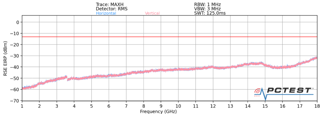
Plot 7-48. Ant 1-n260 Radiated Spurious Plot (1CC QPSK Mid Channel MIMO)
