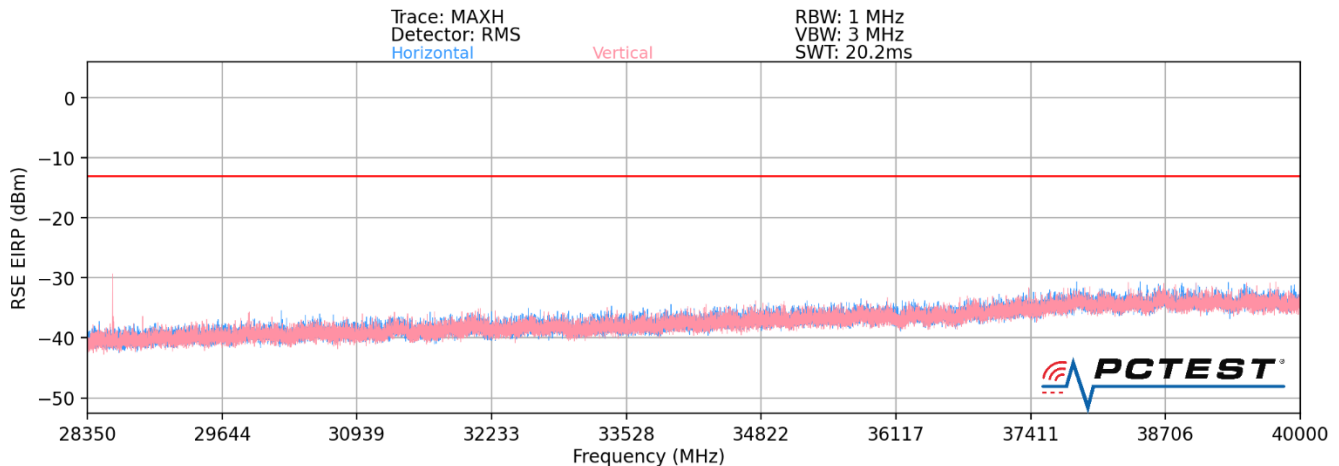
Plot 7-36. Ant 2 - n261 Radiated Spurious Plot (1CC QPSK Mid Channel MIMO)
