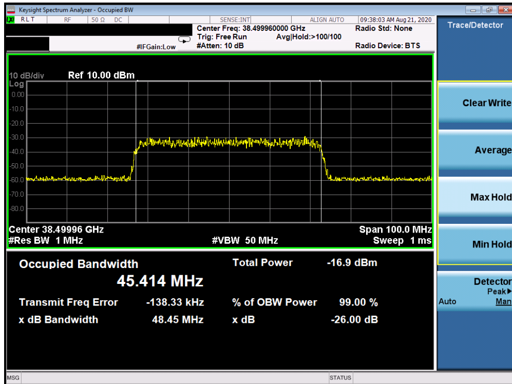
Plot 7-18. Ant 3 Occupied Bandwidth Plot (50MHz-1CC – 16QAM – Mid Channel)
