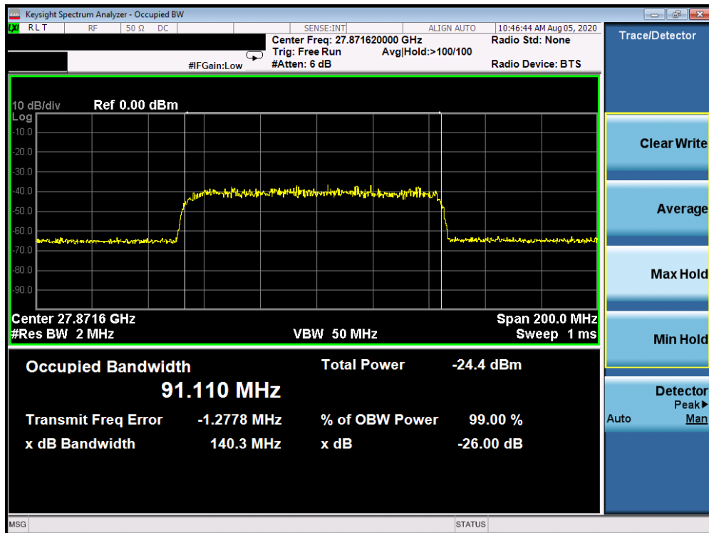
Plot 7-12. Ant 3 Occupied Bandwidth Plot (100MHz-1CC – pi/2-BPSK – Mid Channel)
