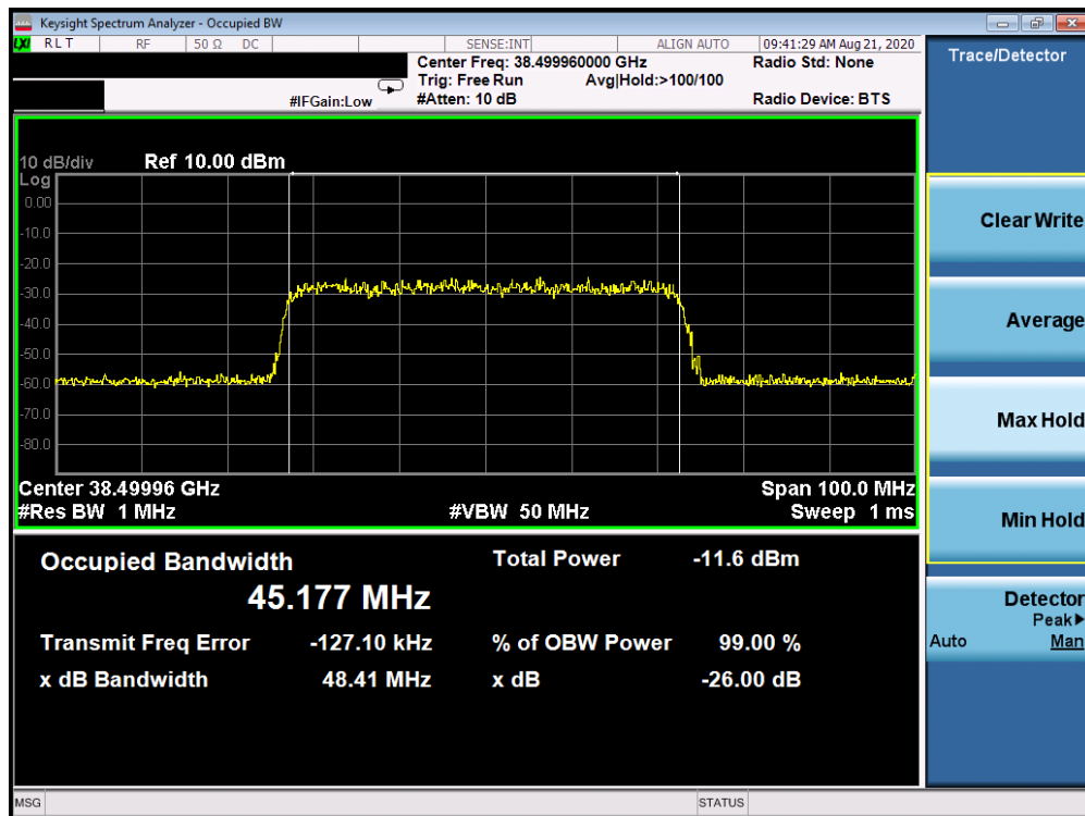
Plot 7-20. Ant 3 Occupied Bandwidth Plot (50MHz-1CC – pi/2-BPSK – Mid Channel)
