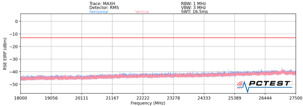
Plot 7-35. Ant 2 - n261 Radiated Spurious Plot (1CC QPSK Mid Channel MIMO)
