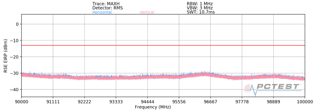
Plot 7-39. Ant 3 - n261 Radiated Spurious Plot (1CC QPSK Mid Channel MIMO)
