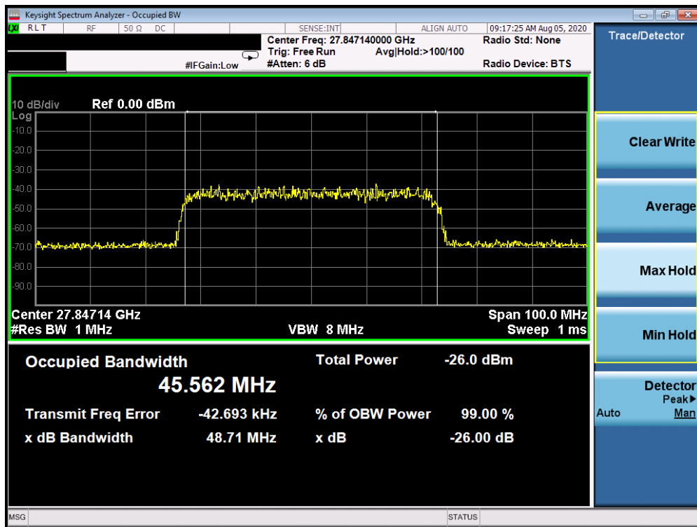
Plot 7-4. Ant 3 Occupied Bandwidth Plot (50MHz-1CC – pi/2-BPSK – Mid Channel)
