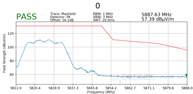
Plot 7-226. Radiated Upper Band Edge Plot MIMO (Peak – UNII Band 3)
