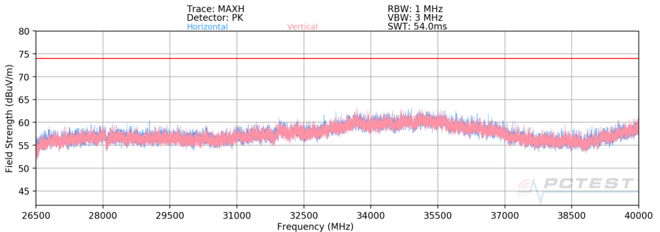
Plot 7-174. Radiated Spurious Plot 26.5GHz - 40GHz MIMO (802.11n)
