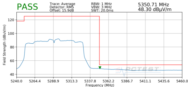
Plot 7-215. Radiated Upper Band Edge Plot SISO ANT2 (Average – UNII Band 2A)
