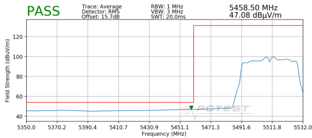
Plot 7-210. Radiated Lower Band Edge Plot SISO ANT2 (Average – UNII Band 2C)
