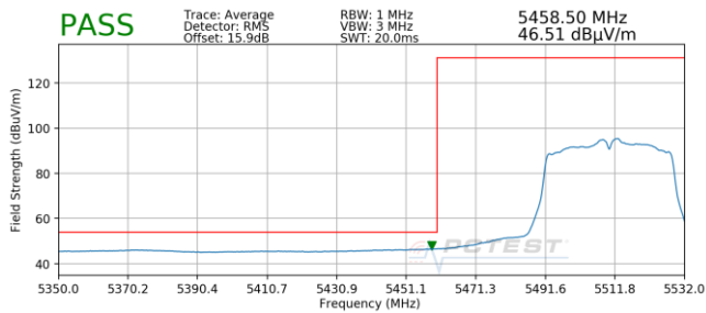
Plot 7-231. Radiated Lower Band Edge Plot MIMO (Average – UNII Band 2C)
