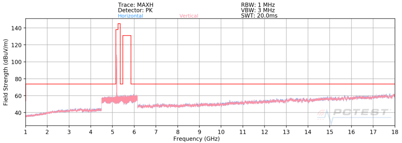
Plot 7-169. Radiated Spurious Plot above 1GHz MIMO (802.11n – U1 Ch. 40)
