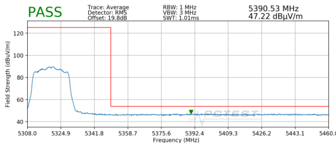
Plot 7-180. Radiated Upper Band Edge Plot SISO ANT1 (Average – UNII Band 2A)
