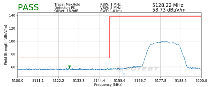
Plot 7-179. Radiated Lower Band Edge Plot SISO ANT1 (Peak – UNII Band 1)
