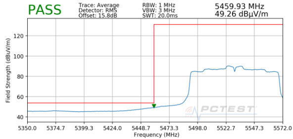
Plot 7-196. Radiated Lower Band Edge Plot SISO ANT1 (Average – UNII Band 2C)
