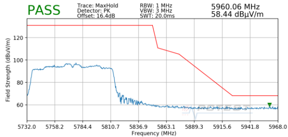
Plot 7-198. Radiated Upper Band Edge Plot SISO ANT1 (Peak – UNII Band 3)
