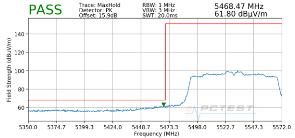
Plot 7-197. Radiated Lower Band Edge Plot SISO ANT1 (Peak – UNII Band 2C)
