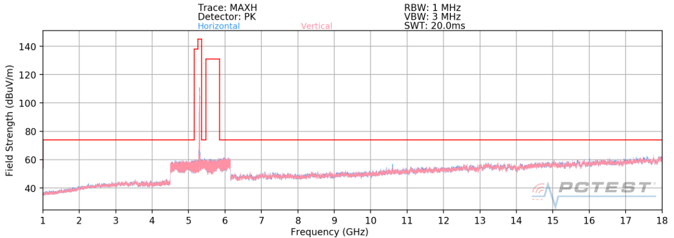
Plot 7-170. Radiated Spurious Plot above 1GHz MIMO (802.11n – U2A Ch. 56)
