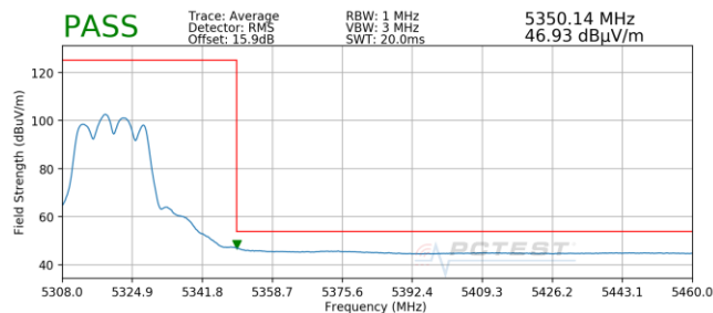
Plot 7-222. Radiated Upper Band Edge Plot MIMO (Average – UNII Band 2A)
