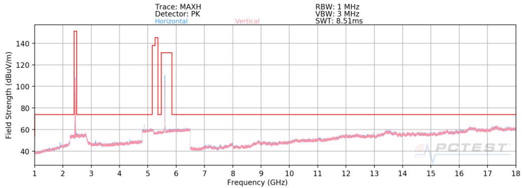
Plot 7-175. Radiated Spurious Plot above 1GHz (2.4GHz – 5GHz)
