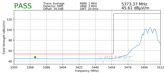
Plot 7-224. Radiated Lower Band Edge Plot MIMO (Average – UNII Band 2C)
