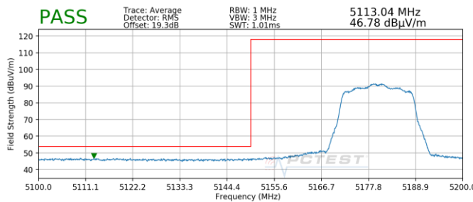
Plot 7-178. Radiated Lower Band Edge Plot SISO ANT1 (Average – UNII Band 1)
