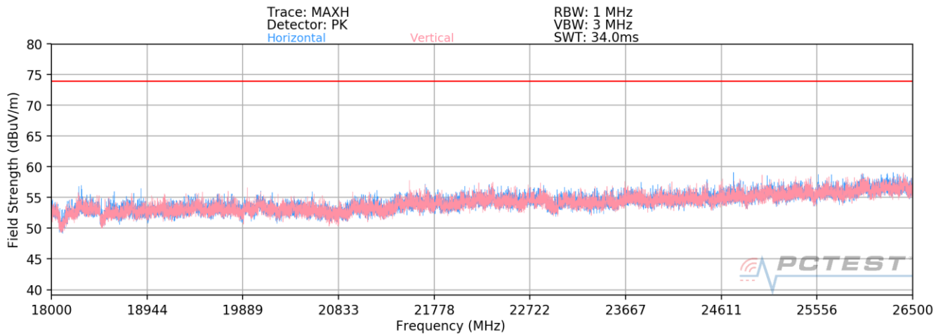
Plot 7-173. Radiated Spurious Plot above 18GHz - 26.5GHz MIMO (802.11n)
