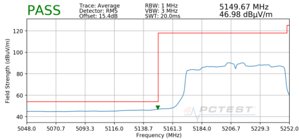
Plot 7-213. Radiated Lower Band Edge Plot SISO ANT2 (Average – UNII Band 1)
