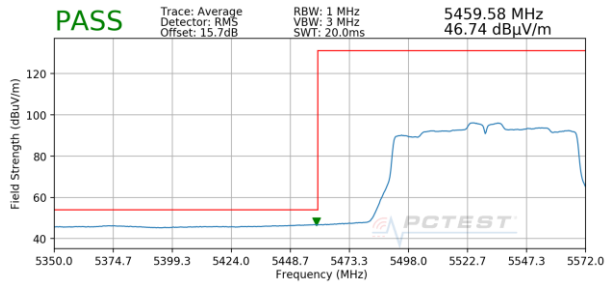
Plot 7-217. Radiated Lower Band Edge Plot SISO ANT2 (Average – UNII Band 2C)
