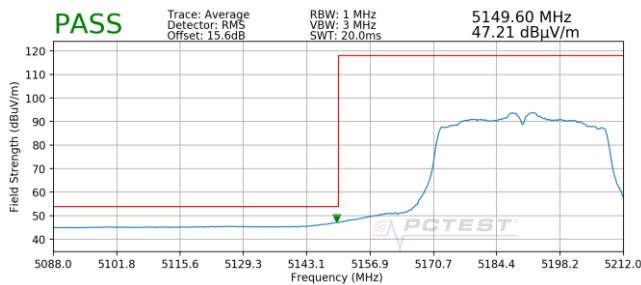
Plot 7-227. Radiated Lower Band Edge Plot MIMO (Average – UNII Band 1)
