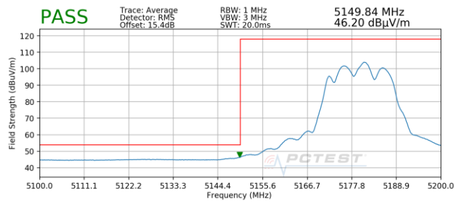
Plot 7-220. Radiated Lower Band Edge Plot MIMO (Average – UNII Band 1)
