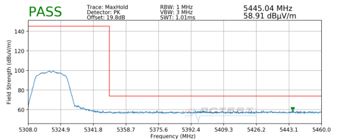
Plot 7-181. Radiated Upper Band Edge Plot SISO ANT1 (Peak – UNII Band 2A)
