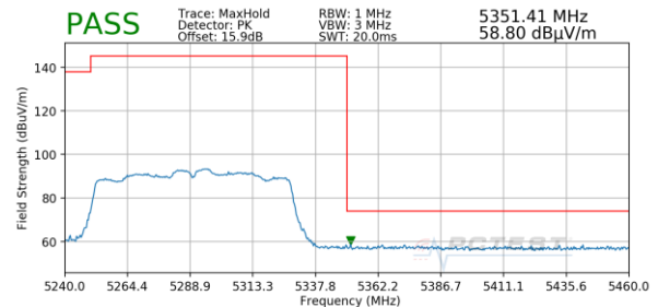
Plot 7-195. Radiated Upper Band Edge Plot SISO ANT1 (Peak – UNII Band 2A)
