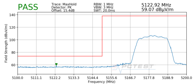
Plot 7-200. Radiated Lower Band Edge Plot SISO ANT2 (Peak – UNII Band 1)
