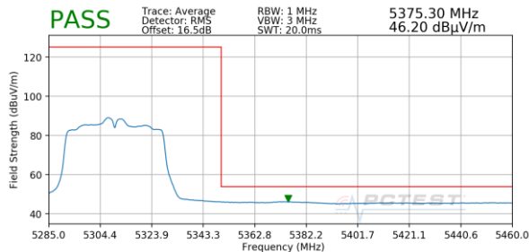
Plot 7-187. Radiated Upper Band Edge Plot SISO ANT1 (Average – UNII Band 2A)
