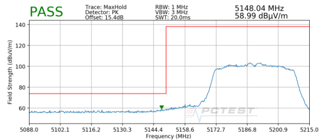
Plot 7-228. Radiated Lower Band Edge Plot MIMO (Peak – UNII Band 1)
