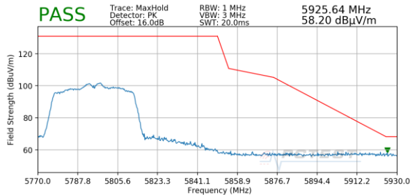
Plot 7-191. Radiated Upper Band Edge Plot SISO ANT1 (Peak – UNII Band 3)
