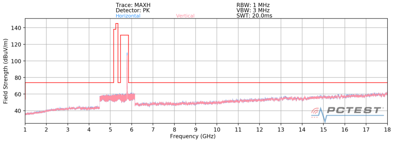
Plot 7-172. Radiated Spurious Plot above 1GHz MIMO (802.11n – U3 Ch. 157)
