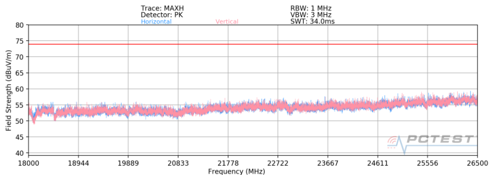
Plot 7-176. Radiated Spurious Plot 18GHz – 26.5GHz (2.4GHz – 5GHz)
