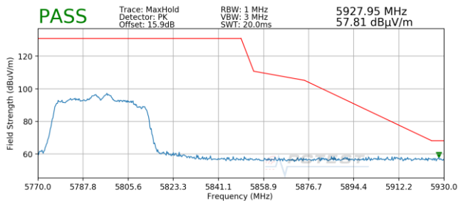
Plot 7-233. Radiated Upper Band Edge Plot MIMO (Peak – UNII Band 3)
