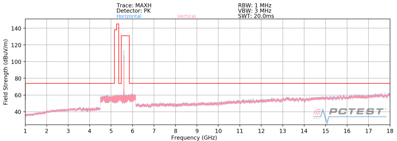
Plot 7-171. Radiated Spurious Plot above 1GHz MIMO (802.11n – U2C Ch. 116)
