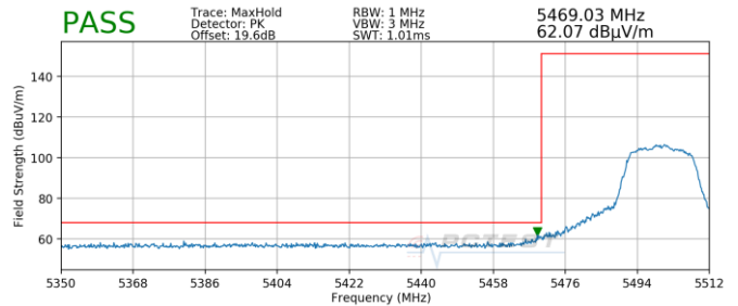
Plot 7-183. Radiated Lower Band Edge Plot SISO ANT1 (Peak – UNII Band 2C)
