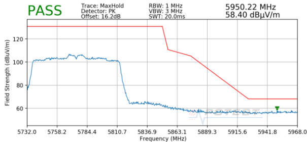
Plot 7-219. Radiated Upper Band Edge Plot SISO ANT2 (Peak – UNII Band 3)
