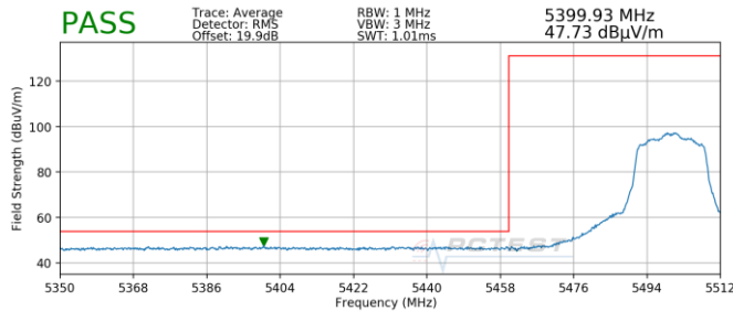
Plot 7-182. Radiated Lower Band Edge Plot SISO ANT1 (Average – UNII Band 2C)
