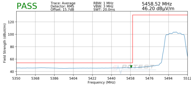
Plot 7-203. Radiated Lower Band Edge Plot SISO ANT2 (Average – UNII Band 2C)
