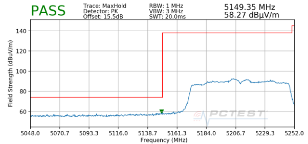
Plot 7-193. Radiated Lower Band Edge Plot SISO ANT1 (Peak – UNII Band 1)
