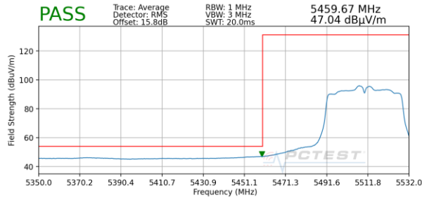
Plot 7-189. Radiated Lower Band Edge Plot SISO ANT1 (Average – UNII Band 2C)
