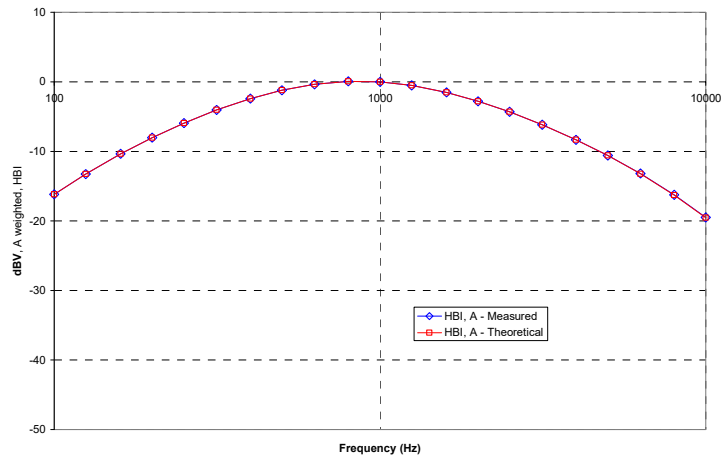
Figure 4-9 ABM2 Frequency Response Validation
