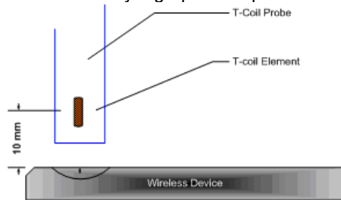
Figure 4-12 Measurement Distance
