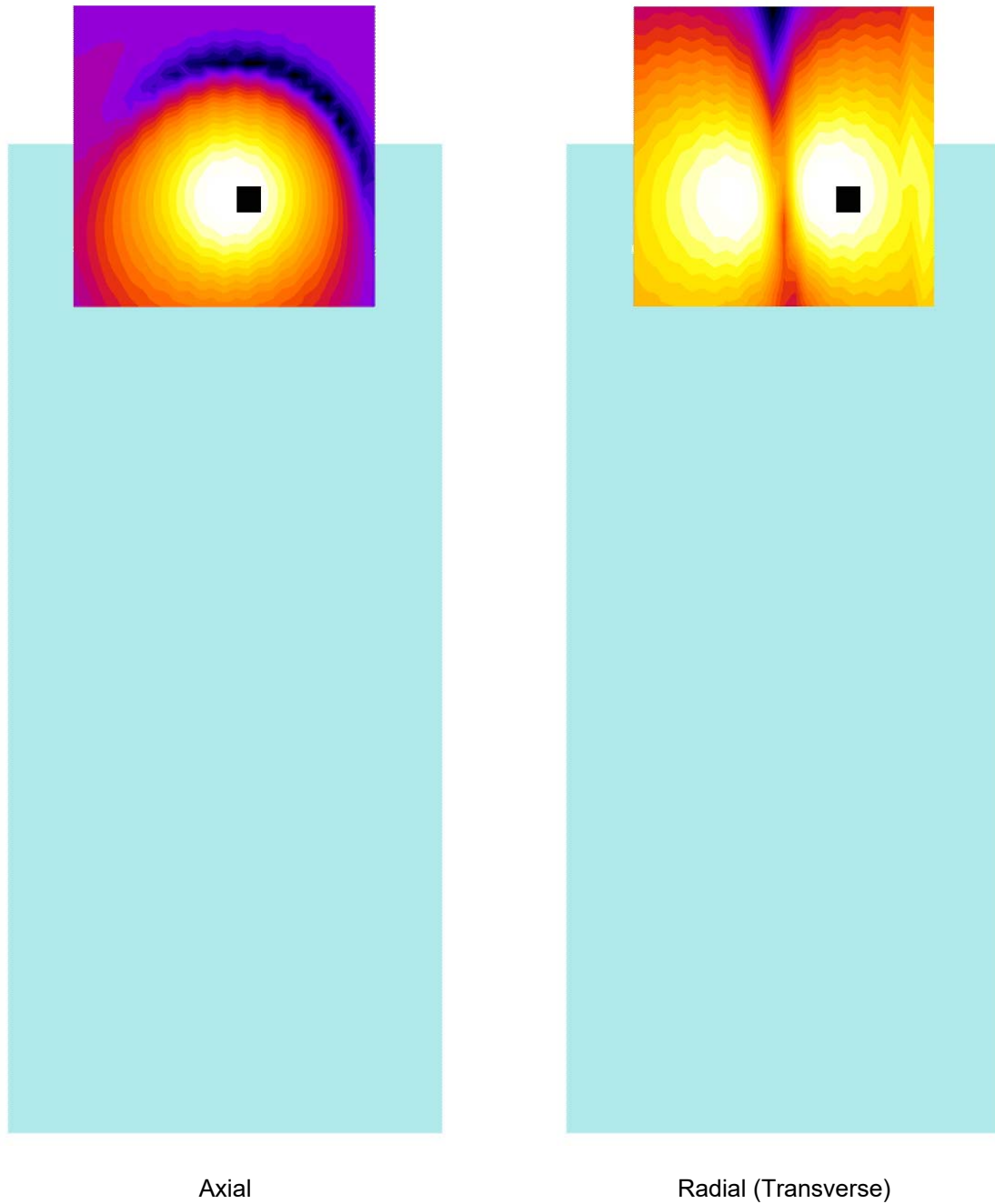
Figure 9-1 T-Coil Scan Overlay Magnetic Field Distributions
