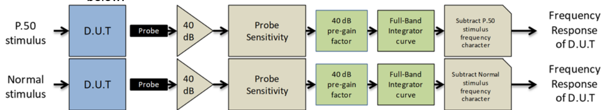
Figure 4-8 Frequency Response Validation
