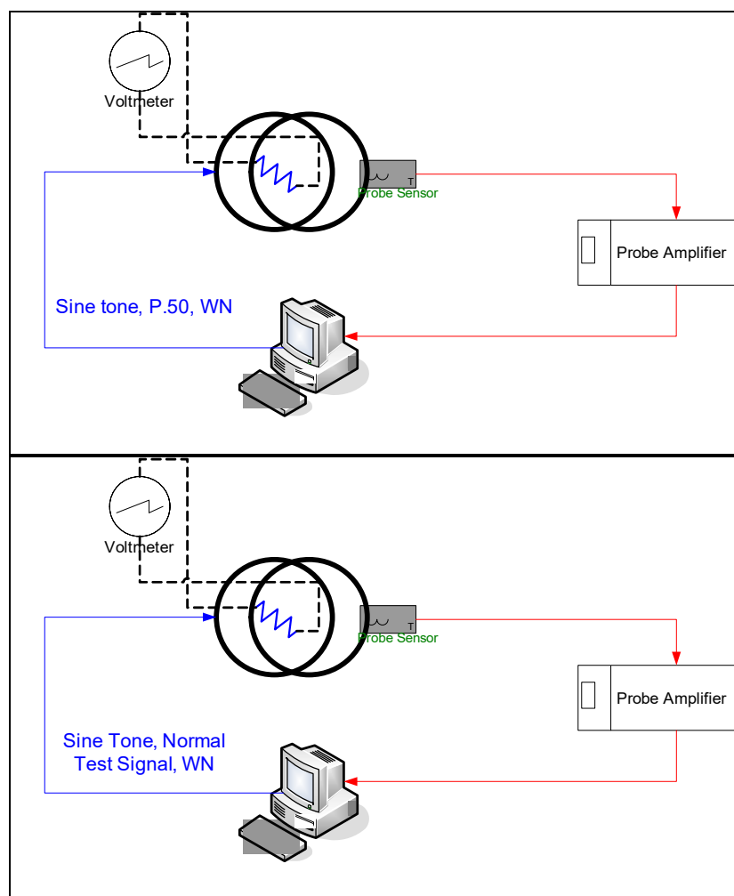
Figure 4-1 Validation Setup with Helmholtz Coil
