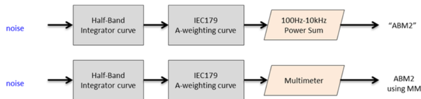
Figure 4-10 ABM2 Validation Block Diagram
