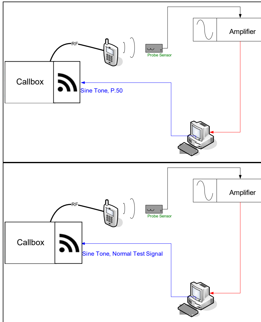
Figure 4-2 T-Coil Test Setup
