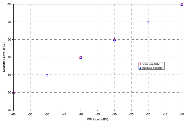
Figure 4-11 ABM2 Power Sum Validation
