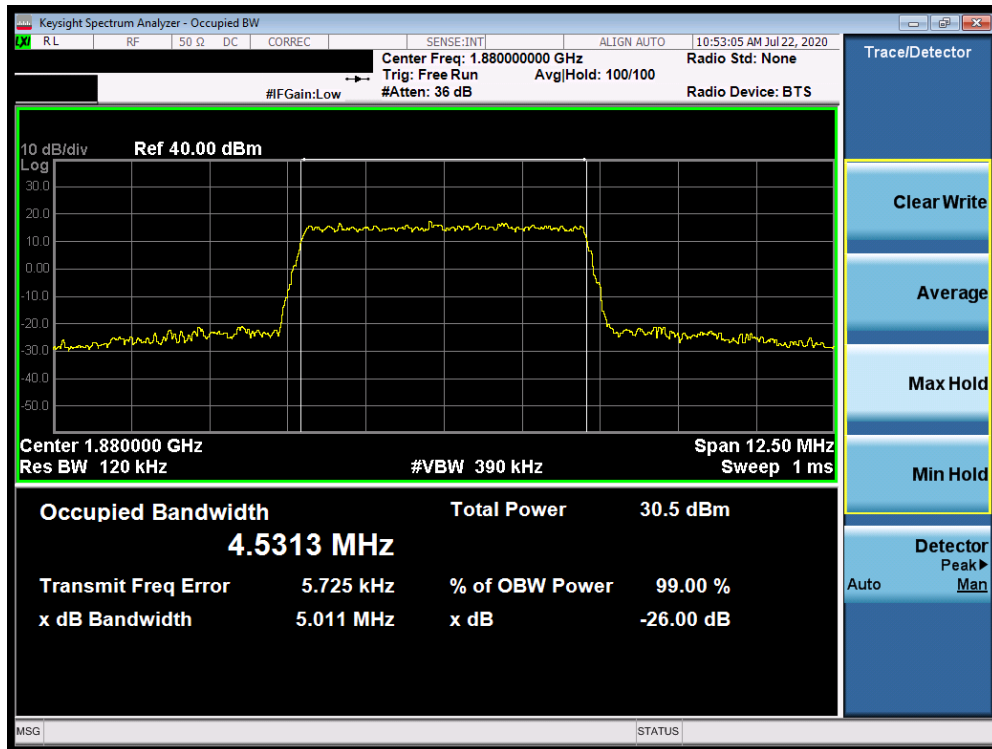
Plot 7-97. Occupied Bandwidth Plot (Band 2 - 5.0MHz 64-QAM - Full RB Configuration)
