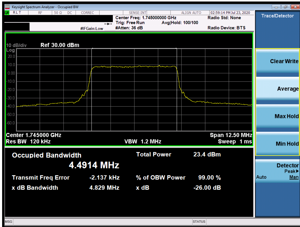
Plot 7-71. Occupied Bandwidth Plot (NR Band n66 - 5.0MHz CP-OFDM 16QAM - Full RB)
