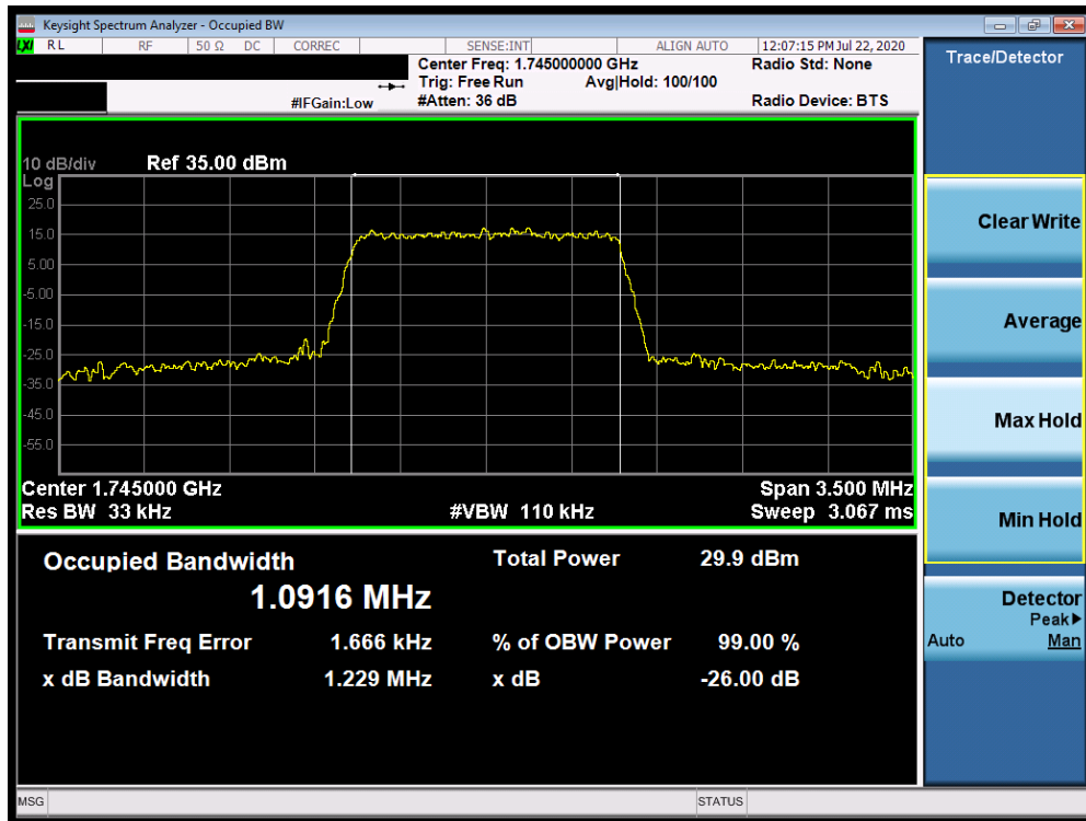
Plot 7-53. Occupied Bandwidth Plot (Band 66/4 - 1.4.0MHz 64-QAM - Full RB Configuration)
