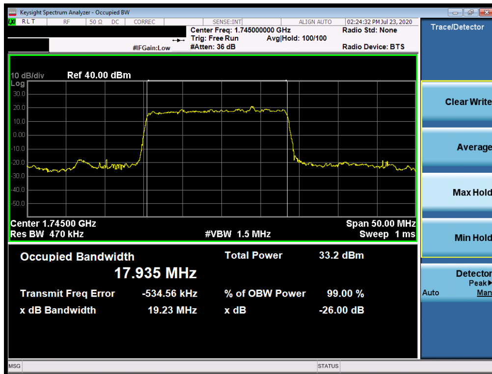
Plot 7-84. Occupied Bandwidth Plot (NR Band n66 - 20.0MHz DFT-s-OFDM BPSK - Full RB)
