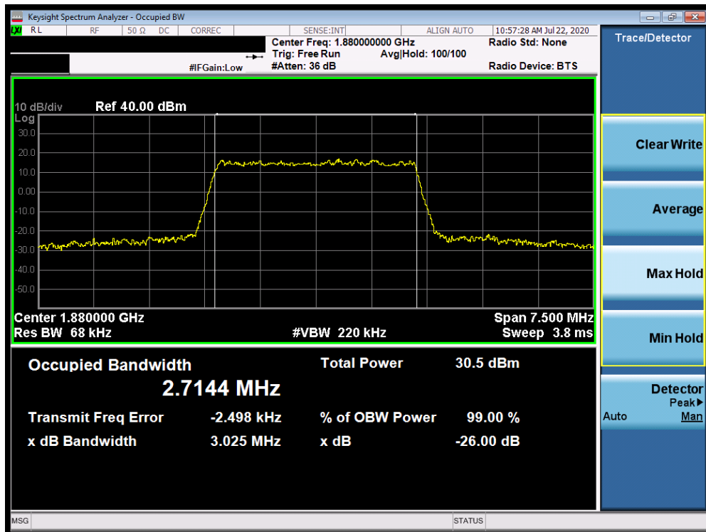
Plot 7-94. Occupied Bandwidth Plot (Band 2 - 3.0MHz 64-QAM - Full RB Configuration)
