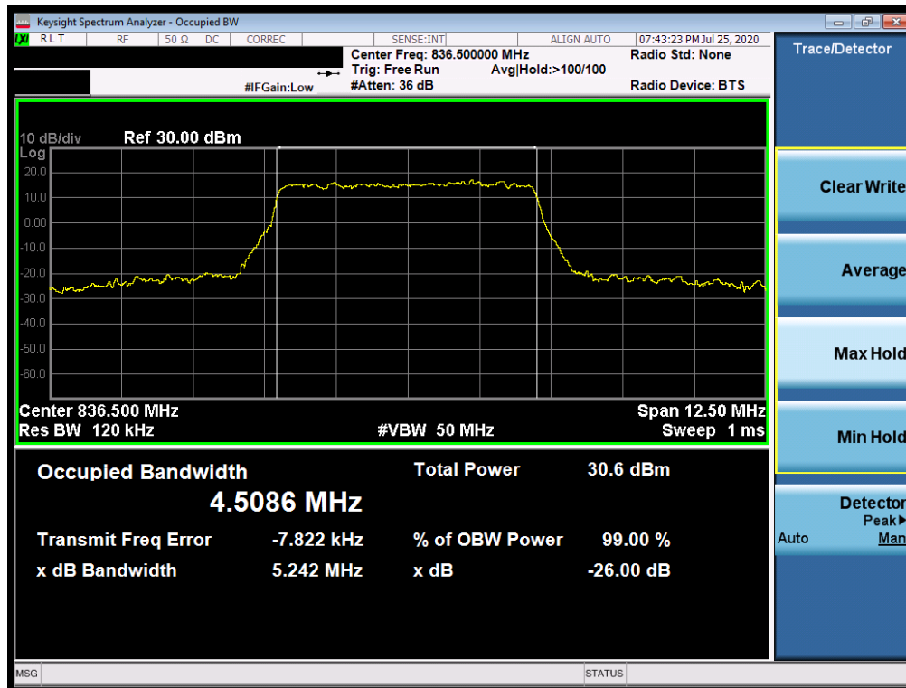
Plot 7-32. Occupied Bandwidth Plot (NR Band n5 - 5.0MHz CP-OFDM QPSK - Full RB)
