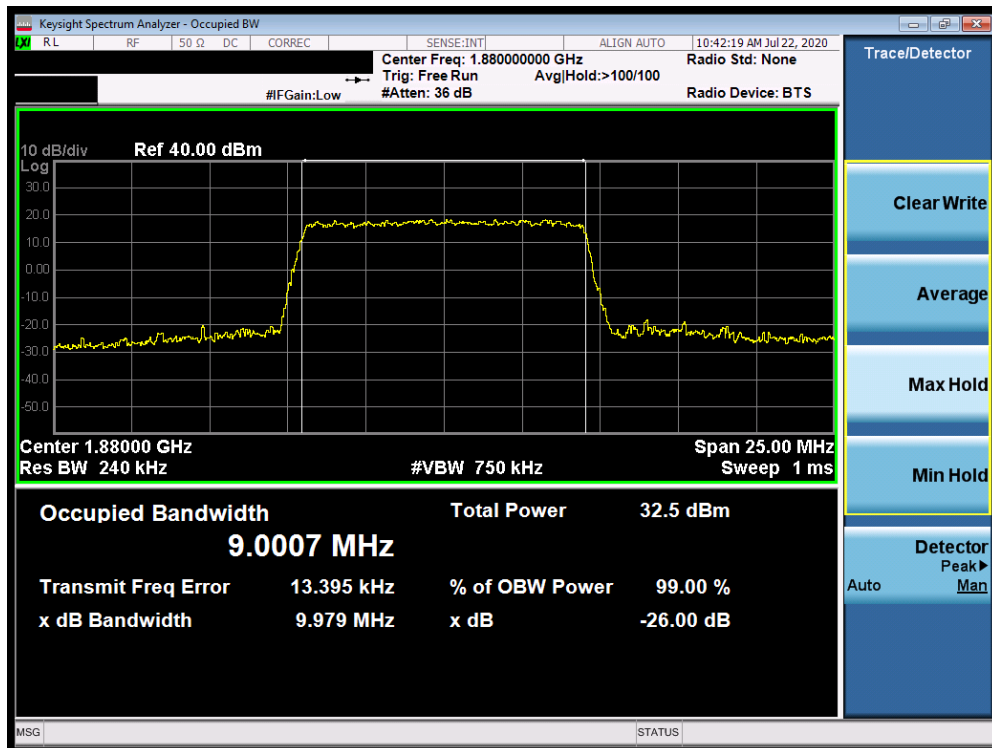
Plot 7-98. Occupied Bandwidth Plot (Band 2 - 10.0MHz QPSK - Full RB Configuration)
