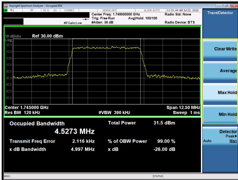
Plot 7-58. Occupied Bandwidth Plot (Band 66/4 - 5.0MHz 16-QAM - Full RB Configuration)
