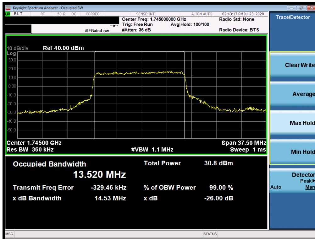
Plot 7-80. Occupied Bandwidth Plot (NR Band n66 - 15.0MHz CP-OFDM QPSK - Full RB)
