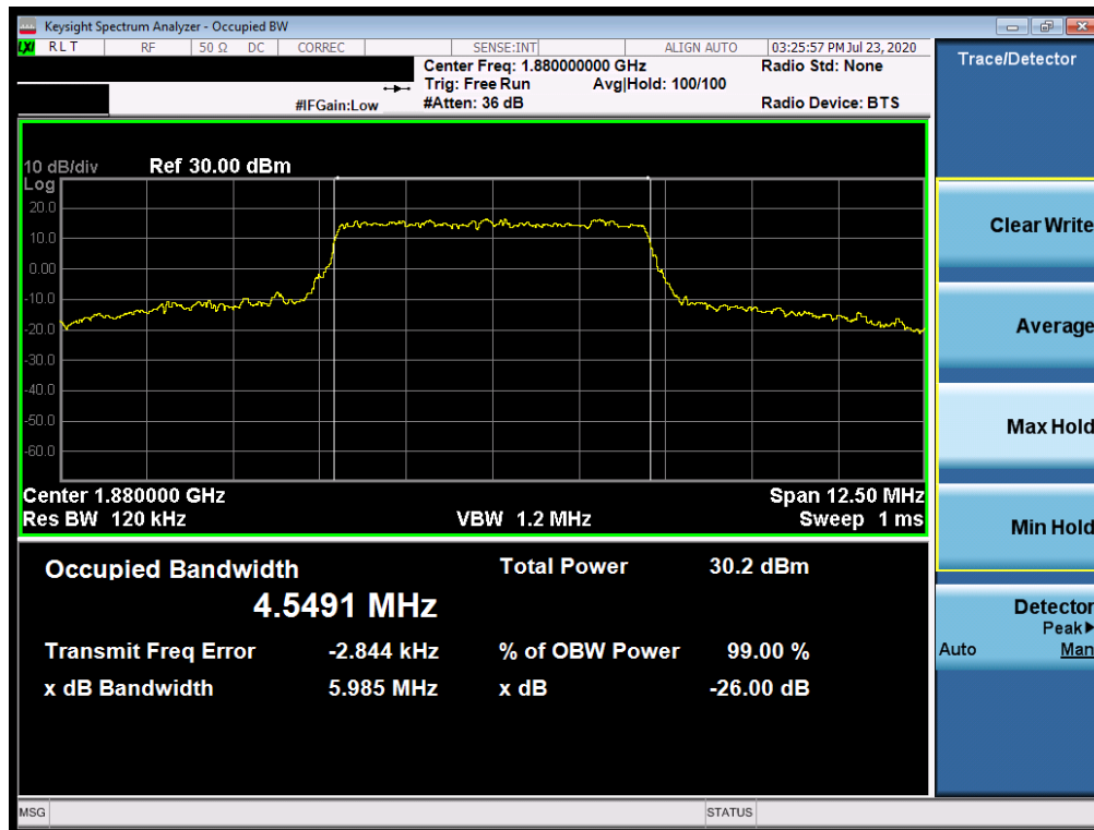
Plot 7-108. Occupied Bandwidth Plot (NR Band n2 - 5.0MHz CP-OFDM QPSK - Full RB)
