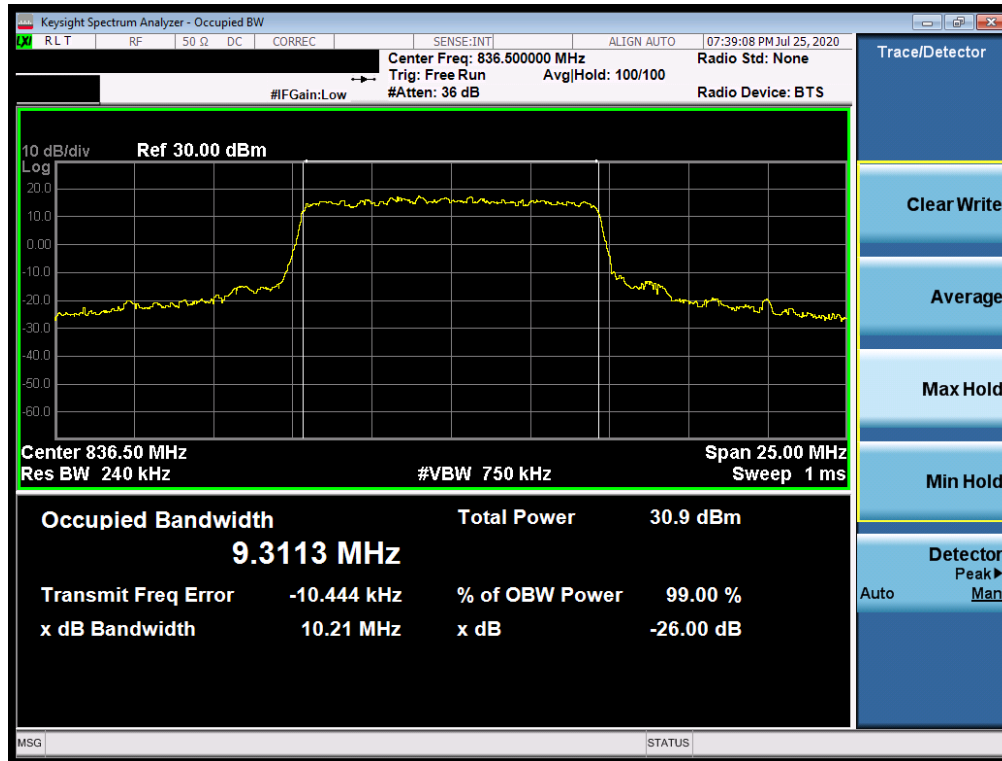
Plot 7-39. Occupied Bandwidth Plot (NR Band n5 - 10.0MHz CP-OFDM 64QAM - Full RB)
