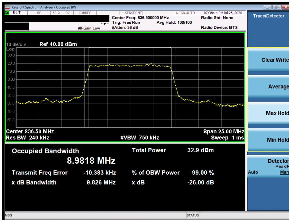
Plot 7-36. Occupied Bandwidth Plot (NR Band n5 - 10.0MHz DFT-s-OFDM BPSK - Full RB)
