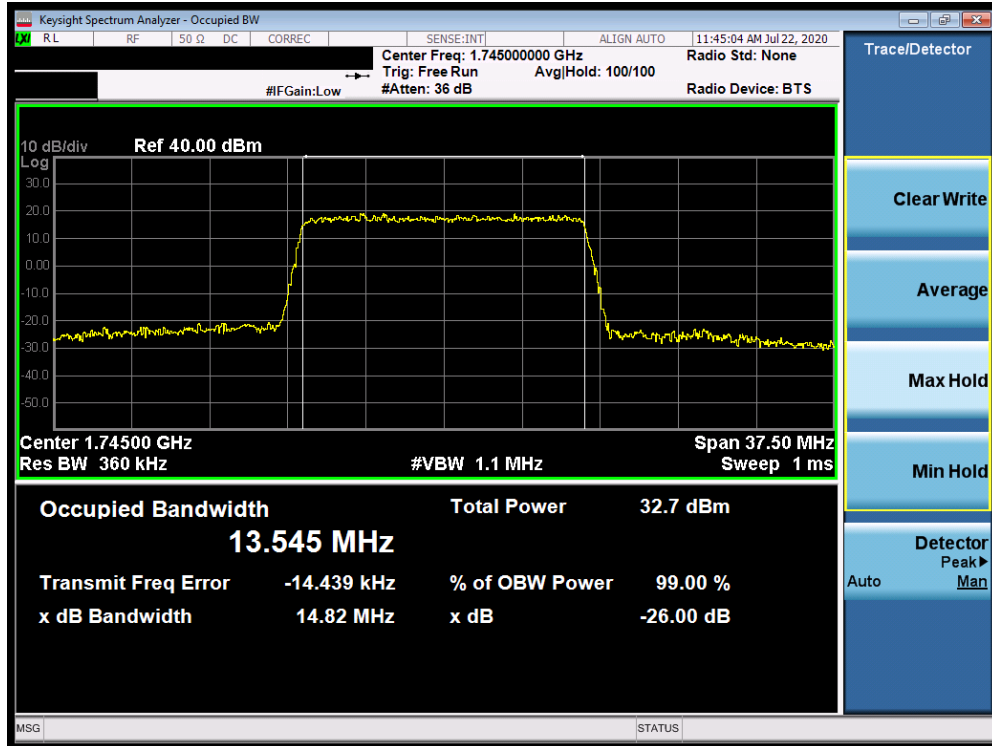
Plot 7-63. Occupied Bandwidth Plot (Band 66/4 - 15.0MHz QPSK - Full RB Configuration)
