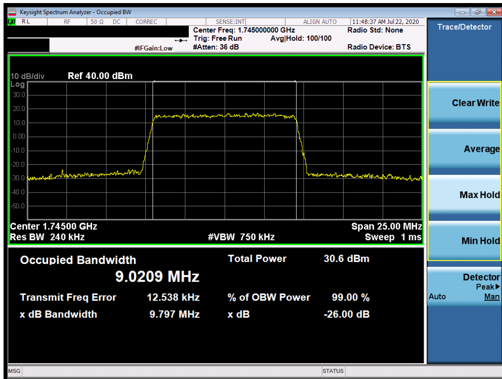
Plot 7-62. Occupied Bandwidth Plot (Band 66/4 - 10.0MHz 64-QAM - Full RB Configuration)
