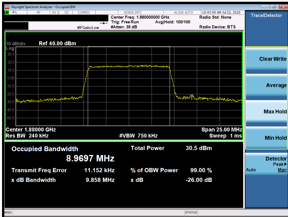
Plot 7-100. Occupied Bandwidth Plot (Band 2 - 10.0MHz 64-QAM - Full RB Configuration)
