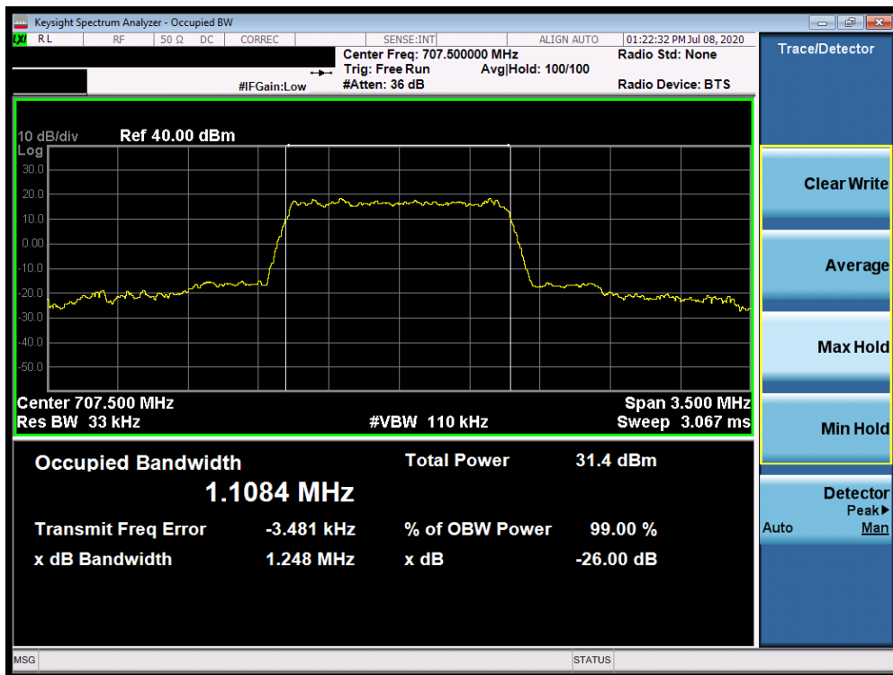
Plot 7-2. Occupied Bandwidth Plot (Band 12 - 1.4.0MHz 16-QAM - Full RB Configuration)
