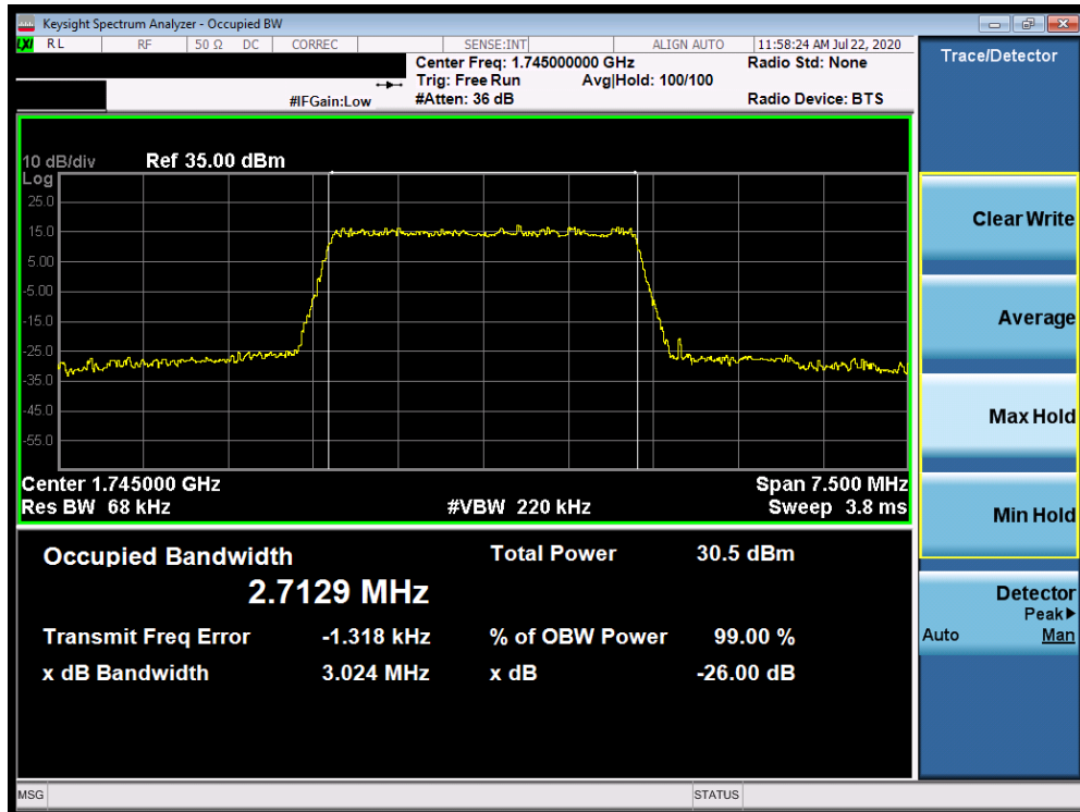
Plot 7-56. Occupied Bandwidth Plot (Band 66/4 - 3.0MHz 64-QAM - Full RB Configuration)
