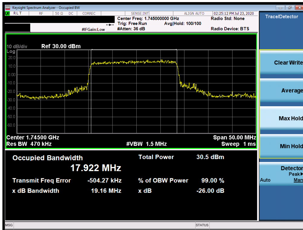
Plot 7-86. Occupied Bandwidth Plot (NR Band n66 - 20.0MHz CP-OFDM 16QAM - Full RB)
