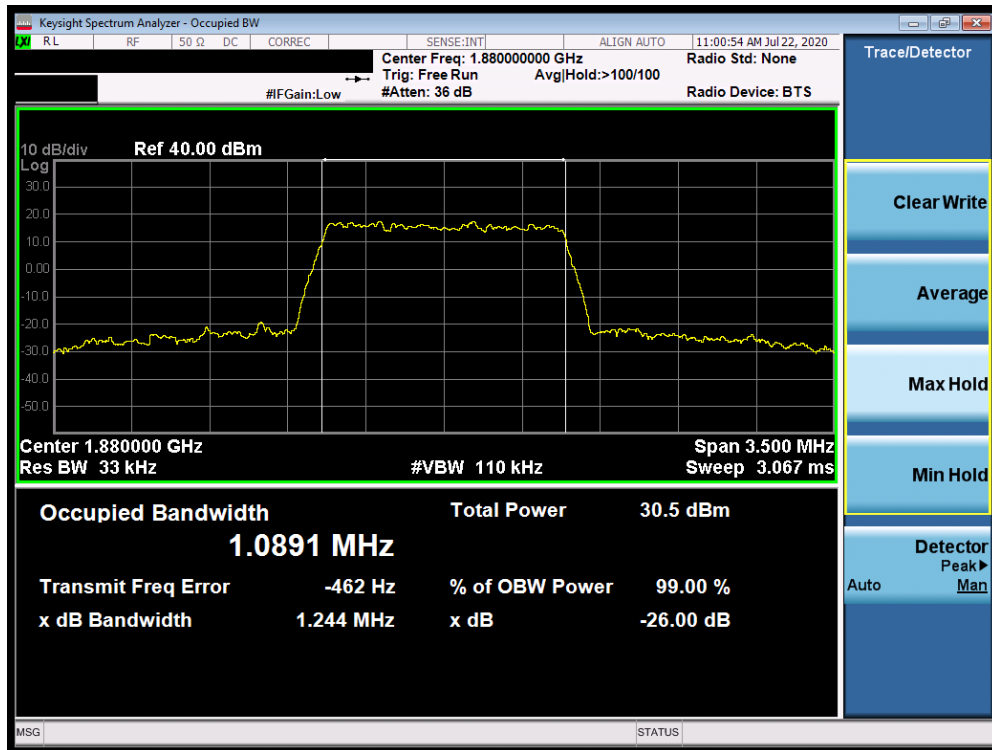
Plot 7-91. Occupied Bandwidth Plot (Band 2 - 1.4.0MHz 64-QAM - Full RB Configuration)
