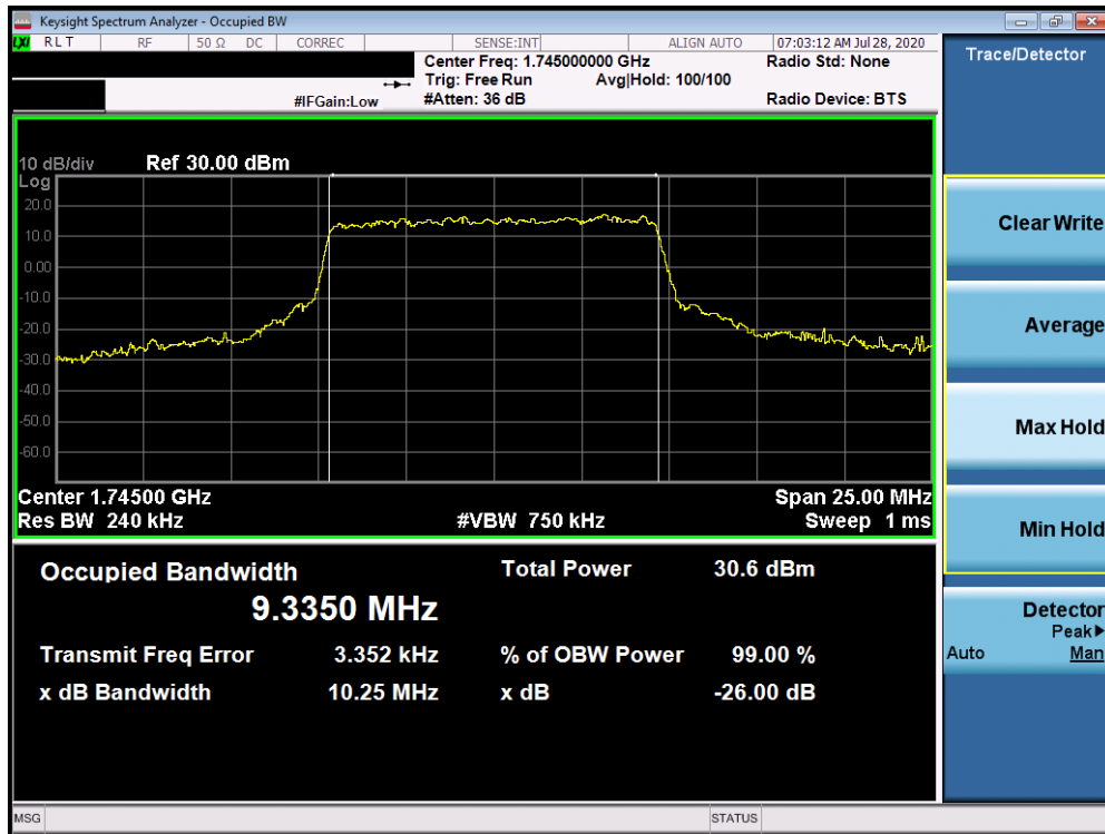
Plot 7-75. Occupied Bandwidth Plot (NR Band n66 - 10.0MHz CP-OFDM QPSK - Full RB)
