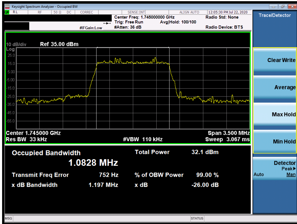
Plot 7-51. Occupied Bandwidth Plot (Band 66/4 - 1.4.0MHz QPSK - Full RB Configuration)
