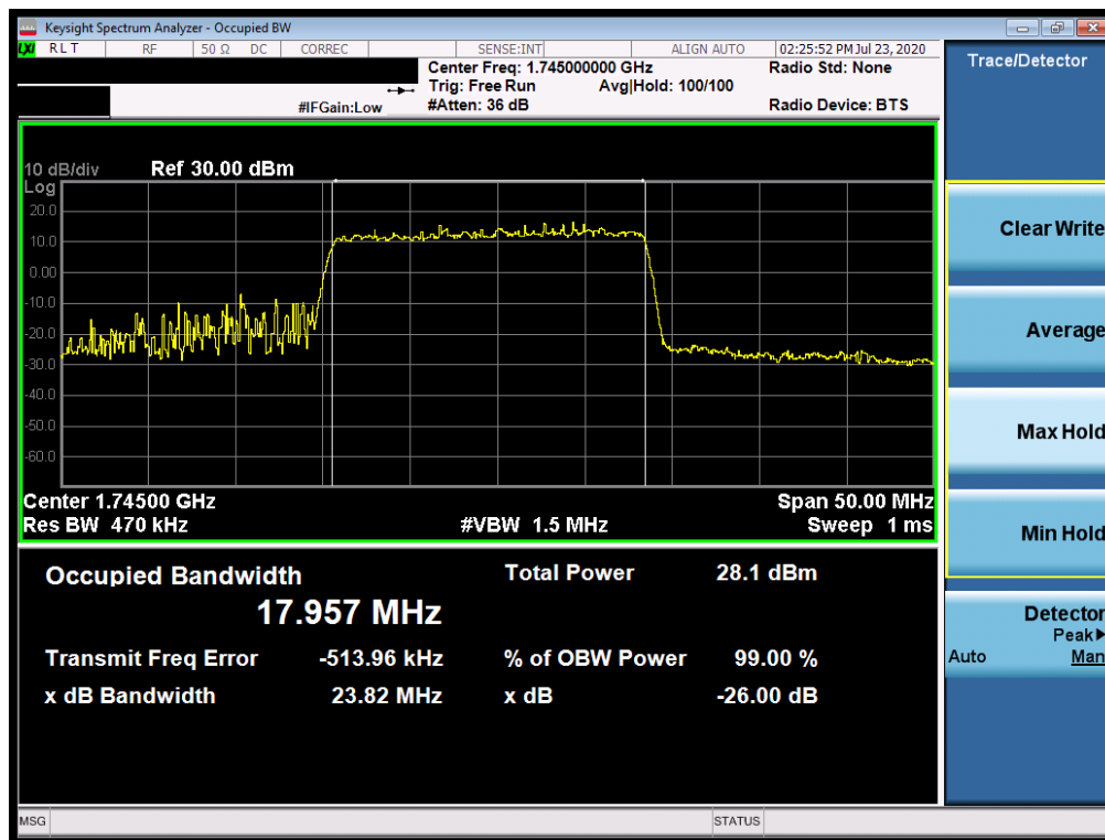
Plot 7-88. Occupied Bandwidth Plot (NR Band n66 - 20.0MHz CP-OFDM 256QAM - Full RB)
