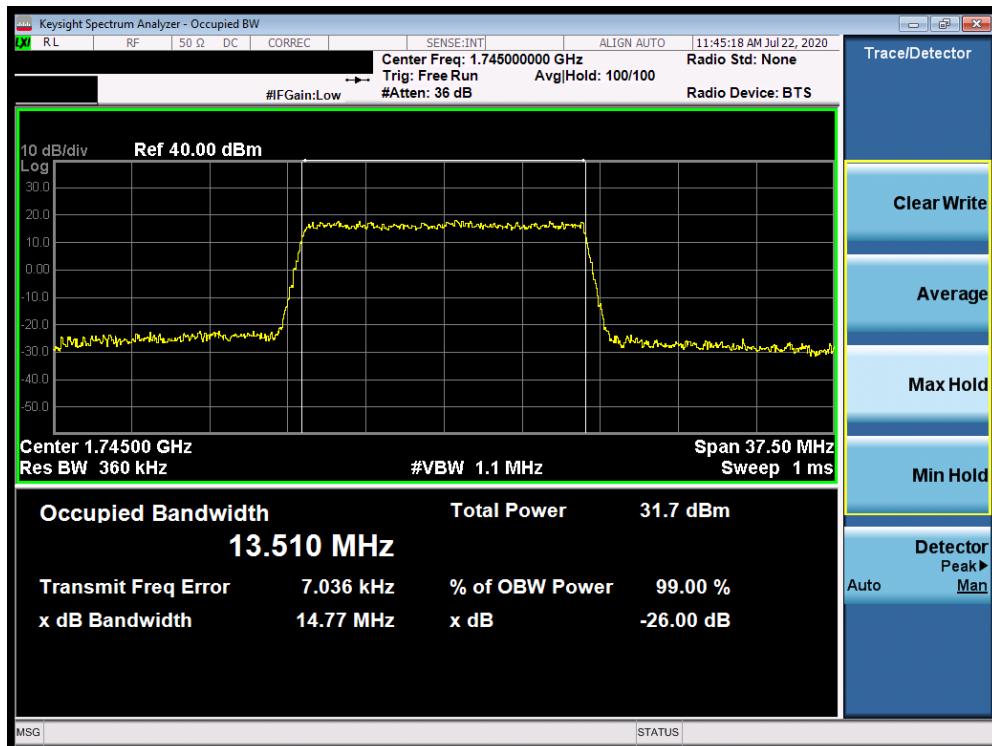
Plot 7-64. Occupied Bandwidth Plot (Band 66/4 - 15.0MHz 16-QAM - Full RB Configuration)
