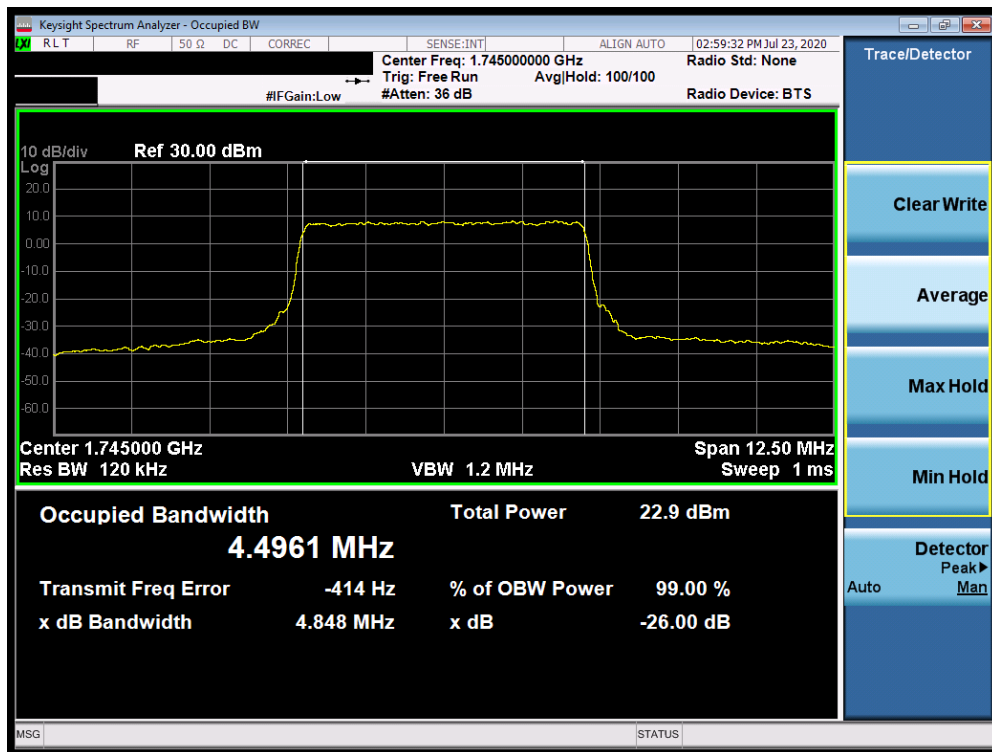
Plot 7-72. Occupied Bandwidth Plot (NR Band n66 - 5.0MHz CP-OFDM 64QAM - Full RB)
