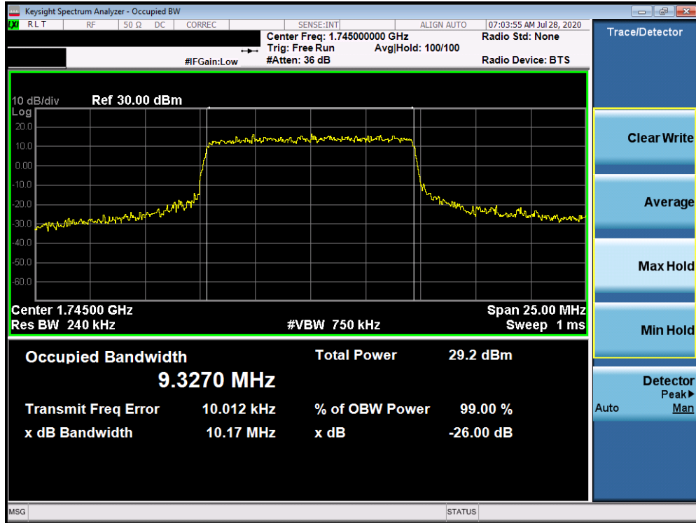
Plot 7-77. Occupied Bandwidth Plot (NR Band n66 - 10.0MHz CP-OFDM 64QAM - Full RB)
