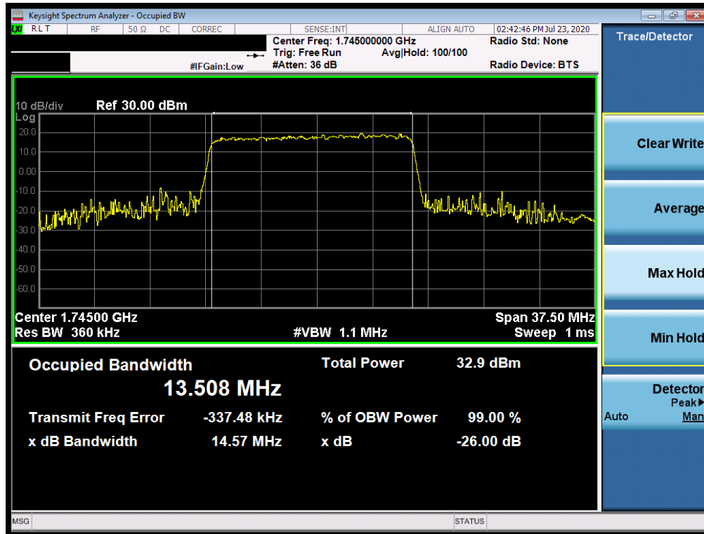
Plot 7-79. Occupied Bandwidth Plot (NR Band n66 - 15.0MHz DFT-s-OFDM BPSK - Full RB)
