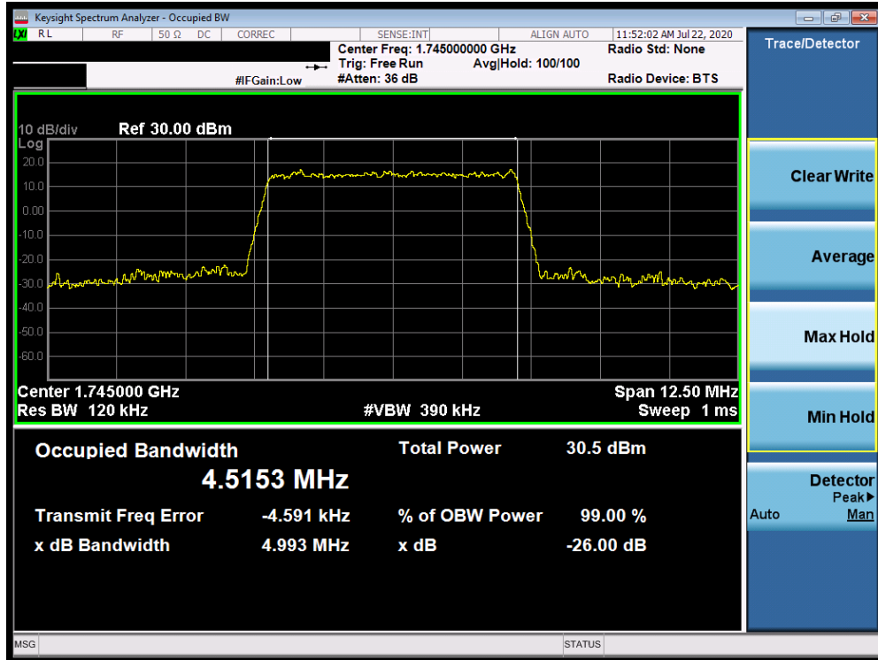
Plot 7-59. Occupied Bandwidth Plot (Band 66/4 - 5.0MHz 64-QAM - Full RB Configuration)
