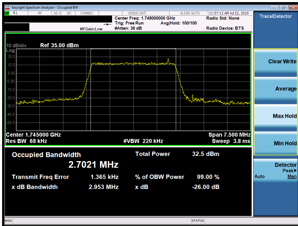
Plot 7-54. Occupied Bandwidth Plot (Band 66/4 - 3.0MHz QPSK - Full RB Configuration)
