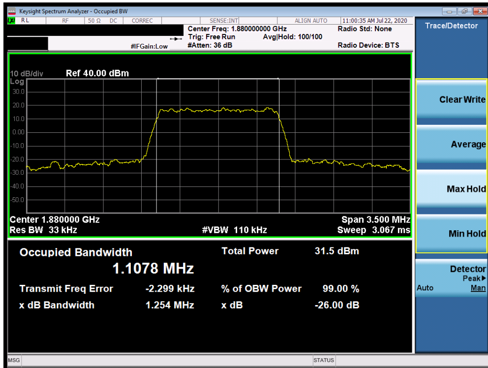
Plot 7-90. Occupied Bandwidth Plot (Band 2 - 1.4.0MHz 16-QAM - Full RB Configuration)
