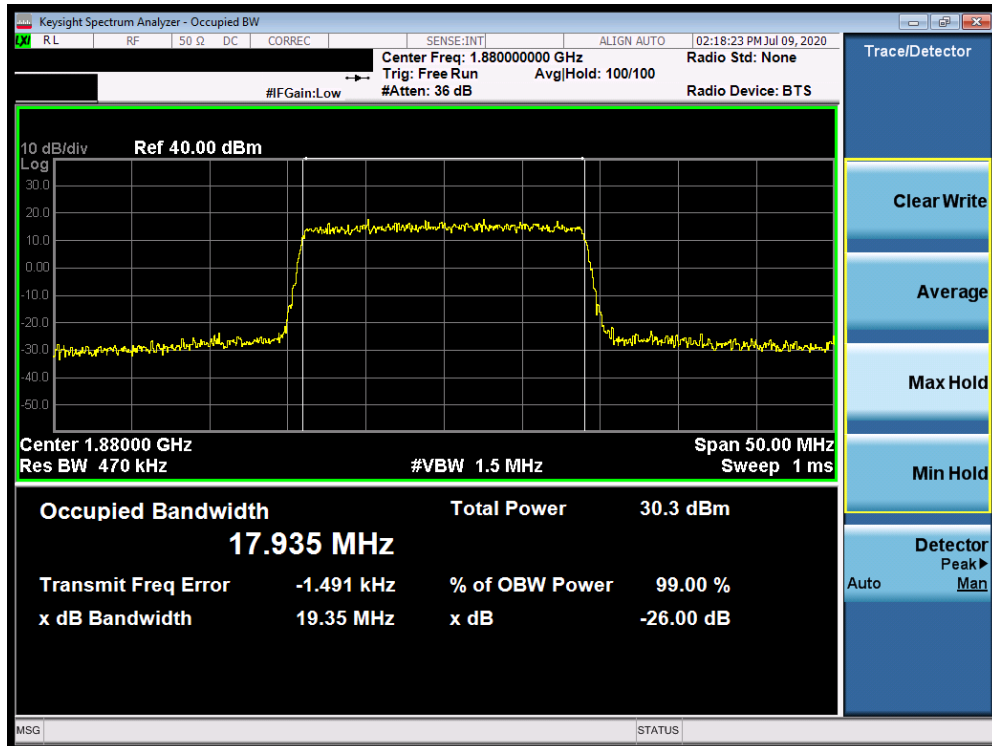
Plot 7-106. Occupied Bandwidth Plot (Band 2 - 20.0MHz 64-QAM - Full RB Configuration)
