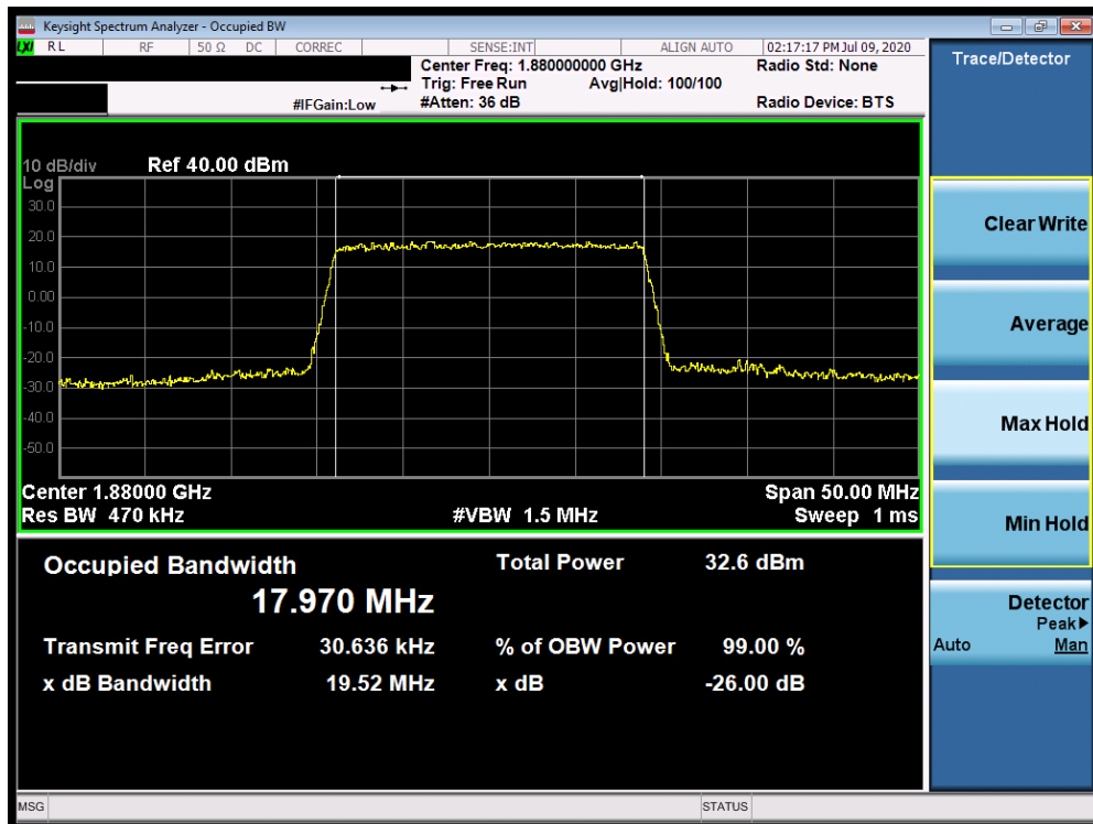
Plot 7-104. Occupied Bandwidth Plot (Band 2 - 20.0MHz QPSK - Full RB Configuration)
