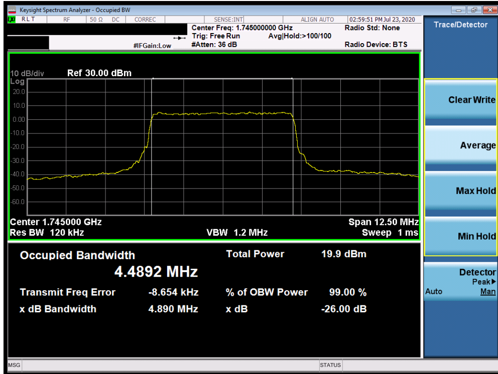
Plot 7-73. Occupied Bandwidth Plot (NR Band n66 - 5.0MHz CP-OFDM 256QAM - Full RB)
