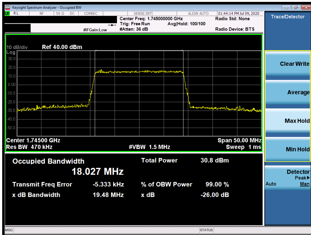
Plot 7-68. Occupied Bandwidth Plot (Band 66/4 - 20.0MHz 64-QAM - Full RB Configuration)
