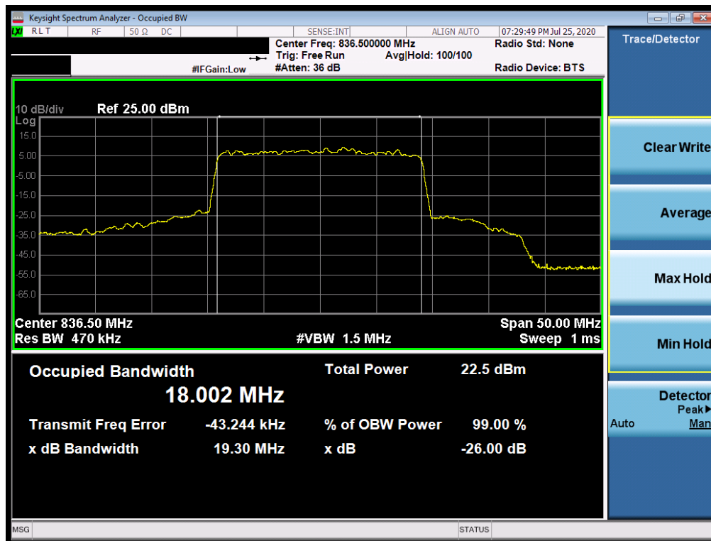
Plot 7-46. Occupied Bandwidth Plot (NR Band n5 - 20.0MHz DFT-s-OFDM BPSK - Full RB)
