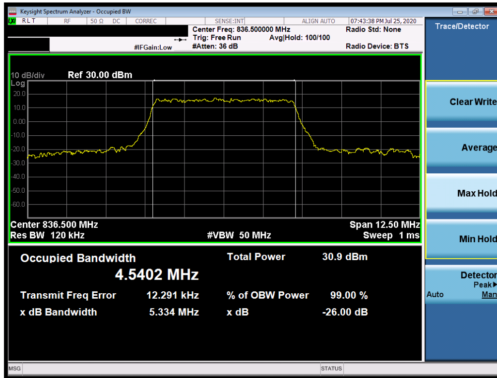
Plot 7-33. Occupied Bandwidth Plot (NR Band n5 - 5.0MHz CP-OFDM 16QAM - Full RB)
