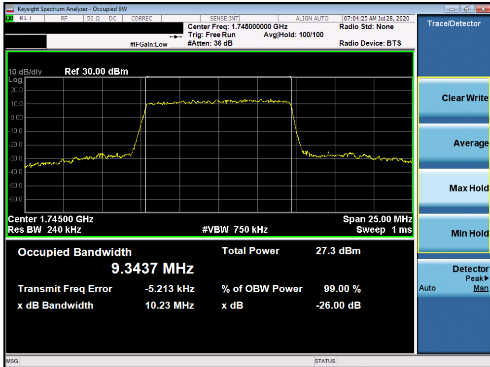
Plot 7-78. Occupied Bandwidth Plot (NR Band n66 - 10.0MHz CP-OFDM 256QAM - Full RB)
