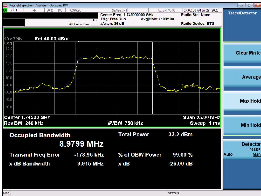
Plot 7-74. Occupied Bandwidth Plot (NR Band n66 - 10.0MHz DFT-s-OFDM BPSK - Full RB)
