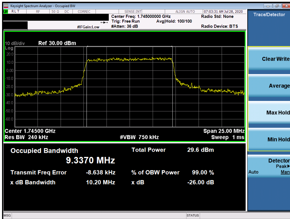
Plot 7-76. Occupied Bandwidth Plot (NR Band n66 - 10.0MHz CP-OFDM 16QAM - Full RB)
