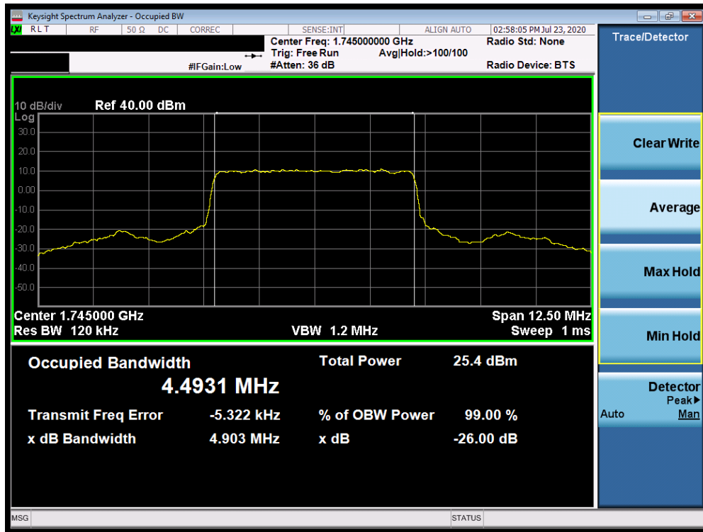
Plot 7-69. Occupied Bandwidth Plot (NR Band n66 - 5.0MHz DFT-s-OFDM BPSK - Full RB)
