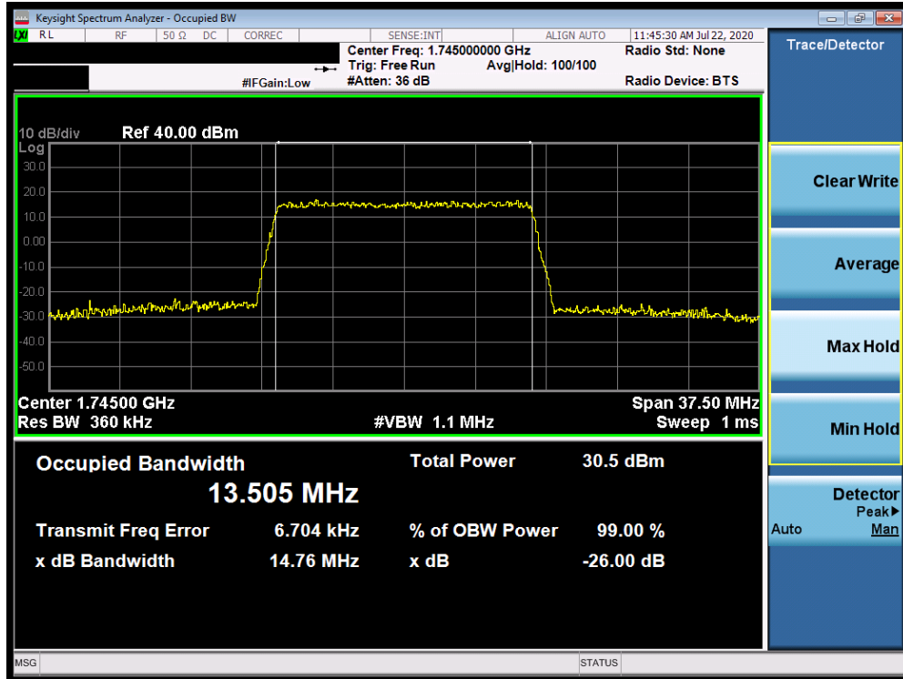
Plot 7-65. Occupied Bandwidth Plot (Band 66/4 - 15.0MHz 64-QAM - Full RB Configuration)
