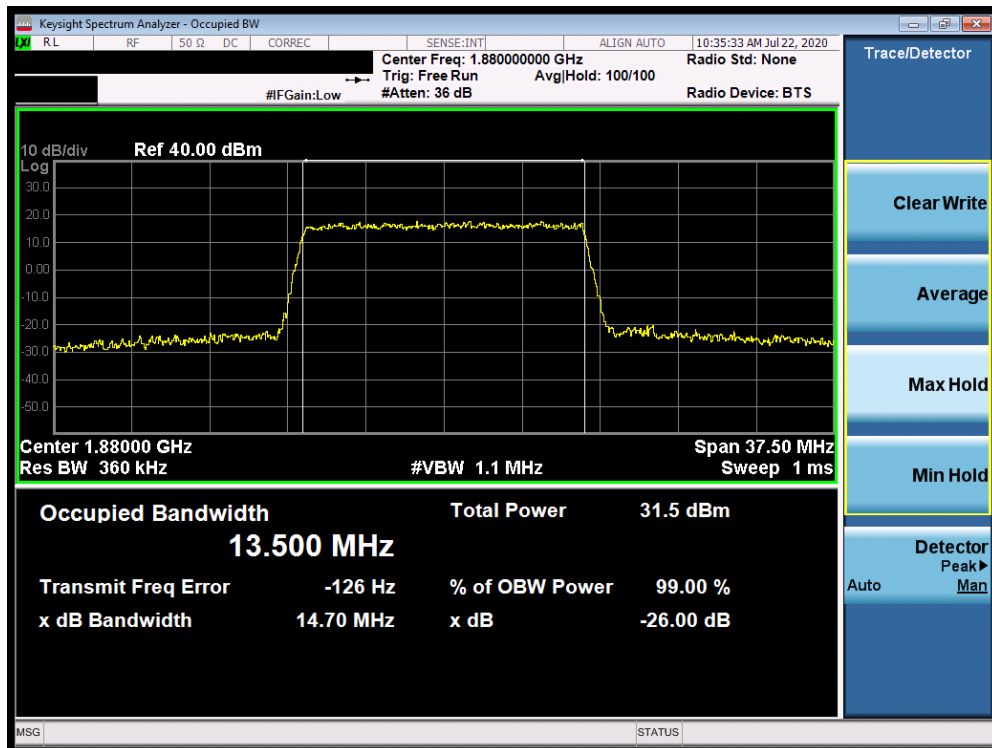
Plot 7-102. Occupied Bandwidth Plot (Band 2 - 15.0MHz 16-QAM - Full RB Configuration)
