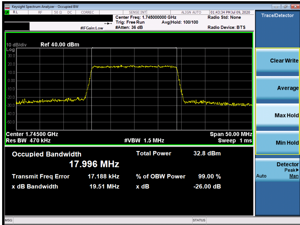
Plot 7-66. Occupied Bandwidth Plot (Band 66/4 - 20.0MHz QPSK - Full RB Configuration)
