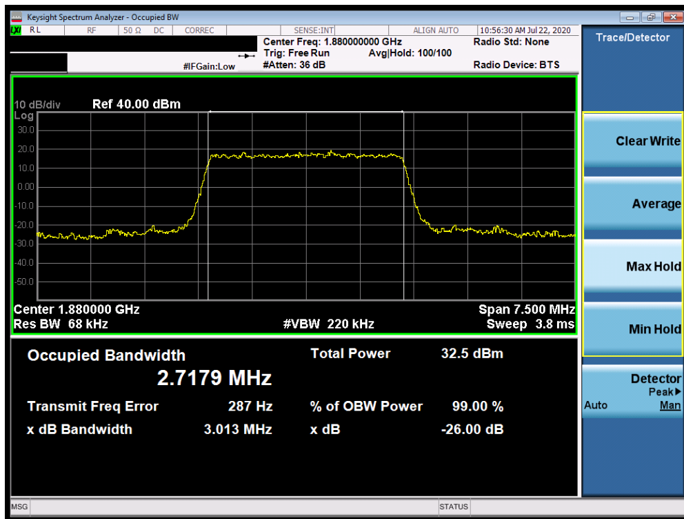
Plot 7-92. Occupied Bandwidth Plot (Band 2 - 3.0MHz QPSK - Full RB Configuration)
