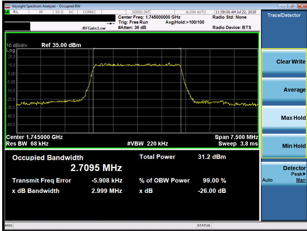
Plot 7-55. Occupied Bandwidth Plot (Band 66/4 - 3.0MHz 16-QAM - Full RB Configuration)
