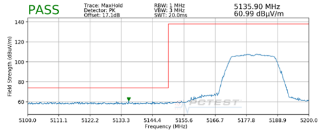
Plot 7-2. Radiated Lower Band Edge Plot SISO ANT1 (Peak – UNII Band 1)
