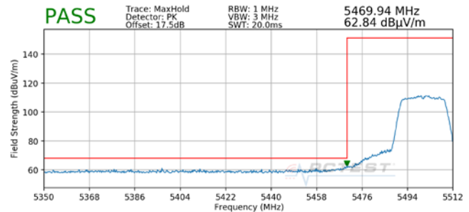
Plot 7-20. Radiated Lower Band Edge Plot MIMO (Peak – UNII Band 2C)
