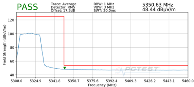
Plot 7-10. Radiated Upper Band Edge Plot SISO ANT2 (Average – UNII Band 2A)
