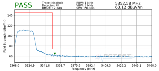
Plot 7-18. Radiated Upper Band Edge Plot MIMO (Peak – UNII Band 2A)
