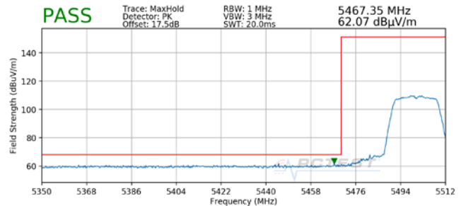
Plot 7-13. Radiated Lower Band Edge Plot SISO ANT2 (Peak – UNII Band 2C)
