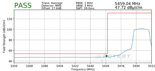
Plot 7-19. Radiated Lower Band Edge Plot MIMO (Average – UNII Band 2C)
