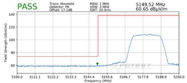
Plot 7-9. Radiated Lower Band Edge Plot SISO ANT2 (Peak – UNII Band 1)
