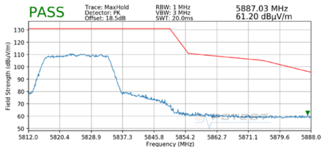
Plot 7-21. Radiated Upper Band Edge Plot MIMO (Peak – UNII Band 3)
