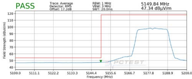
Plot 7-1. Radiated Lower Band Edge Plot SISO ANT1 (Average – UNII Band 1)
