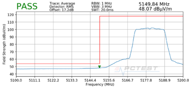
Plot 7-15. Radiated Lower Band Edge Plot MIMO (Average – UNII Band 1)
