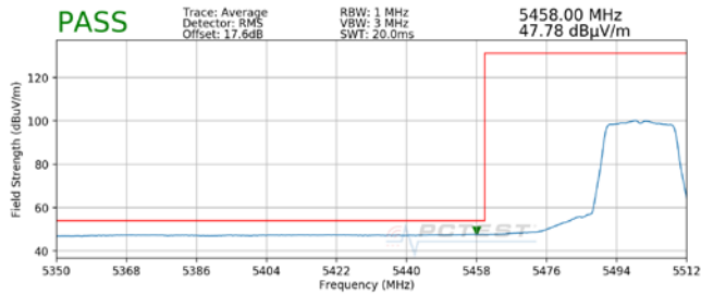
Plot 7-12. Radiated Lower Band Edge Plot SISO ANT2 (Average – UNII Band 2C)
