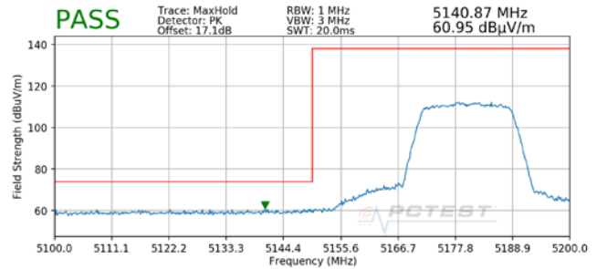
Plot 7-16. Radiated Lower Band Edge Plot MIMO (Peak – UNII Band 1)
