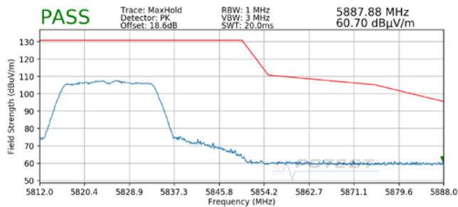
Plot 7-14. Radiated Upper Band Edge Plot SISO ANT2 (Peak – UNII Band 3)
