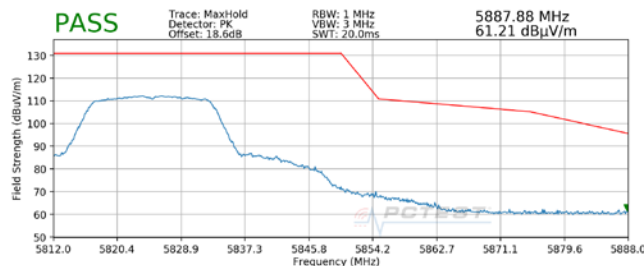
Plot 7-7. Radiated Upper Band Edge Plot SISO ANT1 (Peak - UNII Band 3)
