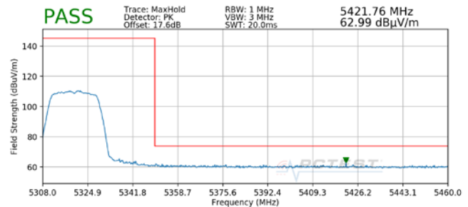
Plot 7-11. Radiated Upper Band Edge Plot SISO ANT2 (Peak – UNII Band 2A)
