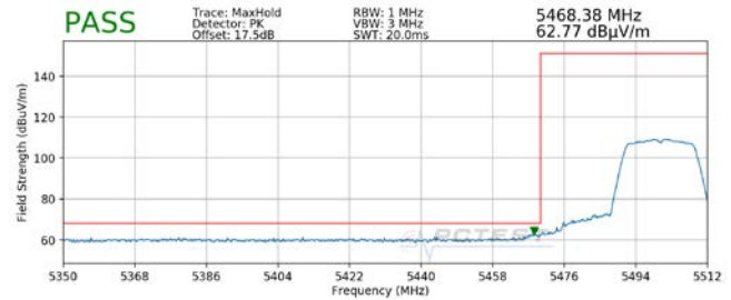
Plot 7-6. Radiated Lower Band Edge Plot SISO ANT1 (Peak - UNII Band 2C)
