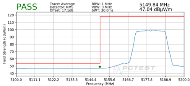
Plot 7-8. Radiated Lower Band Edge Plot SISO ANT2 (Average – UNII Band 1)
