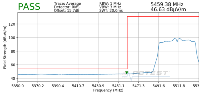
Plot 7-205. Radiated Lower Band Edge Plot SISO ANT2 (Average – UNII Band 2C)
