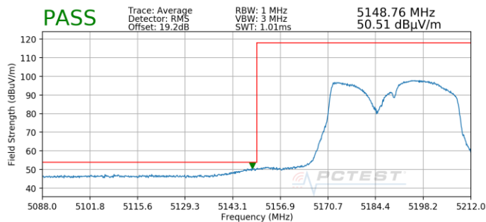
Plot 7-222. Radiated Lower Band Edge Plot MIMO (Average – UNII Band 1)
