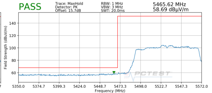
Plot 7-213. Radiated Lower Band Edge Plot SISO ANT2 (Peak – UNII Band 2C)
