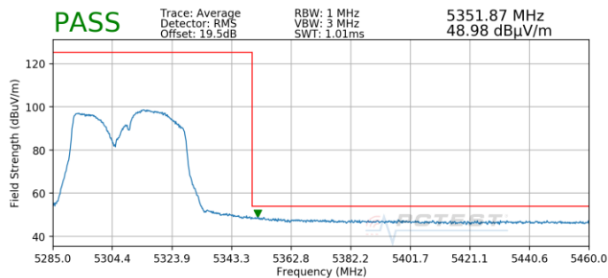
Plot 7-224. Radiated Upper Band Edge Plot MIMO (Average – UNII Band 2A)
