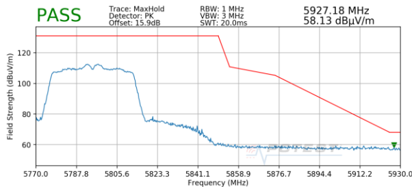
Plot 7-207. Radiated Upper Band Edge Plot SISO ANT2 (Peak – UNII Band 3)
