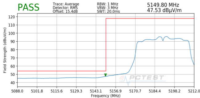
Plot 7-201. Radiated Lower Band Edge Plot SISO ANT2 (Average – UNII Band 1)
