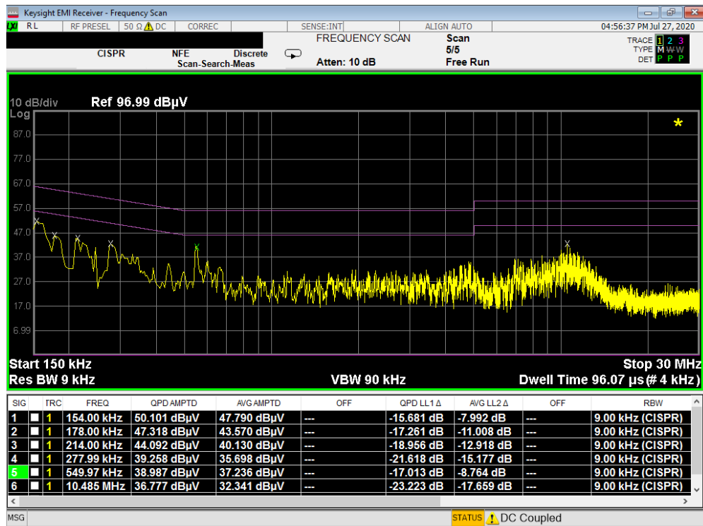
Plot 7-239. Line Conducted Plot with 802.11a UNII Band 1 (N)
