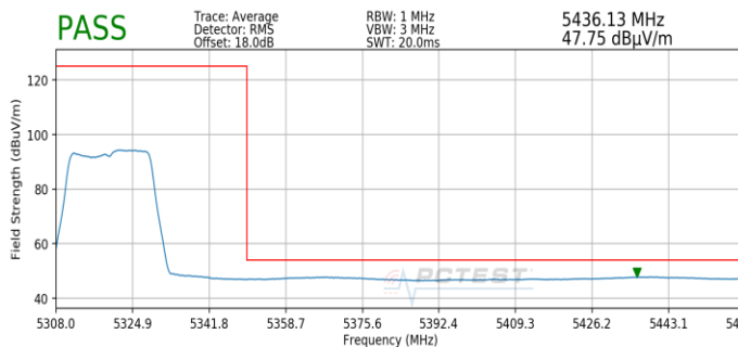
Plot 7-217. Radiated Upper Band Edge Plot MIMO (Average – UNII Band 2A)
