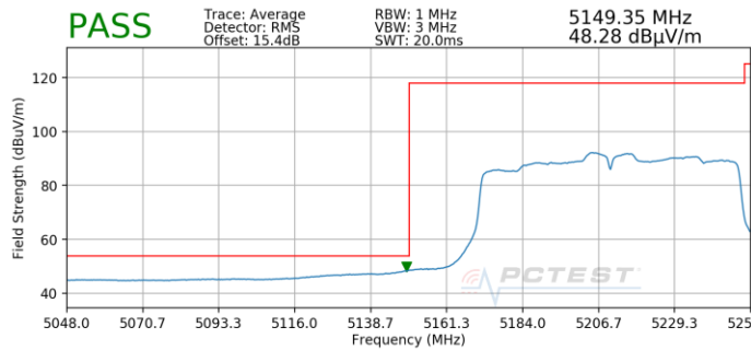
Plot 7-208. Radiated Lower Band Edge Plot SISO ANT2 (Average – UNII Band 1)
