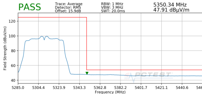
Plot 7-203. Radiated Upper Band Edge Plot SISO ANT2 (Average – UNII Band 2A)
