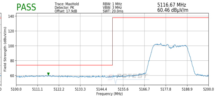
Plot 7-216. Radiated Lower Band Edge Plot MIMO (Peak – UNII Band 1)
