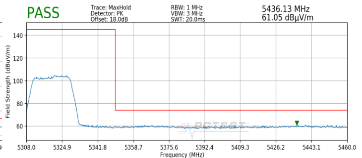
Plot 7-218. Radiated Upper Band Edge Plot MIMO (Peak – UNII Band 2A)
