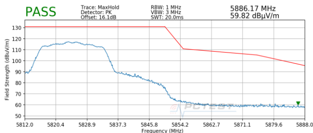
Plot 7-200. Radiated Upper Band Edge Plot SISO ANT2 (Peak – UNII Band 3)
