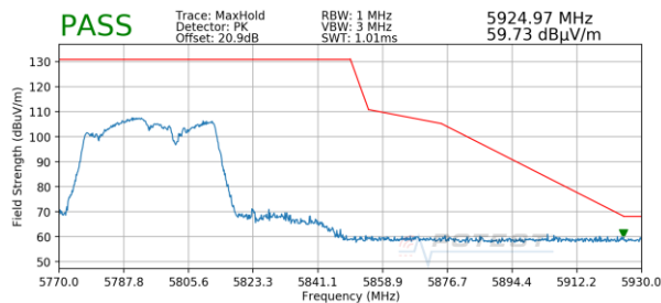
Plot 7-228. Radiated Upper Band Edge Plot MIMO (Peak – UNII Band 3)
