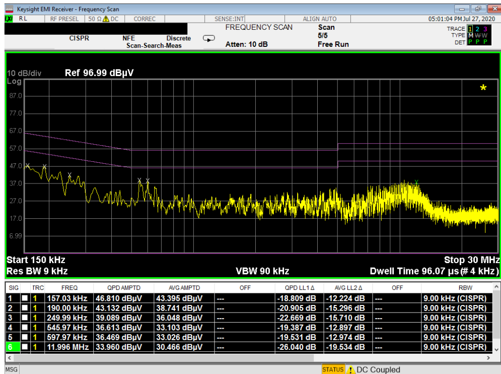
Plot 7-241. Line Conducted Plot with 802.11a UNII Band 2A (N)
