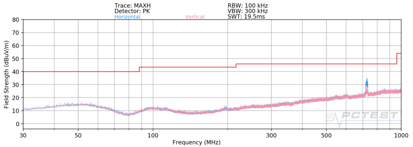
Plot 7-237. Radiated Spurious Plot below 1GHz (2.4GHz – 5GHz)
