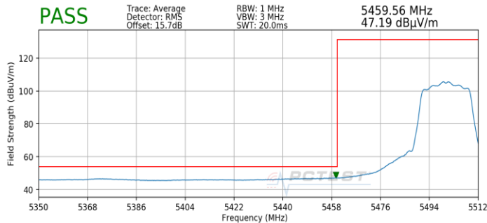
Plot 7-198. Radiated Lower Band Edge Plot SISO ANT2 (Average – UNII Band 2C)
