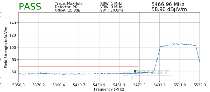
Plot 7-206. Radiated Lower Band Edge Plot SISO ANT2 (Peak – UNII Band 2C)
