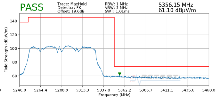
Plot 7-232. Radiated Upper Band Edge Plot MIMO (Peak – UNII Band 2A)
