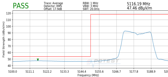
Plot 7-215. Radiated Lower Band Edge Plot MIMO (Average – UNII Band 1)
