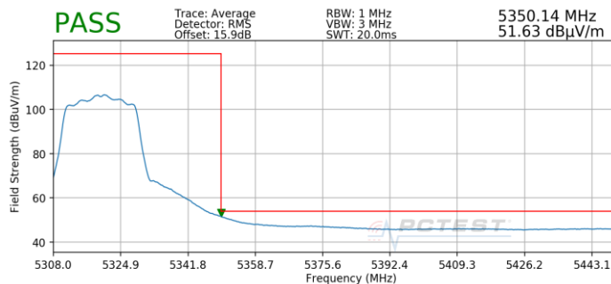
Plot 7-196. Radiated Upper Band Edge Plot SISO ANT2 (Average – UNII Band 2A)
