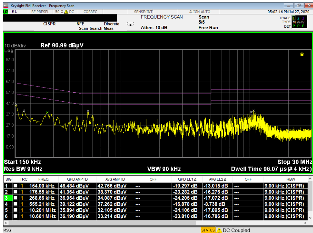
Plot 7-243. Line Conducted Plot with 802.11a UNII Band 2C (N)
