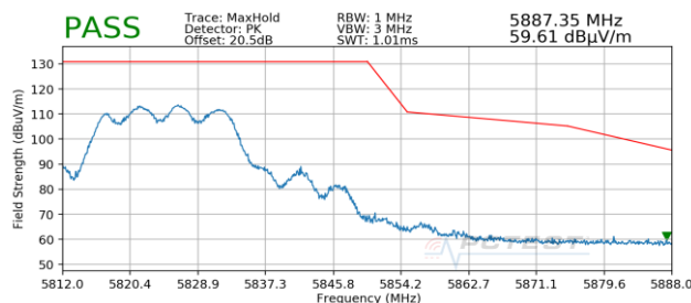
Plot 7-221. Radiated Upper Band Edge Plot MIMO (Peak – UNII Band 3)
