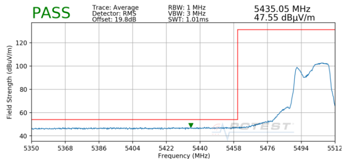
Plot 7-219. Radiated Lower Band Edge Plot MIMO (Average – UNII Band 2C)
