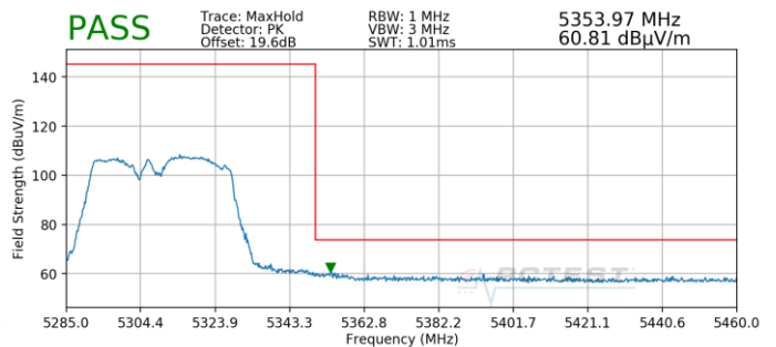
Plot 7-225. Radiated Upper Band Edge Plot MIMO (Peak – UNII Band 2A)
