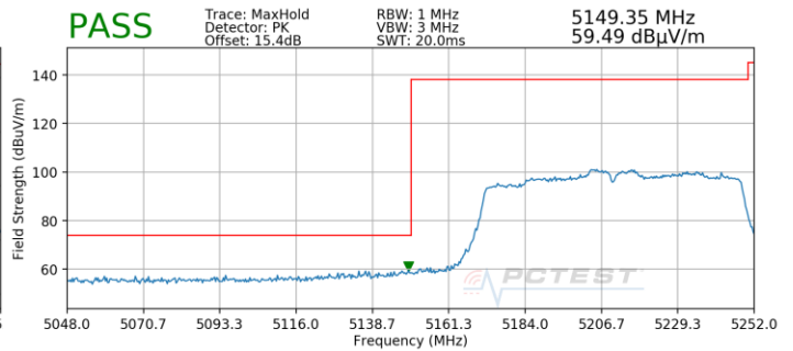
Plot 7-209. Radiated Lower Band Edge Plot SISO ANT2 (Peak – UNII Band 1)
