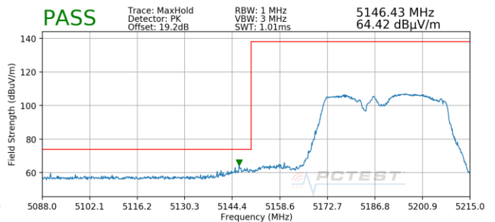
Plot 7-223. Radiated Lower Band Edge Plot MIMO (Peak – UNII Band 1)
