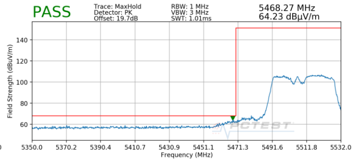
Plot 7-227. Radiated Lower Band Edge Plot MIMO (Peak – UNII Band 2C)
