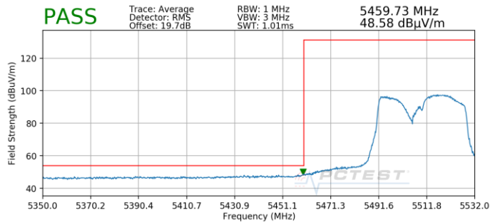
Plot 7-226. Radiated Lower Band Edge Plot MIMO (Average – UNII Band 2C)
