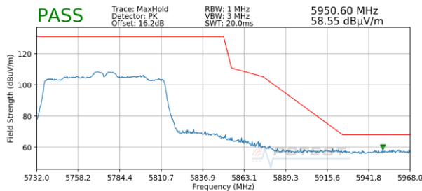
Plot 7-214. Radiated Upper Band Edge Plot SISO ANT2 (Peak – UNII Band 3)
