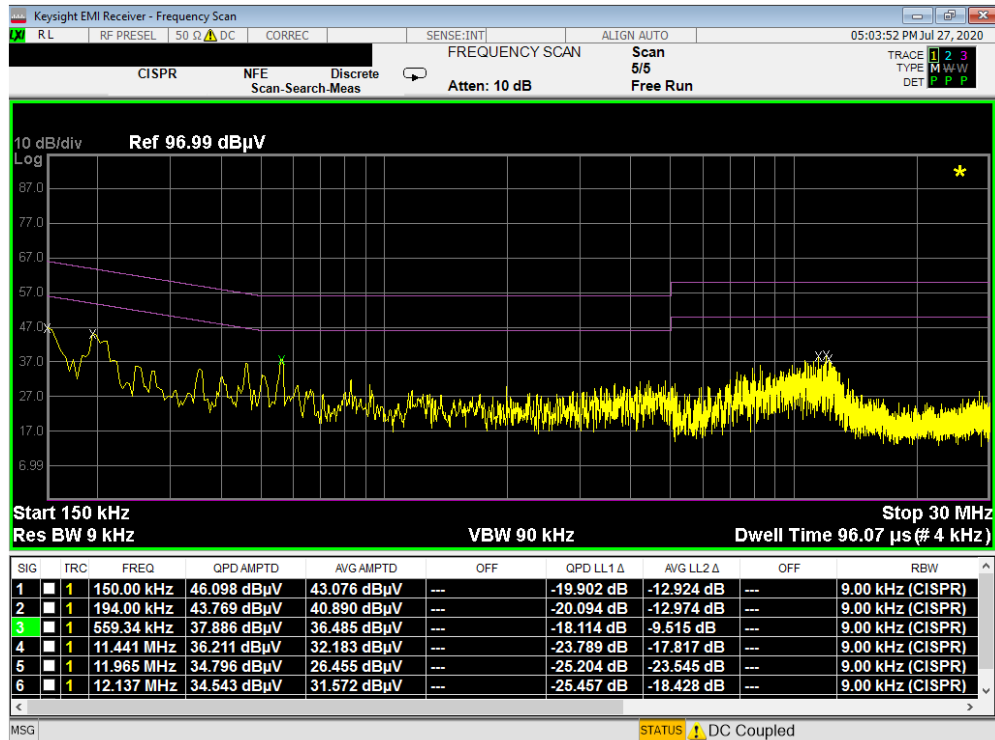
Plot 7-242. Line Conducted Plot with 802.11a UNII Band 2C (L1)
