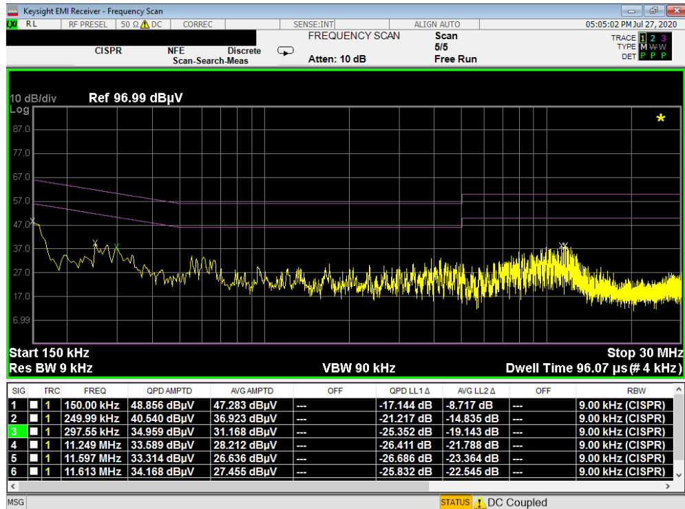
Plot 7-244. Line Conducted Plot with 802.11a UNII Band 3 (L1)
