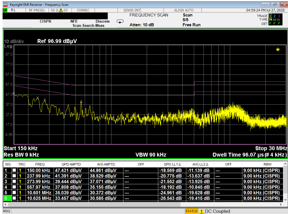
Plot 7-240. Line Conducted Plot with 802.11a UNII Band 2A (L1)
