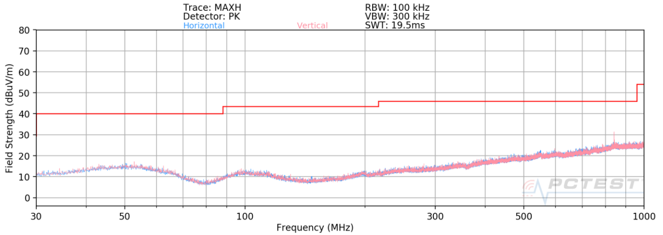
Plot 7-236. Radiated Spurious Plot below 18GHz MIMO
