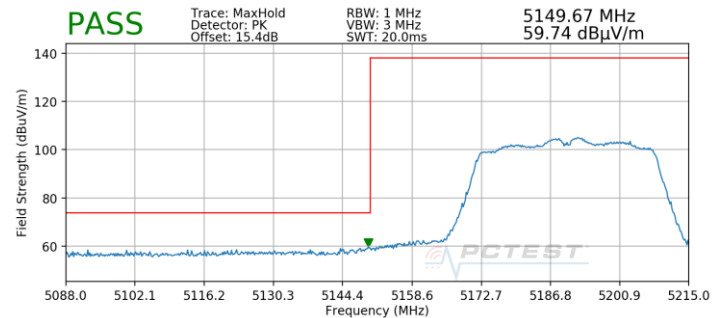
Plot 7-202. Radiated Lower Band Edge Plot SISO ANT2 (Peak – UNII Band 1)
