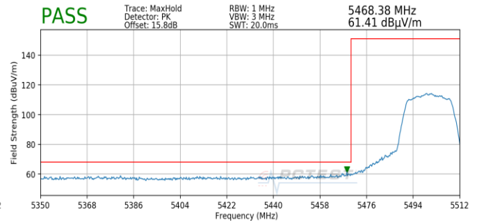
Plot 7-199. Radiated Lower Band Edge Plot SISO ANT2 (Peak – UNII Band 2C)
