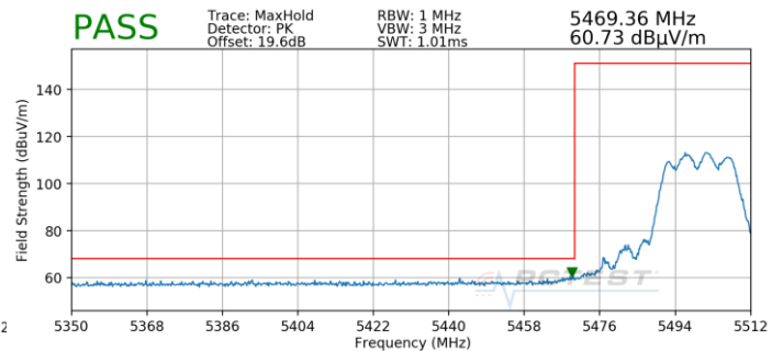
Plot 7-220. Radiated Lower Band Edge Plot MIMO (Peak – UNII Band 2C)
