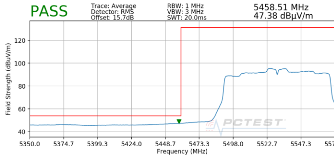
Plot 7-212. Radiated Lower Band Edge Plot SISO ANT2 (Average – UNII Band 2C)
