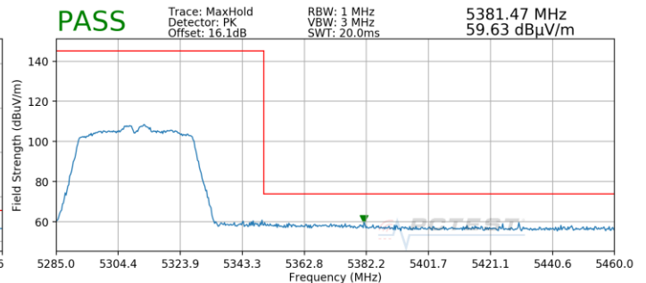
Plot 7-204. Radiated Upper Band Edge Plot SISO ANT2 (Peak – UNII Band 2A)
