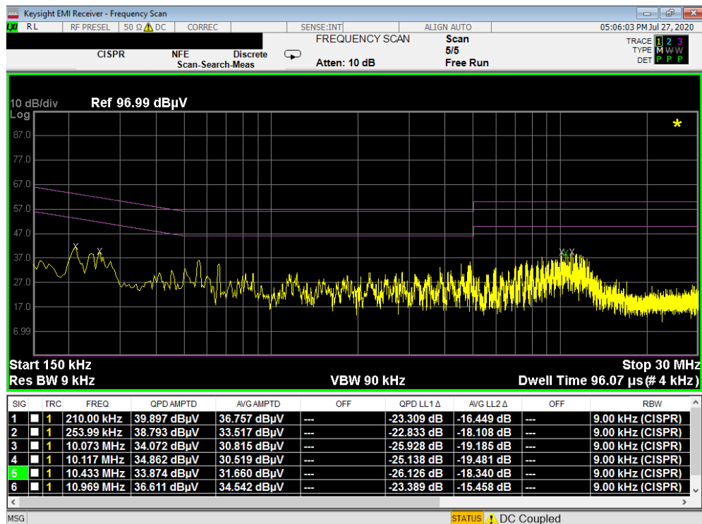
Plot 7-245. Line Conducted Plot with 802.11a UNII Band 3 (N)
