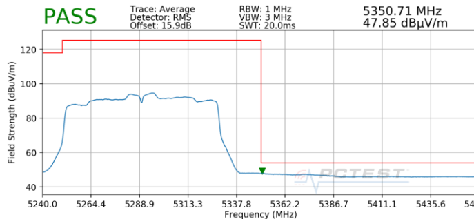
Plot 7-210. Radiated Upper Band Edge Plot SISO ANT2 (Average – UNII Band 2A)
