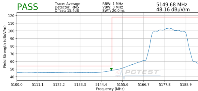
Plot 7-194. Radiated Lower Band Edge Plot SISO ANT2 (Average – UNII Band 1)
