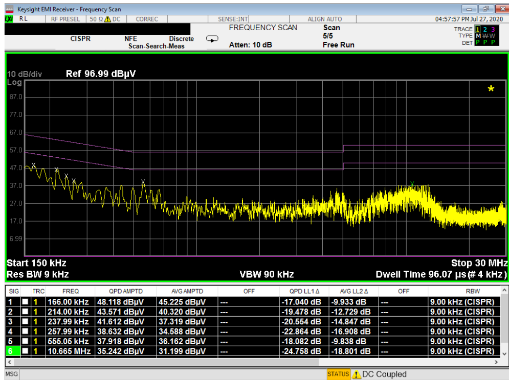
Plot 7-238. Line Conducted Plot with 802.11a UNII Band 1 (L1)
