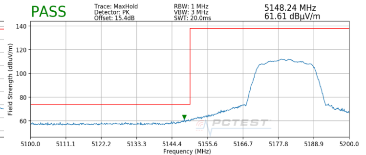
Plot 7-195. Radiated Lower Band Edge Plot SISO ANT2 (Peak – UNII Band 1)
