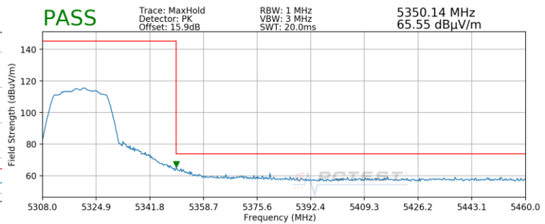
Plot 7-197. Radiated Upper Band Edge Plot SISO ANT2 (Peak – UNII Band 2A)
