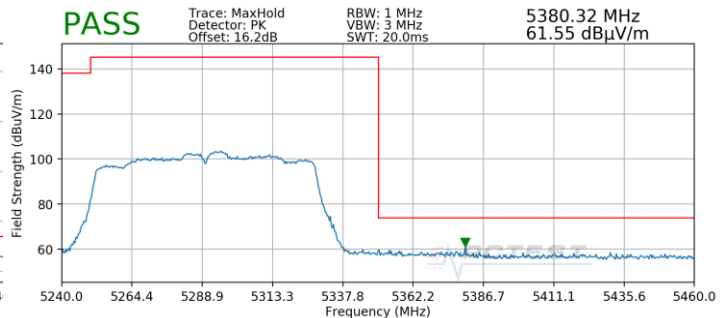
Plot 7-211. Radiated Upper Band Edge Plot SISO ANT2 (Peak – UNII Band 2A)
