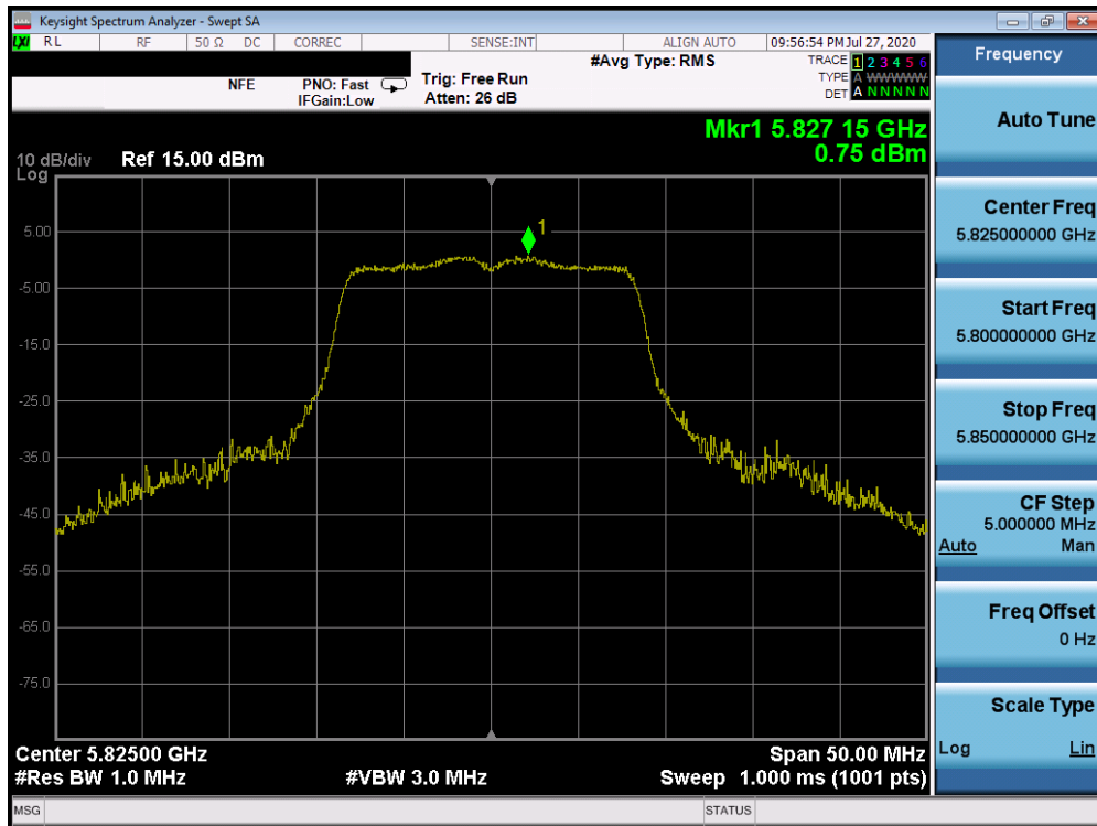
Plot 7-150. Power Spectral Density Plot SISO ANT1 (802.11a (UNII Band 3) – Ch. 165)
