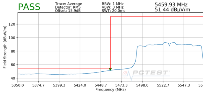
Plot 7-191. Radiated Lower Band Edge Plot SISO ANT1 (Average – UNII Band 2C)
