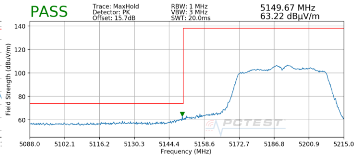
Plot 7-181. Radiated Lower Band Edge Plot SISO ANT1 (Peak – UNII Band 1)
