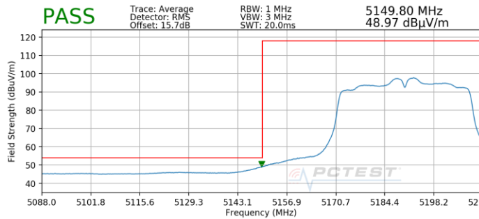
Plot 7-180. Radiated Lower Band Edge Plot SISO ANT1 (Average – UNII Band 1)
