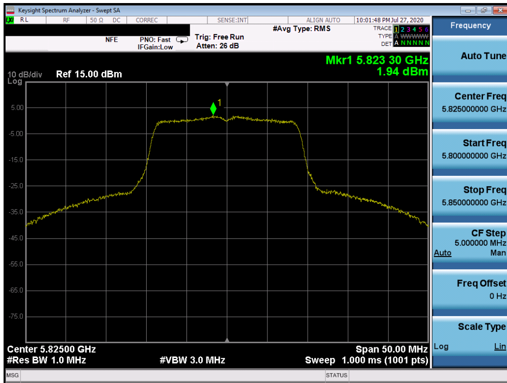
Plot 7-153. Power Spectral Density Plot SISO ANT1 (20MHz BW 802.11n (UNII Band 3) – Ch. 165)
