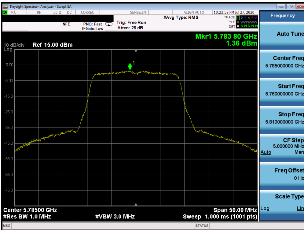
Plot 7-113. Power Spectral Density Plot SISO ANT2 (20MHz BW 802.11n (UNII Band 3) – Ch. 157)
