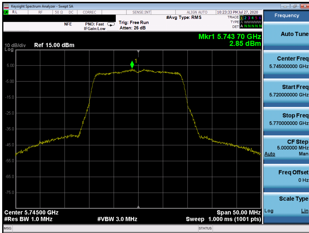
Plot 7-112. Power Spectral Density Plot SISO ANT2 (20MHz BW 802.11n (UNII Band 3) – Ch. 149)
