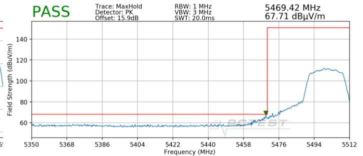
Plot 7-178. Radiated Lower Band Edge Plot SISO ANT1 (Peak – UNII Band 2C)
