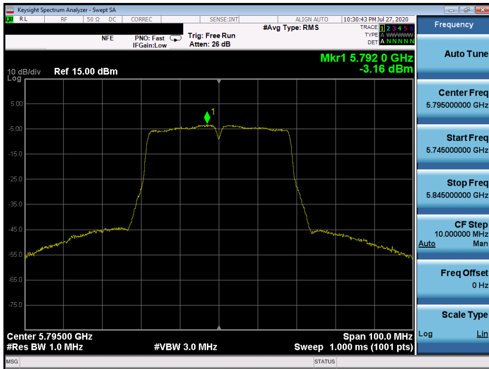
Plot 7-116. Power Spectral Density Plot SISO ANT2 (40MHz BW 802.11n (UNII Band 3) – Ch. 159)
