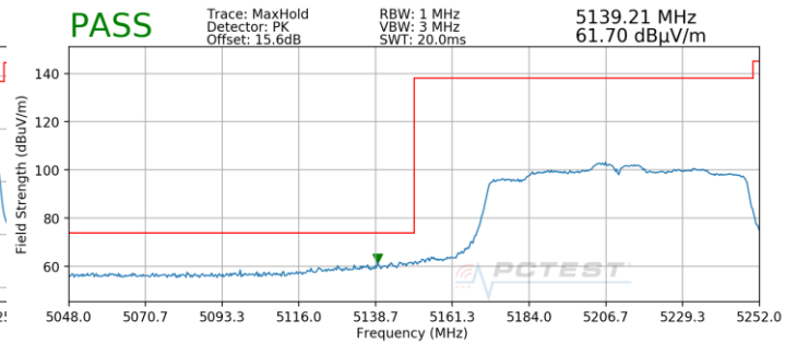
Plot 7-188. Radiated Lower Band Edge Plot SISO ANT1 (Peak – UNII Band 1)
