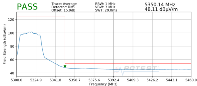
Plot 7-175. Radiated Upper Band Edge Plot SISO ANT1 (Average – UNII Band 2A)
