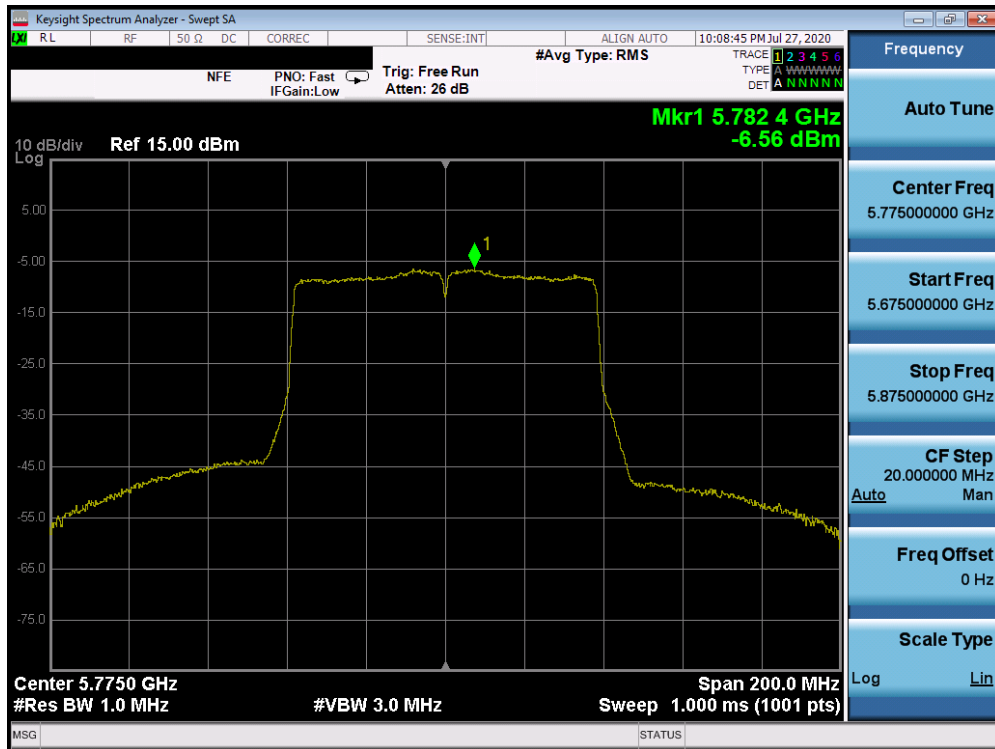
Plot 7-156. Power Spectral Density Plot SISO ANT1 (80MHz BW 802.11ac (UNII Band 3) – Ch. 155)
