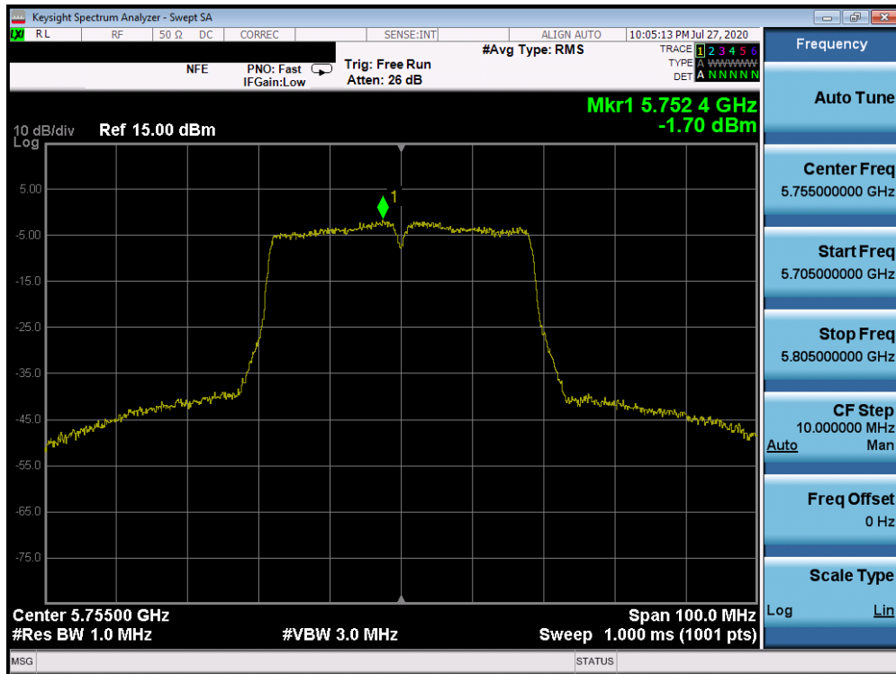
Plot 7-154. Power Spectral Density Plot SISO ANT1 (40MHz BW 802.11n (UNII Band 3) – Ch. 151)
