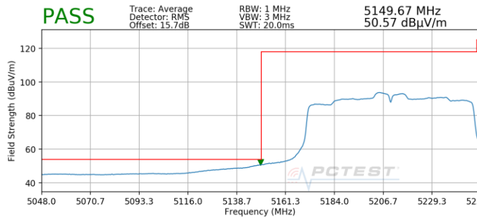
Plot 7-187. Radiated Lower Band Edge Plot SISO ANT1 (Average – UNII Band 1)
