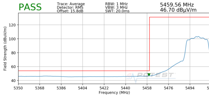
Plot 7-177. Radiated Lower Band Edge Plot SISO ANT1 (Average – UNII Band 2C)
