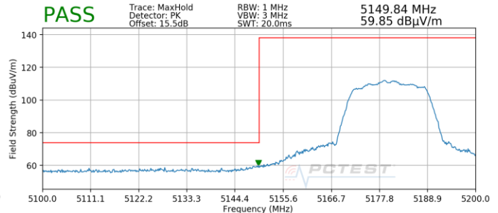
Plot 7-174. Radiated Lower Band Edge Plot SISO ANT1 (Peak – UNII Band 1)
