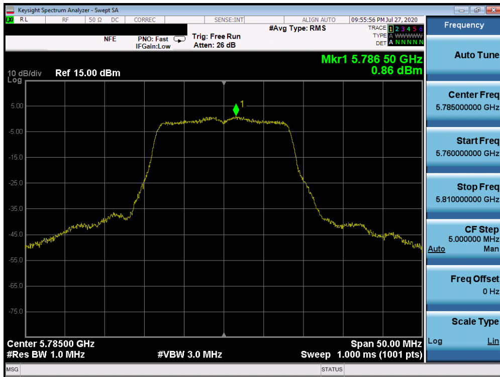
Plot 7-149. Power Spectral Density Plot SISO ANT1 (802.11a (UNII Band 3) – Ch. 157)
