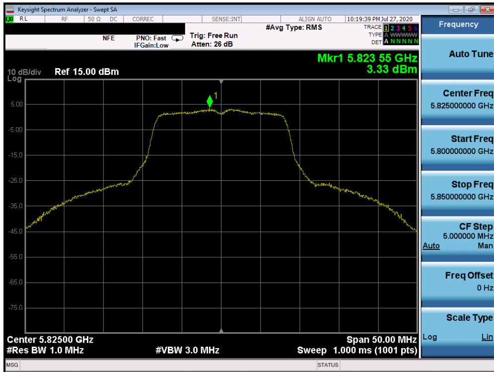
Plot 7-111. Power Spectral Density Plot SISO ANT2 (802.11a (UNII Band 3) – Ch. 165)
