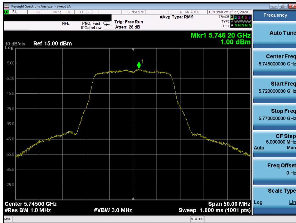
Plot 7-109. Power Spectral Density Plot SISO ANT2 (802.11a (UNII Band 3) – Ch. 149)
