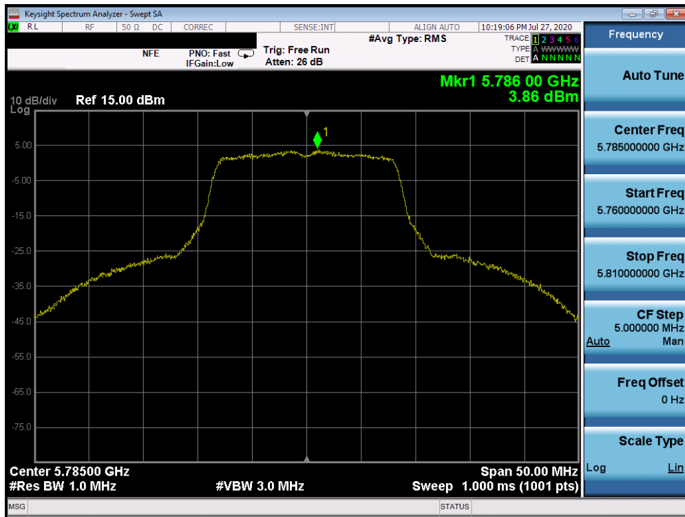
Plot 7-110. Power Spectral Density Plot SISO ANT2 (802.11a (UNII Band 3) – Ch. 157)
