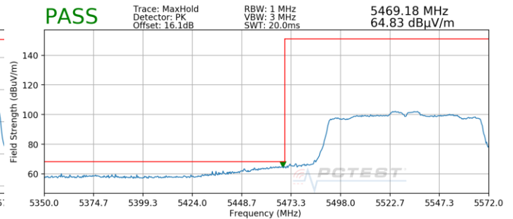
Plot 7-192. Radiated Lower Band Edge Plot SISO ANT1 (Peak – UNII Band 2C)
