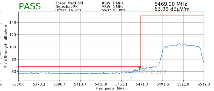
Plot 7-185. Radiated Lower Band Edge Plot SISO ANT1 (Peak – UNII Band 2C)
