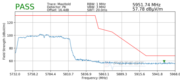
Plot 7-193. Radiated Upper Band Edge Plot SISO ANT1 (Peak – UNII Band 3)
