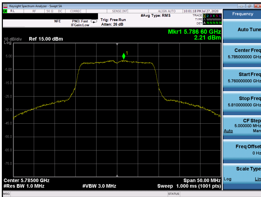
Plot 7-152. Power Spectral Density Plot SISO ANT1 (20MHz BW 802.11n (UNII Band 3) – Ch. 157)
