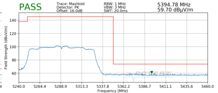
Plot 7-190. Radiated Upper Band Edge Plot SISO ANT1 (Peak – UNII Band 2A)
