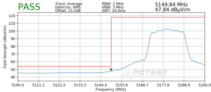
Plot 7-173. Radiated Lower Band Edge Plot SISO ANT1 (Average – UNII Band 1)
