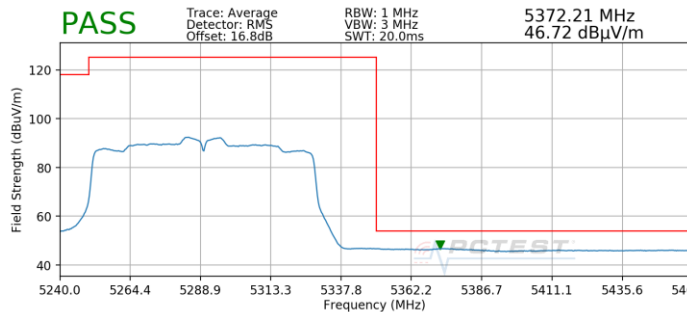
Plot 7-189. Radiated Upper Band Edge Plot SISO ANT1 (Average – UNII Band 2A)
