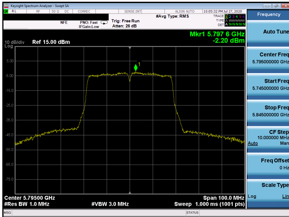
Plot 7-155. Power Spectral Density Plot SISO ANT1 (40MHz BW 802.11n (UNII Band 3) – Ch. 159)
