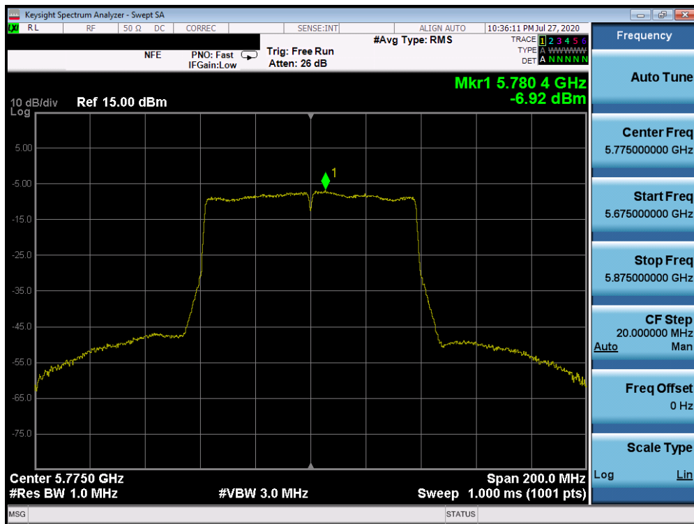
Plot 7-117. Power Spectral Density Plot SISO ANT2 (80MHz BW 802.11ac (UNII Band 3) – Ch. 155)
