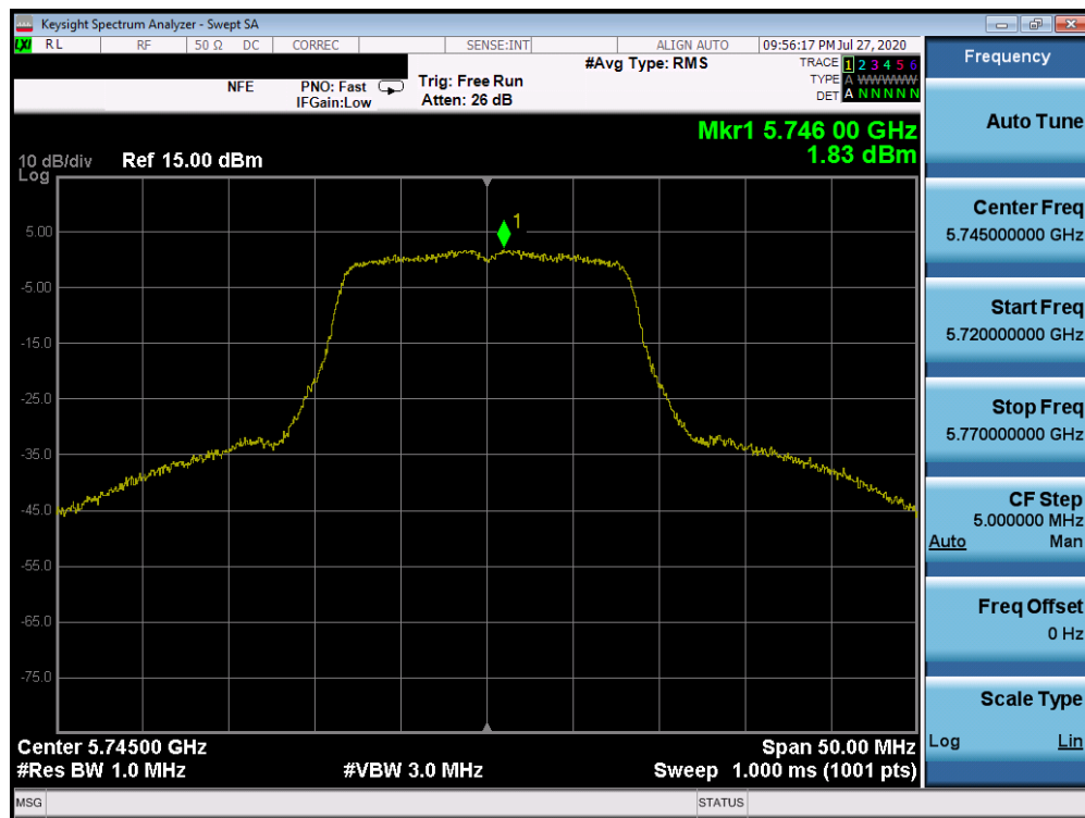
Plot 7-148. Power Spectral Density Plot SISO ANT1 (802.11a (UNII Band 3) – Ch. 149)
