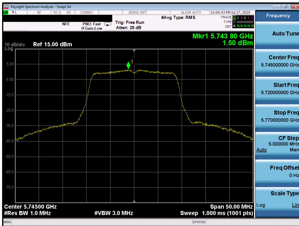
Plot 7-151. Power Spectral Density Plot SISO ANT1 (20MHz BW 802.11n (UNII Band 3) – Ch. 149)
