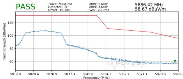
Plot 7-179. Radiated Upper Band Edge Plot SISO ANT1 (Peak – UNII Band 3)
