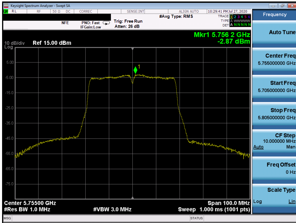
Plot 7-115. Power Spectral Density Plot SISO ANT2 (40MHz BW 802.11n (UNII Band 3) – Ch. 151)
