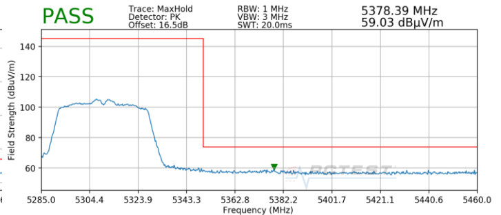
Plot 7-183. Radiated Upper Band Edge Plot SISO ANT1 (Peak – UNII Band 2A)
