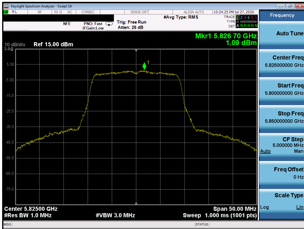
Plot 7-114. Power Spectral Density Plot SISO ANT2 (20MHz BW 802.11n (UNII Band 3) – Ch. 165)
