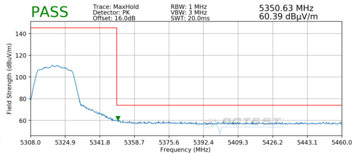
Plot 7-176. Radiated Upper Band Edge Plot SISO ANT1 (Peak – UNII Band 2A)
