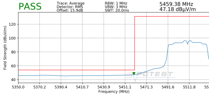
Plot 7-184. Radiated Lower Band Edge Plot SISO ANT1 (Average – UNII Band 2C)
