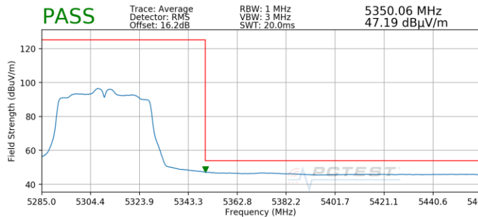
Plot 7-182. Radiated Upper Band Edge Plot SISO ANT1 (Average – UNII Band 2A)
