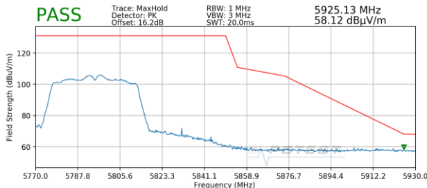
Plot 7-186. Radiated Upper Band Edge Plot SISO ANT1 (Peak – UNII Band 3)
