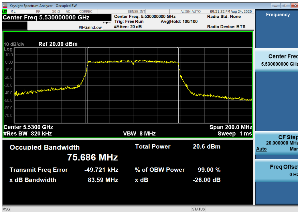
Plot 7-28. 26dB Bandwidth Plot SISO ANT1 (80MHz BW 802.11ac (UNII Band 2C) – Ch. 106)
