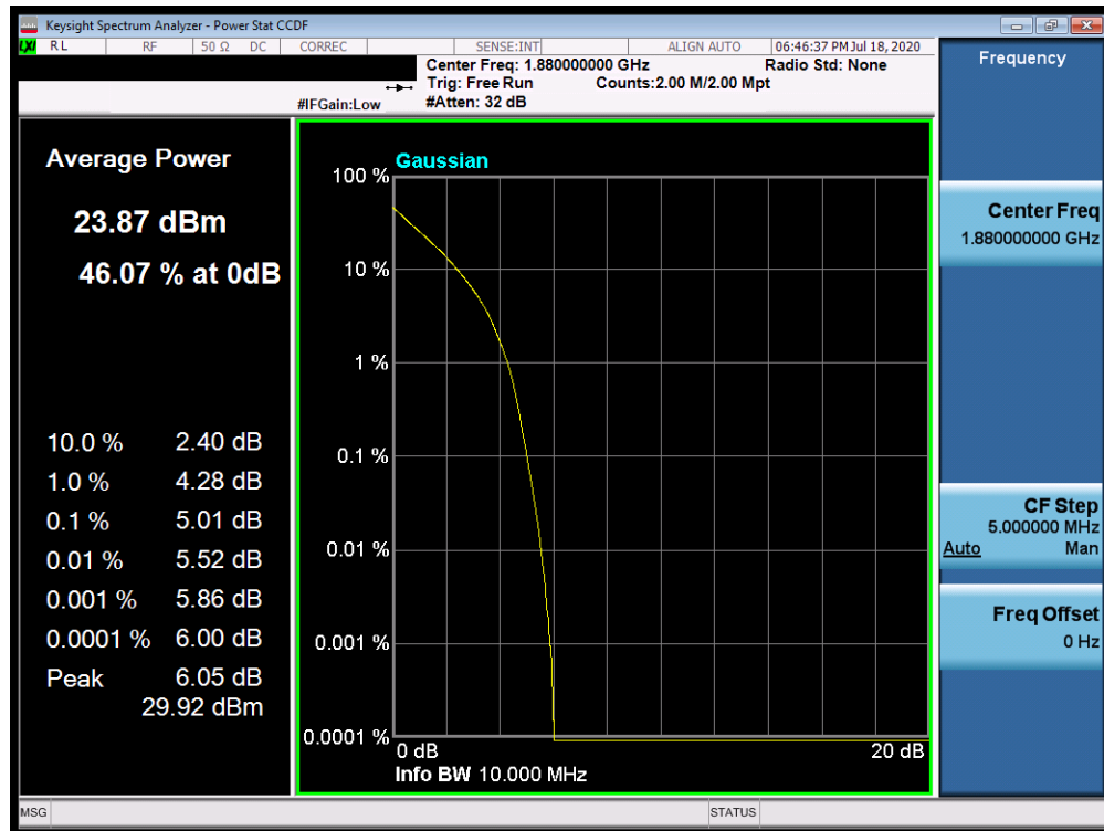
Plot 7-527. PAR Plot (Band 25/2 - 10.0MHz QPSK - Full RB Configuration)
