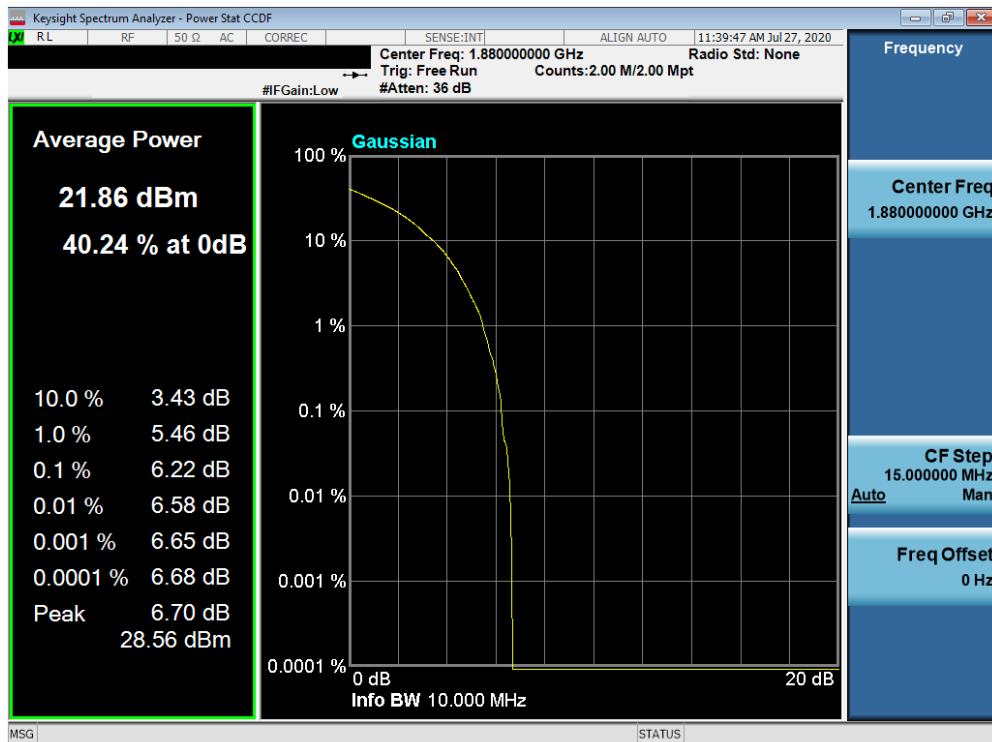
Plot 7-556. PAR Plot (NR n25/2 - 10.0MHz 16-QAM - Full RB Configuration)
