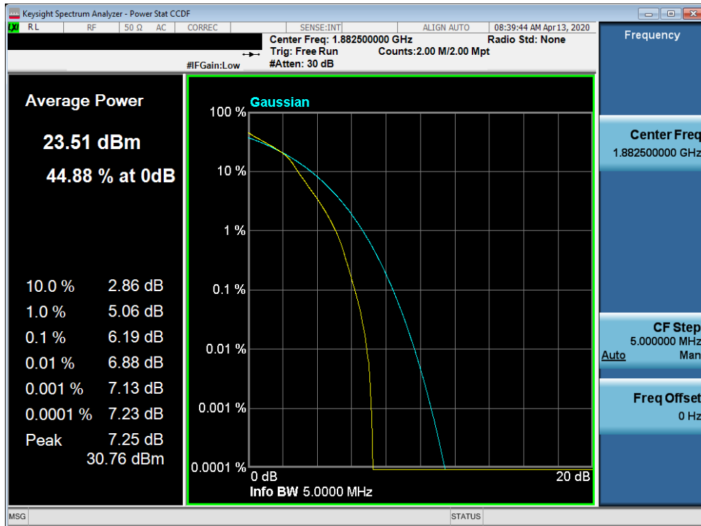
Plot 7-525. PAR Plot (Band 25/2 - 5.0MHz 16-QAM - Full RB Configuration)
