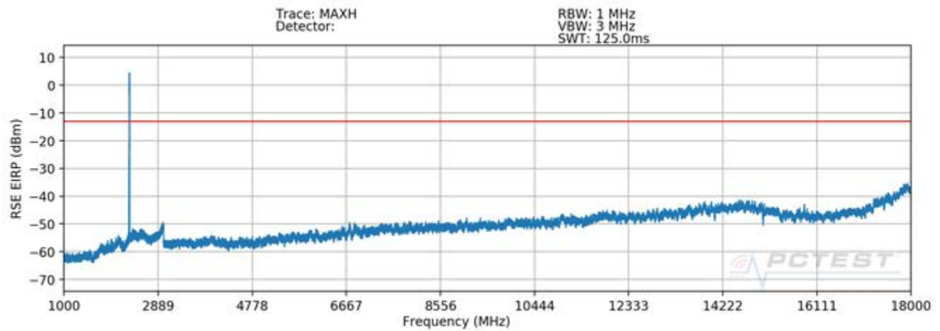
Plot 7-580. Radiated Spurious Plot above 1GHz (Band n5 + B66)
