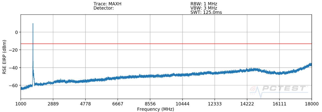
Plot 7-583. Radiated Spurious Plot above 1GHz (Band n66 + B12)
