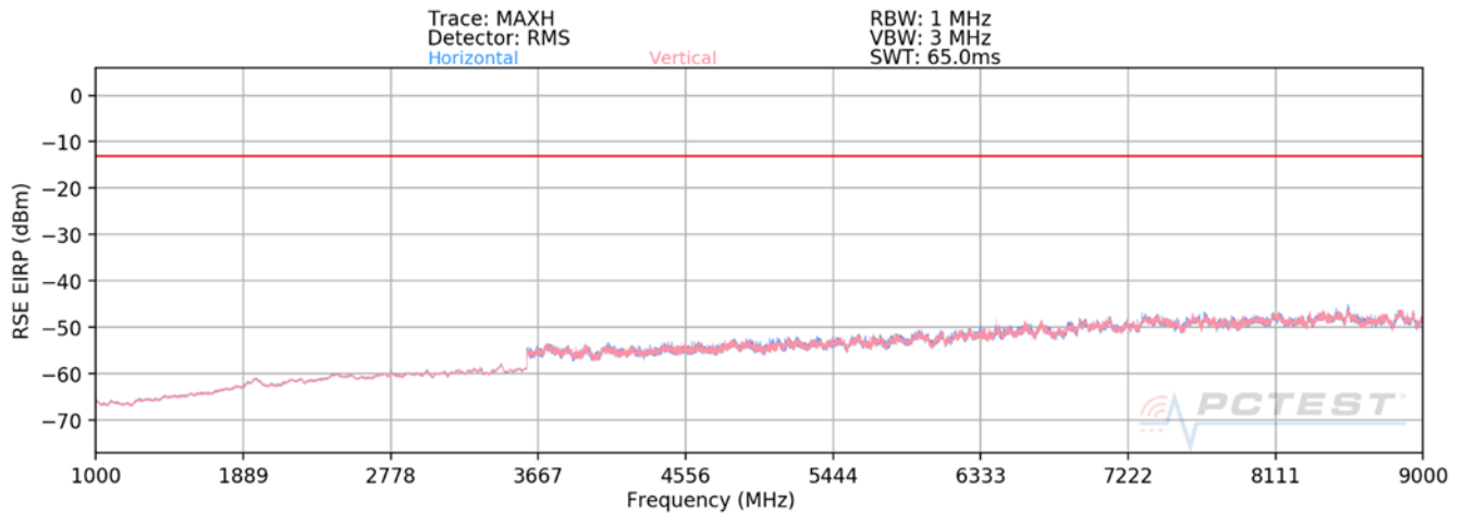
Plot 7-579. Radiated Spurious Plot above 1GHz (Band n5)
