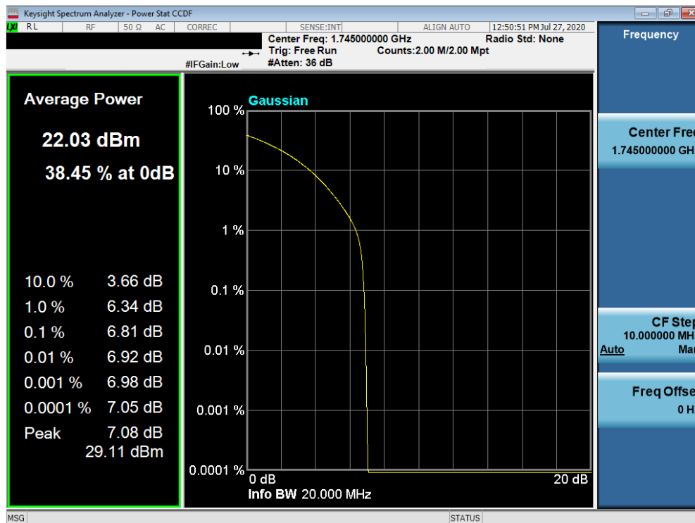
Plot 7-536. PAR Plot (NR n66/4 - 5.0MHz 16-QAM - Full RB Configuration)
