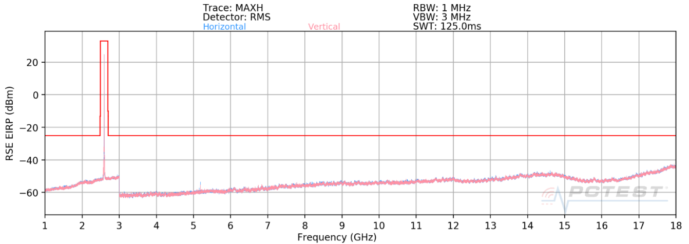
Plot 7-589. Radiated Spurious Plot above 1GHz (Band 41)
