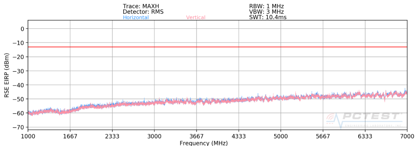
Plot 7-574. Radiated Spurious Plot above 1GHz (n71)
