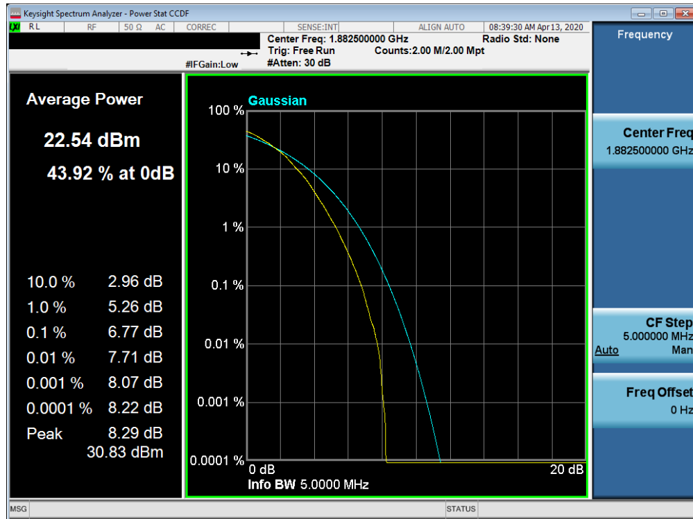
Plot 7-526. PAR Plot (Band 25/2 - 5.0MHz 64-QAM - Full RB Configuration)
