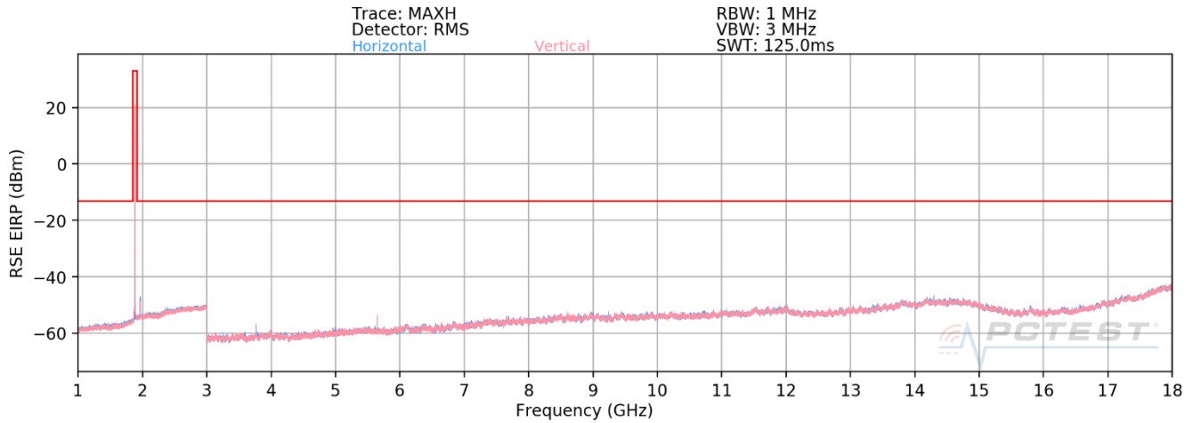
Plot 7-585. Radiated Spurious Plot above 1GHz (Band 25/2)
