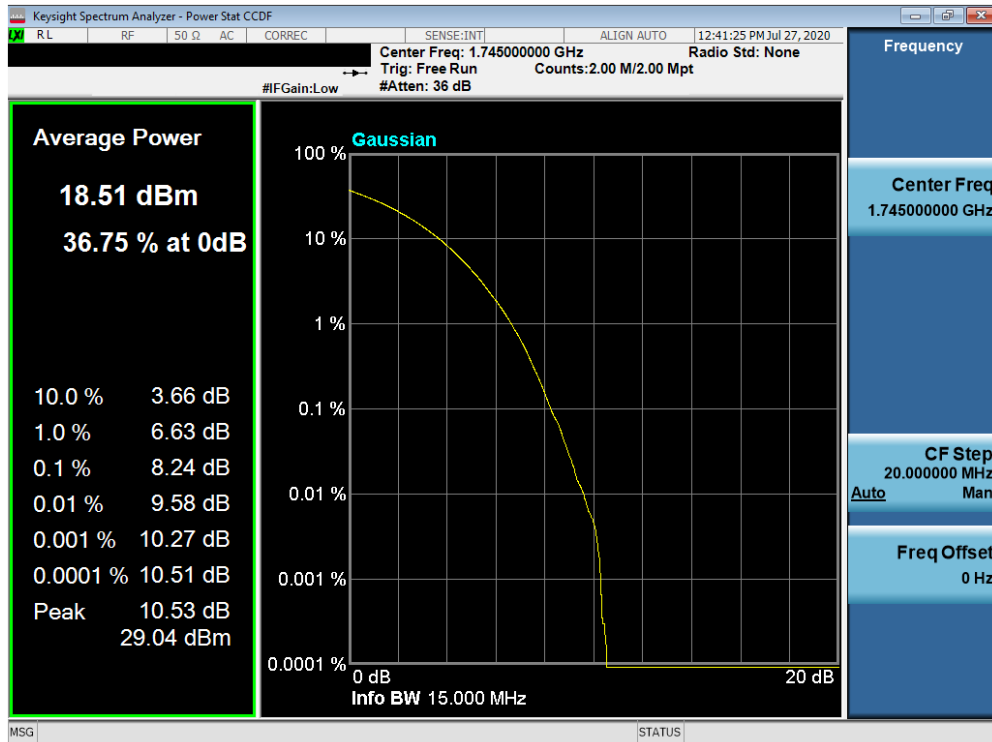
Plot 7-546. PAR Plot (NR n66/4 - 15.0MHz 256-QAM - Full RB Configuration)
