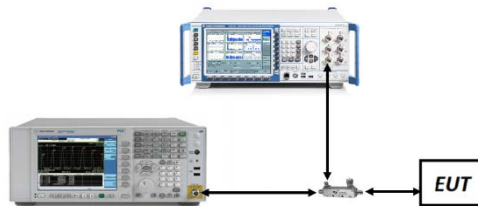
Figure 7-7. Test Instrument & Measurement Setup
