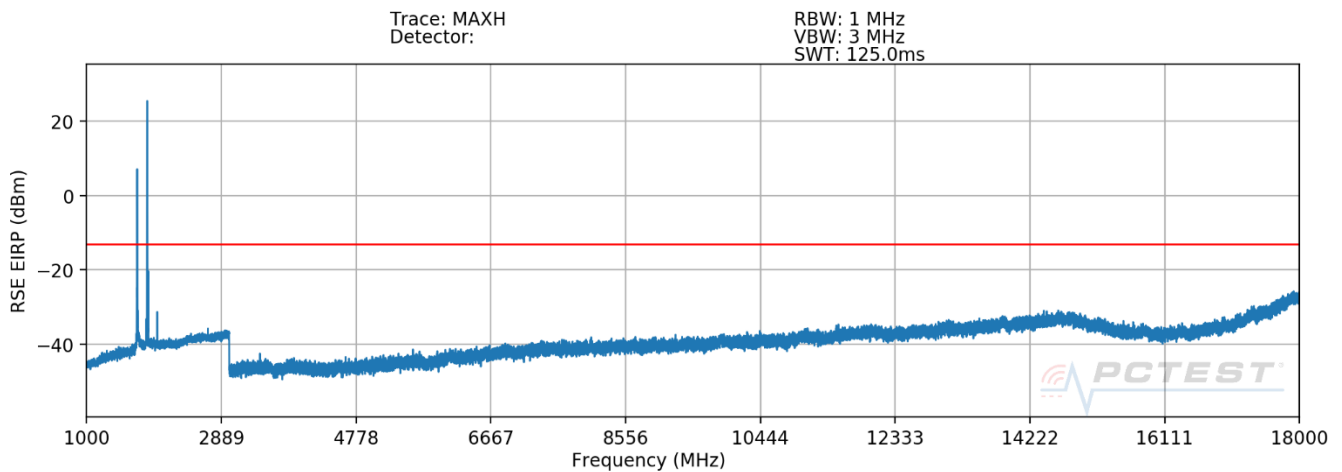
Plot 7-584. Radiated Spurious Plot above 1GHz (Band n66 + B2)
