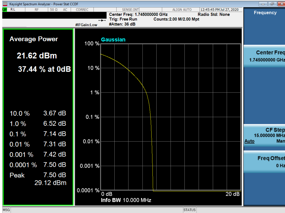
Plot 7-541. PAR Plot (NR n66/4 - 10.0MHz 64-QAM - Full RB Configuration)
