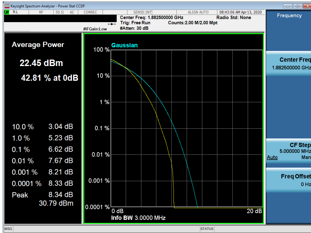
Plot 7-523. PAR Plot (Band 25/2 - 3.0MHz 64-QAM - Full RB Configuration)
