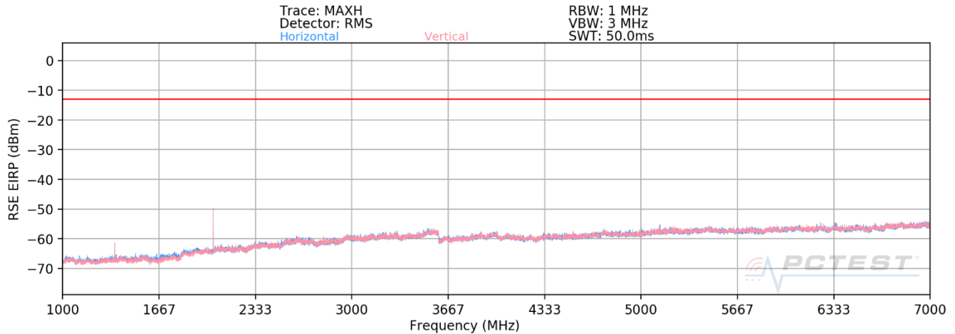
Plot 7-573. Radiated Spurious Plot above 1GHz (Band 71)
