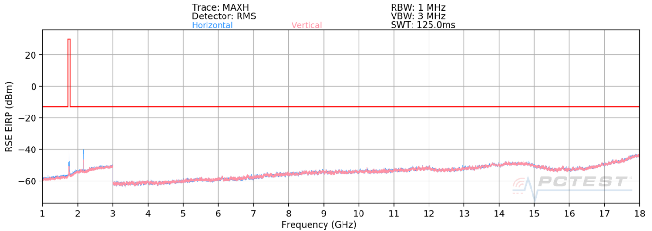
Plot 7-582. Radiated Spurious Plot above 1GHz (Band n66)
