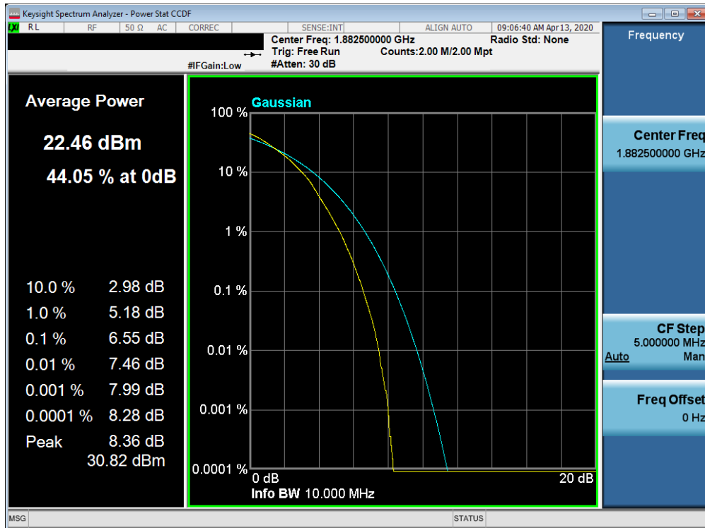
Plot 7-529. PAR Plot (Band 25/2 - 10.0MHz 64-QAM - Full RB Configuration)
