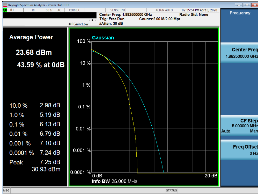
Plot 7-531. PAR Plot (Band 25/2 - 15.0MHz 16-QAM - Full RB Configuration)
