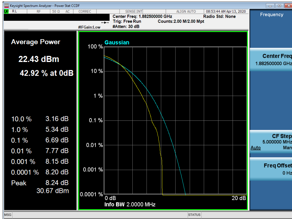
Plot 7-520. PAR Plot (Band 25/2 - 1.4MHz 64-QAM - Full RB Configuration)
