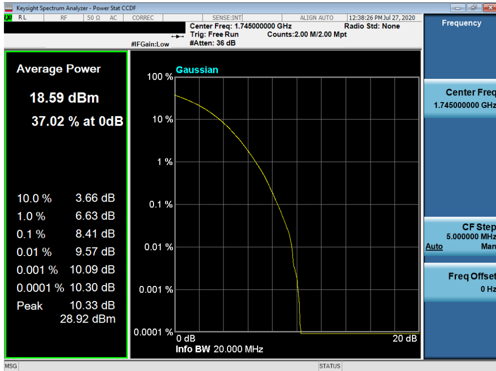
Plot 7-550. PAR Plot (NR n66/4 - 20.0MHz 256-QAM - Full RB Configuration)
