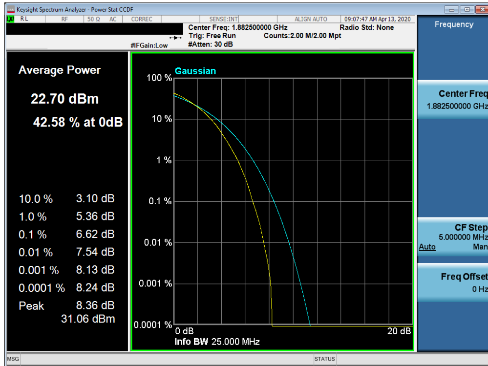
Plot 7-532. PAR Plot (Band 25/2 - 15.0MHz 64-QAM - Full RB Configuration)
