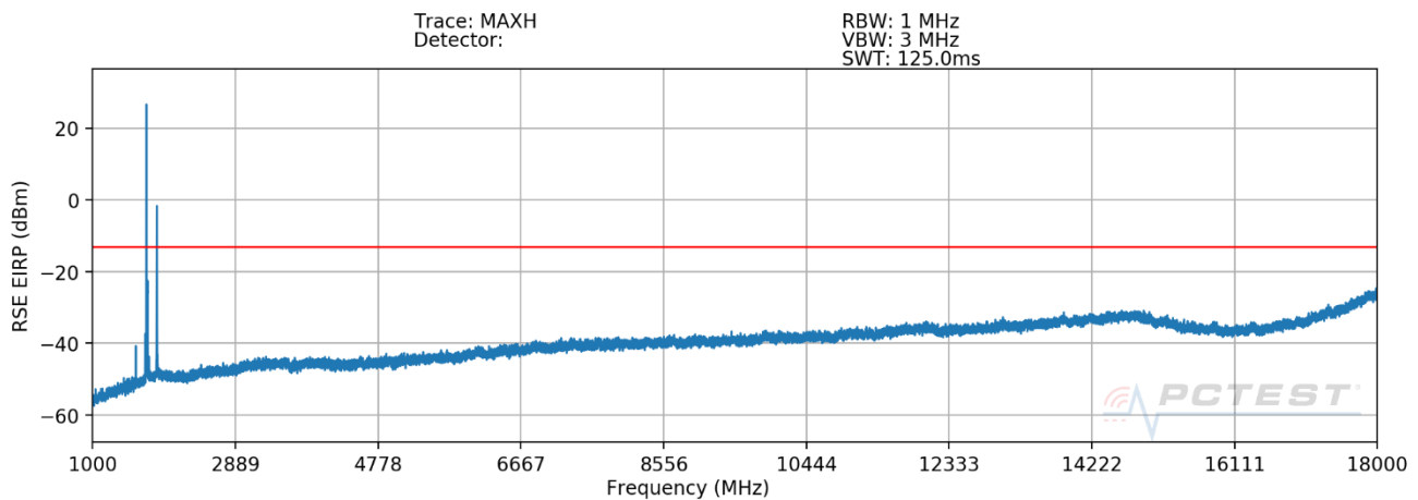
Plot 7-588. Radiated Spurious Plot above 1GHz (n2+ Anchor B66 EN-DC)
