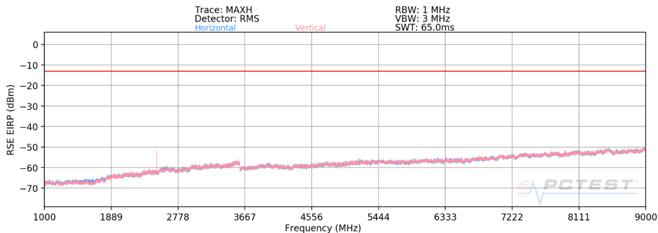
Plot 7-578. Radiated Spurious Plot above 1GHz (Band 26)
