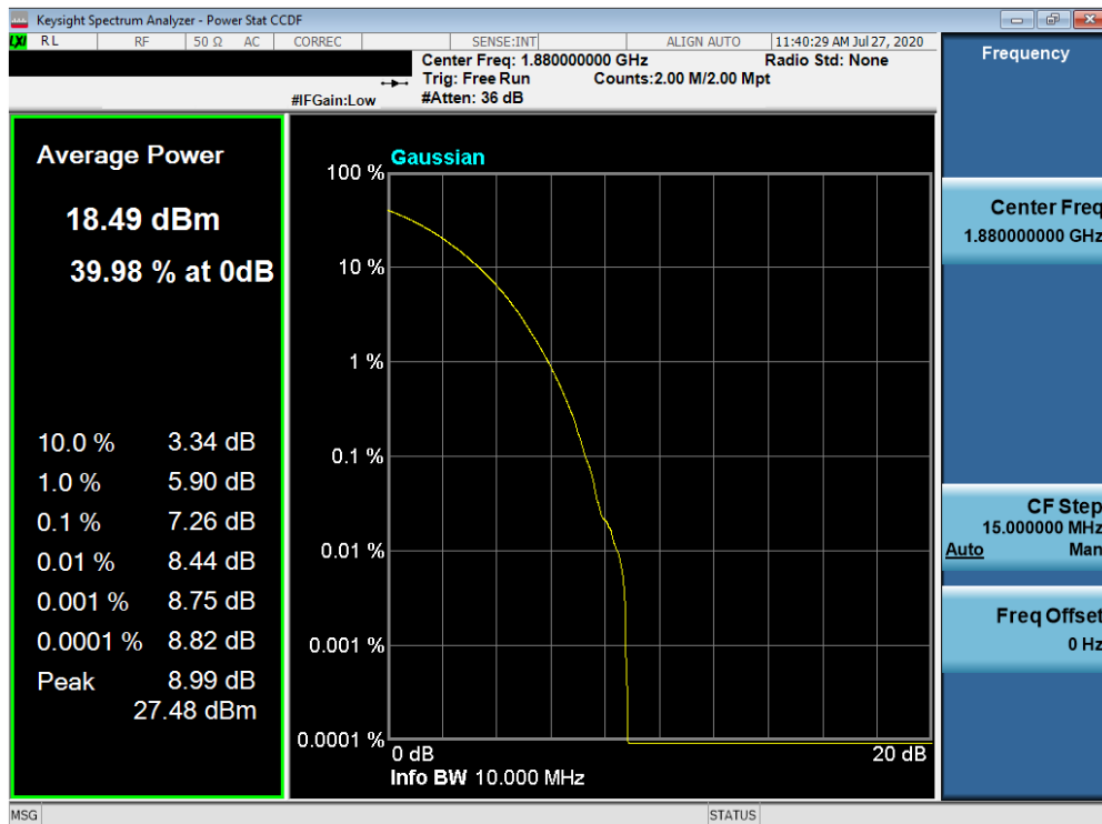
Plot 7-558. PAR Plot (NR n25/2 - 10.0MHz 256-QAM - Full RB Configuration)
