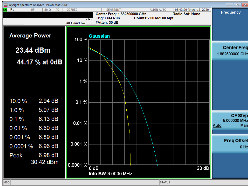
Plot 7-522. PAR Plot (Band 25/2 - 3.0MHz 16-QAM - Full RB Configuration)
