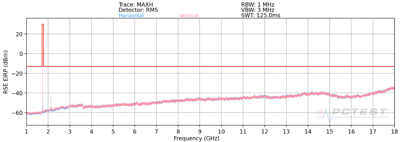
Plot 7-592. Radiated Spurious Plot 1GHz - 18GHz (ULCA 12A-66A)
