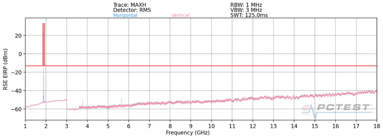
Plot 7-586. Radiated Spurious Plot above 1GHz (n25/2 Standalone)
