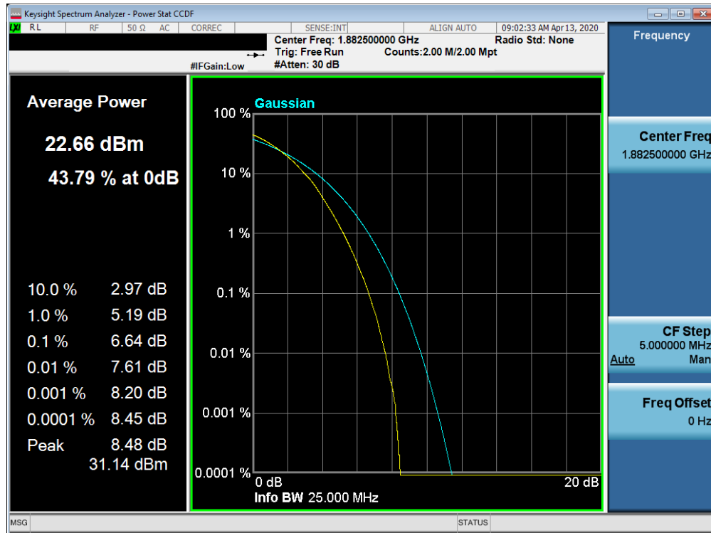
Plot 7-534. PAR Plot (Band 25/2 - 20.0MHz 64-QAM - Full RB Configuration)
