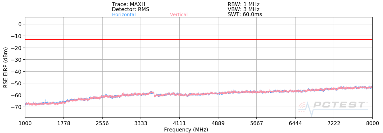
Plot 7-576. Radiated Spurious Plot above 1GHz (Band 12)
