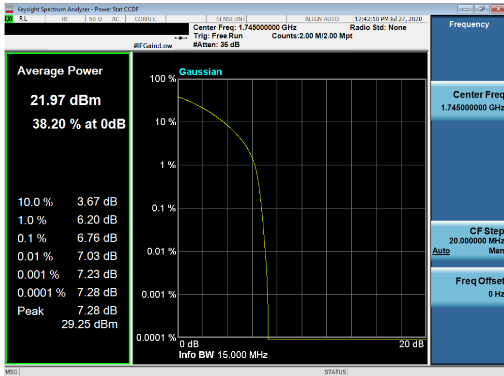
Plot 7-544. PAR Plot (NR n66/4 - 15.0MHz 16-QAM - Full RB Configuration)
