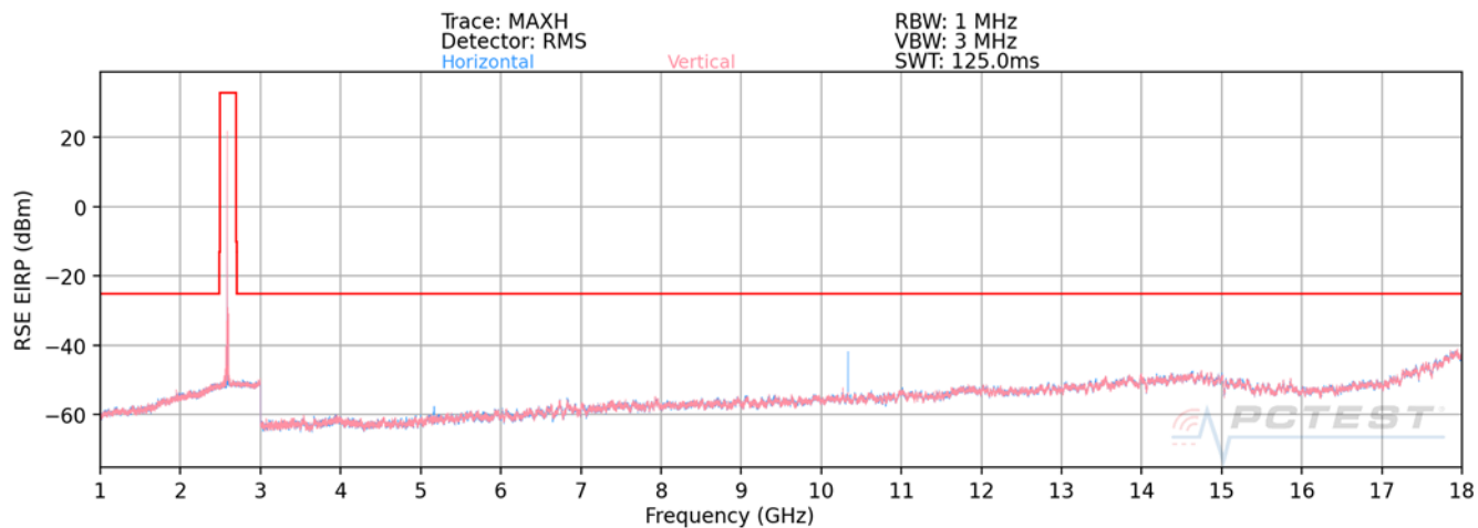
Plot 7-591. Radiated Spurious Plot above 1GHz (n41 Standalone)
