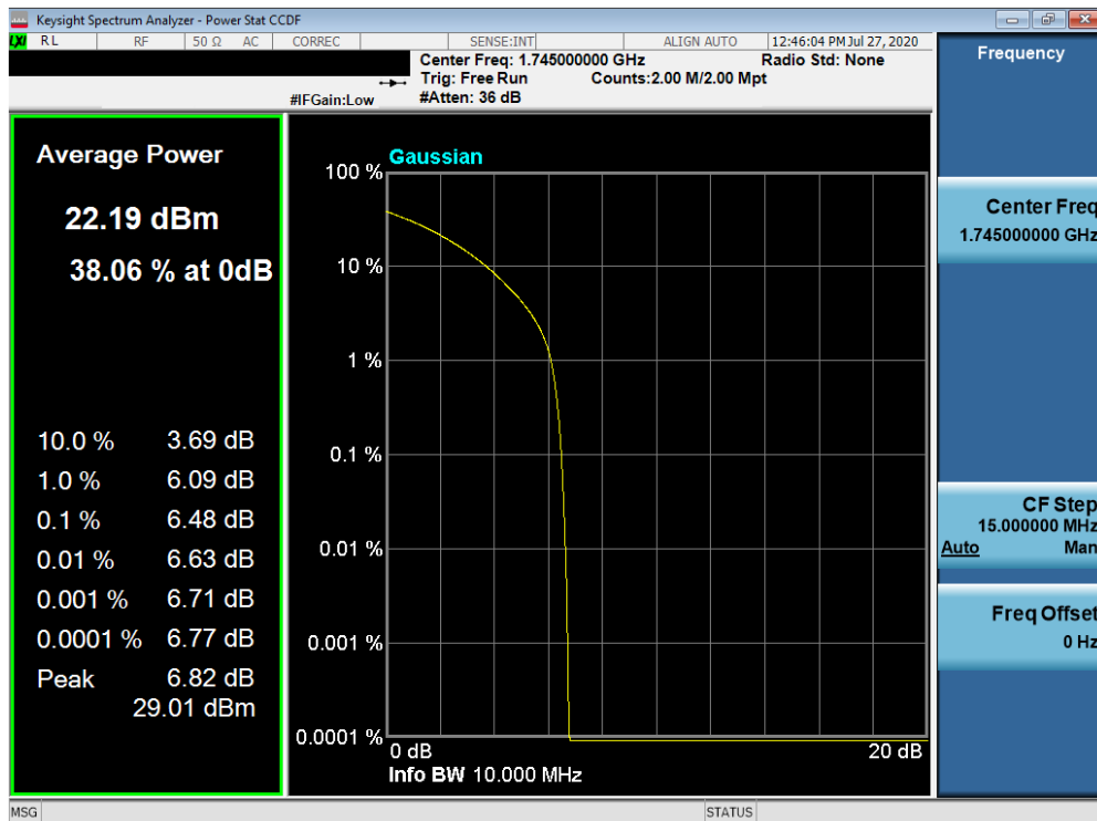
Plot 7-540. PAR Plot (NR n66/4 - 10.0MHz 16-QAM - Full RB Configuration)
