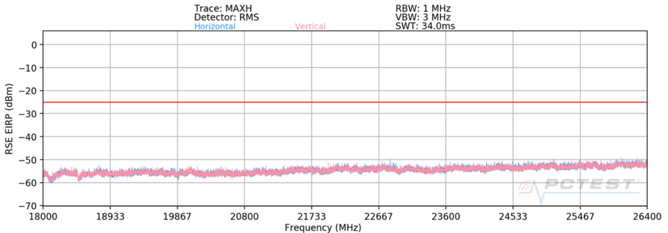
Plot 7-590. Radiated Spurious Plot 18GHz – 26.5GHz (Band 41)
