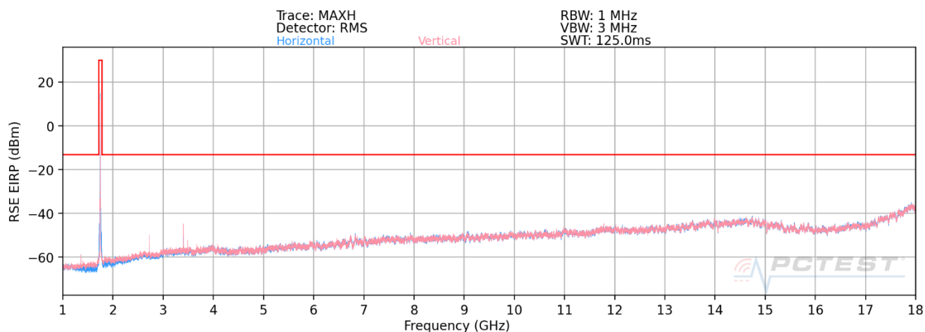
Plot 7-575. Radiated Spurious Plot above 1GHz (n71 + B66)
