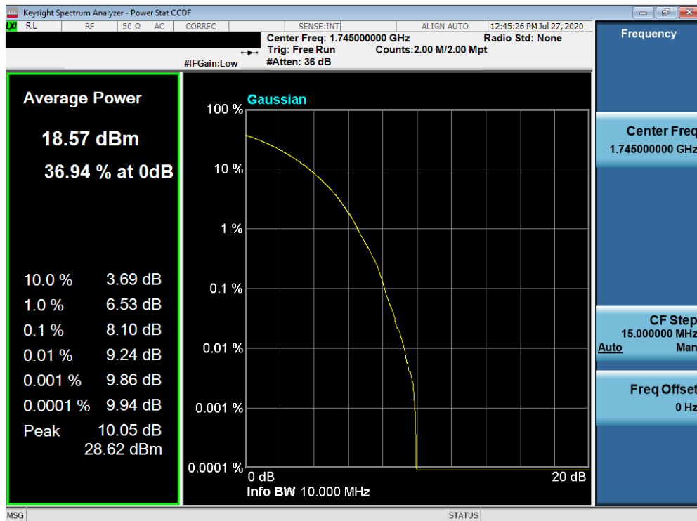
Plot 7-542. PAR Plot (NR n66/4 - 10.0MHz 256-QAM - Full RB Configuration)
