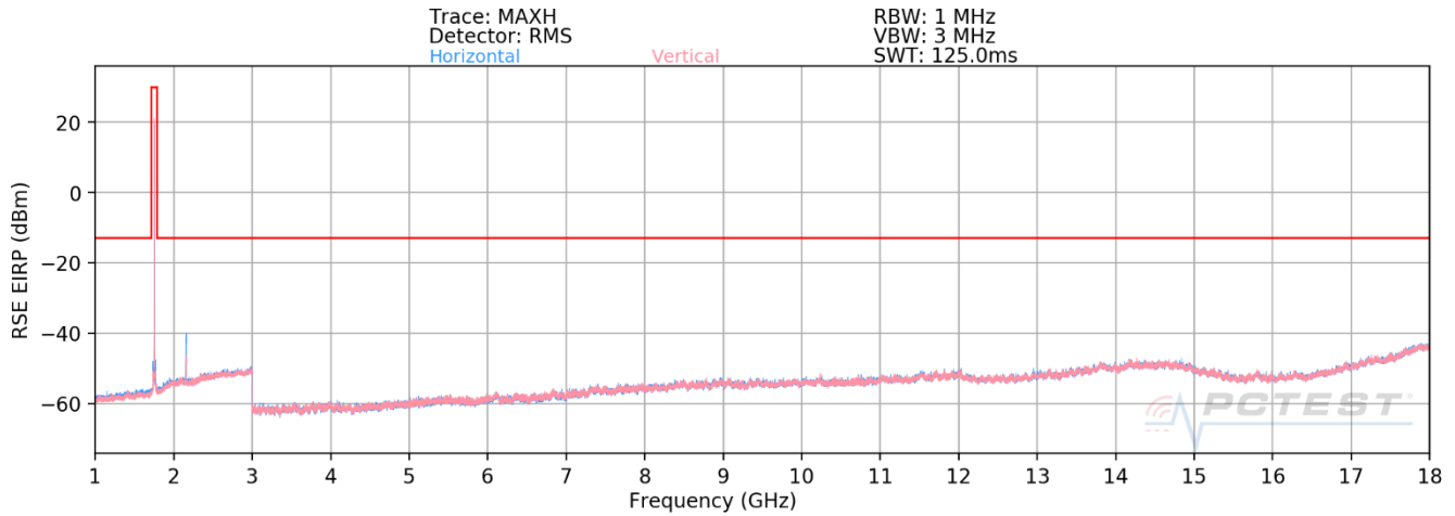
Plot 7-581. Radiated Spurious Plot above 1GHz (Band 66/4)
