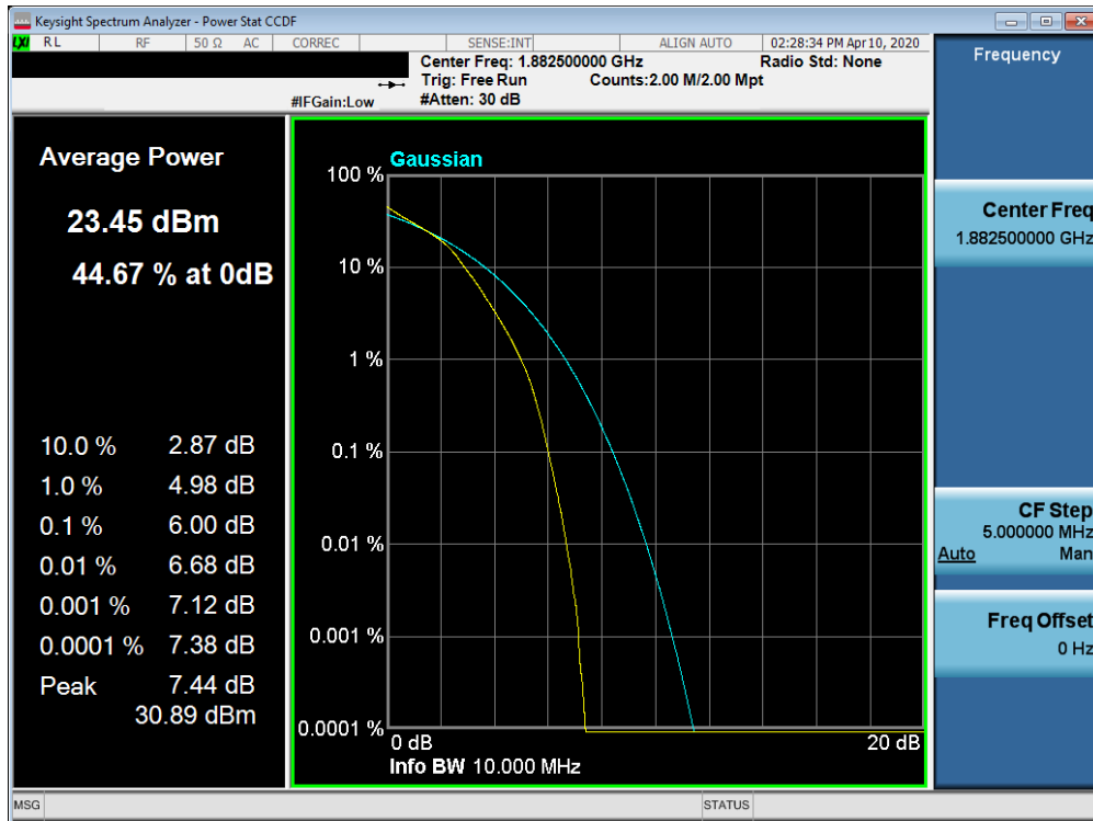
Plot 7-528. PAR Plot (Band 25/2 - 10.0MHz 16-QAM - Full RB Configuration)
