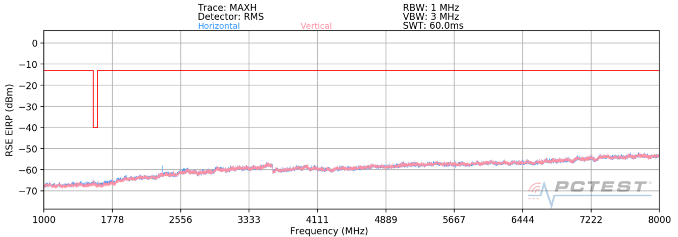
Plot 7-577. Radiated Spurious Plot above 1GHz (Band 13)
