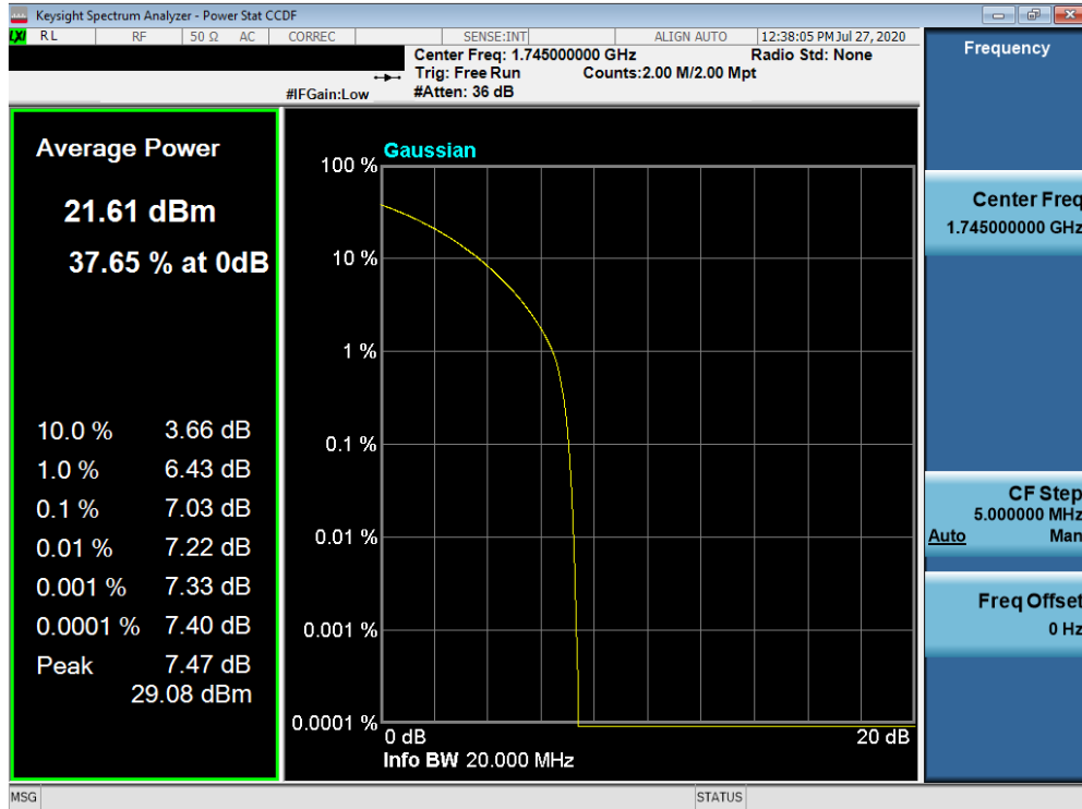
Plot 7-549. PAR Plot (NR n66/4 - 20.0MHz 64-QAM - Full RB Configuration)
