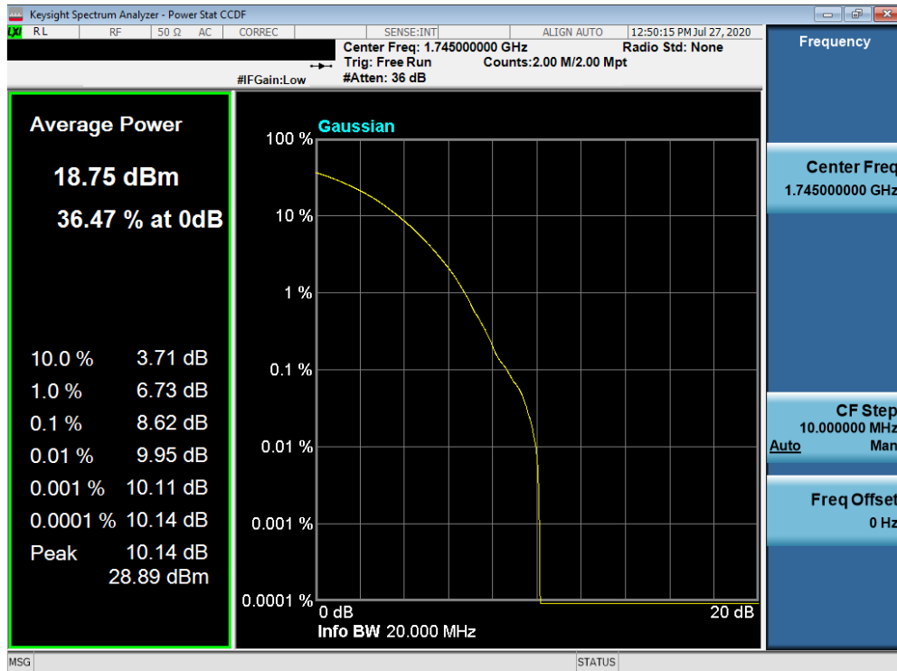
Plot 7-538. PAR Plot (NR n66/4 - 5.0MHz 256-QAM - Full RB Configuration)
