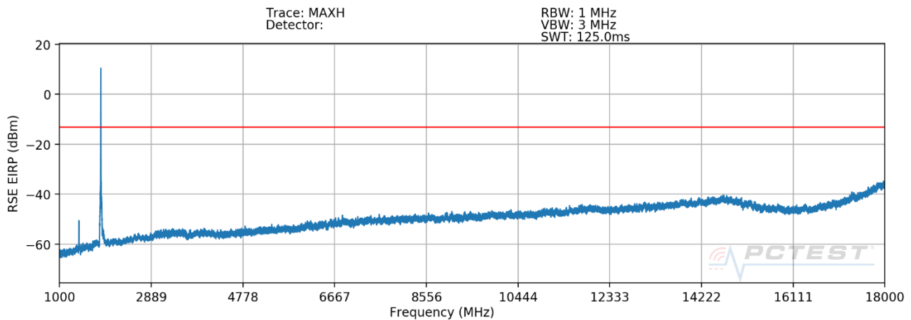
Plot 7-587. Radiated Spurious Plot above 1GHz (n2+ Anchor B12 EN-DC)
