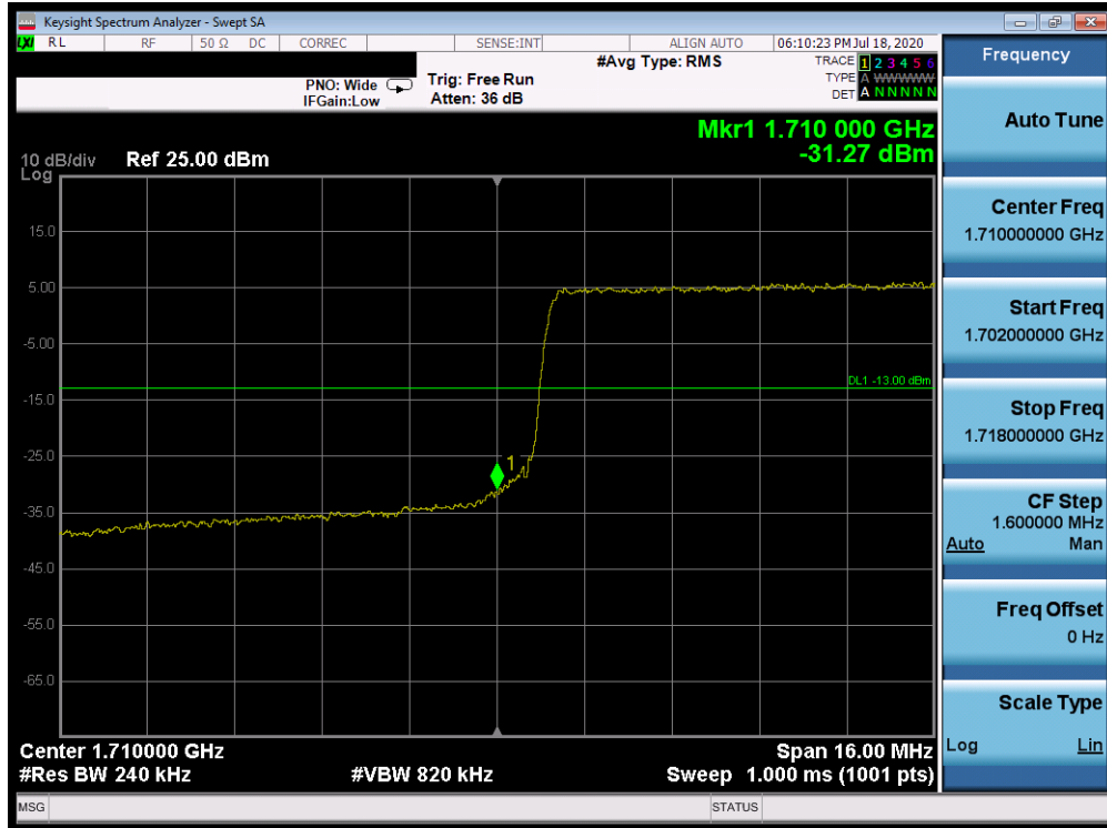
Plot 7-396. Lower Band Edge Plot (Band 66/4 - 20.0MHz QPSK - Full RB Configuration)
