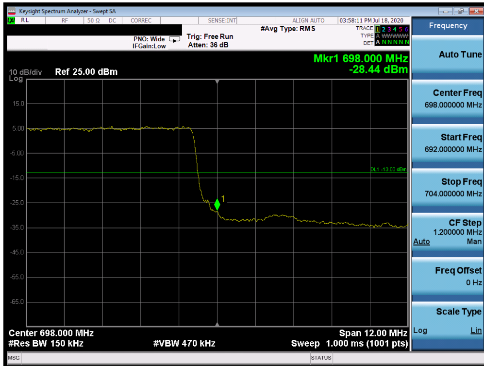
Plot 7-319. Upper Band Edge Plot (Band 71 - 15.0MHz QPSK - Full RB Configuration)
