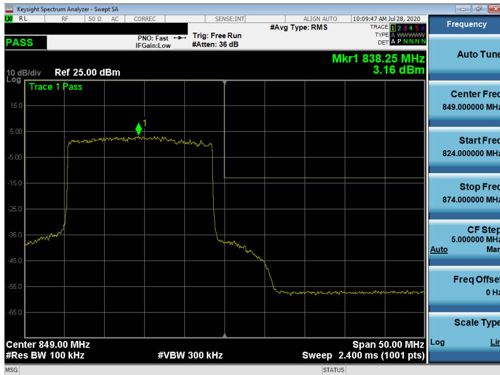
Plot 7-365. Upper Band Edge Plot (NR Band n5 - 20.0MHz - Full RB)
