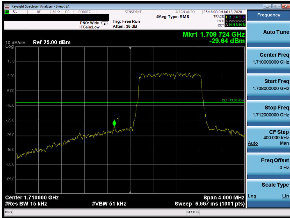
Plot 7-366. Lower Band Edge Plot (Band 66/4 - 1.4MHz QPSK - Full RB Configuration)
