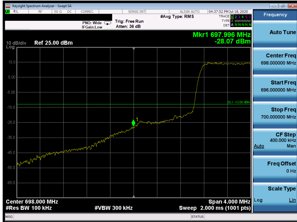
Plot 7-330. Lower Band Edge Plot (Band 12 - 1.4MHz QPSK - Full RB Configuration)
