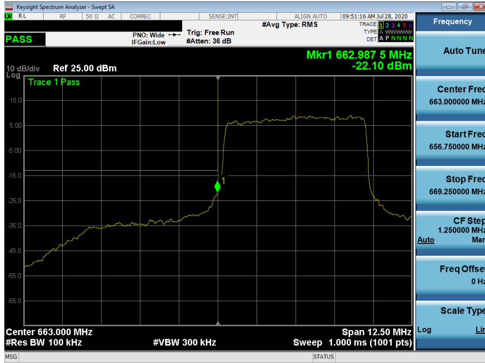
Plot 7-322. Lower Band Edge Plot (NR Band n71 – 5.0MHz - Full RB)
