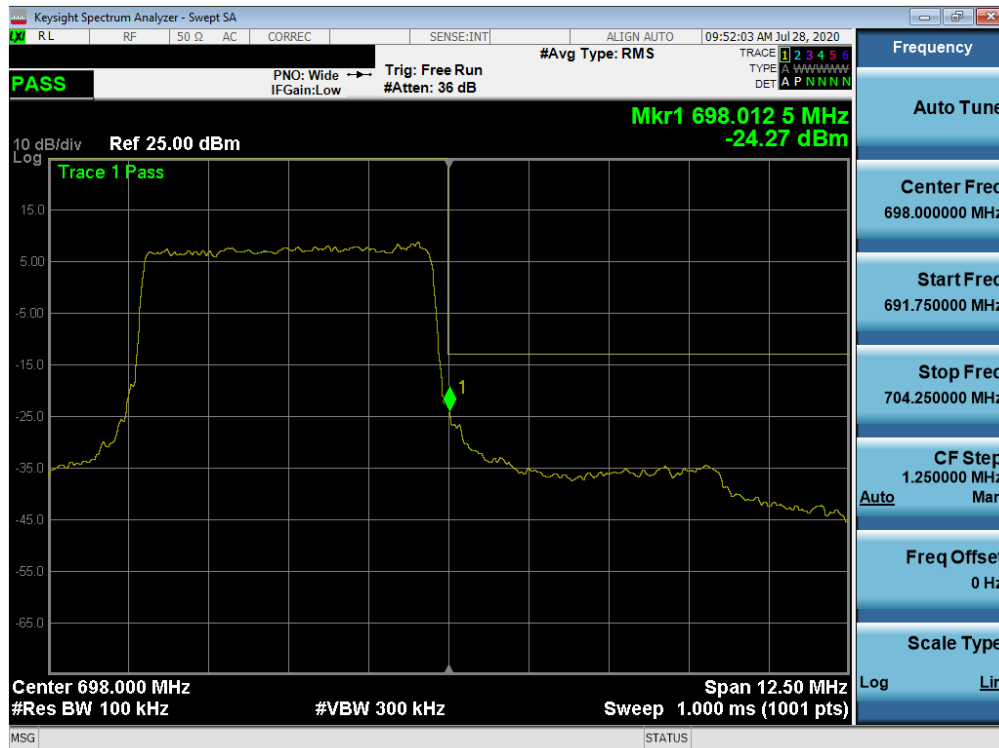
Plot 7-323. Upper Band Edge Plot (NR Band n71 – 5.0MHz - Full RB)
