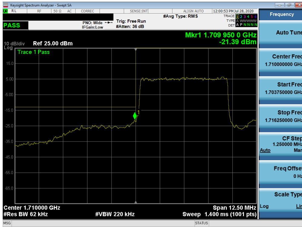
Plot 7-402. Lower Band Edge Plot (NR Band n66 – 5.0MHz - Full RB)
