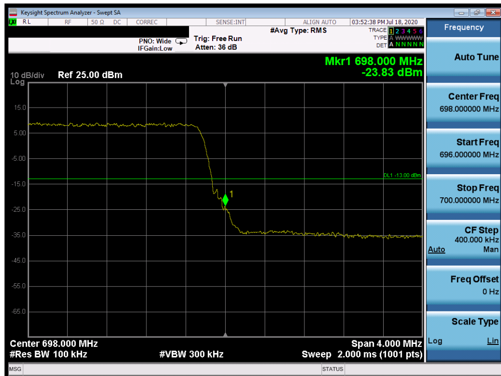
Plot 7-315. Upper Band Edge Plot (Band 71 – 5.0MHz QPSK - Full RB Configuration)
