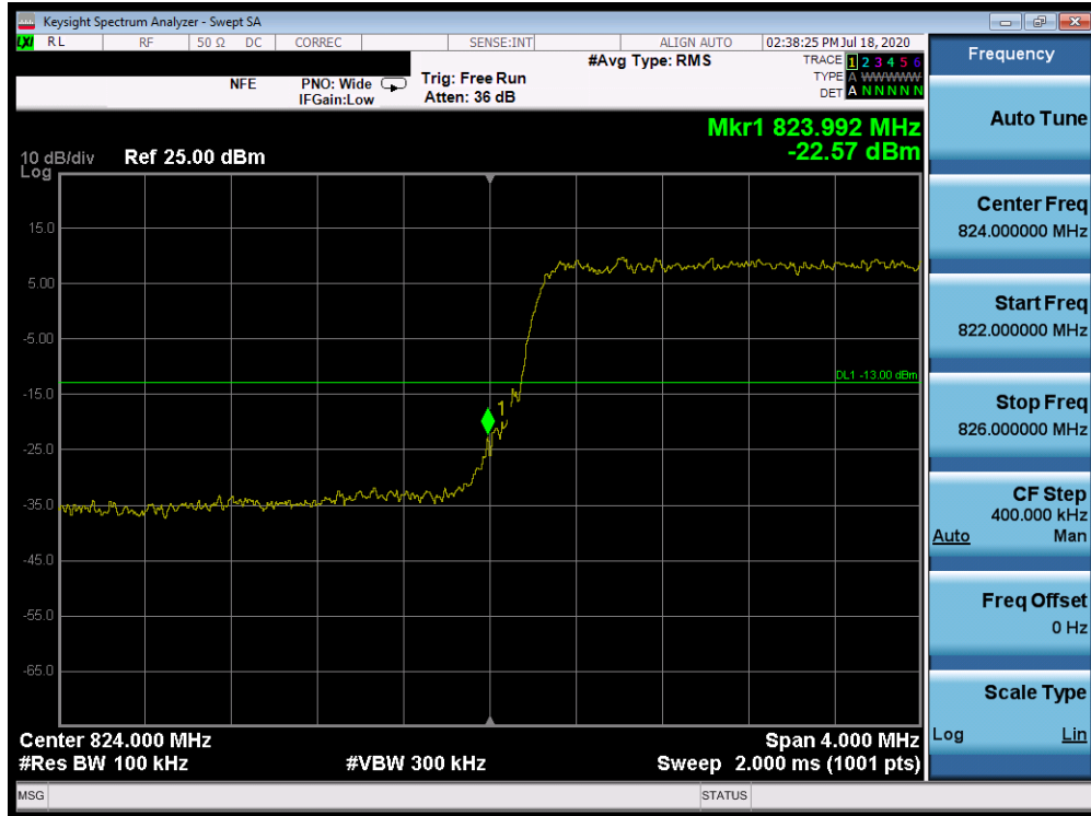
Plot 7-352. Lower Band Edge Plot (Band 26/5 - 5.0MHz QPSK - Full RB Configuration)
