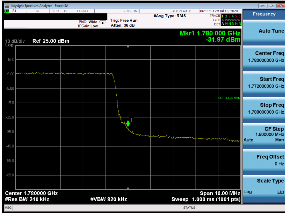
Plot 7-400. Upper Band Edge Plot (Band 66 - 20.0MHz QPSK - Full RB Configuration)
