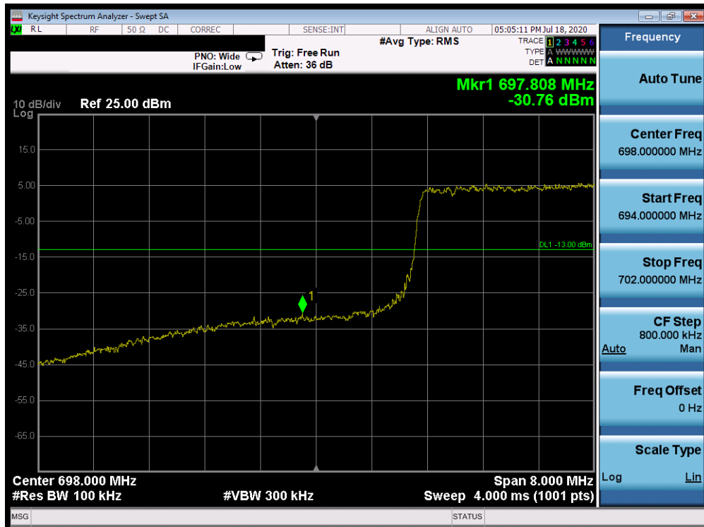
Plot 7-337. Lower Band Edge Plot (Band 12 - 10.0MHz QPSK - Full RB Configuration)
