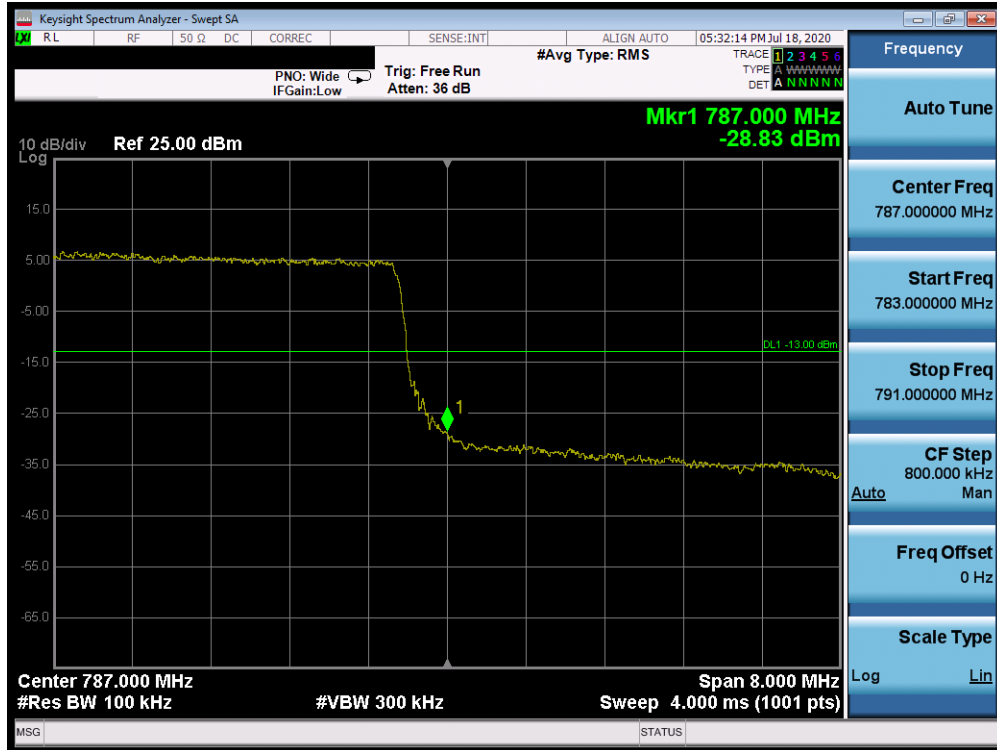
Plot 7-346. Upper Band Edge Plot (Band 13 - 10.0MHz QPSK - Full RB Configuration)
