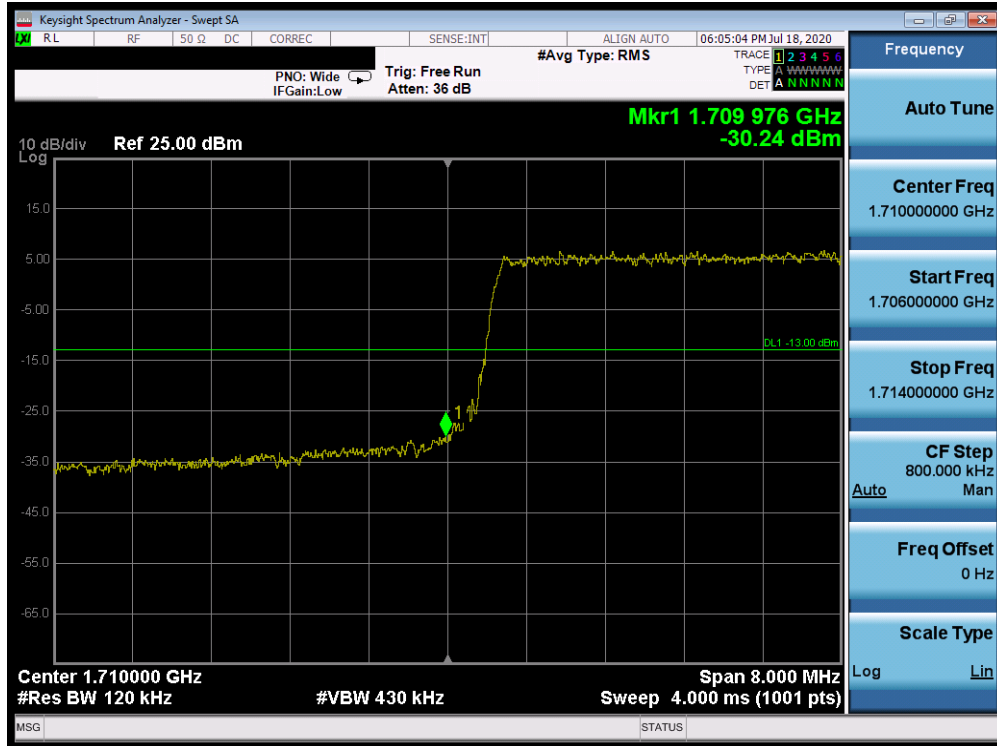
Plot 7-384. Lower Band Edge Plot (Band 66/4 - 10.0MHz QPSK - Full RB Configuration)
