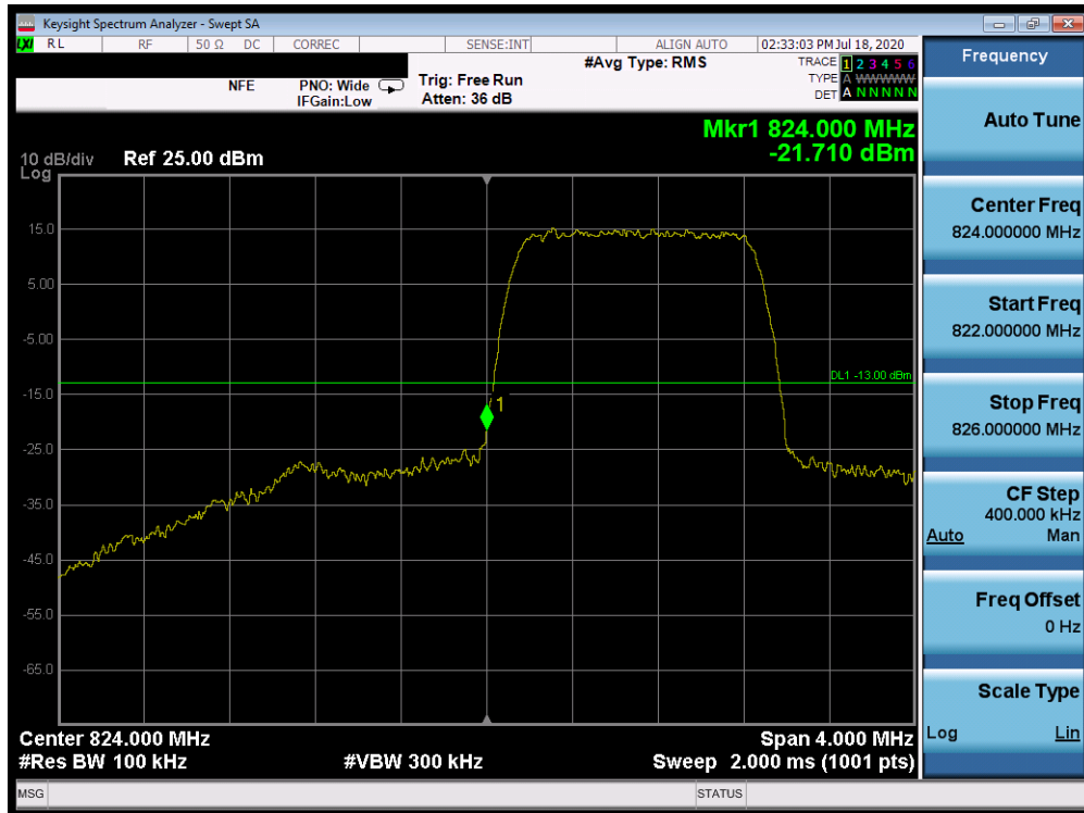
Plot 7-348. Lower Band Edge Plot (Band 26/5 - 1.4MHz QPSK - Full RB Configuration)
