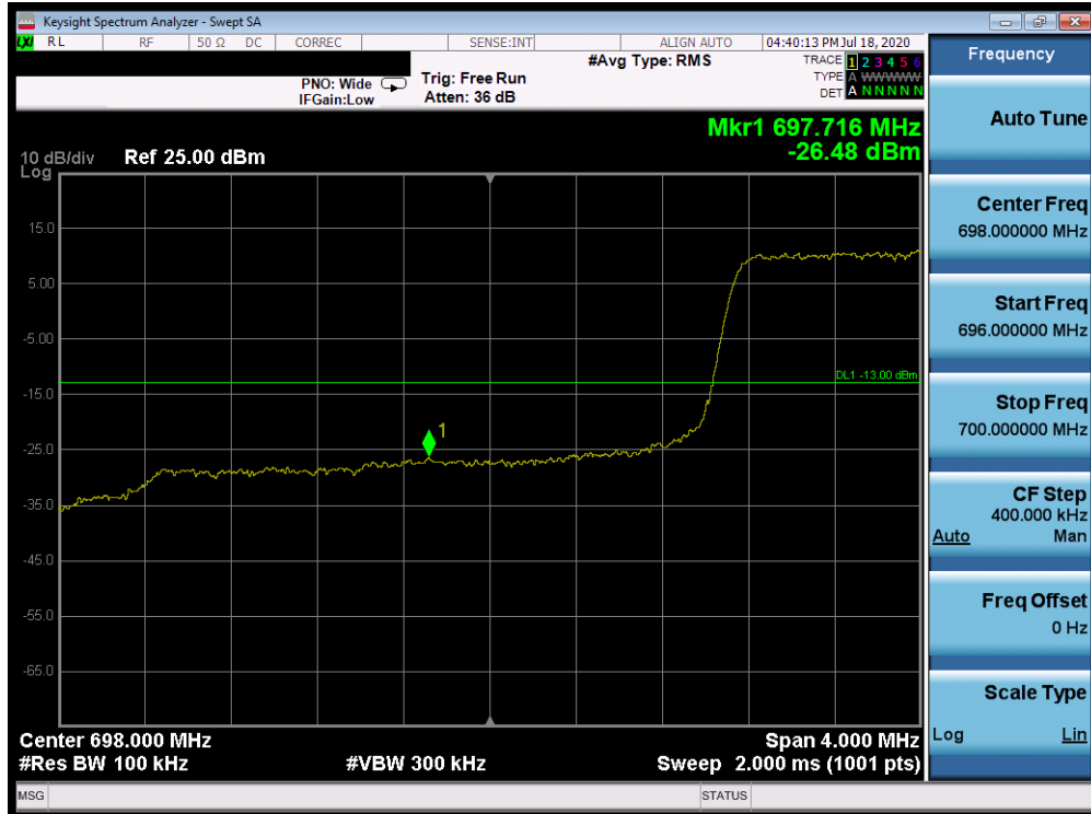
Plot 7-332. Lower Band Edge Plot (Band 12 - 3.0MHz QPSK - Full RB Configuration)
