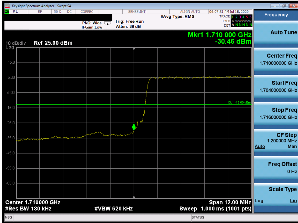
Plot 7-390. Lower Band Edge Plot (Band 66/4 - 15.0MHz QPSK - Full RB Configuration)
