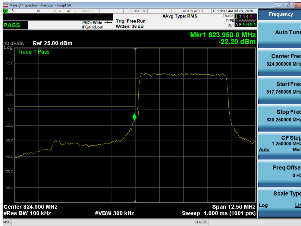
Plot 7-358. Lower Band Edge Plot (NR Band n5 – 5.0MHz - Full RB)
