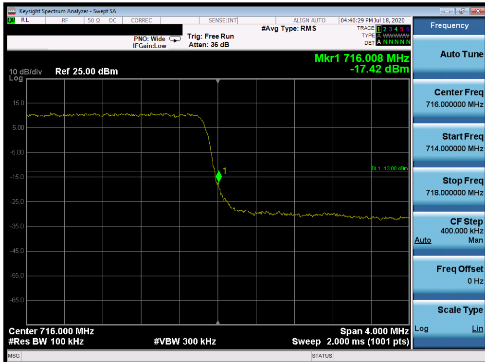
Plot 7-333. Upper Band Edge Plot (Band 12 - 3.0MHz QPSK - Full RB Configuration)
