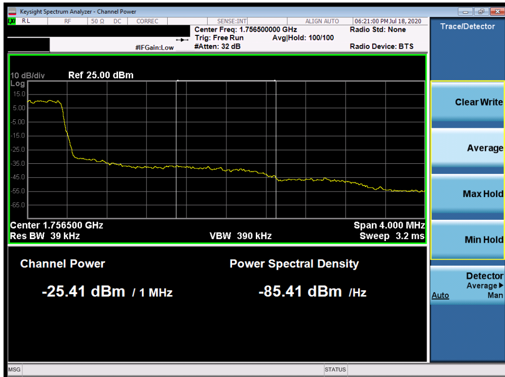
Plot 7-369. Upper Extended Band Edge Plot (Band 4 - 1.4MHz QPSK - Full RB Configuration)
