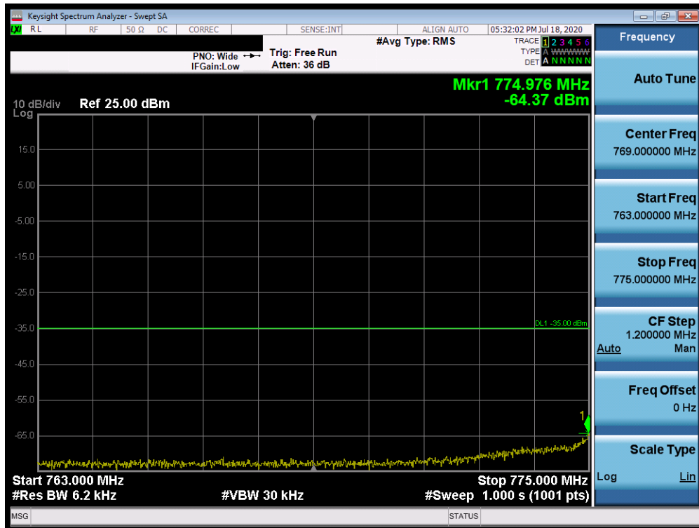
Plot 7-345. Lower Emission Mask Plot (Band 13 - 10.0MHz QPSK - Full RB Configuration)
