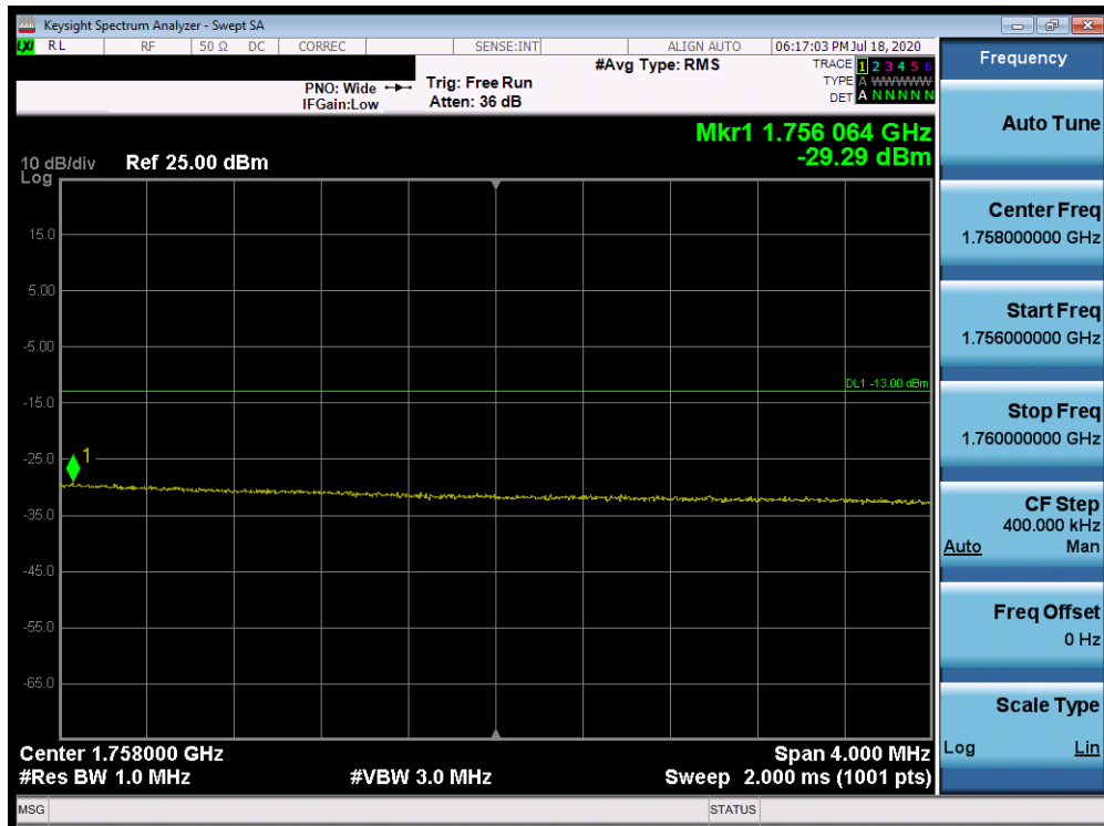
Plot 7-399. Upper Extended Band Edge Plot (Band 4 - 20.0MHz QPSK - Full RB Configuration)
