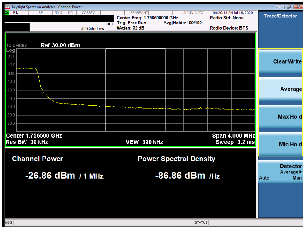
Plot 7-375. Upper Extended Band Edge Plot (Band 4 - 3.0MHz QPSK - Full RB Configuration)
