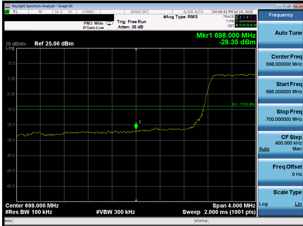
Plot 7-334. Lower Band Edge Plot (Band 12 - 5.0MHz QPSK - Full RB Configuration)
