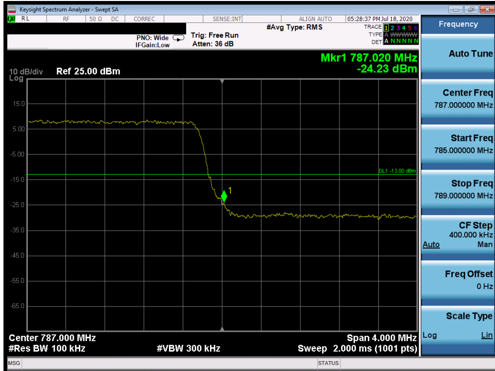
Plot 7-342. Upper Band Edge Plot (Band 13 - 5.0MHz QPSK - Full RB Configuration)
