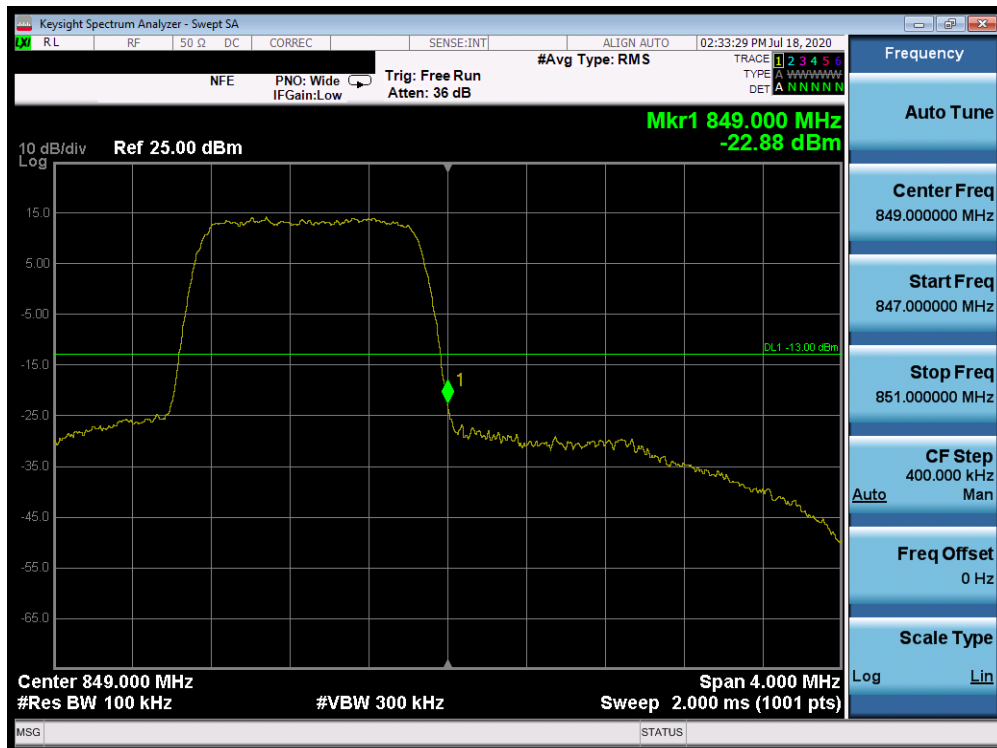
Plot 7-349. Upper Band Edge Plot (Band 26/5 - 1.4MHz QPSK - Full RB Configuration)
