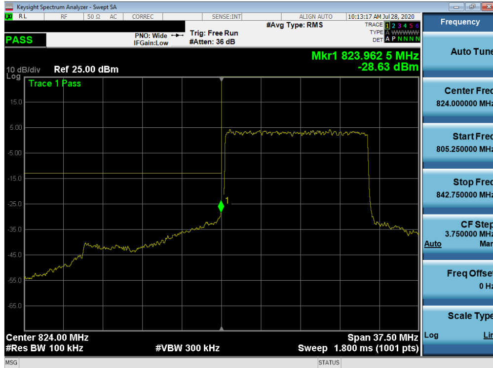
Plot 7-362. Lower Band Edge Plot (NR Band n5 - 15.0MHz - Full RB)
