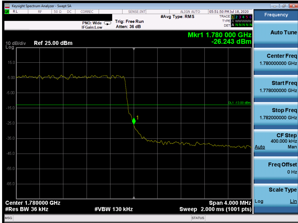
Plot 7-376. Upper Band Edge Plot (Band 66 - 3.0MHz QPSK - Full RB Configuration)
