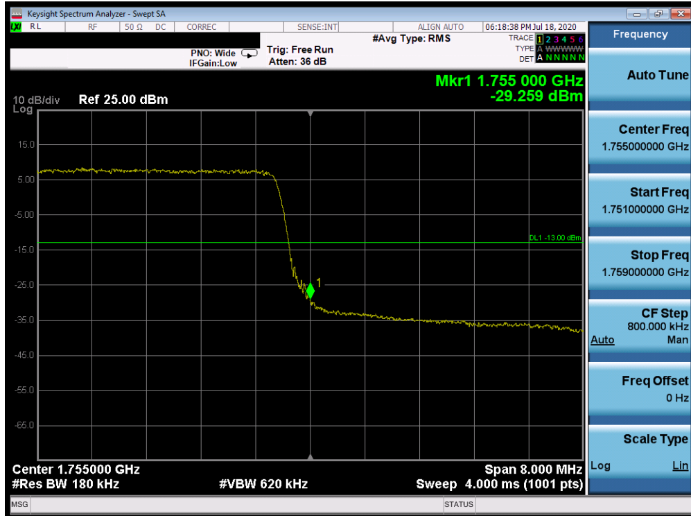
Plot 7-386. Upper Band Edge Plot (Band 4 - 10.0MHz QPSK - Full RB Configuration)
