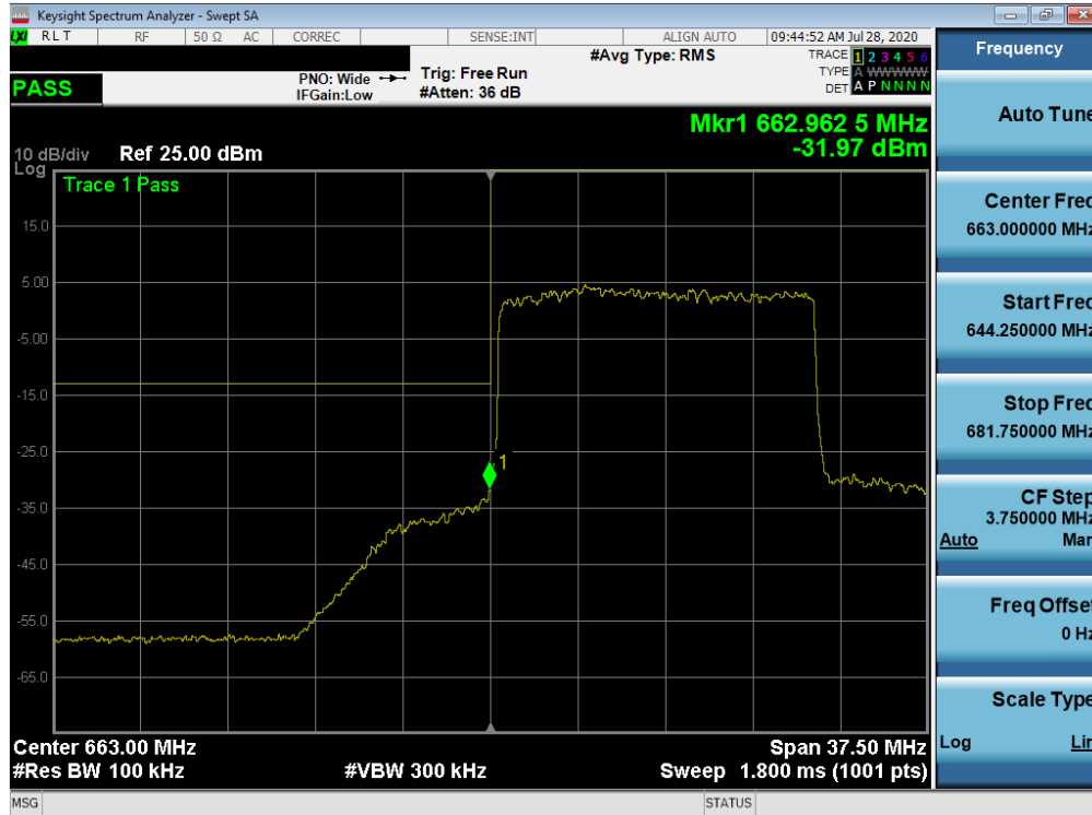
Plot 7-326. Lower Band Edge Plot (NR Band n71 - 15.0MHz - Full RB)
