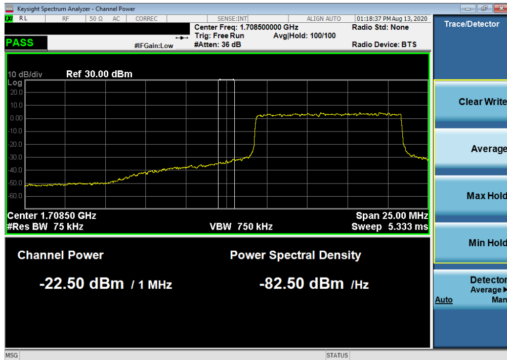
Plot 7-407. Lower Extended Band Edge Plot (NR Band n66 – 10.0MHz - Full RB)
