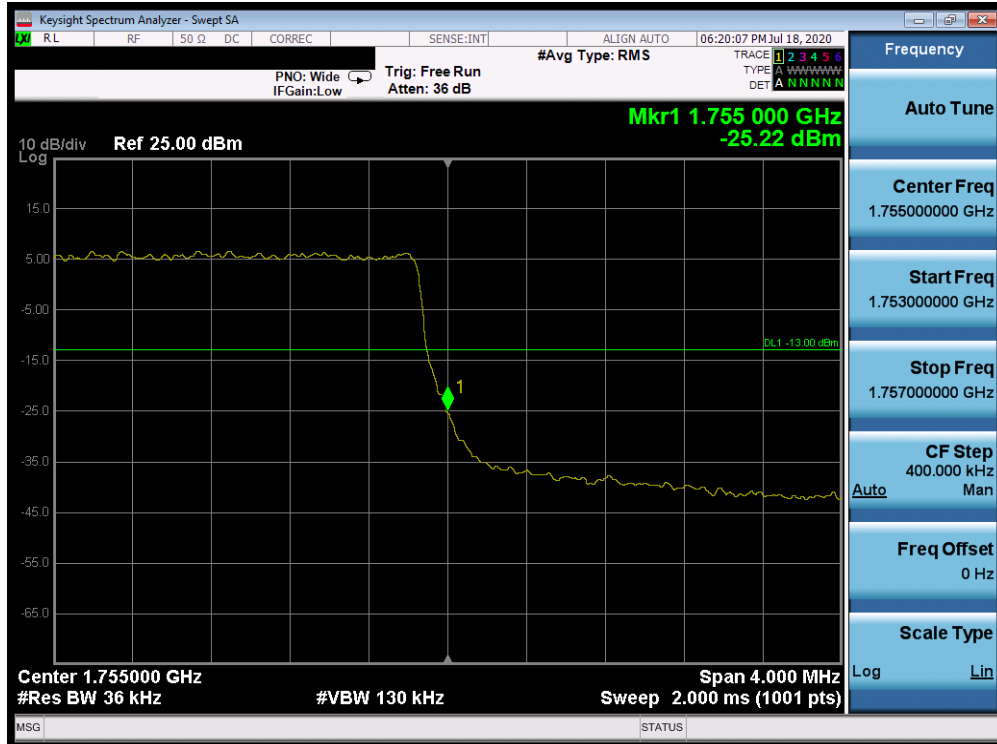
Plot 7-374. Upper Band Edge Plot (Band 4 - 3.0MHz QPSK - Full RB Configuration)
