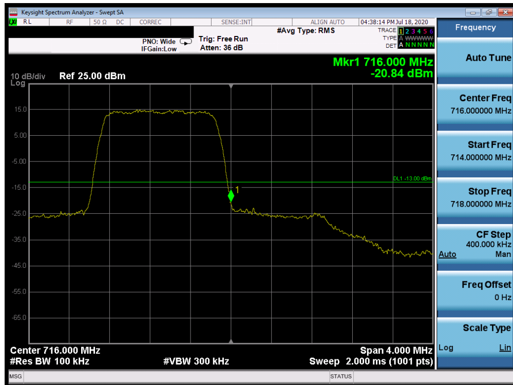
Plot 7-331. Upper Band Edge Plot (Band 12 - 1.4MHz QPSK - Full RB Configuration)
