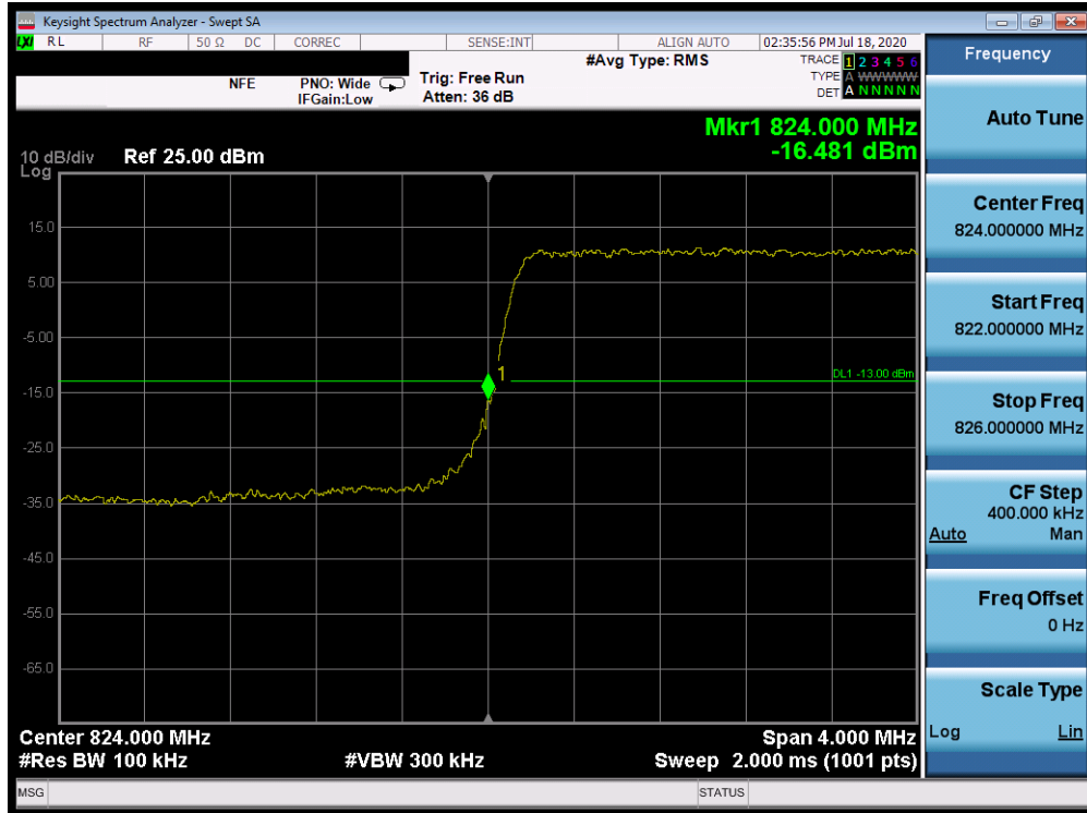
Plot 7-350. Lower Band Edge Plot (Band 26/5 - 3.0MHz QPSK - Full RB Configuration)
