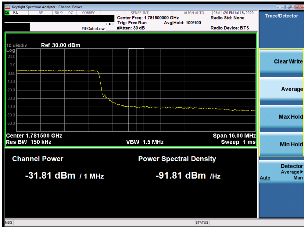
Plot 7-401. Upper Extended Band Edge Plot (Band 66 - 20.0MHz QPSK - Full RB Configuration)
