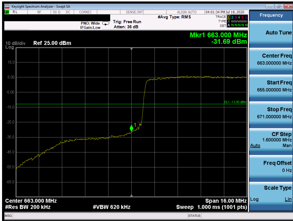
Plot 7-320. Lower Band Edge Plot (Band 71 - 20.0MHz QPSK - Full RB Configuration)
