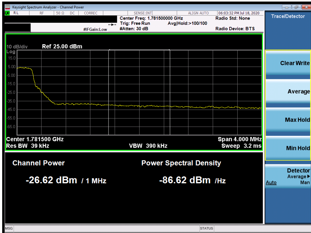
Plot 7-383. Upper Extended Band Edge Plot (Band 66 - 5.0MHz QPSK - Full RB Configuration)
