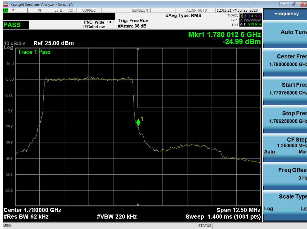
Plot 7-404. Upper Band Edge Plot (NR Band n66 – 5.0MHz - Full RB)
