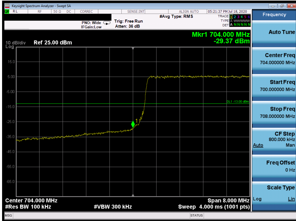
Plot 7-338. Lower Band Edge Plot (Band 17 - 10.0MHz QPSK - Full RB Configuration)
