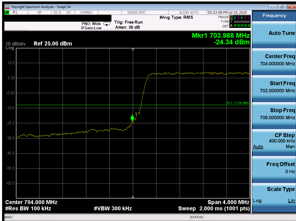
Plot 7-335. Lower Band Edge Plot (Band 17 - 5.0MHz QPSK - Full RB Configuration)
