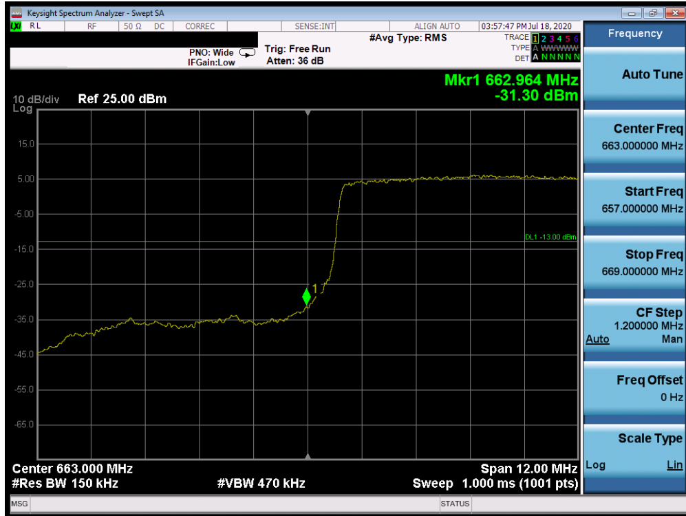
Plot 7-318. Lower Band Edge Plot (Band 71 - 15.0MHz QPSK - Full RB Configuration)
