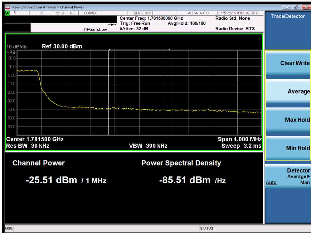
Plot 7-377. Upper Extended Band Edge Plot (Band 66 - 3.0MHz QPSK - Full RB Configuration)
