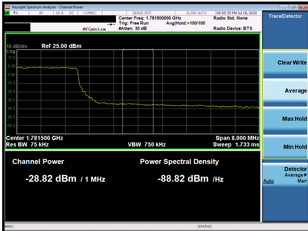
Plot 7-389. Upper Extended Band Edge Plot (Band 66 - 10.0MHz QPSK - Full RB Configuration)
