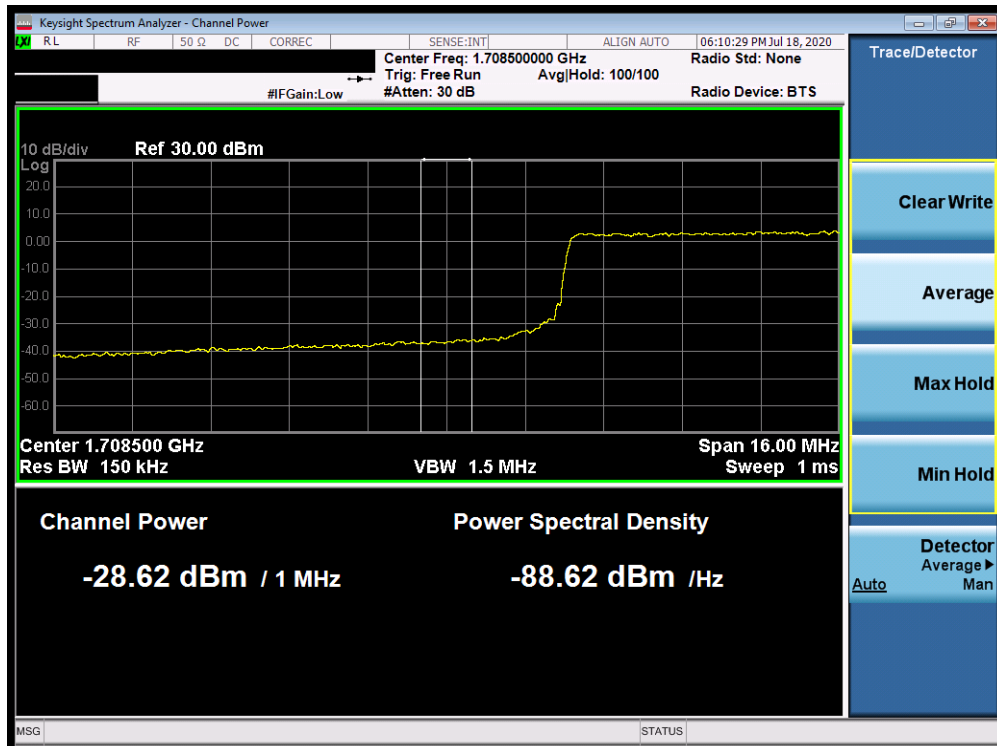
Plot 7-397. Lower Extended Band Edge Plot (Band 66/4 - 20.0MHz QPSK - Full RB Configuration)
