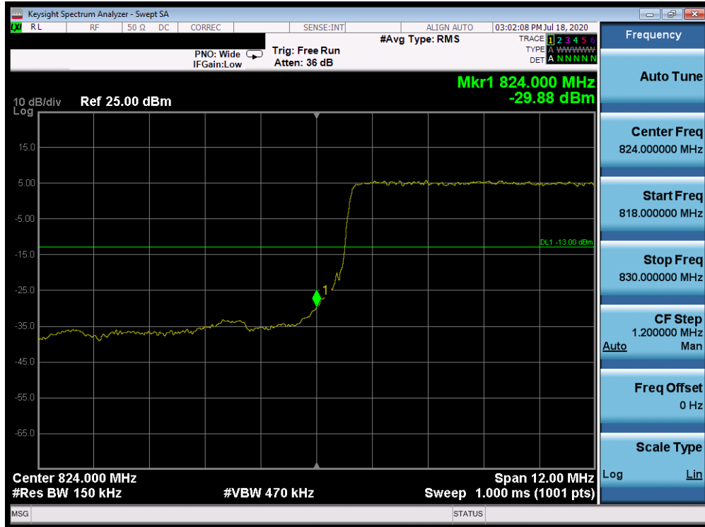
Plot 7-356. Lower Band Edge Plot (Band 26 - 15.0MHz QPSK - Full RB Configuration)
