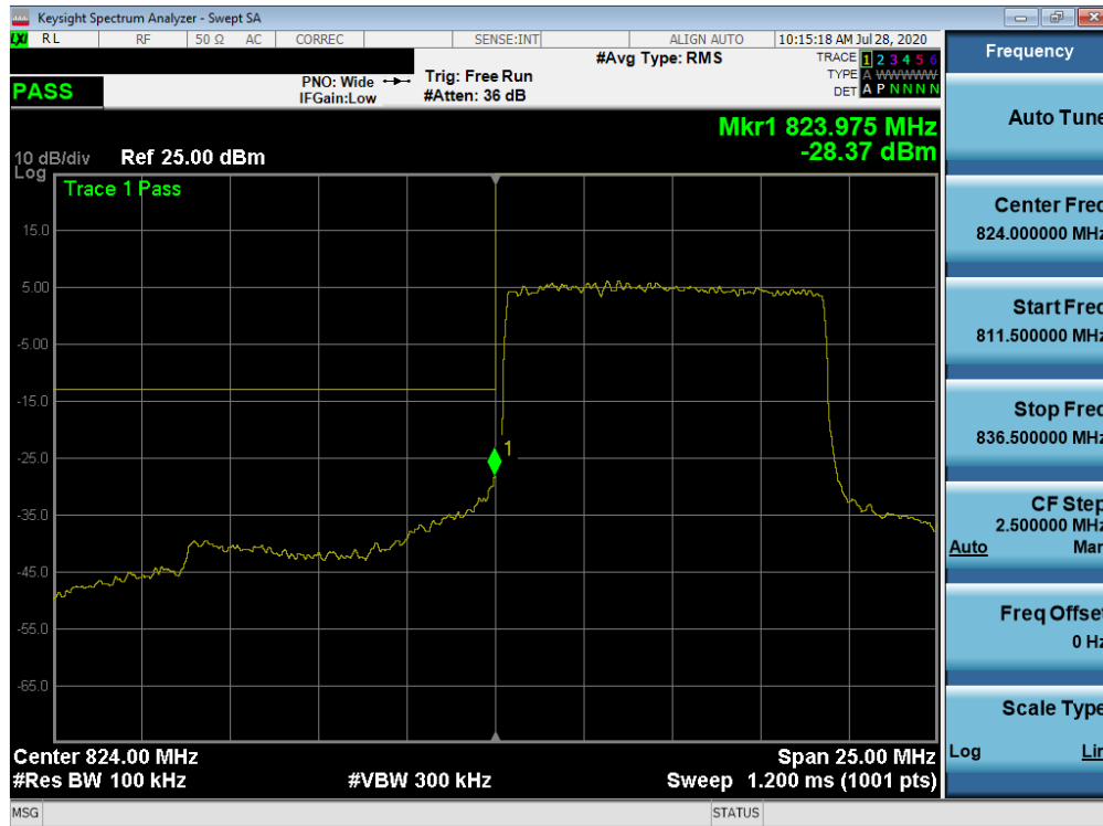
Plot 7-360. Lower Band Edge Plot (NR Band n5 - 10.0MHz - Full RB)
