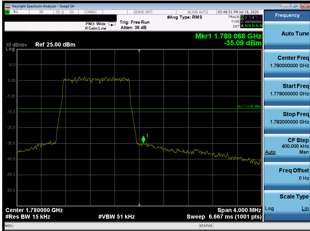
Plot 7-370. Upper Band Edge Plot (Band 66 - 1.4MHz QPSK - Full RB Configuration)
