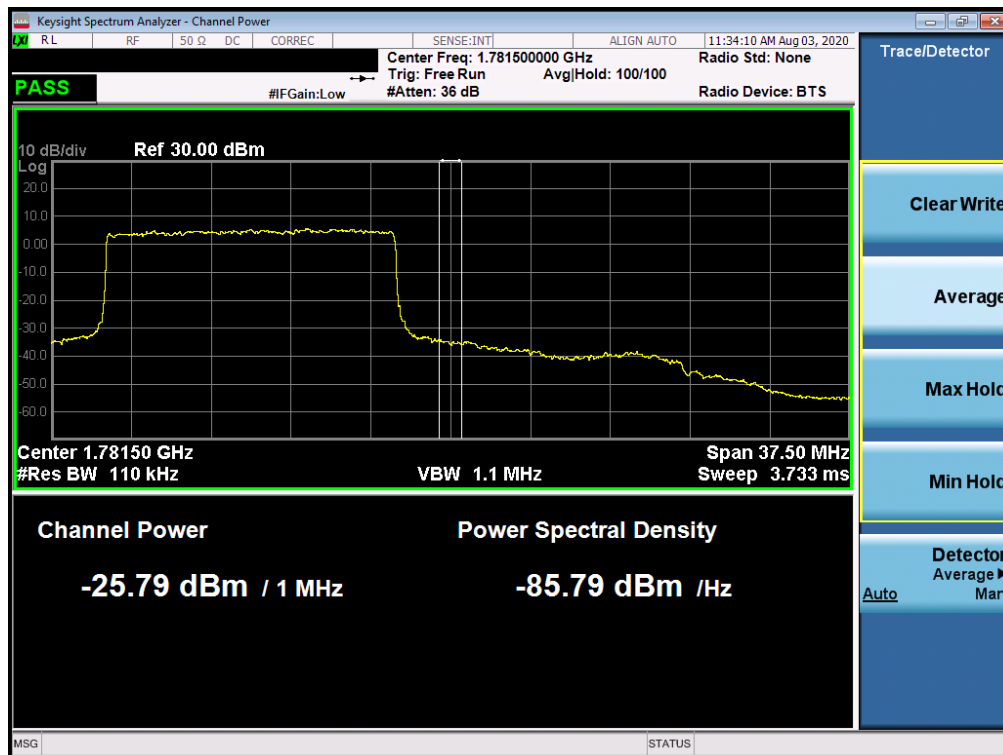
Plot 7-413. Upper Extended Band Edge Plot (NR Band n66 – 15.0MHz - Full RB)
