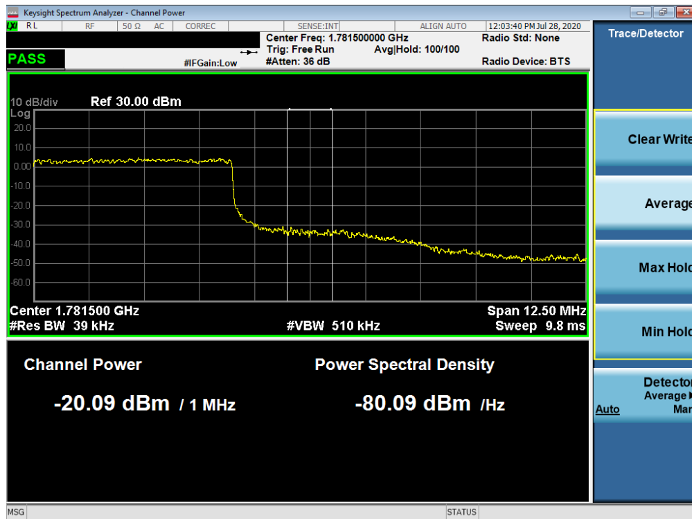
Plot 7-405. Upper Extended Band Edge Plot (NR Band n66 – 5.0MHz - Full RB)
