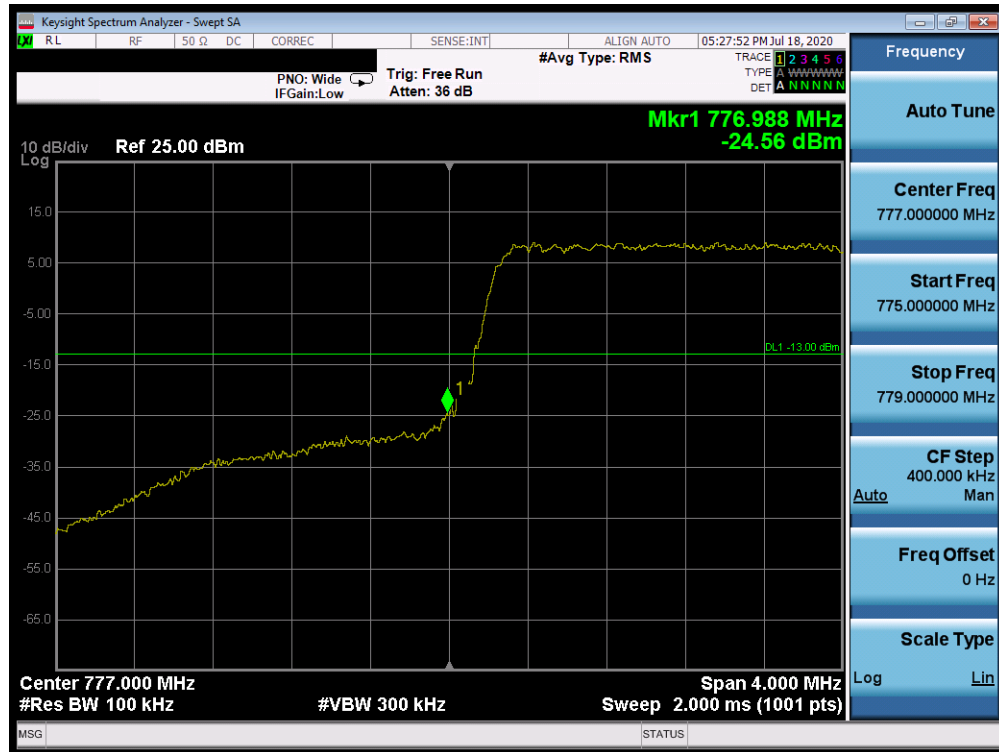
Plot 7-340. Lower Band Edge Plot (Band 13 - 5.0MHz QPSK - Full RB Configuration)
