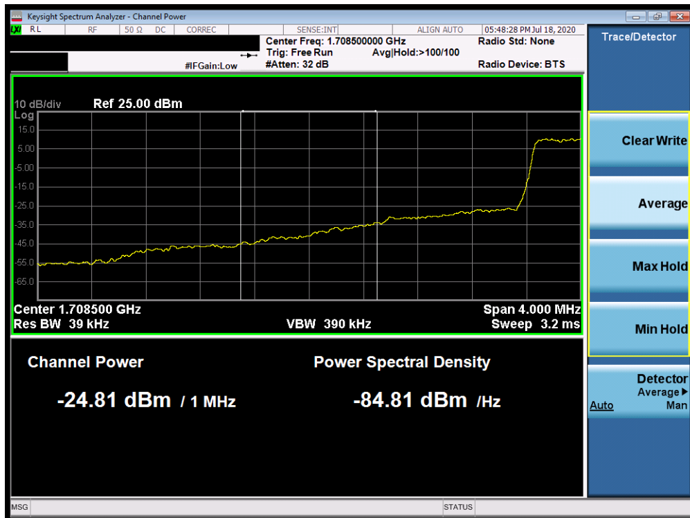
Plot 7-367. Lower Extended Band Edge Plot (Band 66/4 - 1.4MHz QPSK - Full RB Configuration)
