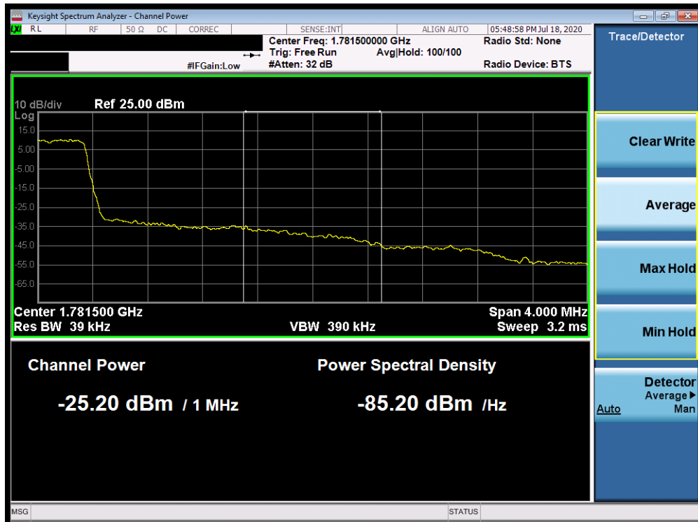
Plot 7-371. Upper Extended Band Edge Plot (Band 66 - 1.4MHz QPSK - Full RB Configuration)
