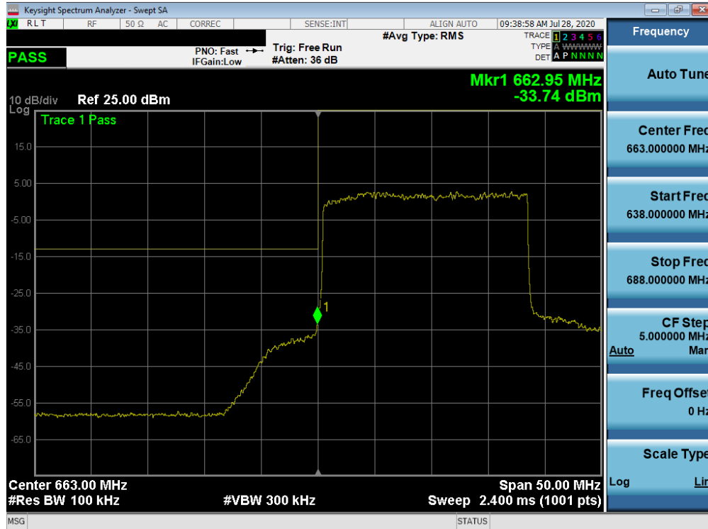
Plot 7-328. Lower Band Edge Plot (NR Band n71 - 20.0MHz - Full RB)
