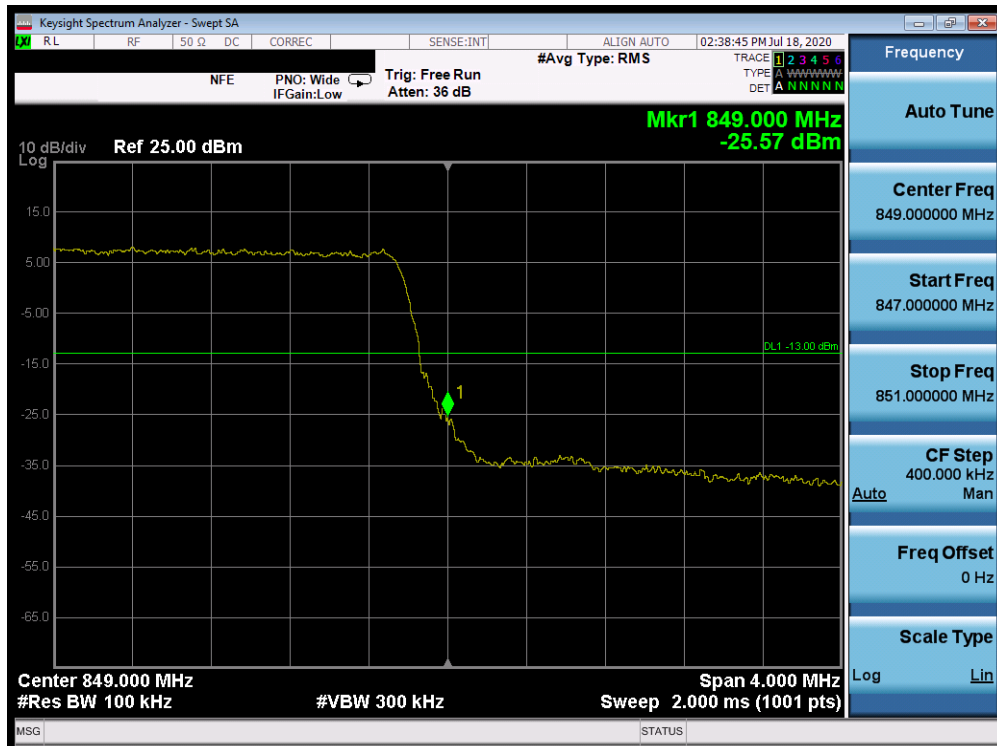
Plot 7-353. Upper Band Edge Plot (Band 26/5 - 5.0MHz QPSK - Full RB Configuration)
