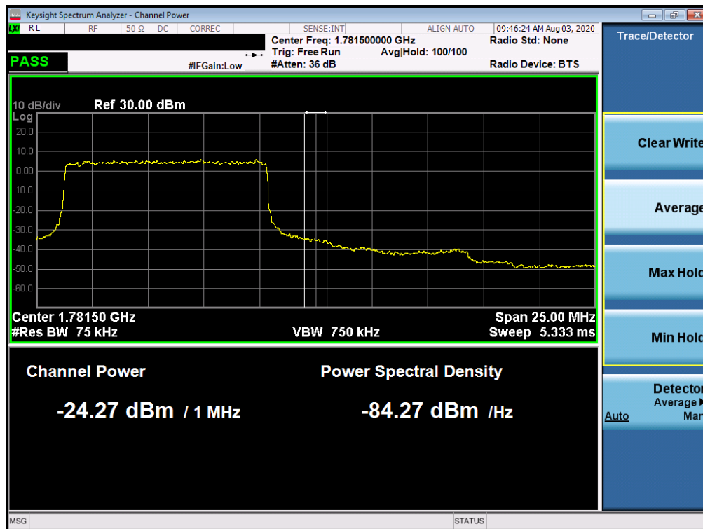
Plot 7-409. Upper Extended Band Edge Plot (NR Band n66 – 10.0MHz - Full RB)
