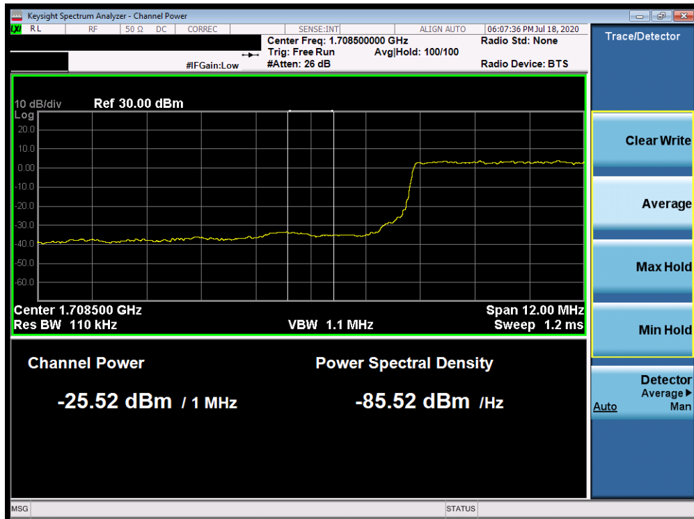
Plot 7-391. Lower Extended Band Edge Plot (Band 66/4 - 15.0MHz QPSK - Full RB Configuration)
