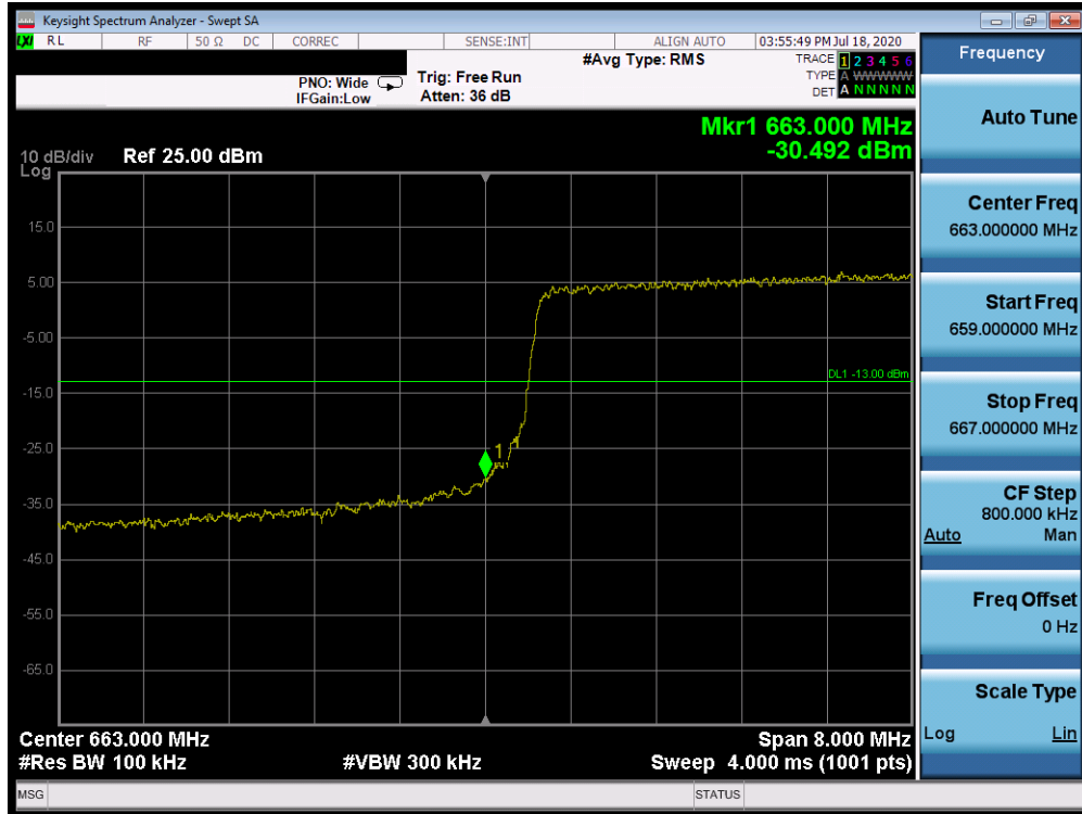
Plot 7-316. Lower Band Edge Plot (Band 71 - 10.0MHz QPSK - Full RB Configuration)
