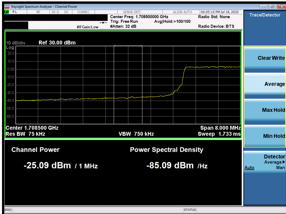
Plot 7-385. Lower Extended Band Edge Plot (Band 66/4 - 10.0MHz QPSK - Full RB Configuration)
