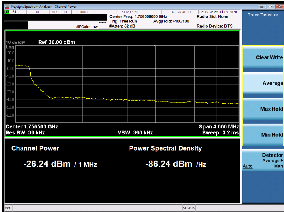
Plot 7-381. Upper Extended Band Edge Plot (Band 4 - 5.0MHz QPSK - Full RB Configuration)
