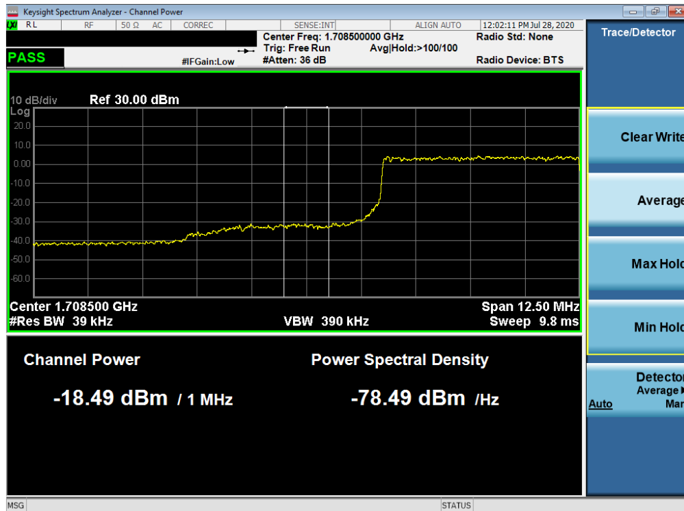
Plot 7-403. Lower Extended Band Edge Plot (NR Band n66 – 5.0MHz - Full RB)
