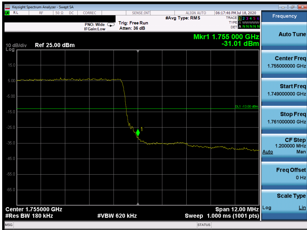
Plot 7-392. Upper Band Edge Plot (Band 4 - 15.0MHz QPSK - Full RB Configuration)
