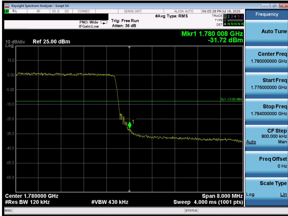
Plot 7-388. Upper Band Edge Plot (Band 66 - 10.0MHz QPSK - Full RB Configuration)
