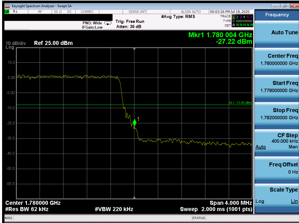
Plot 7-382. Upper Band Edge Plot (Band 66 - 5.0MHz QPSK - Full RB Configuration)
