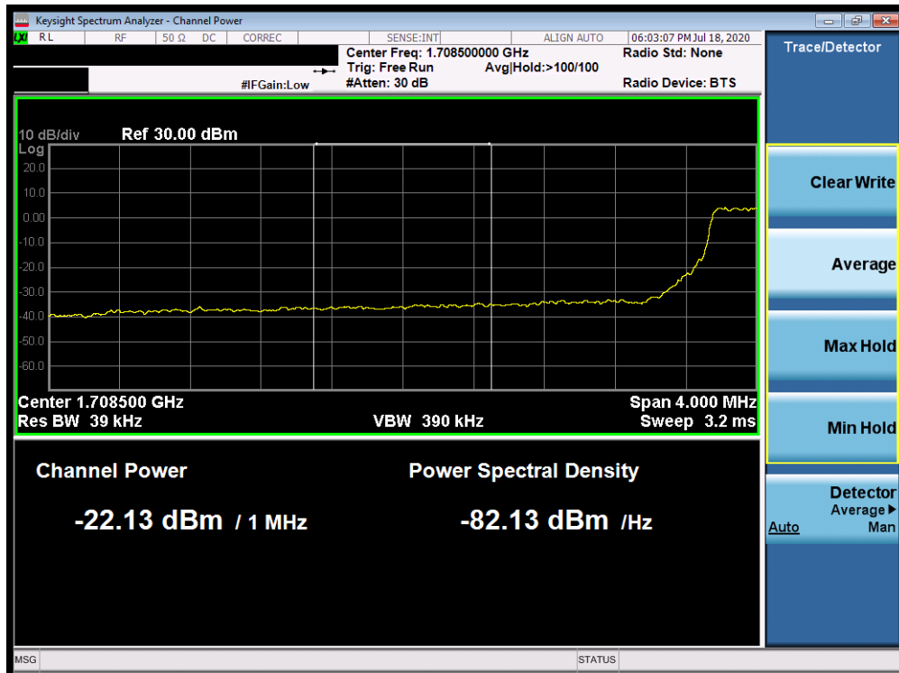
Plot 7-379. Lower Extended Band Edge Plot (Band 66/4 - 5.0MHz QPSK - Full RB Configuration)
