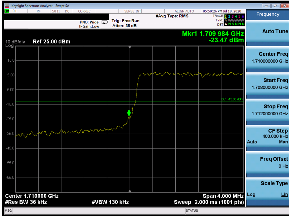
Plot 7-372. Lower Band Edge Plot (Band 66/4 - 3.0MHz QPSK - Full RB Configuration)
