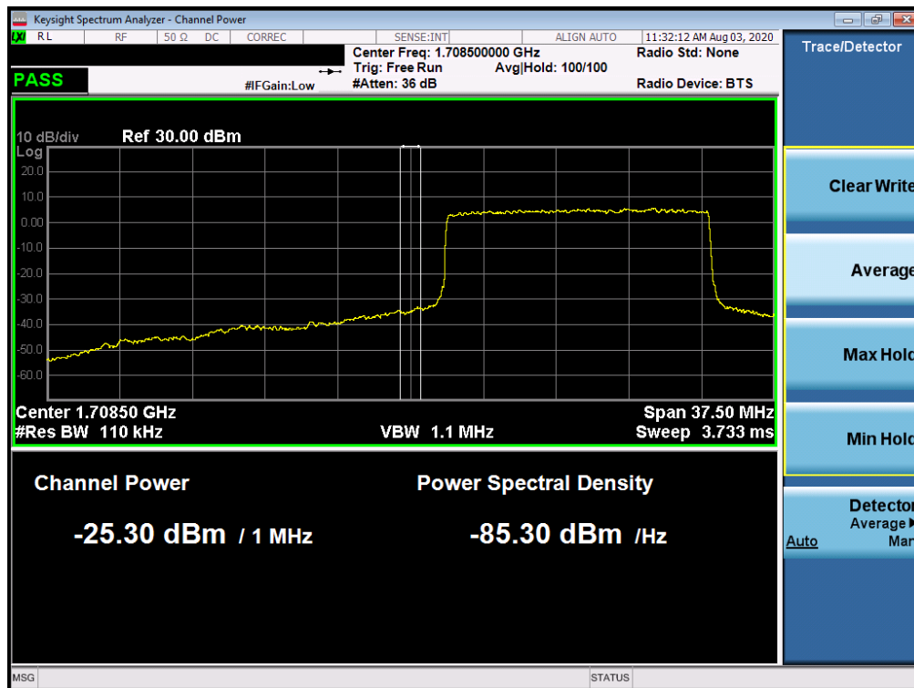
Plot 7-411. Lower Extended Band Edge Plot (NR Band n66 – 15.0MHz - Full RB)
