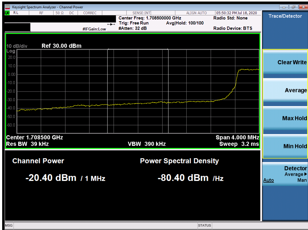
Plot 7-373. Lower Extended Band Edge Plot (Band 66/4 - 3.0MHz QPSK - Full RB Configuration)
