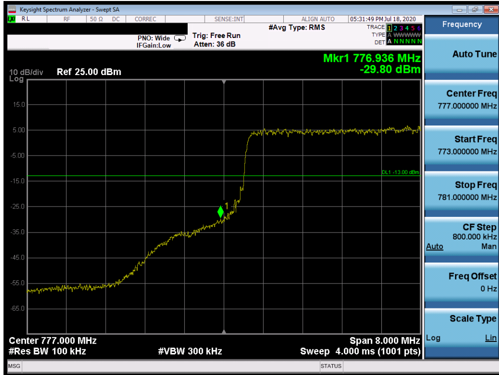
Plot 7-344. Lower Band Edge Plot (Band 13 - 10.0MHz QPSK - Full RB Configuration)
