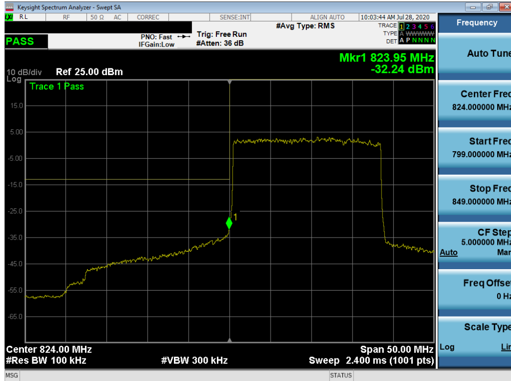
Plot 7-364. Lower Band Edge Plot (NR Band n5 - 20.0MHz - Full RB)
