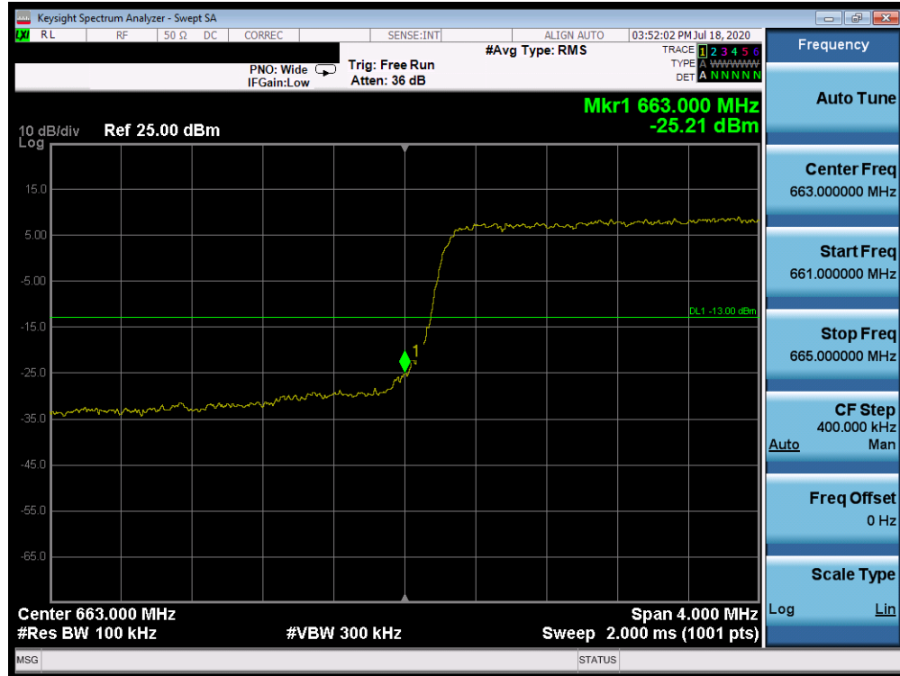
Plot 7-314. Lower Band Edge Plot (Band 71 – 5.0MHz QPSK - Full RB Configuration)
