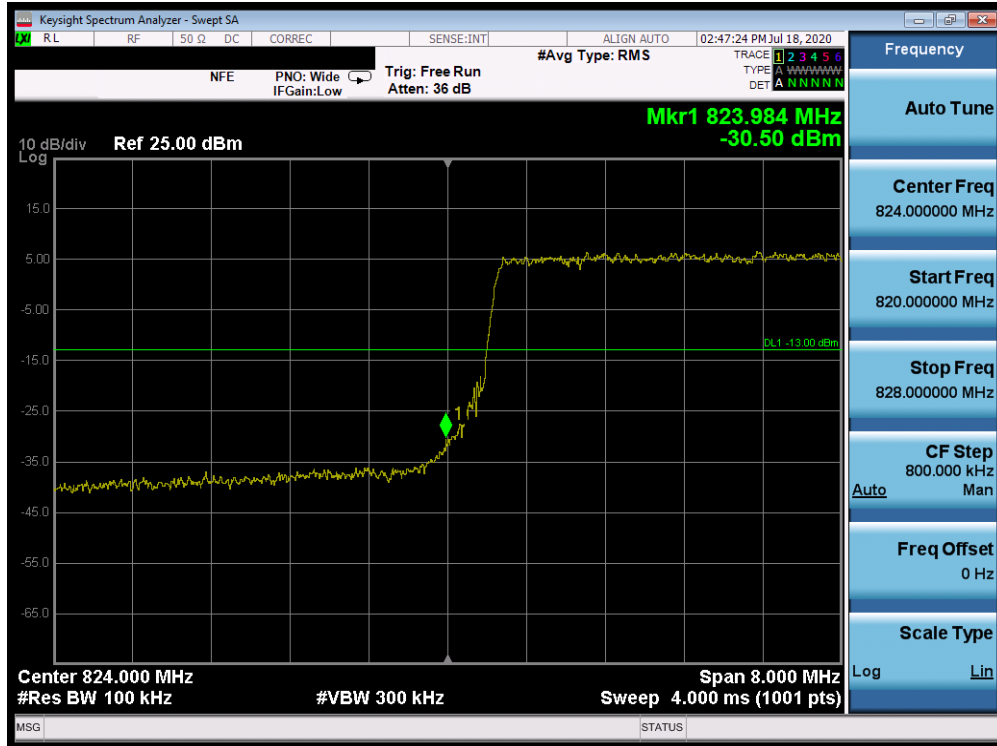
Plot 7-354. Lower Band Edge Plot (Band 26/5 - 10.0MHz QPSK - Full RB Configuration)
