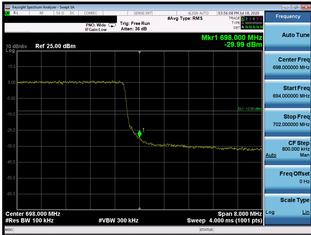
Plot 7-317. Upper Band Edge Plot (Band 71 - 10.0MHz QPSK - Full RB Configuration)
