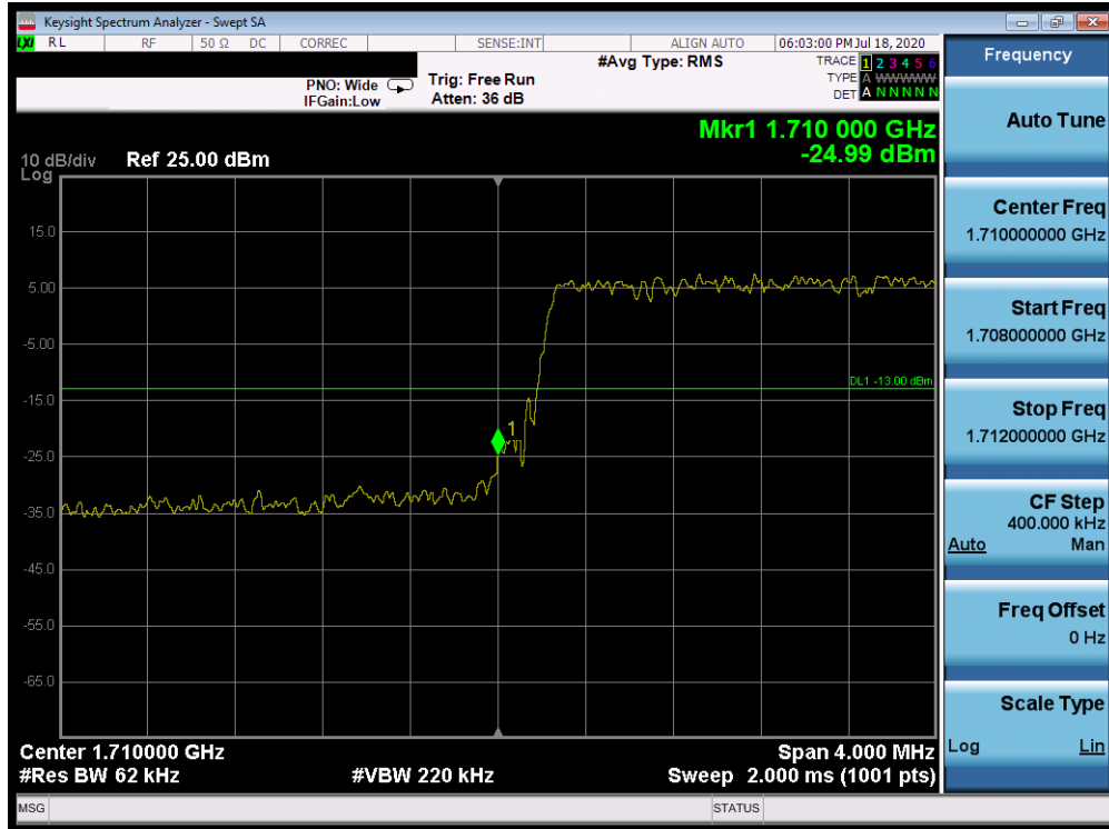
Plot 7-378. Lower Band Edge Plot (Band 66/4 - 5.0MHz QPSK - Full RB Configuration)
