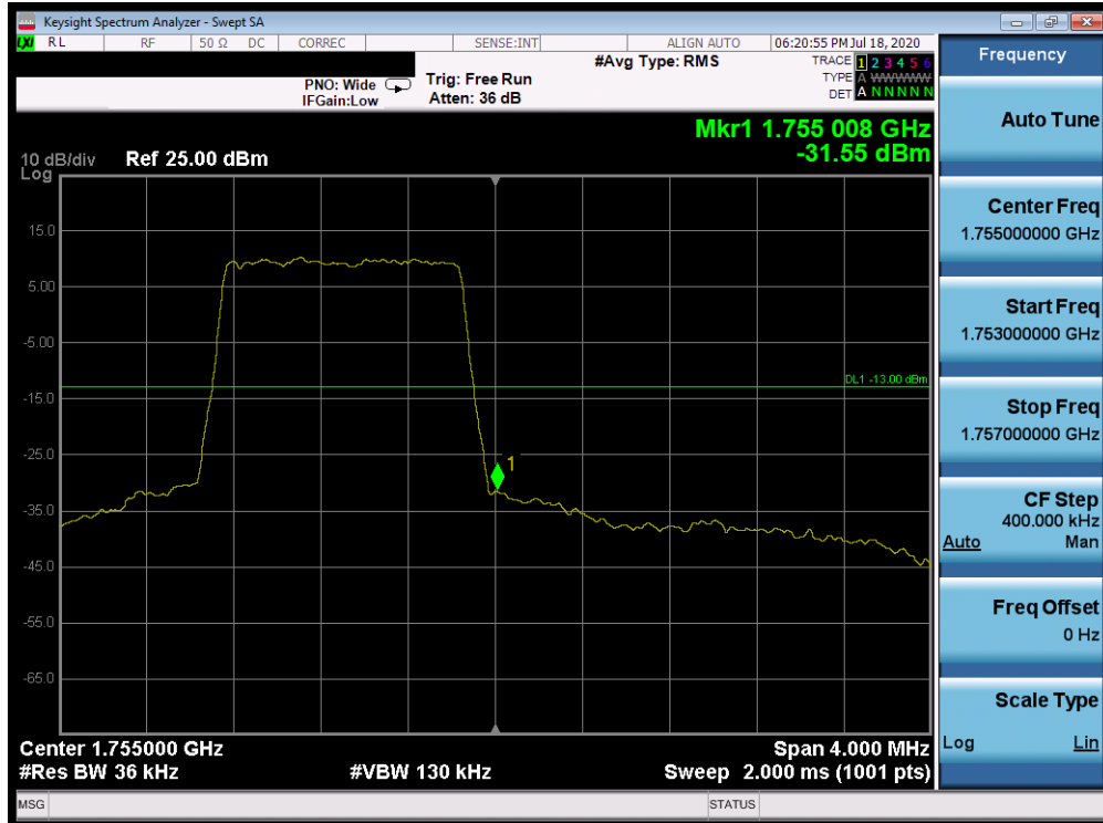
Plot 7-368. Upper Band Edge Plot (Band 4 - 1.4MHz QPSK - Full RB Configuration)
