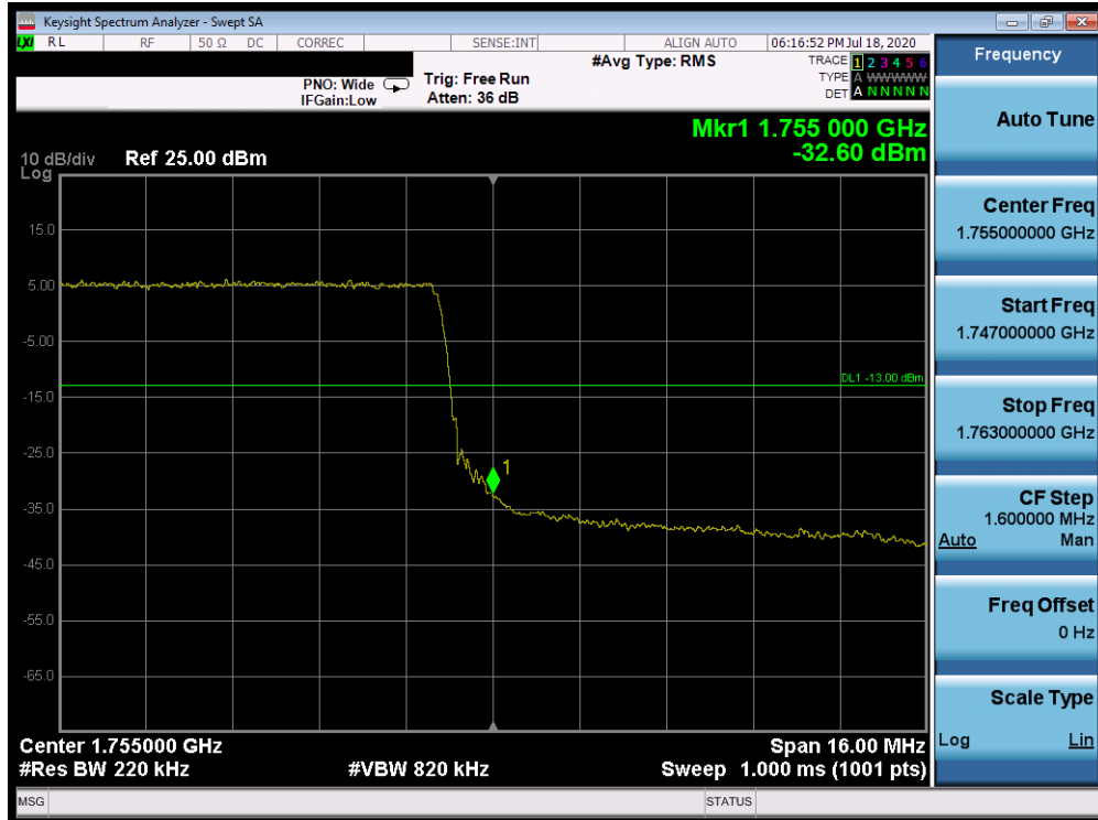
Plot 7-398. Upper Band Edge Plot (Band 4 - 20.0MHz QPSK - Full RB Configuration)
