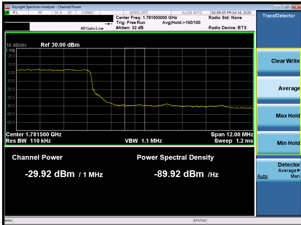
Plot 7-395. Upper Extended Band Edge Plot (Band 66 - 15.0MHz QPSK - Full RB Configuration)
