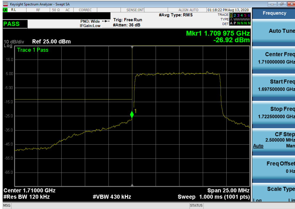
Plot 7-406. Lower Band Edge Plot (NR Band n66 – 10.0MHz - Full RB)
