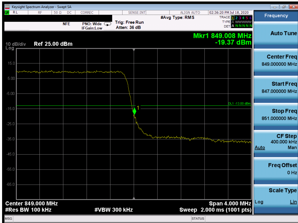
Plot 7-351. Upper Band Edge Plot (Band 26/5 - 3.0MHz QPSK - Full RB Configuration)
