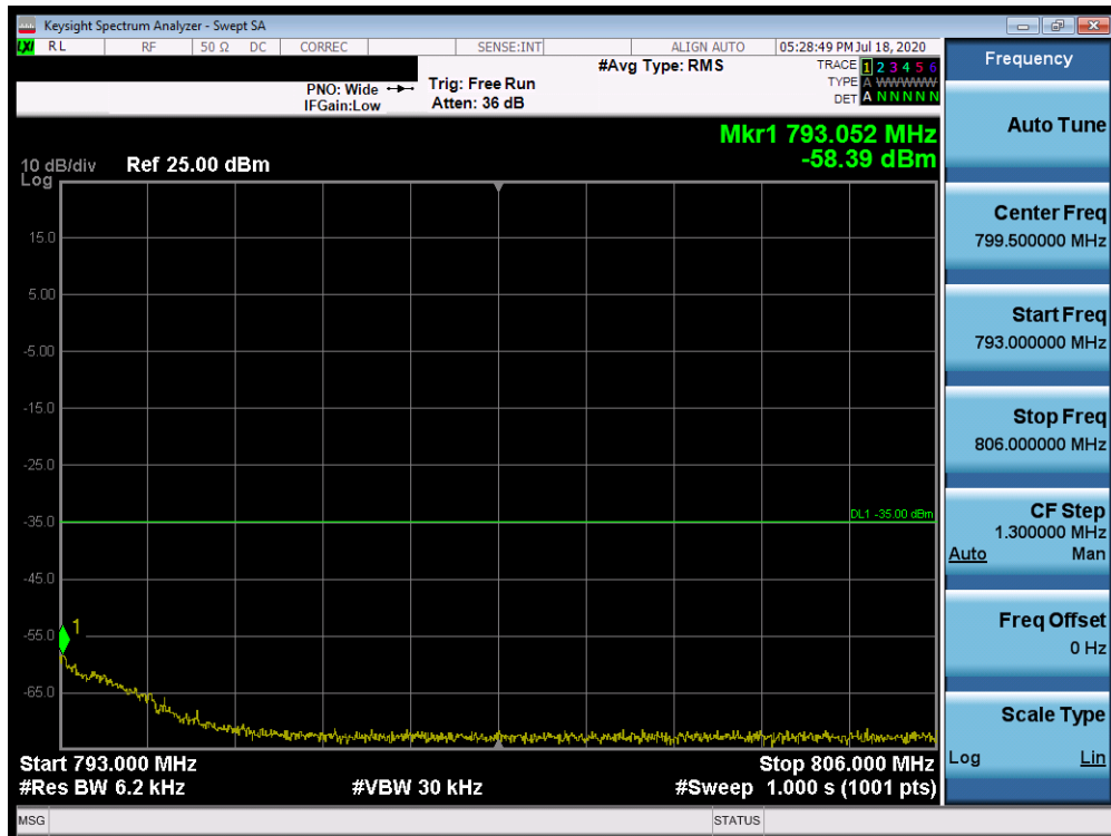
Plot 7-343. Upper Emission Mask Plot (Band 13 - 5.0MHz QPSK - Full RB Configuration)
