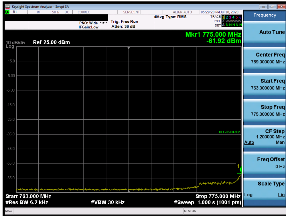
Plot 7-341. Lower Emission Mask Plot (Band 13 - 5.0MHz QPSK - Full RB Configuration)
