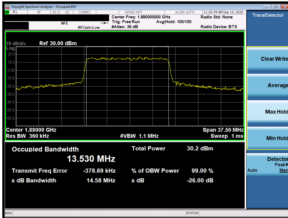
Plot 7-154. Occupied Bandwidth Plot (NR Band n25/2 - 15.0MHz CP-OFDM 16QAM - Full RB)
