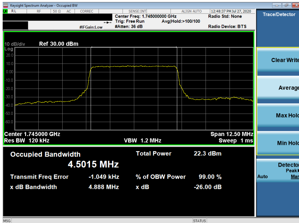
Plot 7-107. Occupied Bandwidth Plot (NR Band n66 - 5.0MHz CP-OFDM 64QAM - Full RB)
