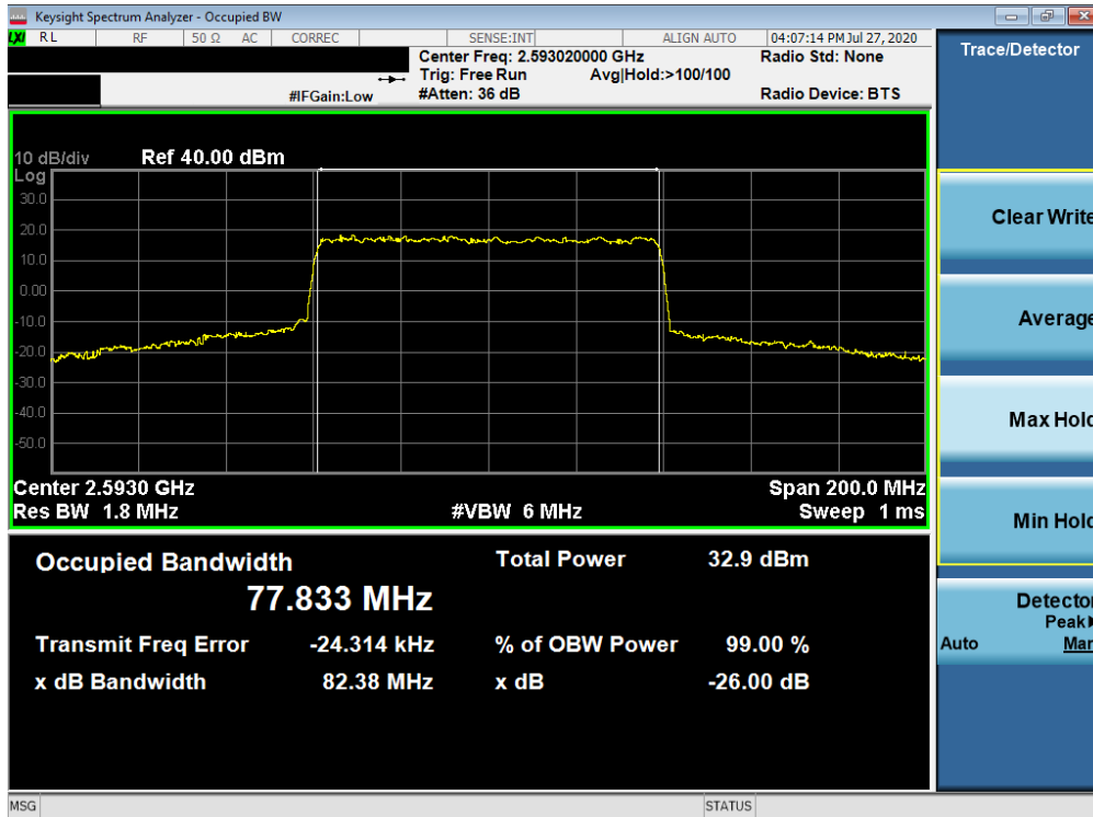
Plot 7-195. Occupied Bandwidth Plot (NR Band n41 - 80MHz CP-OFDM QPSK - Full RB)
