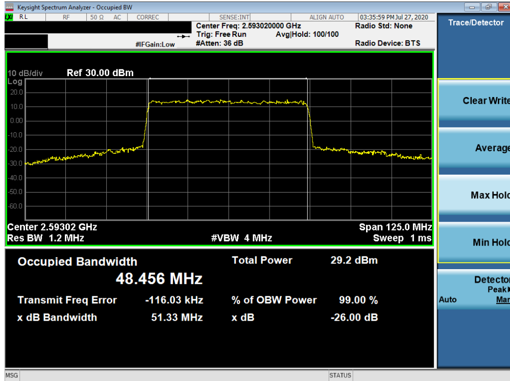
Plot 7-188. Occupied Bandwidth Plot (NR Band n41 - 50MHz CP-OFDM 256-QAM - Full RB)
