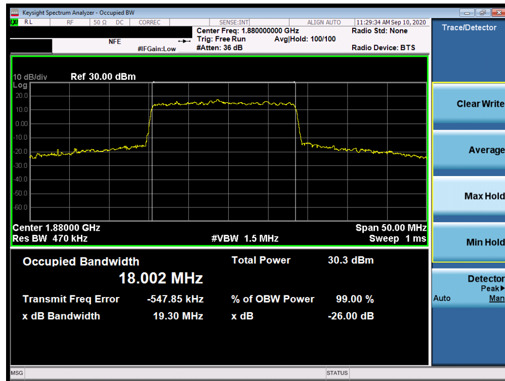
Plot 7-161. Occupied Bandwidth Plot (NR Band n25/2 - 20.0MHz CP-OFDM 256QAM - Full RB)
