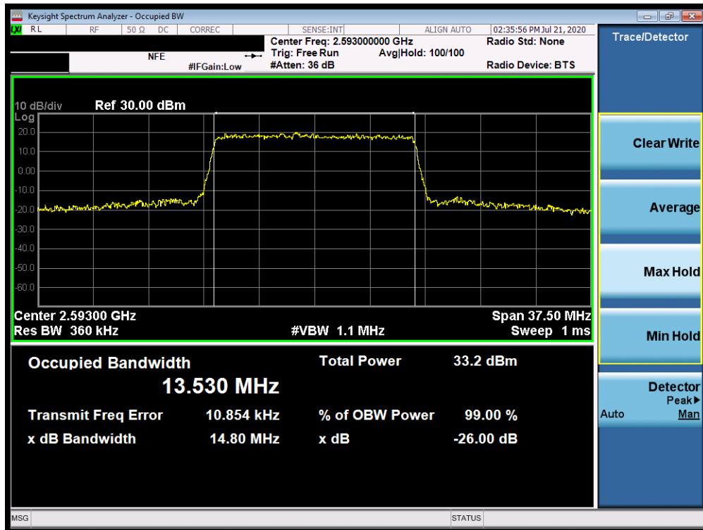
Plot 7-169. Occupied Bandwidth Plot (Band 41 - 15.0MHz 16-QAM - Full RB Configuration)
