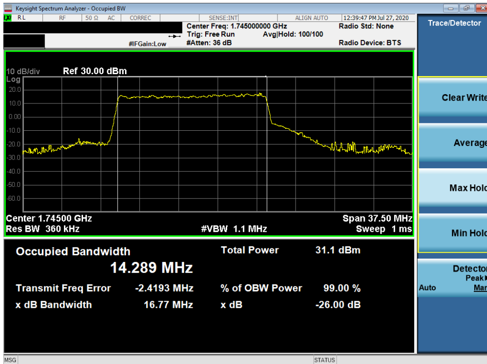
Plot 7-115. Occupied Bandwidth Plot (NR Band n66 - 15.0MHz CP-OFDM QPSK - Full RB)
