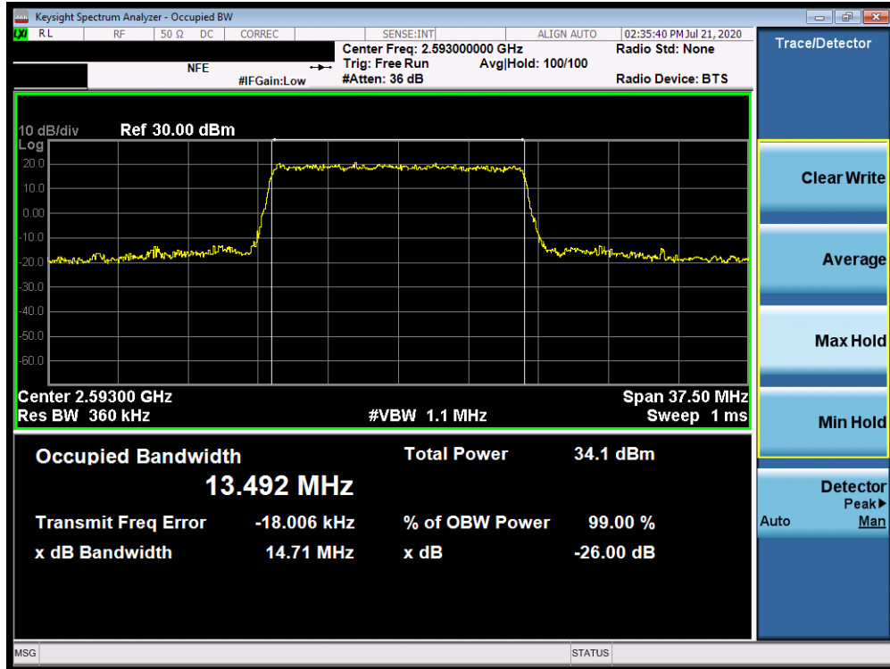
Plot 7-168. Occupied Bandwidth Plot (Band 41 - 15.0MHz QPSK - Full RB Configuration)
