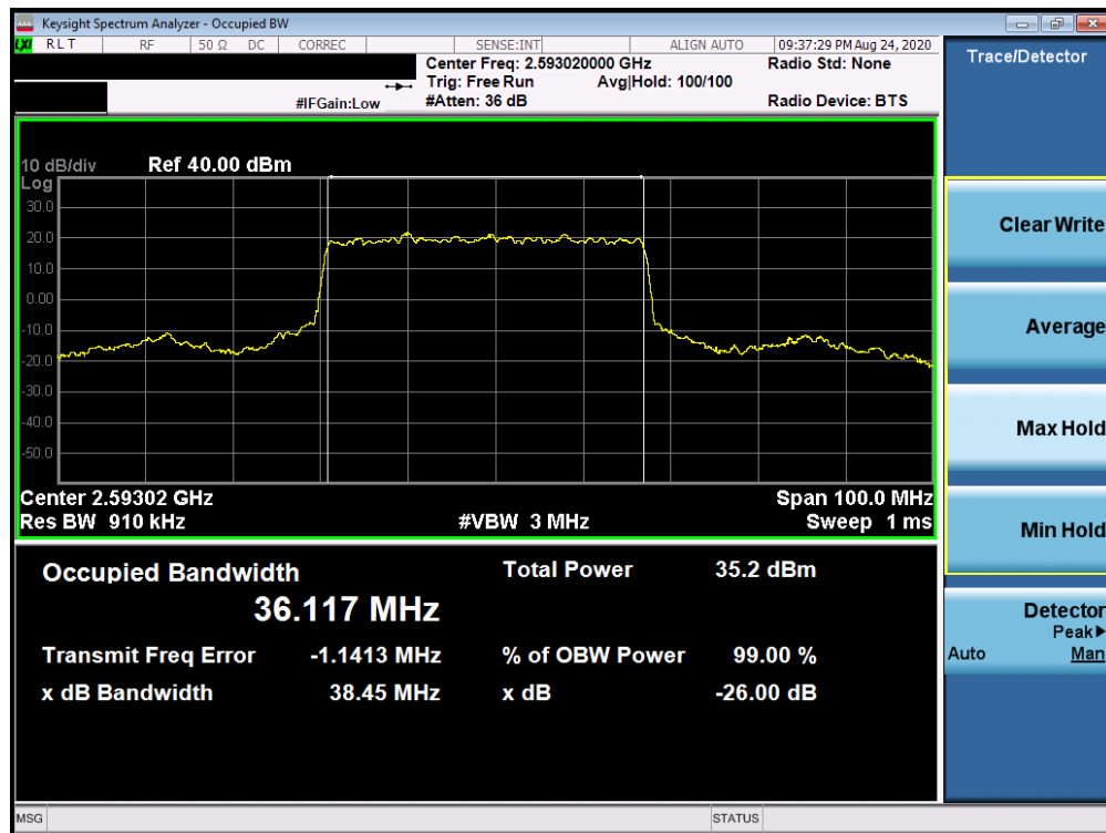
Plot 7-179. Occupied Bandwidth Plot (NR Band n41 - 40MHz DFT-s-OFDM BPSK - Full RB)
