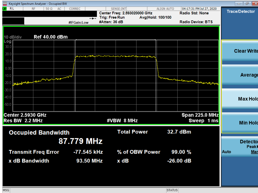
Plot 7-200. Occupied Bandwidth Plot (NR Band n41 - 90MHz CP-OFDM QPSK - Full RB)
