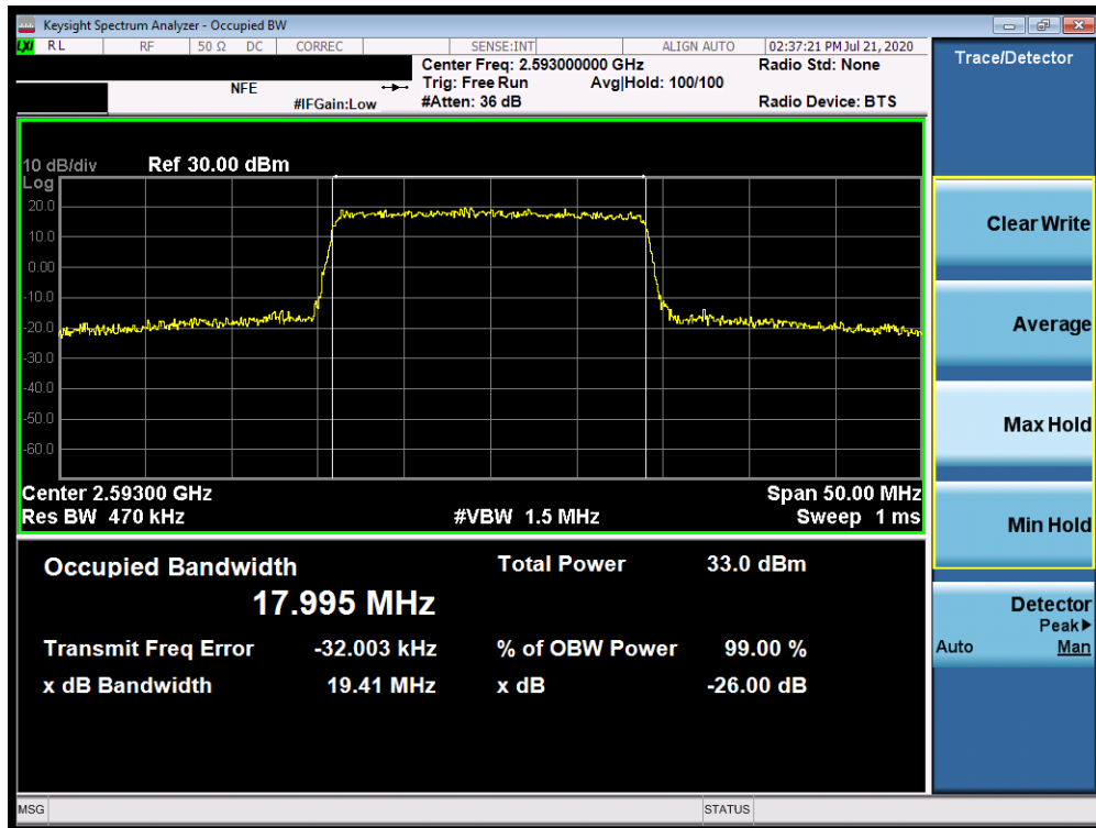
Plot 7-173. Occupied Bandwidth Plot (Band 41 - 20.0MHz 64-QAM - Full RB Configuration)
