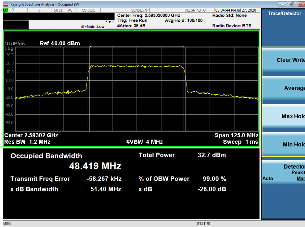
Plot 7-186. Occupied Bandwidth Plot (NR Band n41 - 50MHz CP-OFDM 16-QAM - Full RB)
