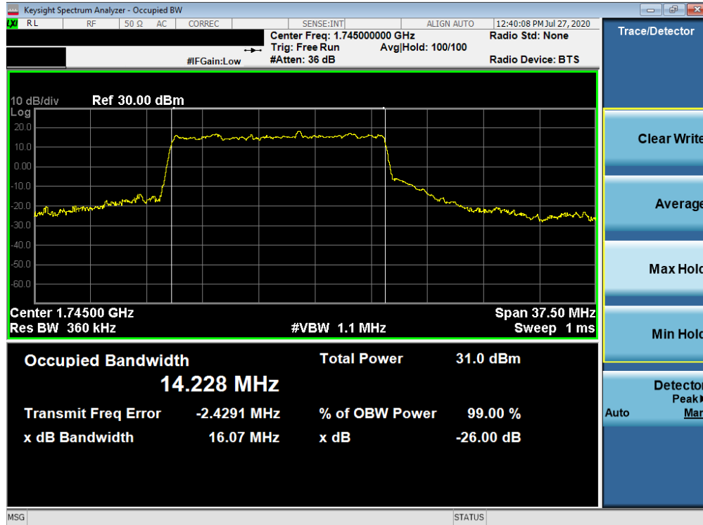
Plot 7-116. Occupied Bandwidth Plot (NR Band n66 - 15.0MHz CP-OFDM 16QAM - Full RB)
