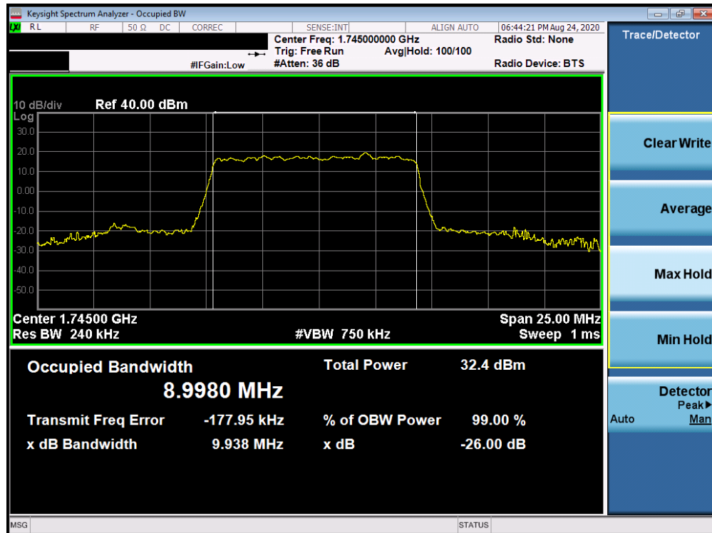
Plot 7-109. Occupied Bandwidth Plot (NR Band n66 - 10.0MHz DFT-s-OFDM BPSK - Full RB)
