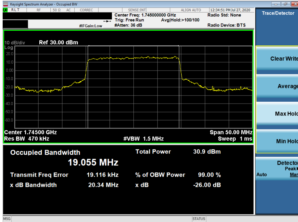
Plot 7-120. Occupied Bandwidth Plot (NR Band n66 - 20.0MHz CP-OFDM QPSK - Full RB)
