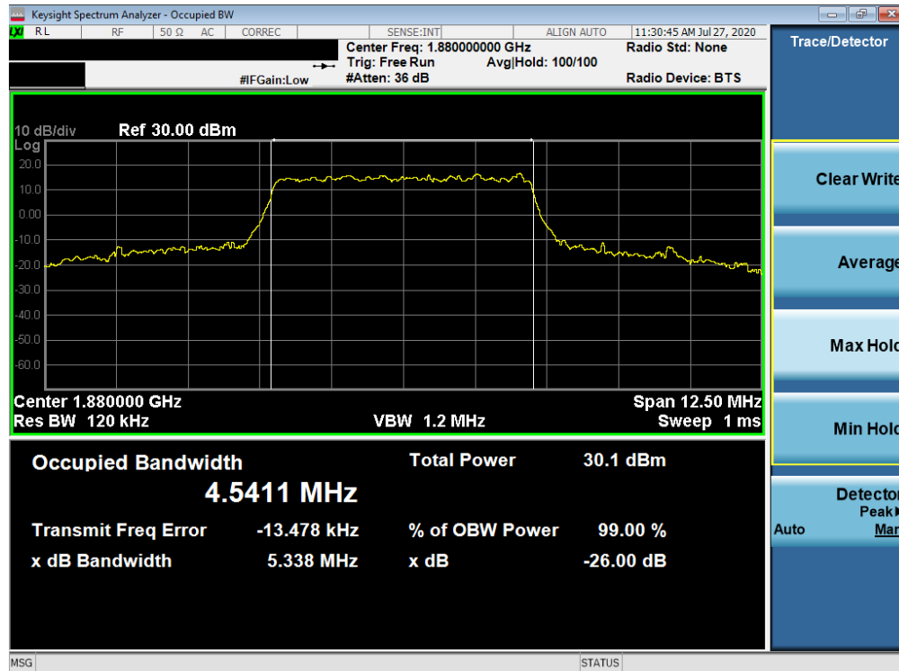
Plot 7-144. Occupied Bandwidth Plot (NR Band n25/2 - 5.0MHz CP-OFDM 16QAM - Full RB)
