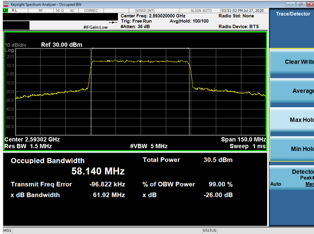
Plot 7-190. Occupied Bandwidth Plot (NR Band n41 - 60MHz CP-OFDM QPSK - Full RB)
