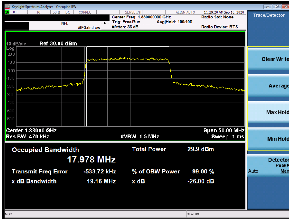
Plot 7-160. Occupied Bandwidth Plot (NR Band n25/2 - 20.0MHz CP-OFDM 64QAM - Full RB)
