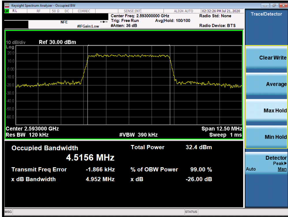
Plot 7-164. Occupied Bandwidth Plot (Band 41 – 5.0MHz 64-QAM - Full RB Configuration)
