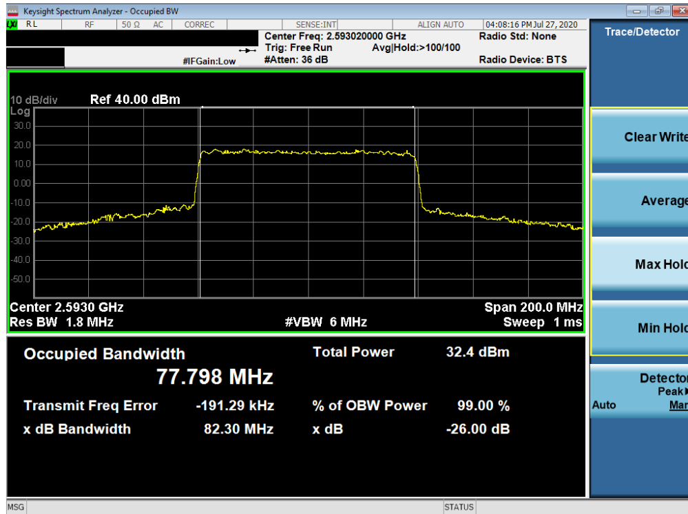
Plot 7-197. Occupied Bandwidth Plot (NR Band n41 - 80MHz CP-OFDM 64-QAM - Full RB)
