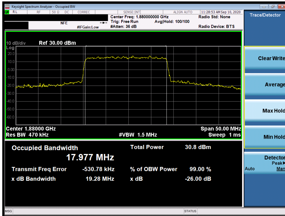
Plot 7-158. Occupied Bandwidth Plot (NR Band n25/2 - 20.0MHz CP-OFDM QPSK - Full RB)
