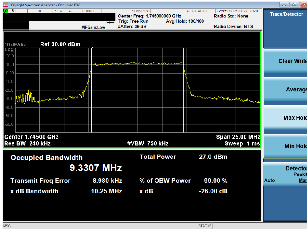
Plot 7-113. Occupied Bandwidth Plot (NR Band n66 - 10.0MHz CP-OFDM 256QAM - Full RB)
