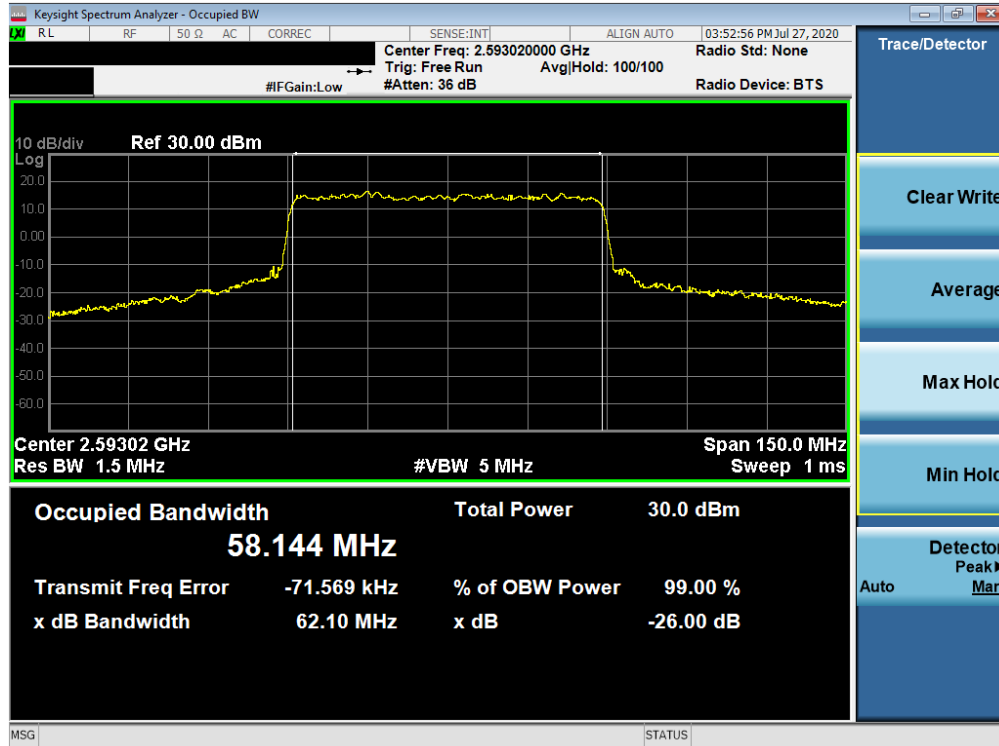
Plot 7-192. Occupied Bandwidth Plot (NR Band n41 - 60MHz CP-OFDM 64-QAM - Full RB)
