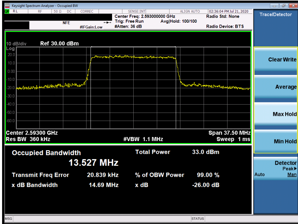
Plot 7-170. Occupied Bandwidth Plot (Band 41 - 15.0MHz 64-QAM - Full RB Configuration)
