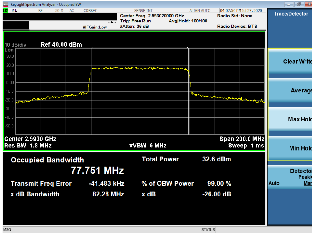
Plot 7-196. Occupied Bandwidth Plot (NR Band n41 - 80MHz CP-OFDM 16-QAM - Full RB)
