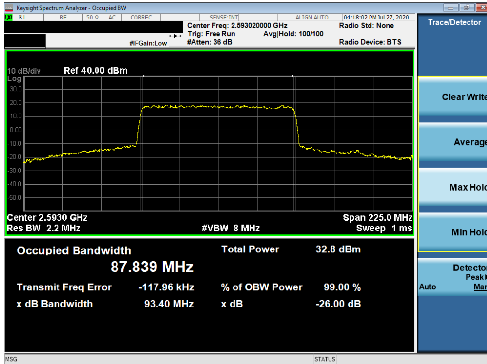
Plot 7-201. Occupied Bandwidth Plot (NR Band n41 - 90MHz CP-OFDM 16-QAM - Full RB)
