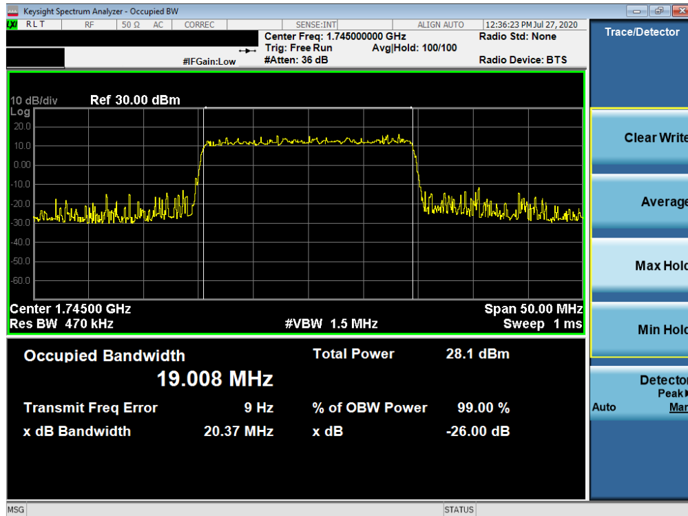
Plot 7-123. Occupied Bandwidth Plot (NR Band n66 - 20.0MHz CP-OFDM 256QAM - Full RB)
