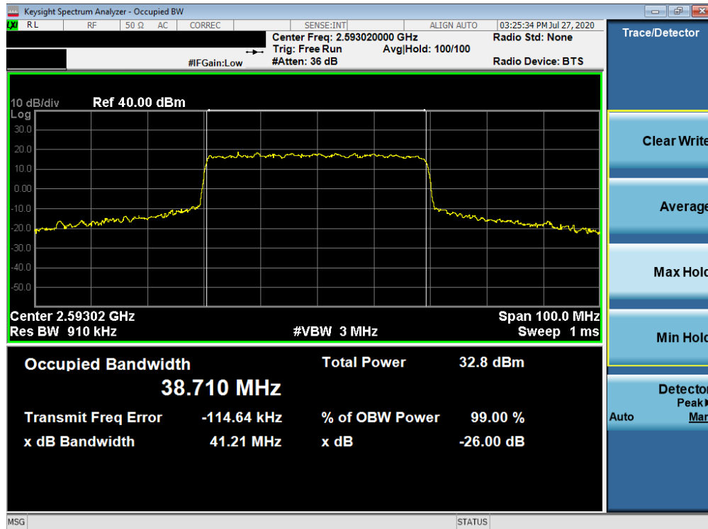
Plot 7-181. Occupied Bandwidth Plot (NR Band n41 - 40MHz CP-OFDM 16-QAM - Full RB)
