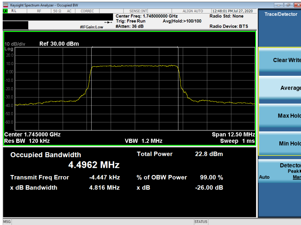
Plot 7-105. Occupied Bandwidth Plot (NR Band n66 - 5.0MHz CP-OFDM QPSK - Full RB)
