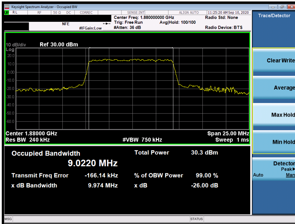
Plot 7-151. Occupied Bandwidth Plot (NR Band n25/2 - 10.0MHz CP-OFDM 256QAM - Full RB)
