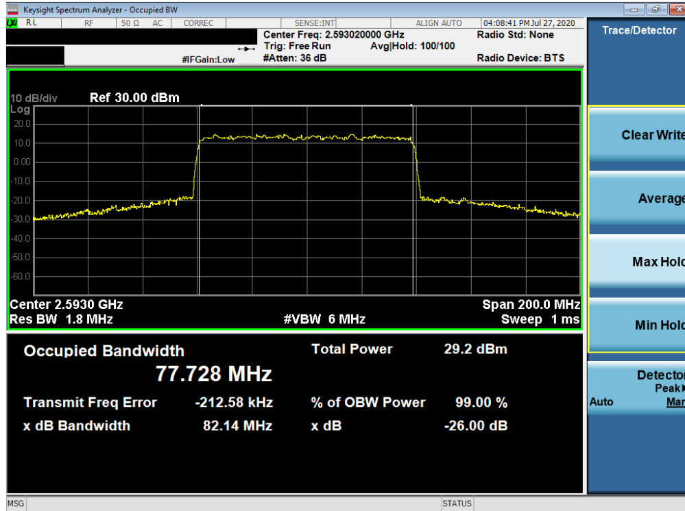
Plot 7-198. Occupied Bandwidth Plot (NR Band n41 - 80MHz CP-OFDM 256-QAM - Full RB)
