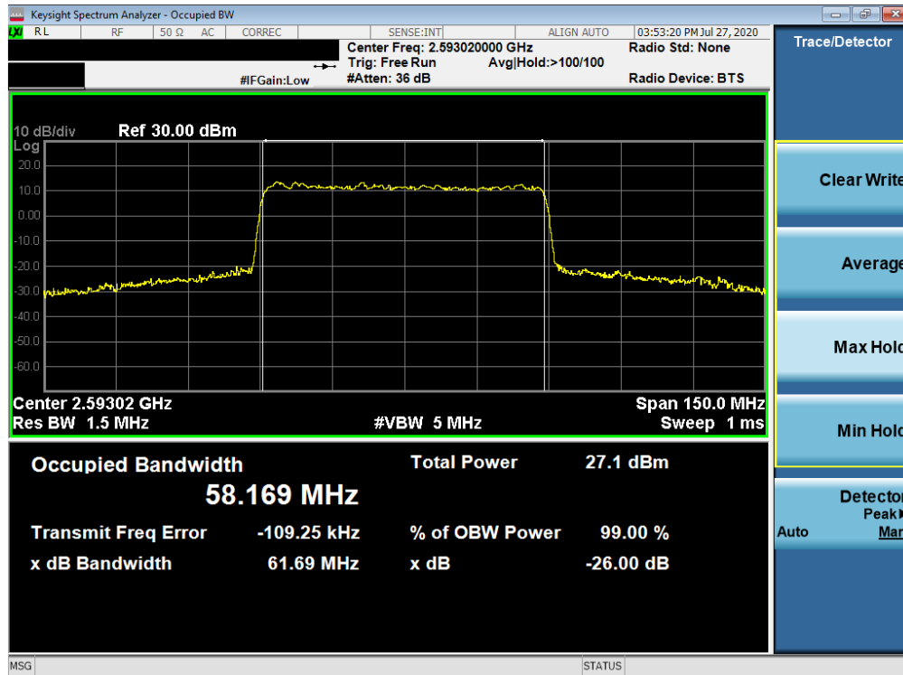
Plot 7-193. Occupied Bandwidth Plot (NR Band n41 - 60MHz CP-OFDM 256-QAM - Full RB)
