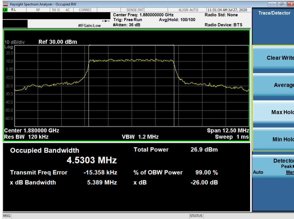
Plot 7-146. Occupied Bandwidth Plot (NR Band n25/2 - 5.0MHz CP-OFDM 256QAM - Full RB)
