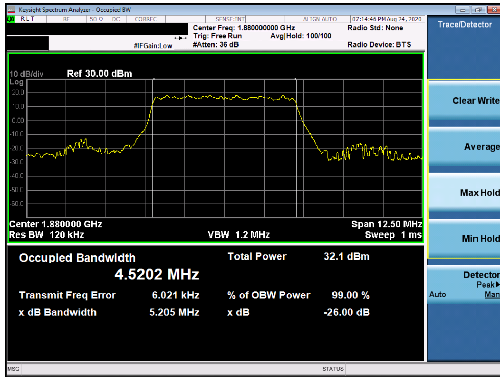
Plot 7-142. Occupied Bandwidth Plot (NR Band n25/2 - 5.0MHz DFT-s-OFDM BPSK - Full RB)
