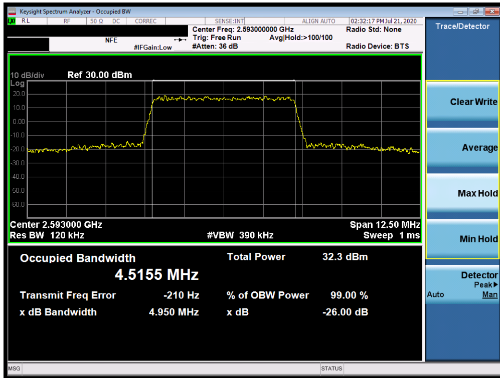
Plot 7-162. Occupied Bandwidth Plot (Band 41 – 5.0MHz QPSK - Full RB Configuration)
