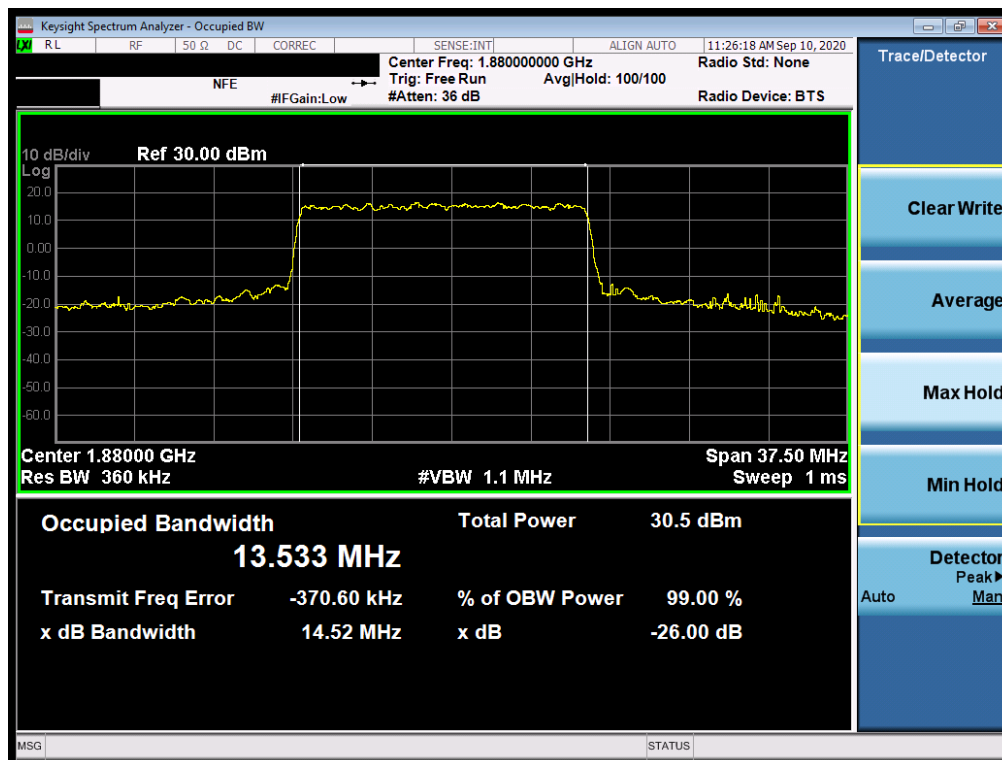
Plot 7-153. Occupied Bandwidth Plot (NR Band n25/2 - 15.0MHz CP-OFDM QPSK - Full RB)
