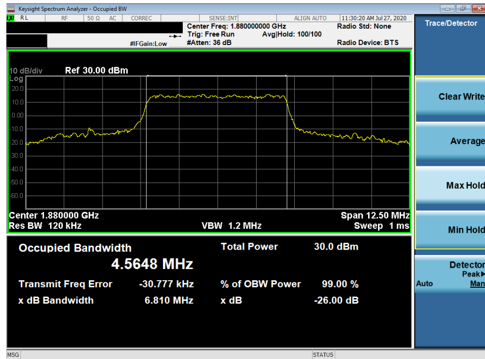
Plot 7-143. Occupied Bandwidth Plot (NR Band n25/2 - 5.0MHz CP-OFDM QPSK - Full RB)
