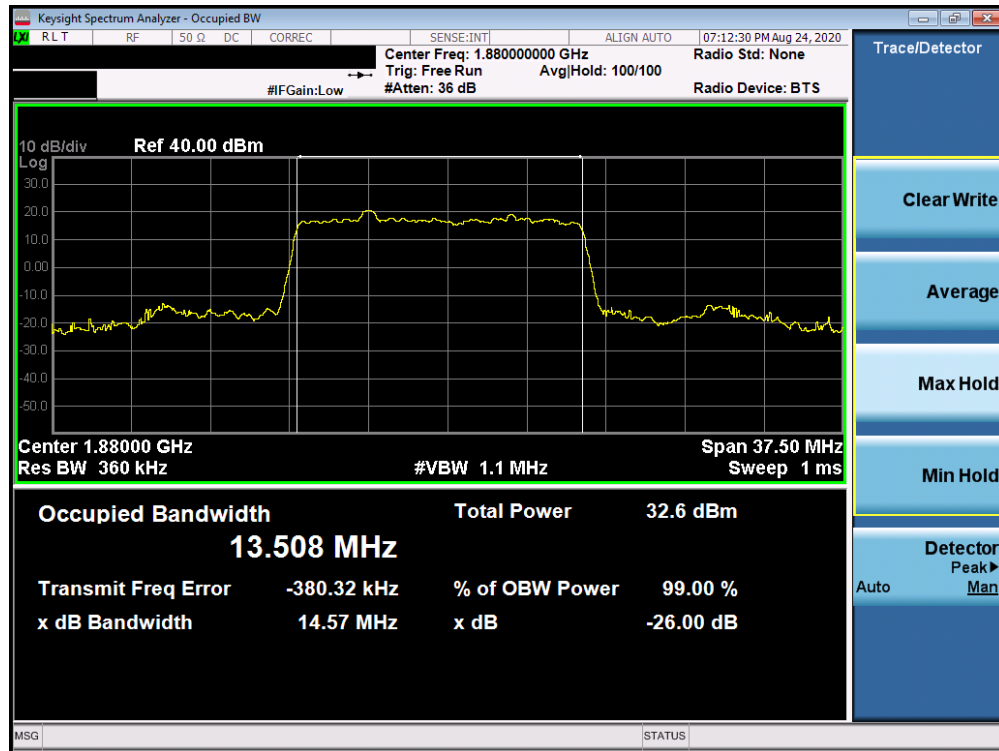
Plot 7-152. Occupied Bandwidth Plot (NR Band n25/2 - 15.0MHz DFT-s-OFDM BPSK - Full RB)
