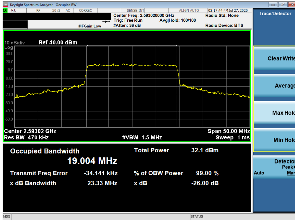
Plot 7-176. Occupied Bandwidth Plot (NR Band n41 - 20MHz CP-OFDM 16-QAM - Full RB)
