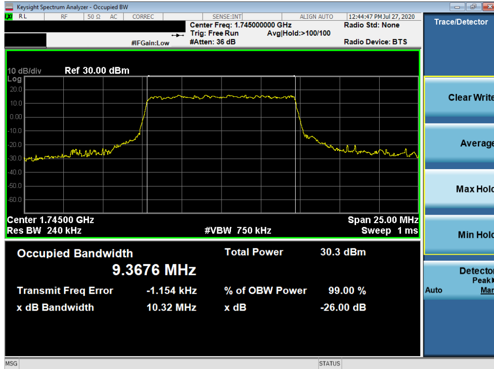
Plot 7-112. Occupied Bandwidth Plot (NR Band n66 - 10.0MHz CP-OFDM 64QAM - Full RB)
