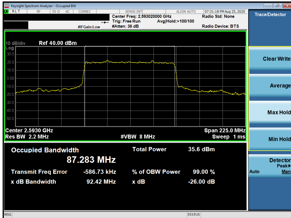
Plot 7-199. Occupied Bandwidth Plot (NR Band n41 - 90MHz DFT-s-OFDM BPSK - Full RB)
