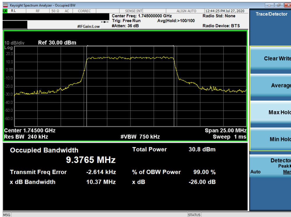
Plot 7-111. Occupied Bandwidth Plot (NR Band n66 - 10.0MHz CP-OFDM 16QAM - Full RB)
