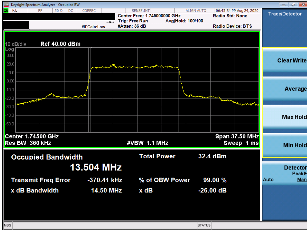
Plot 7-114. Occupied Bandwidth Plot (NR Band n66 - 15.0MHz DFT-s-OFDM BPSK - Full RB)
