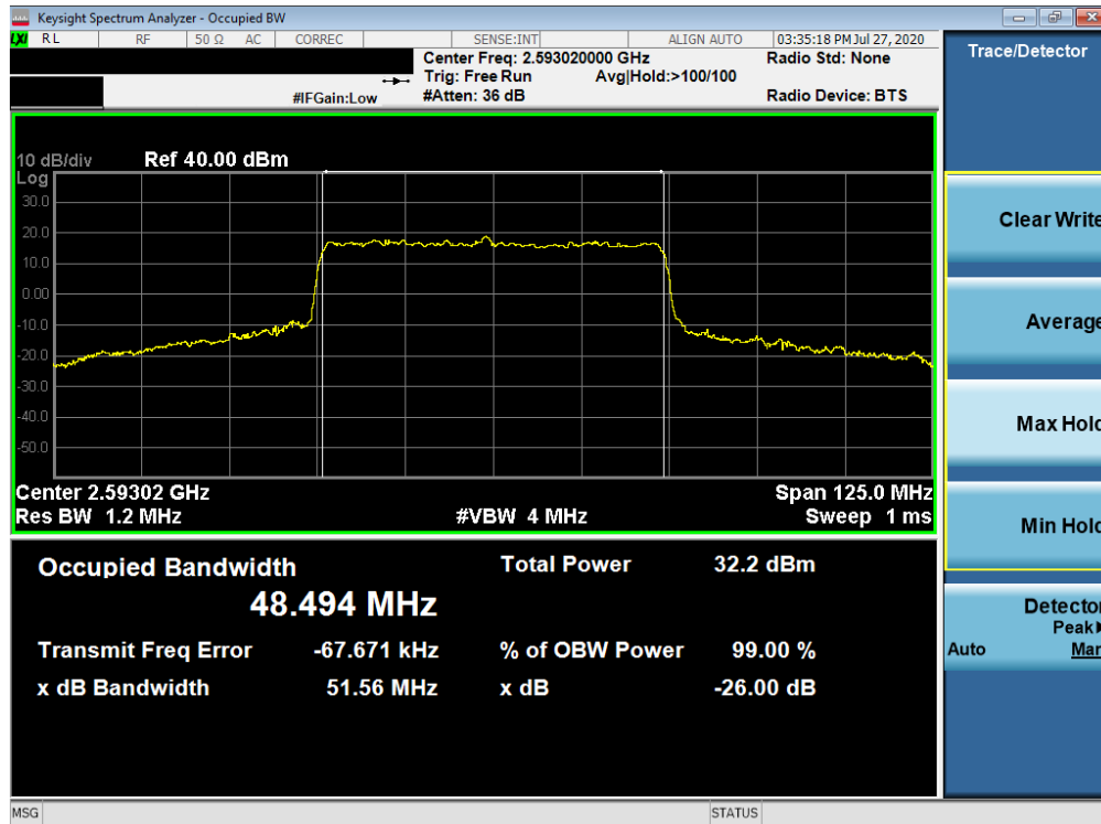
Plot 7-187. Occupied Bandwidth Plot (NR Band n41 - 50MHz CP-OFDM 64-QAM - Full RB)
