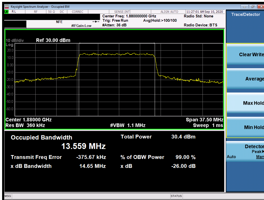
Plot 7-155. Occupied Bandwidth Plot (NR Band n25/2 - 15.0MHz CP-OFDM 64QAM - Full RB)
