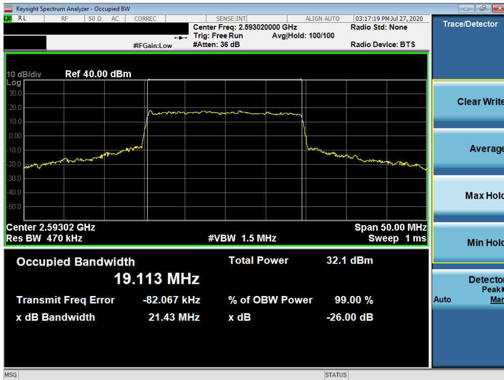
Plot 7-175. Occupied Bandwidth Plot (NR Band n41 - 20MHz CP-OFDM QPSK - Full RB)
