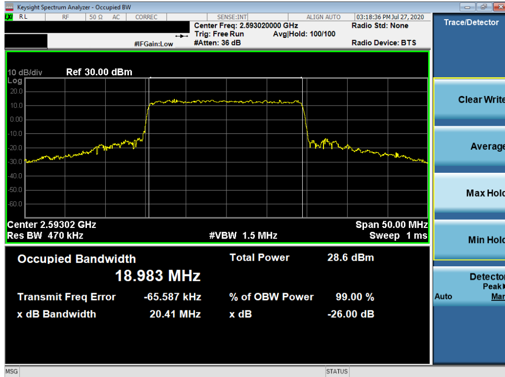
Plot 7-178. Occupied Bandwidth Plot (NR Band n41 - 20MHz CP-OFDM 256-QAM - Full RB)
