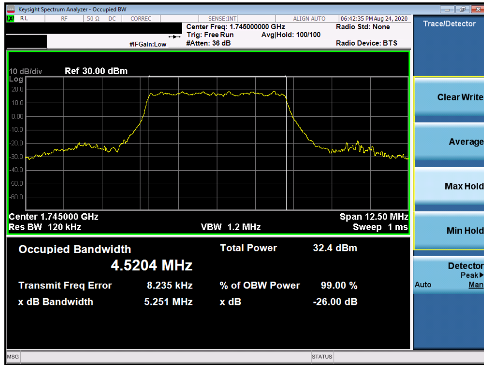
Plot 7-104. Occupied Bandwidth Plot (NR Band n66 - 5.0MHz DFT-s-OFDM BPSK - Full RB)
