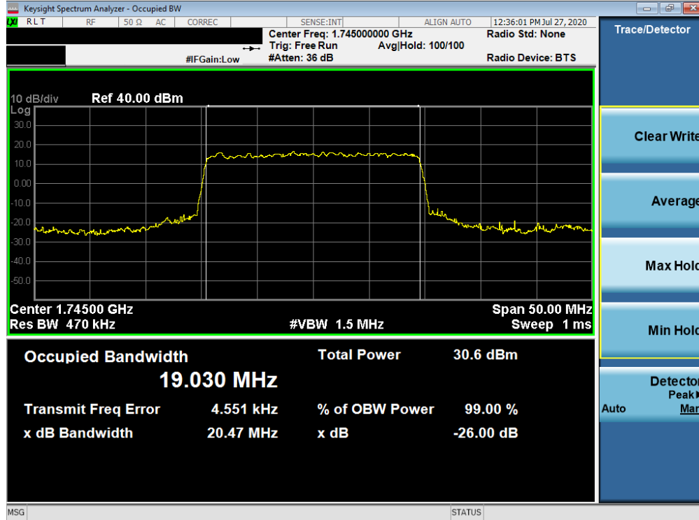
Plot 7-122. Occupied Bandwidth Plot (NR Band n66 - 20.0MHz CP-OFDM 64QAM - Full RB)
