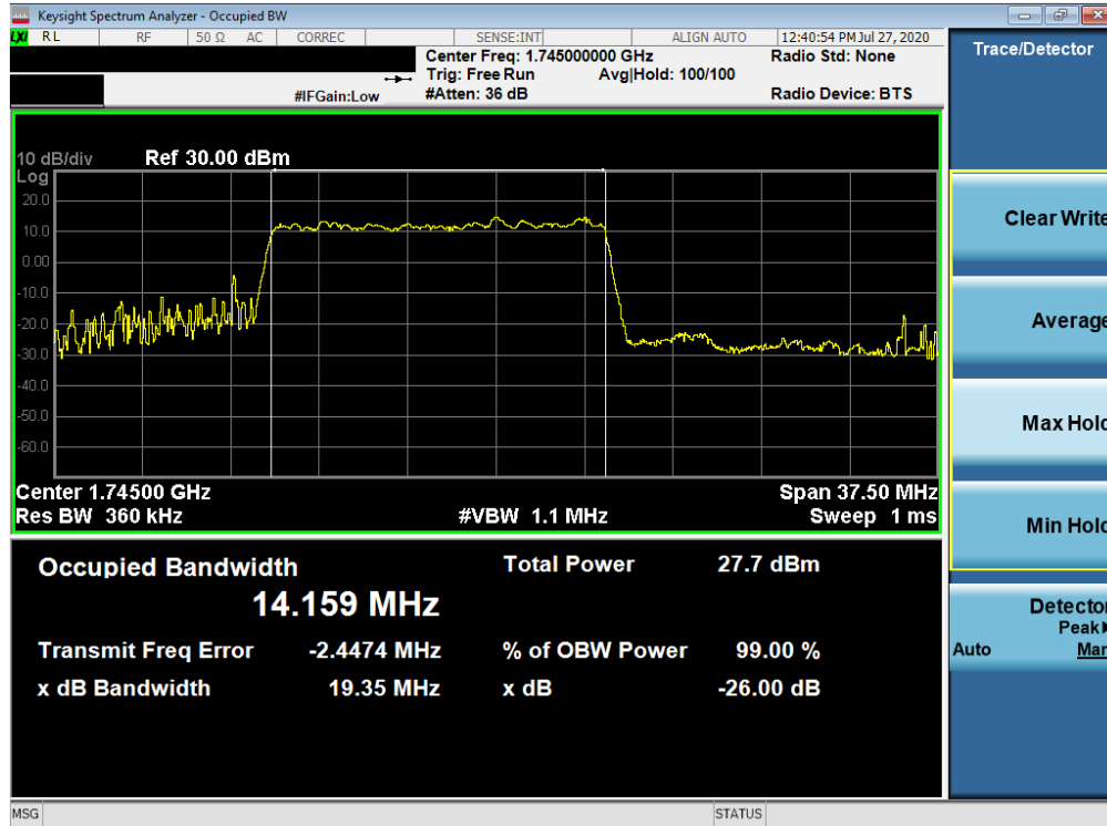
Plot 7-118. Occupied Bandwidth Plot (NR Band n66 - 15.0MHz CP-OFDM 256QAM - Full RB)
