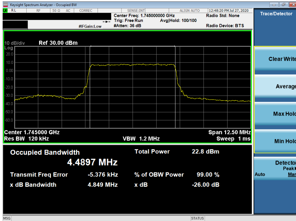
Plot 7-106. Occupied Bandwidth Plot (NR Band n66 - 5.0MHz CP-OFDM 16QAM - Full RB)
