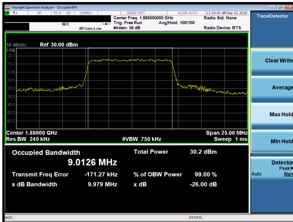
Plot 7-149. Occupied Bandwidth Plot (NR Band n25/2 - 10.0MHz CP-OFDM 16QAM - Full RB)
