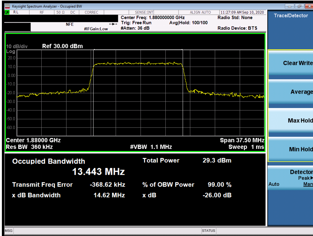
Plot 7-156. Occupied Bandwidth Plot (NR Band n25/2 - 15.0MHz CP-OFDM 256QAM - Full RB)
