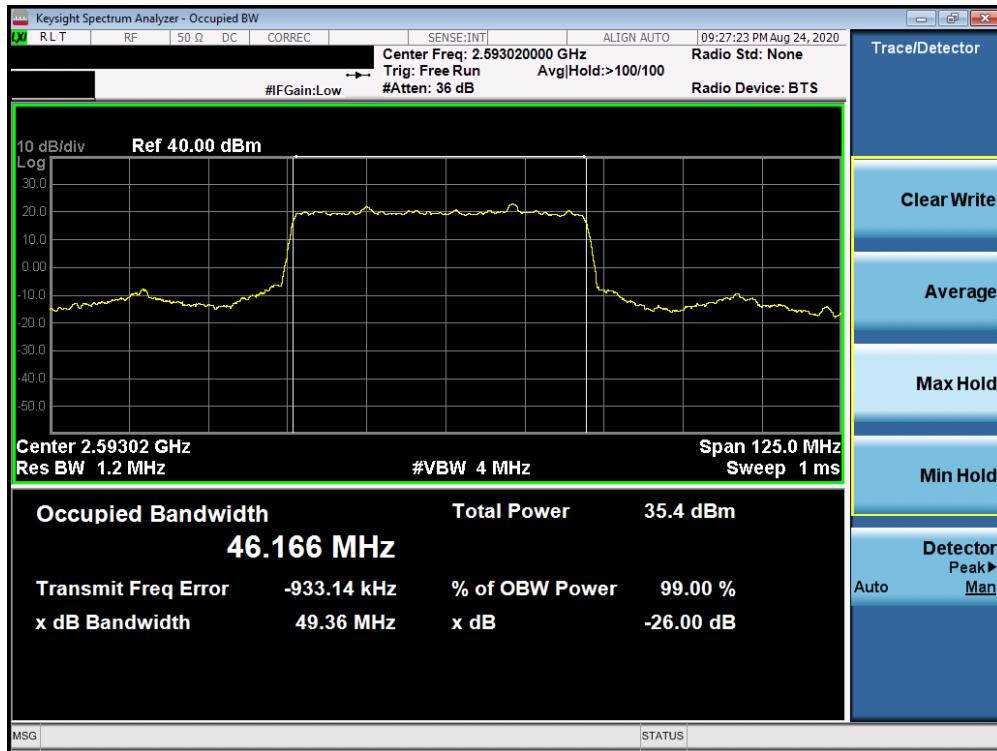
Plot 7-184. Occupied Bandwidth Plot (NR Band n41 - 50MHz DFT-s-OFDM BPSK - Full RB)
