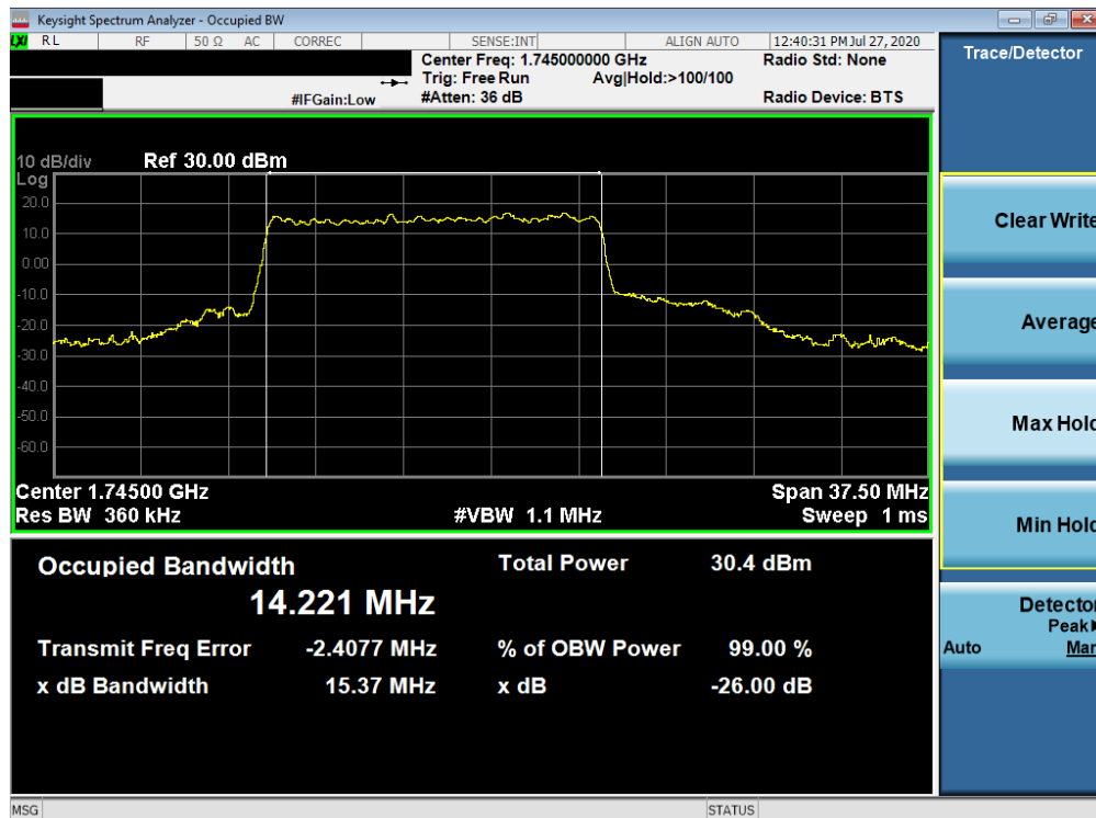
Plot 7-117. Occupied Bandwidth Plot (NR Band n66 - 15.0MHz CP-OFDM 64QAM - Full RB)
