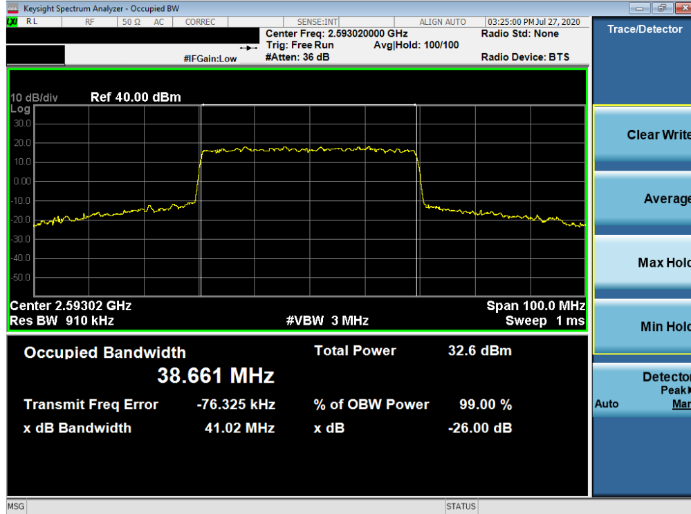
Plot 7-180. Occupied Bandwidth Plot (NR Band n41 - 40MHz CP-OFDM QPSK - Full RB)
