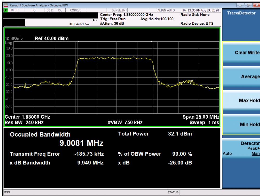
Plot 7-147. Occupied Bandwidth Plot (NR Band n25/2 - 10.0MHz DFT-s-OFDM BPSK - Full RB)
