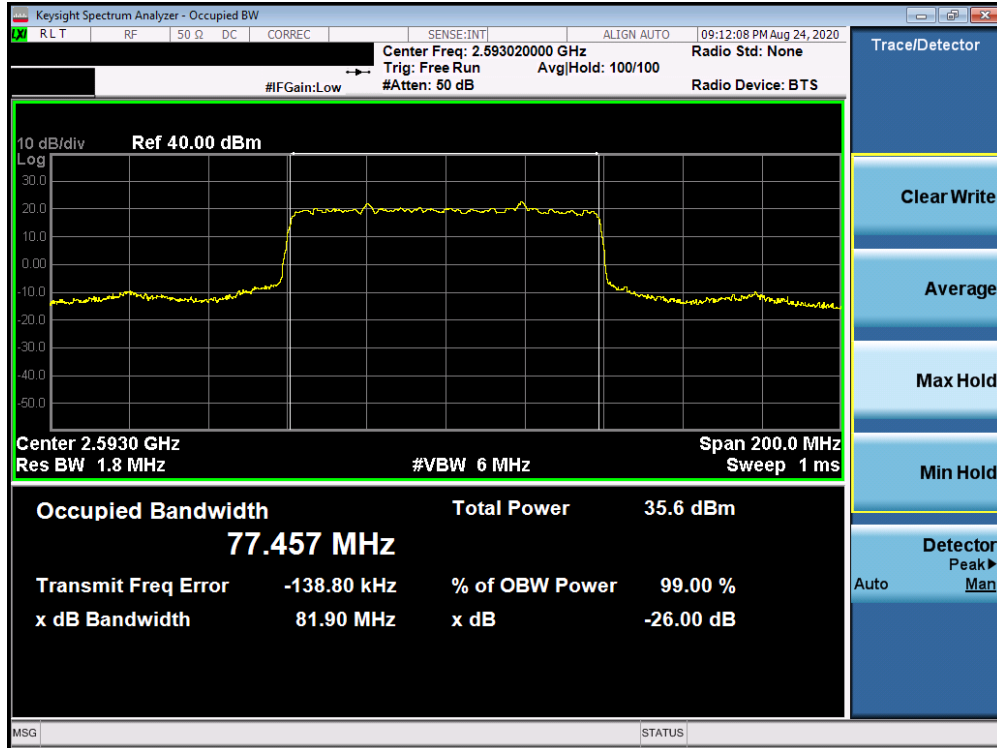
Plot 7-194. Occupied Bandwidth Plot (NR Band n41 - 80MHz DFT-s-OFDM BPSK - Full RB)
