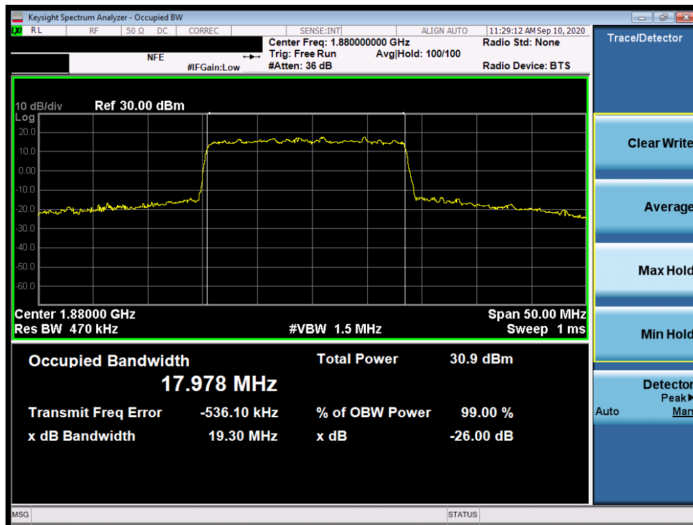
Plot 7-159. Occupied Bandwidth Plot (NR Band n25/2 - 20.0MHz CP-OFDM 16QAM - Full RB)
