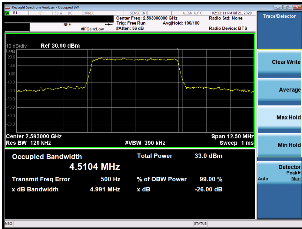
Plot 7-163. Occupied Bandwidth Plot (Band 41 – 5.0MHz 16-QAM - Full RB Configuration)
