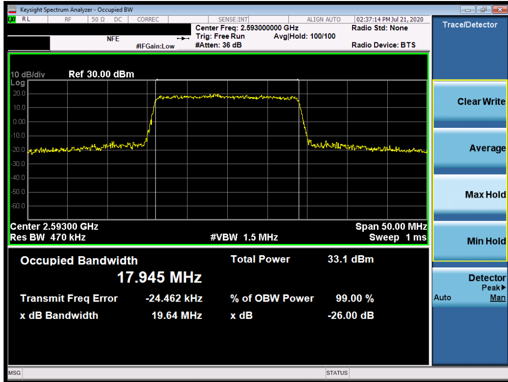
Plot 7-172. Occupied Bandwidth Plot (Band 41 - 20.0MHz 16-QAM - Full RB Configuration)
