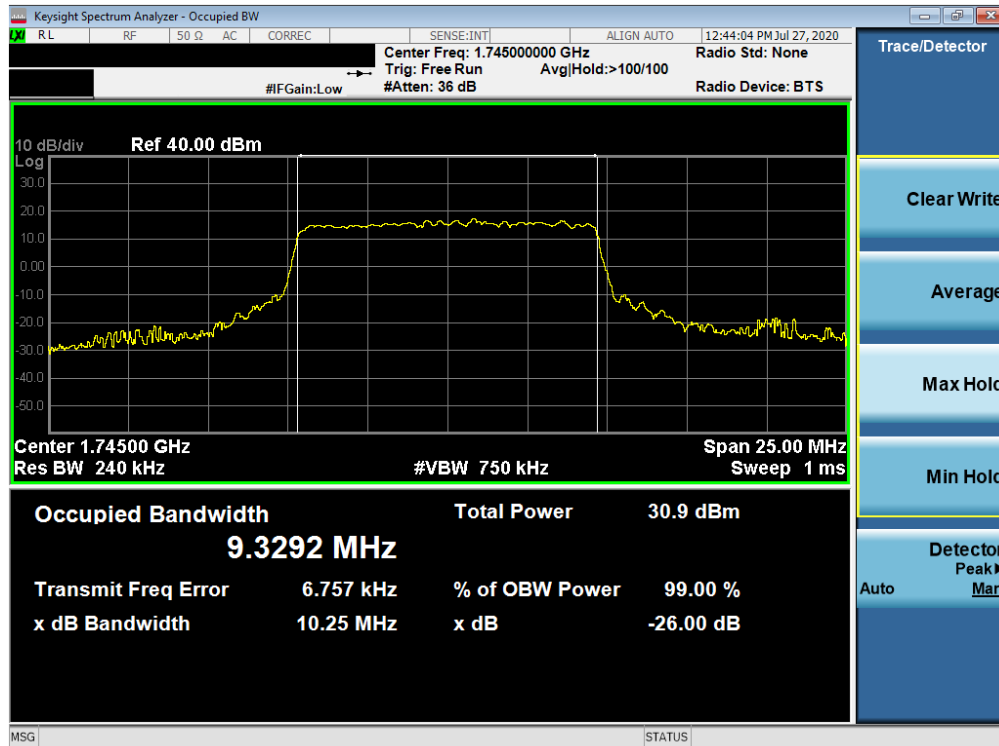
Plot 7-110. Occupied Bandwidth Plot (NR Band n66 - 10.0MHz CP-OFDM QPSK - Full RB)
