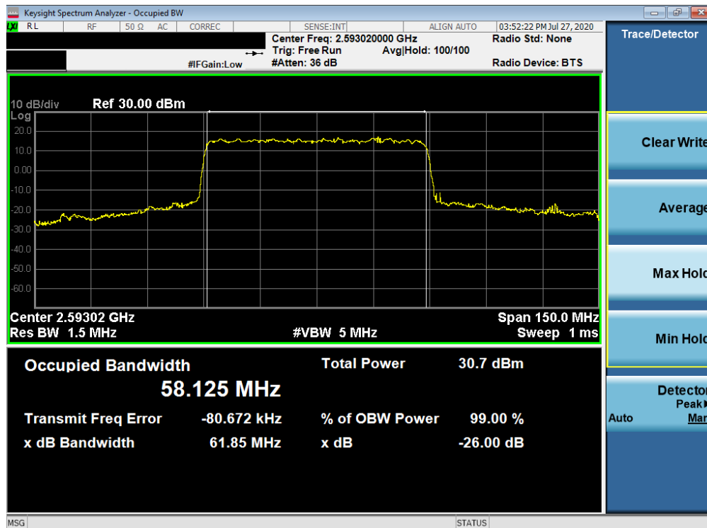
Plot 7-191. Occupied Bandwidth Plot (NR Band n41 - 60MHz CP-OFDM 16-QAM - Full RB)
