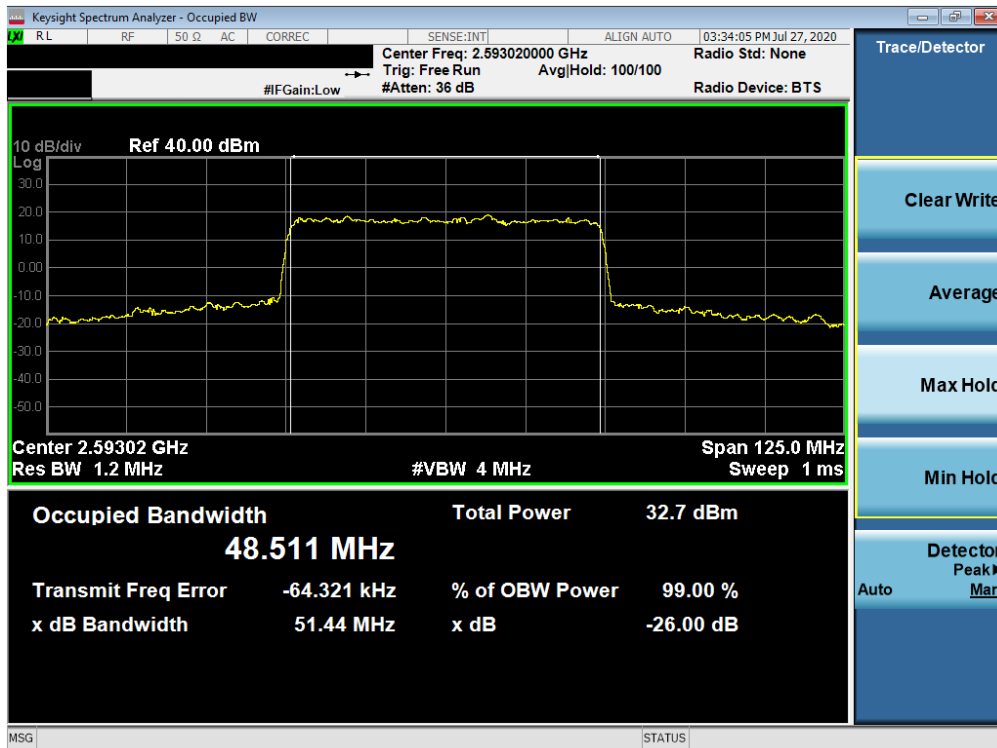
Plot 7-185. Occupied Bandwidth Plot (NR Band n41 - 50MHz CP-OFDM QPSK - Full RB)
