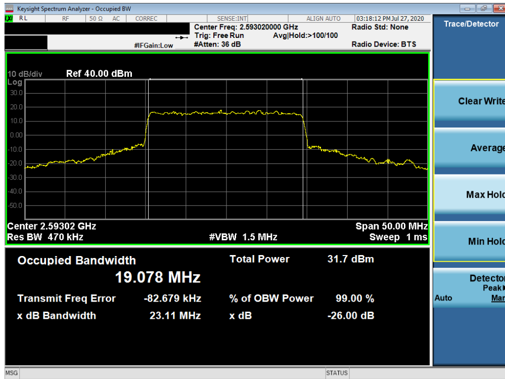
Plot 7-177. Occupied Bandwidth Plot (NR Band n41 - 20MHz CP-OFDM 64-QAM - Full RB)
