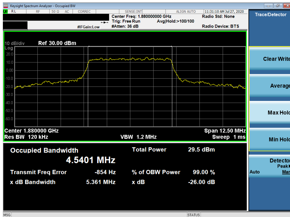
Plot 7-145. Occupied Bandwidth Plot (NR Band n25/2 - 5.0MHz CP-OFDM 64QAM - Full RB)
