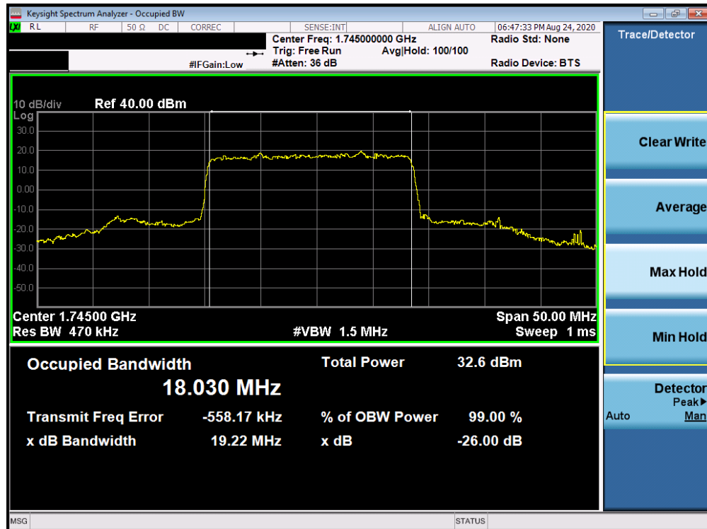
Plot 7-119. Occupied Bandwidth Plot (NR Band n66 - 20.0MHz DFT-s-OFDM BPSK - Full RB)
