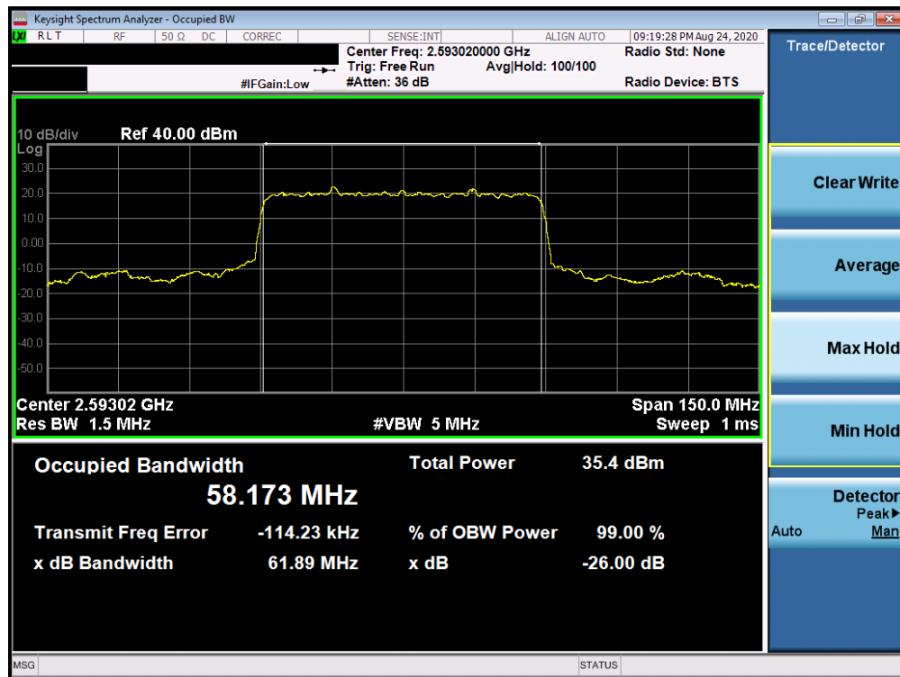
Plot 7-189. Occupied Bandwidth Plot (NR Band n41 - 60MHz DFT-s-OFDM BPSK - Full RB)
