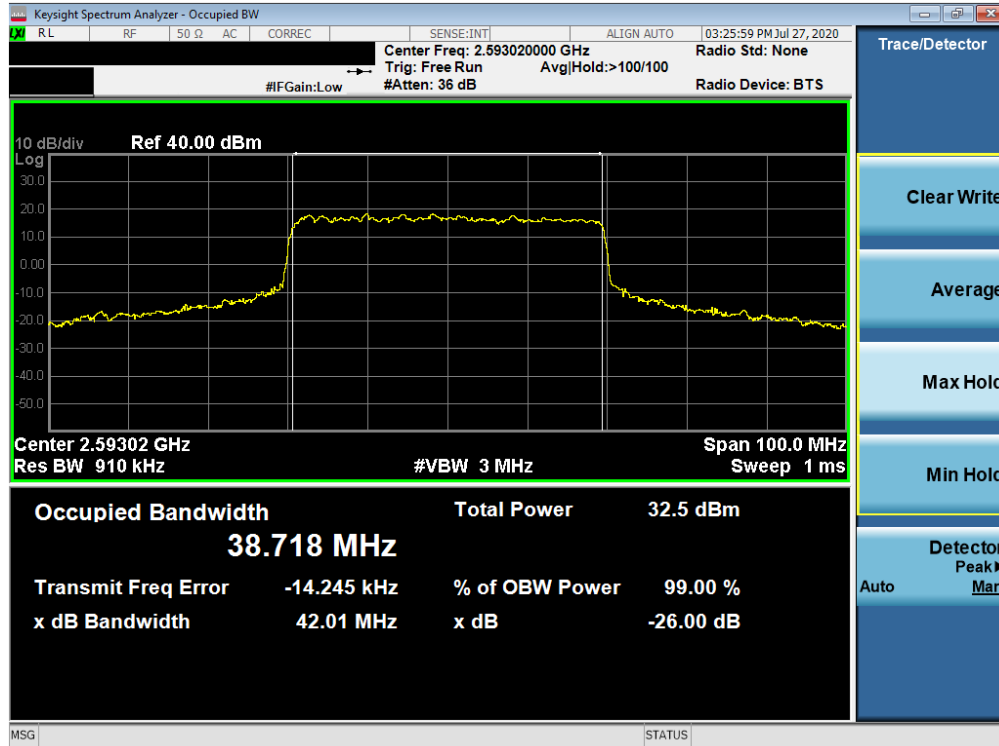
Plot 7-182. Occupied Bandwidth Plot (NR Band n41 - 40MHz CP-OFDM 64-QAM - Full RB)
