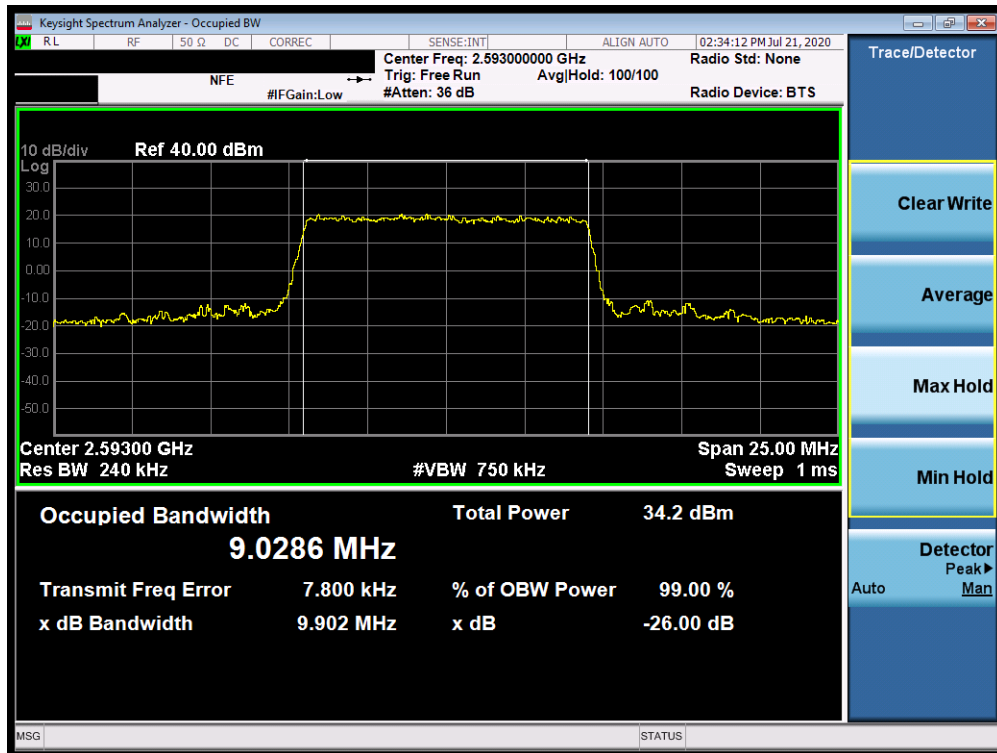
Plot 7-165. Occupied Bandwidth Plot (Band 41 - 10.0MHz QPSK - Full RB Configuration)
