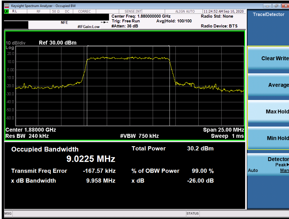
Plot 7-150. Occupied Bandwidth Plot (NR Band n25/2 - 10.0MHz CP-OFDM 64QAM - Full RB)
