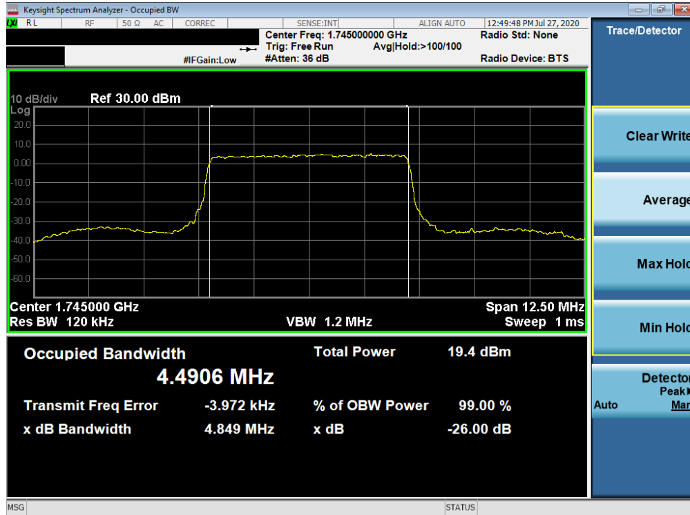
Plot 7-108. Occupied Bandwidth Plot (NR Band n66 - 5.0MHz CP-OFDM 256QAM - Full RB)
