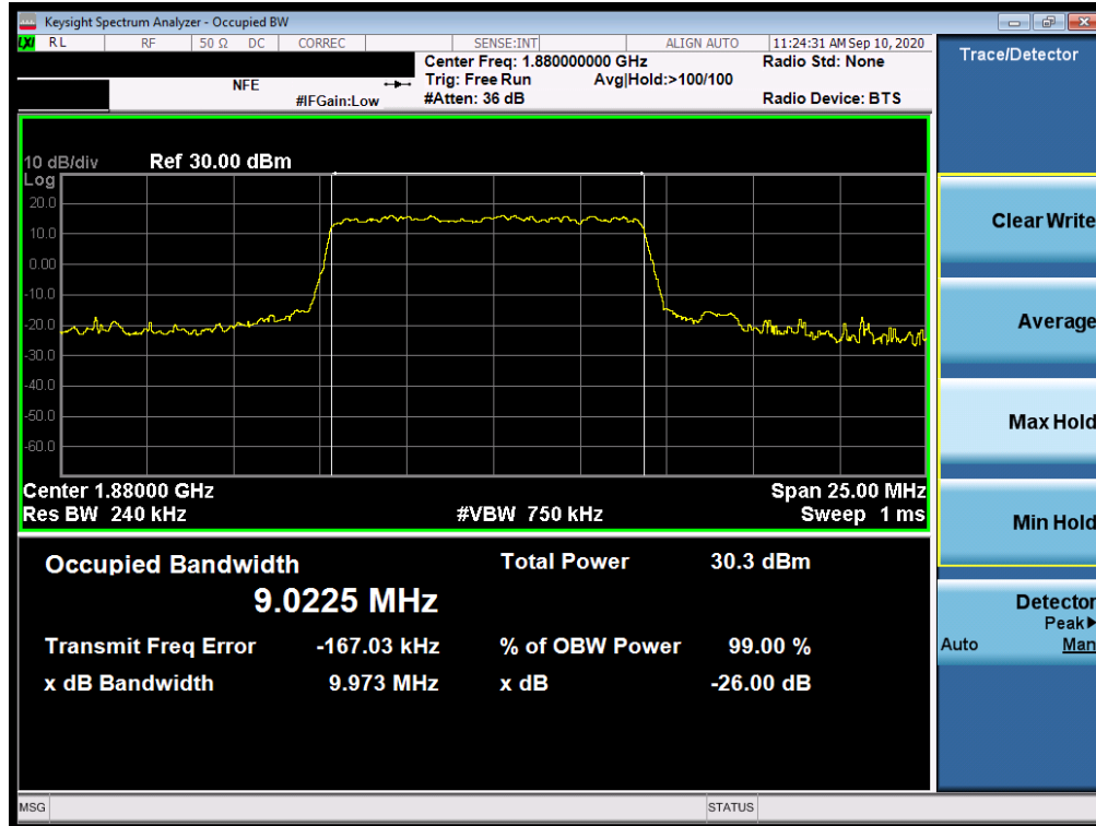
Plot 7-148. Occupied Bandwidth Plot (NR Band n25/2 - 10.0MHz CP-OFDM QPSK - Full RB)
