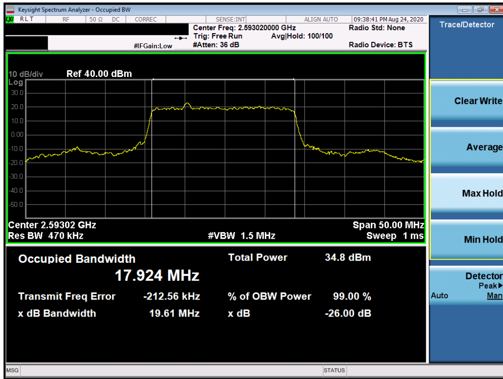
Plot 7-174. Occupied Bandwidth Plot (NR Band n41 - 20MHz DFT-s-OFDM BPSK - Full RB)
