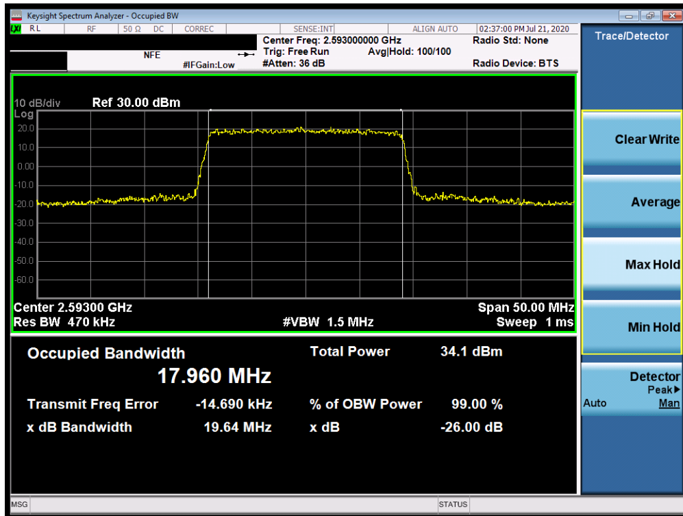
Plot 7-171. Occupied Bandwidth Plot (Band 41 - 20.0MHz QPSK - Full RB Configuration)
