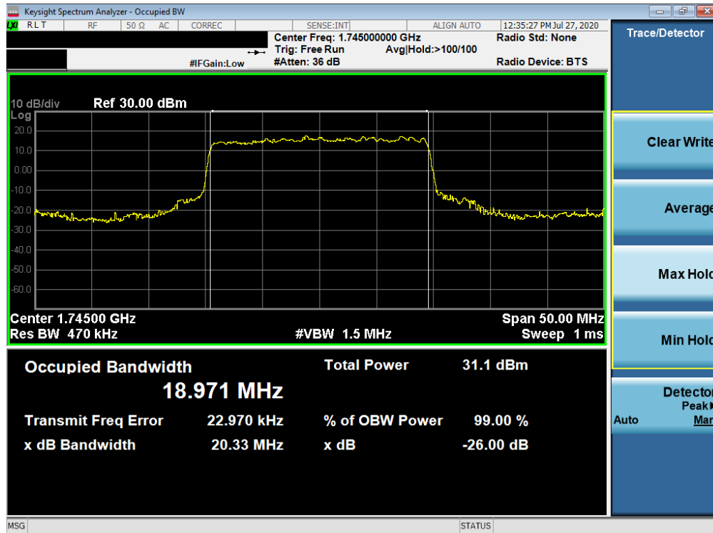
Plot 7-121. Occupied Bandwidth Plot (NR Band n66 - 20.0MHz CP-OFDM 16QAM - Full RB)
