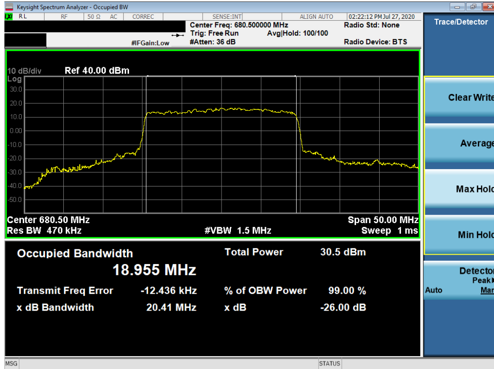
Plot 7-31. Occupied Bandwidth Plot (NR Band n71 - 20MHz CP-OFDM 64-QAM - Full RB)
