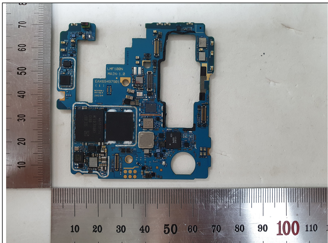
&lt;main PCB _ back view 2&gt;
