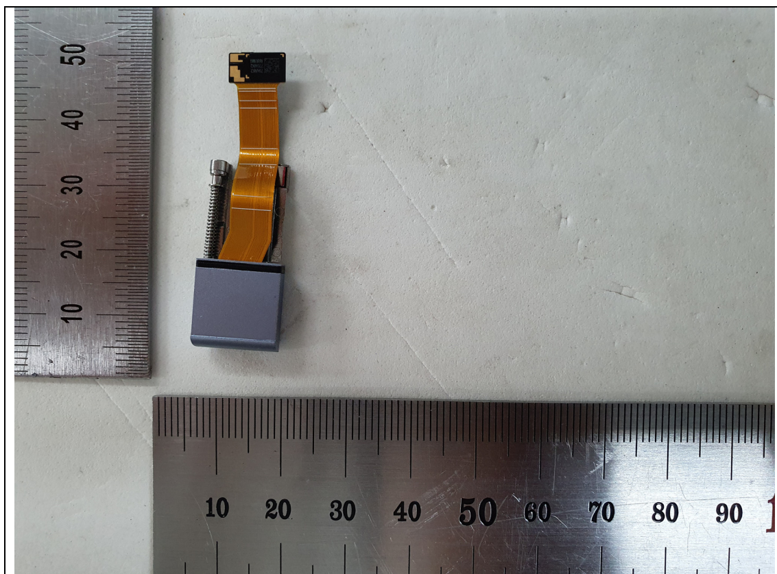
&lt;pop-up camera_ back view&gt;
