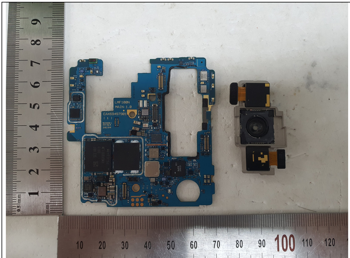
&lt;main PCB _ back view 3&gt;
