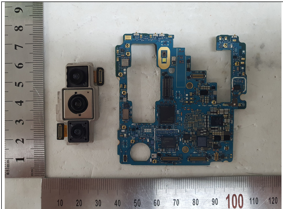
&lt;main PCB _ front view 3&gt;
