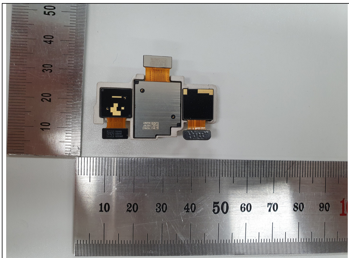
&lt;Rear camera _ back view 1&gt;
