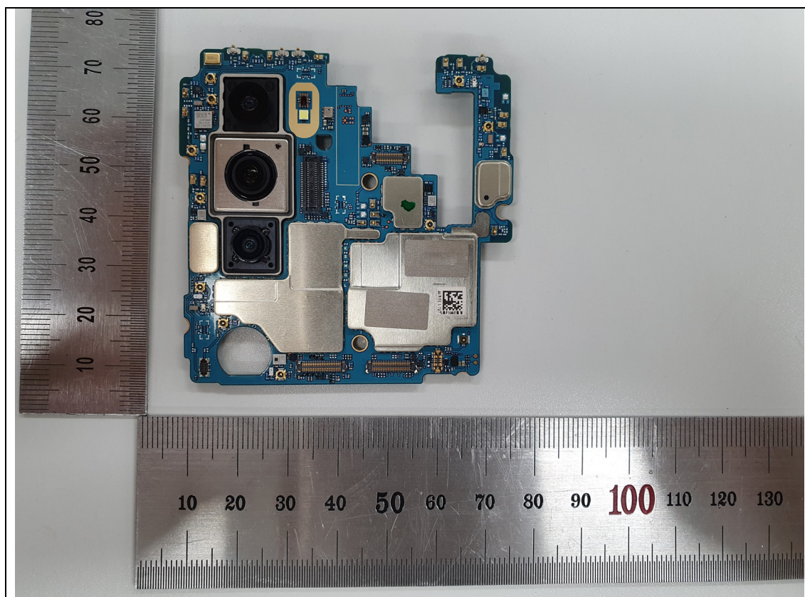
&lt;main PCB _ front view 1&gt;
