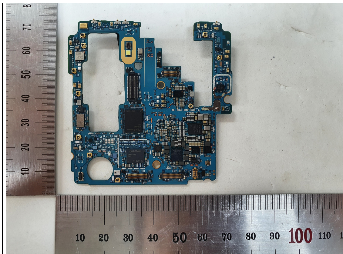
&lt;main PCB _ front view 2&gt;
