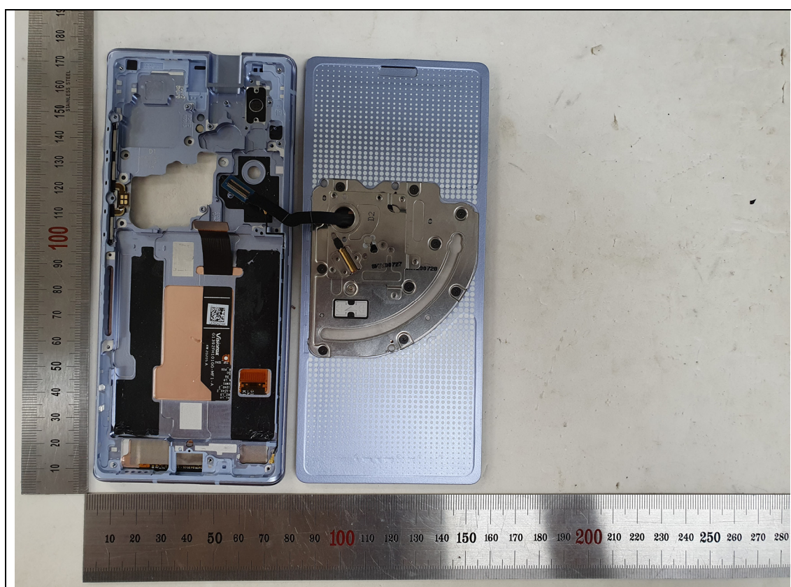
&lt;swivel display &amp; non-swivel display _ back view&gt;
