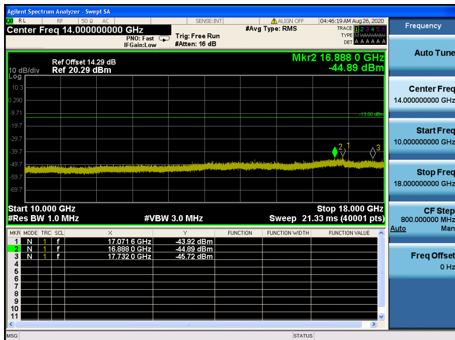
LTE Band 66, 4 / 5 MHz / 64QAM - RB Size/Offset (12/13) – Low Channel
