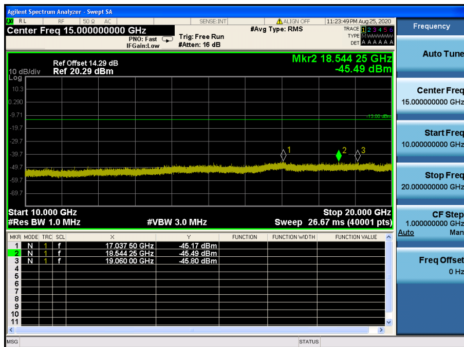
LTE Band 2 / 5 MHz / 64QAM - RB Size/Offset (1/12) – Mid Channel
