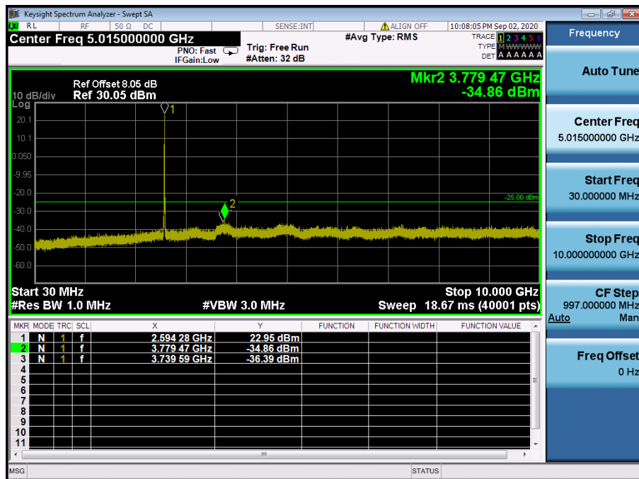
LTE Band 41 / 5 MHz / QPSK - RB Size/Offset (25/0) – Mid Channel
