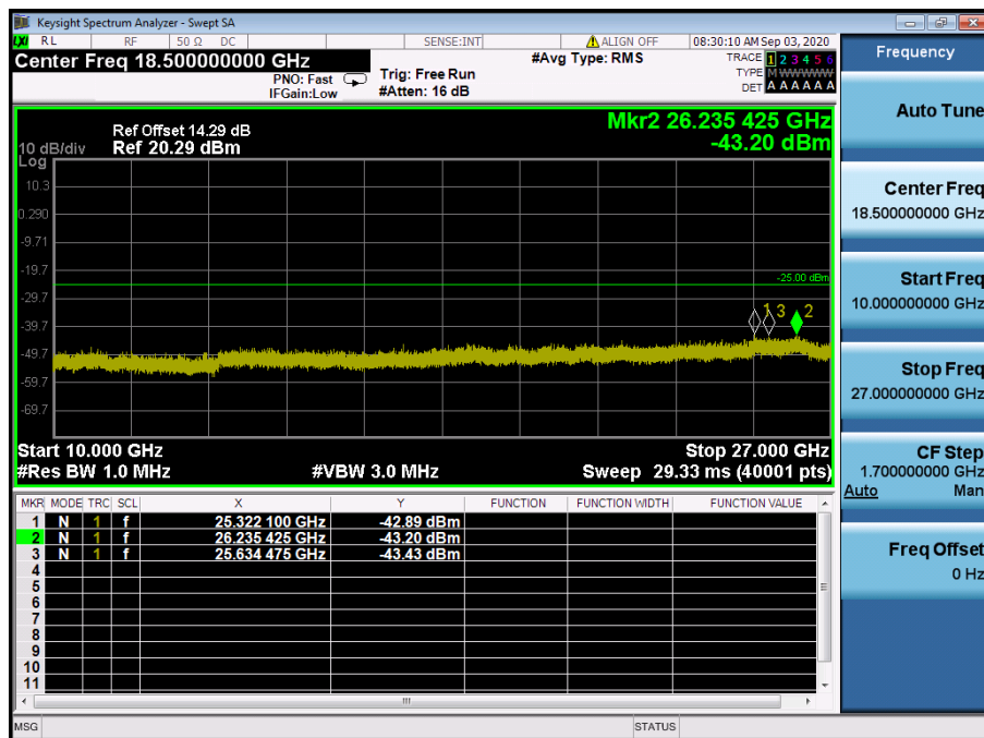
LTE Band 41 / 15 MHz / 64QAM - RB Size/Offset (36/0) – High Channel
