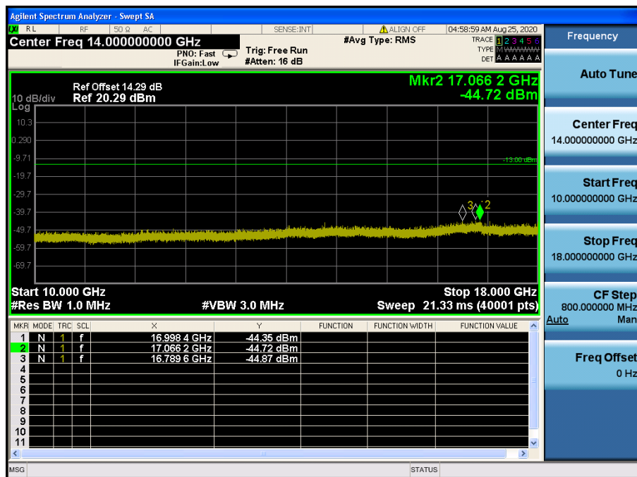
LTE Band 66, 4 / 10 MHz / QPSK - RB Size/Offset (1/49) – Low Channel
