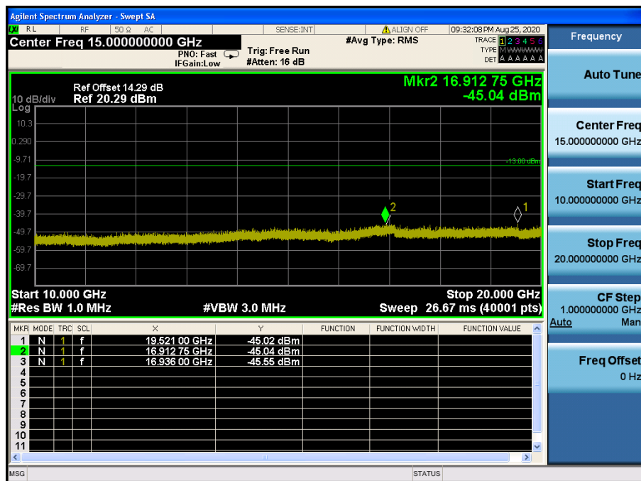
LTE Band 2 / 1.4 MHz / 64QAM - RB Size/Offset (1/5) – Mid Channel
