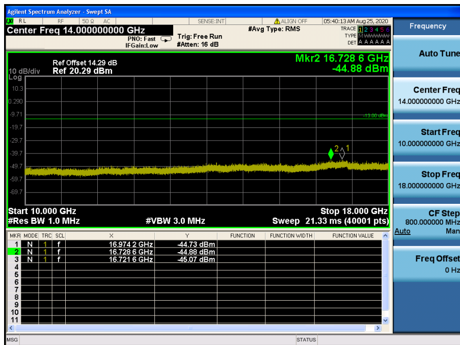
LTE Band 66, 4 / 10 MHz / QPSK - RB Size/Offset (50/0) – High Channel
