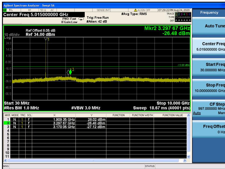
LTE Band 2 / 15 MHz / 16QAM - RB Size/Offset (1/74) – High Channel
