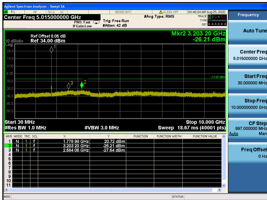
LTE Band 66, 4 / 5 MHz / QPSK - RB Size/Offset (25/0) – High Channel
