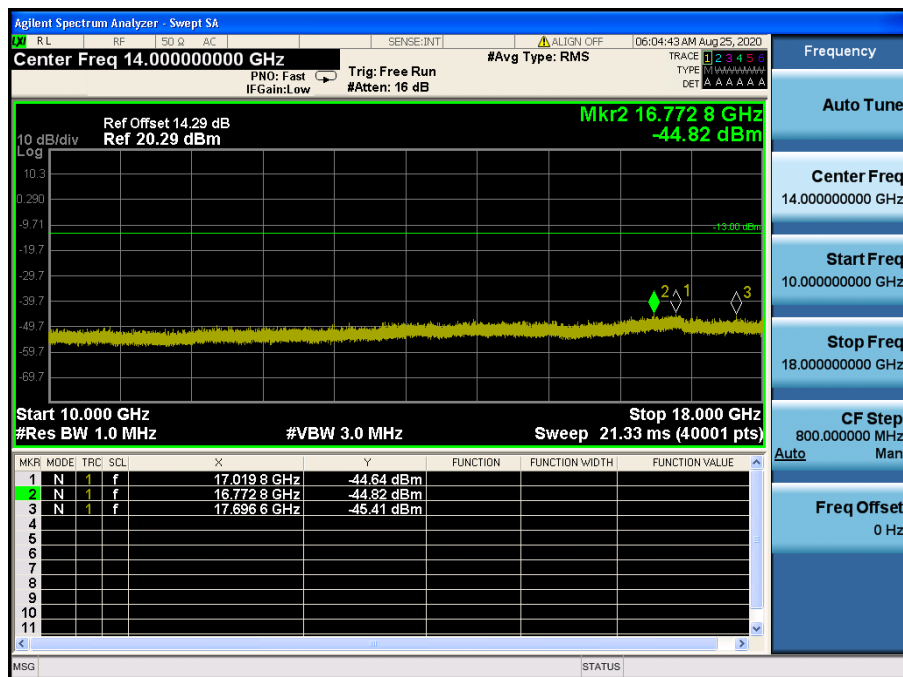
LTE Band 66, 4 / 15 MHz / QPSK - RB Size/Offset (1/0) – Mid Channel
