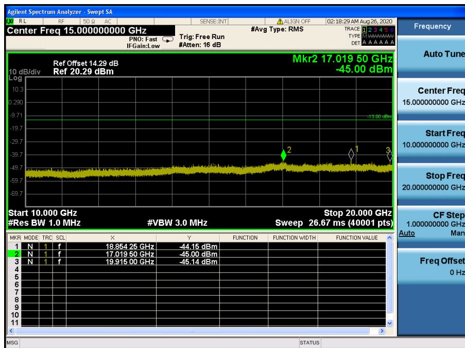
LTE Band 2 / 20 MHz / 64QAM - RB Size/Offset (1/99) – High Channel
