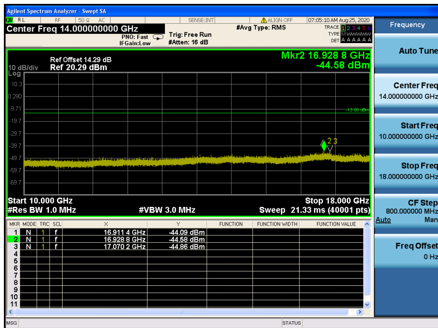
LTE Band 66, 4 / 20 MHz / QPSK - RB Size/Offset (1/0) – High Channel
