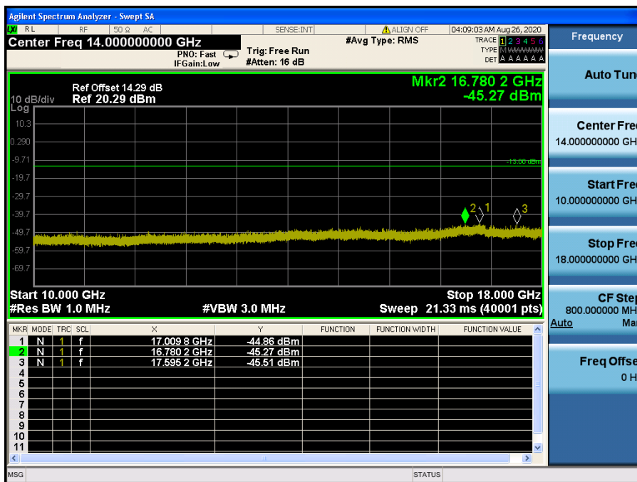
LTE Band 66, 4 / 3 MHz / 64QAM - RB Size/Offset (1/7) – High Channel
