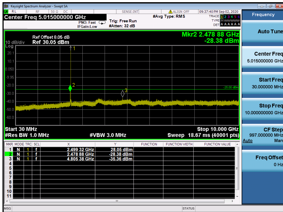
LTE Band 41 / 5 MHz / QPSK - RB Size/Offset (1/12) – Low Channel
