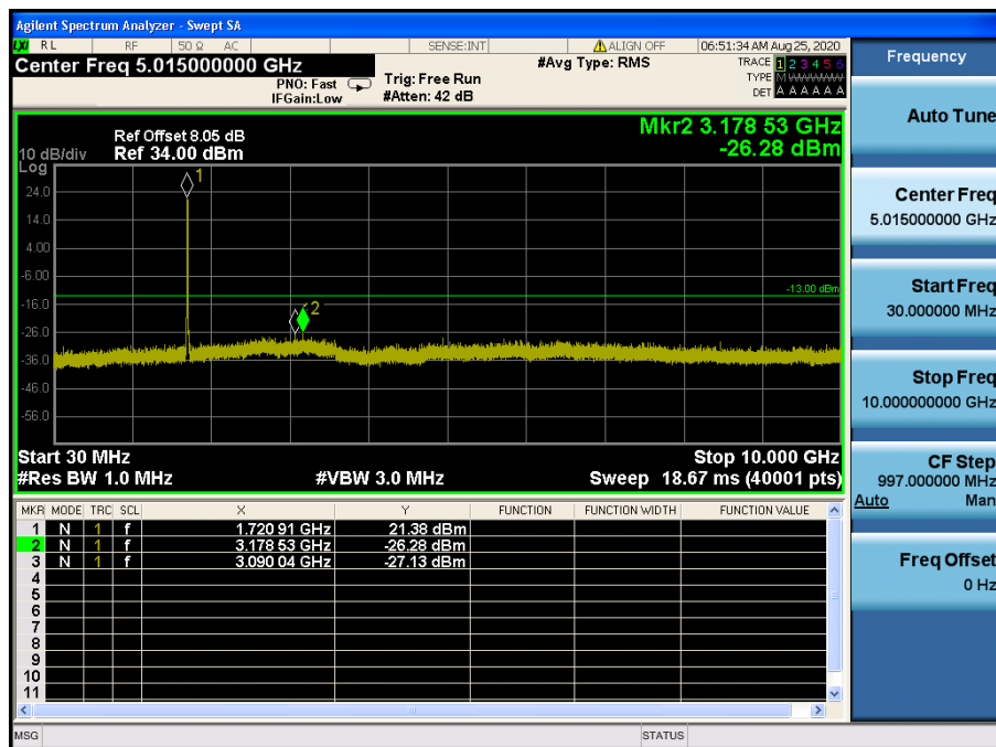
LTE Band 66, 4 / 20 MHz / QPSK - RB Size/Offset (50/50) – Low Channel
