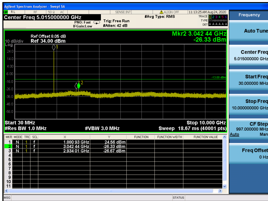
LTE Band 2 / 3 MHz / QPSK - RB Size/Offset (8/7) – Mid Channel
