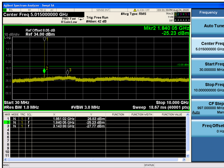
LTE Band 2 / 1.4 MHz / 16QAM - RB Size/Offset (3/2) – Low Channel
