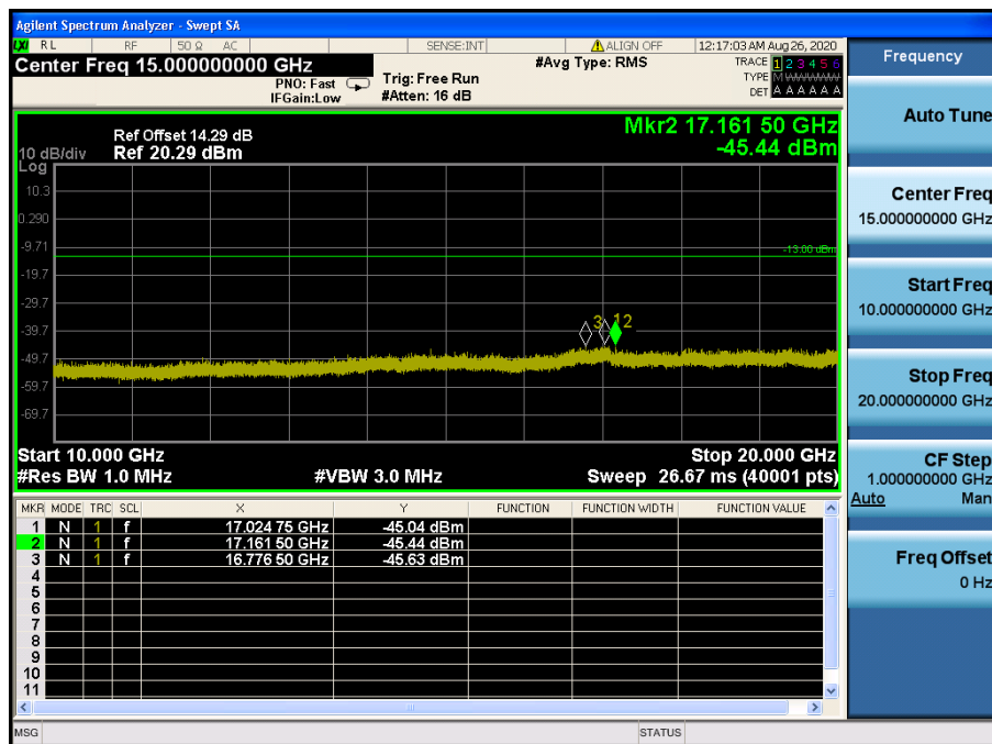
LTE Band 2 / 10 MHz / 64QAM - RB Size/Offset (1/25) – Mid Channel
