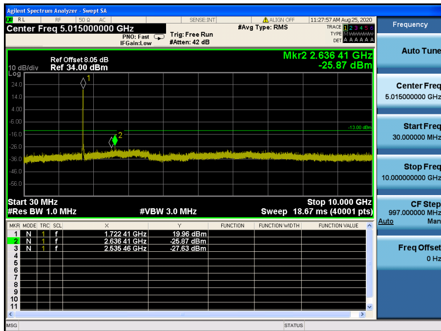
LTE Band 66, 4 / 15 MHz / 16QAM - RB Size/Offset (75/0) – Low Channel
