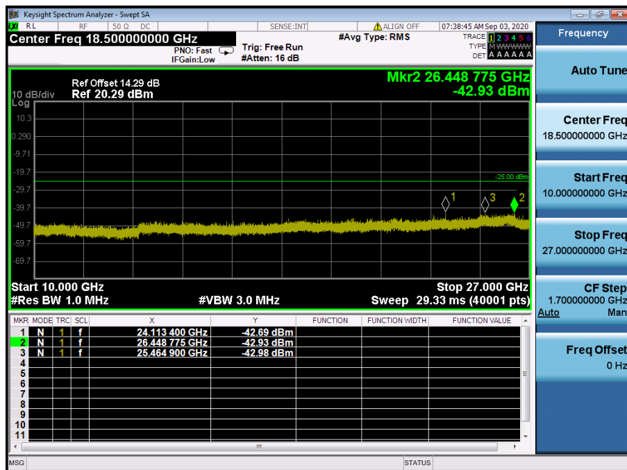
LTE Band 41 / 15 MHz / 64QAM - RB Size/Offset (1/0) – Low Channel
