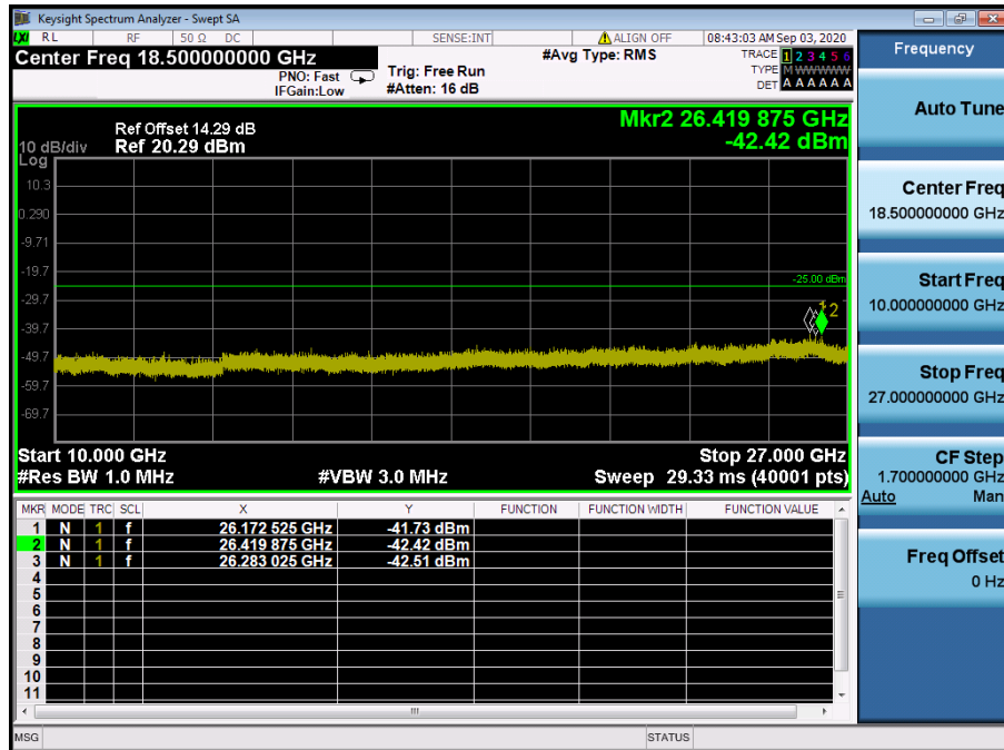
LTE Band 41 / 20 MHz / 64QAM - RB Size/Offset (1/0) – Low Channel
