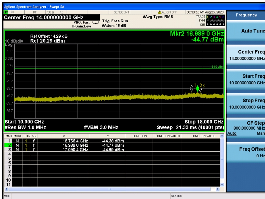
LTE Band 66, 4 / 3 MHz / 16QAM - RB Size/Offset (8/4) – Low Channel
