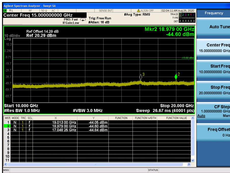
LTE Band 2 / 20 MHz / 64QAM - RB Size/Offset (1/50) – Mid Channel
