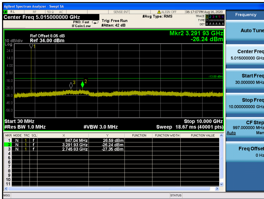
LTE Band 5 / 3 MHz / 64QAM - RB Size/Offset (8/0) – High Channel
