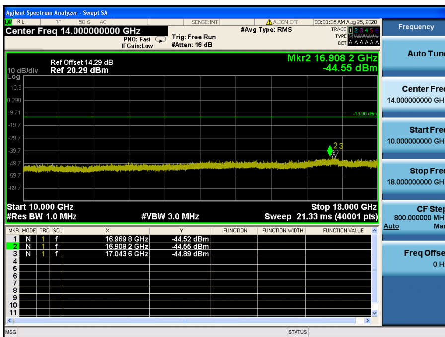
LTE Band 66, 4 / 3 MHz / QPSK - RB Size/Offset (15/0) – Mid Channel
