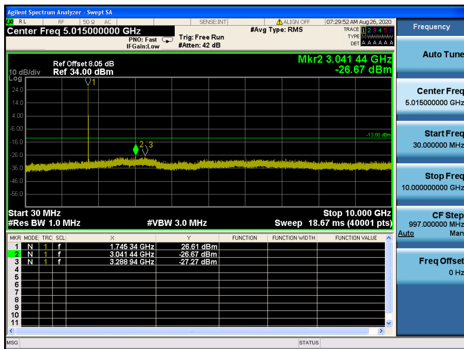
LTE Band 66, 4 / 20 MHz / 64QAM - RB Size/Offset (1/50) – Mid Channel
