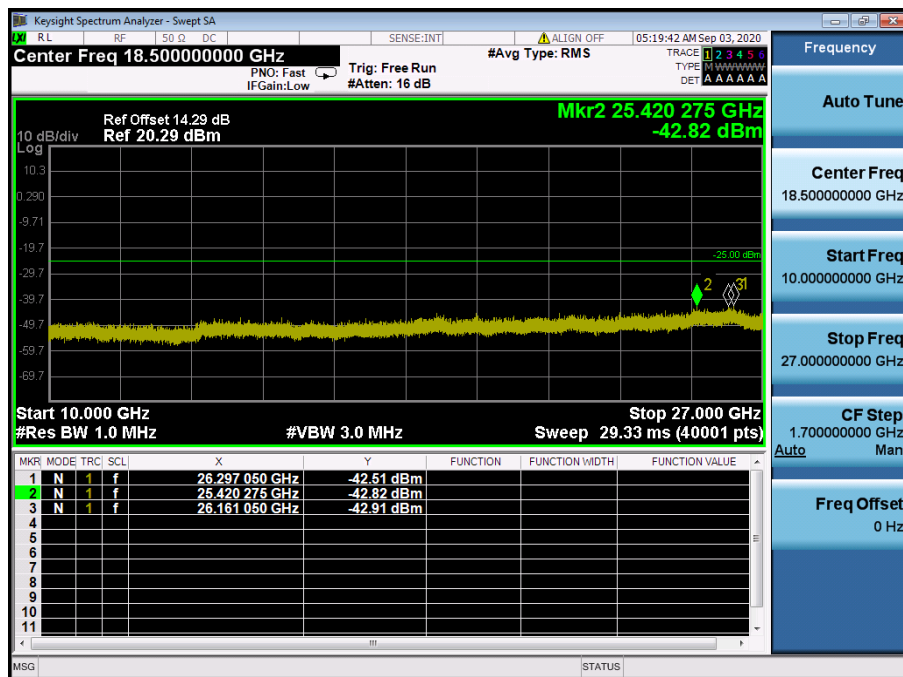
LTE Band 41 / 20 MHz / 16QAM - RB Size/Offset (50/50) – Mid Channel
