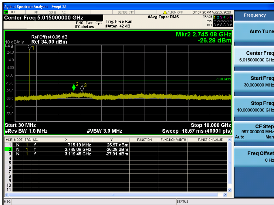
LTE Band 12 / 1.4 MHz / 64QAM - RB Size/Offset (6/0) – High Channel
