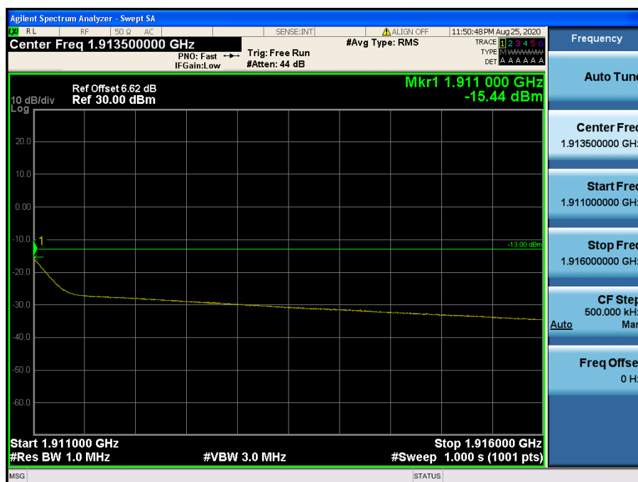
LTE Band 2 / 5 MHz / 64QAM - RB Size/Offset (25/0)
