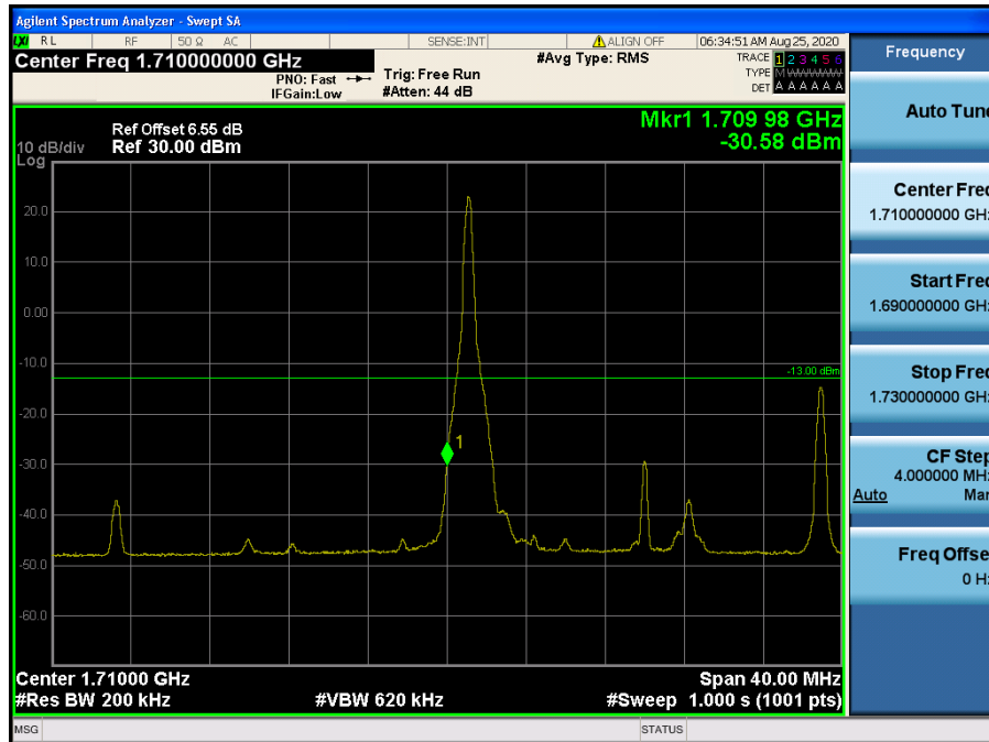
LTE Band 66, 4 / 20 MHz / QPSK - RB Size/Offset (1/0)
