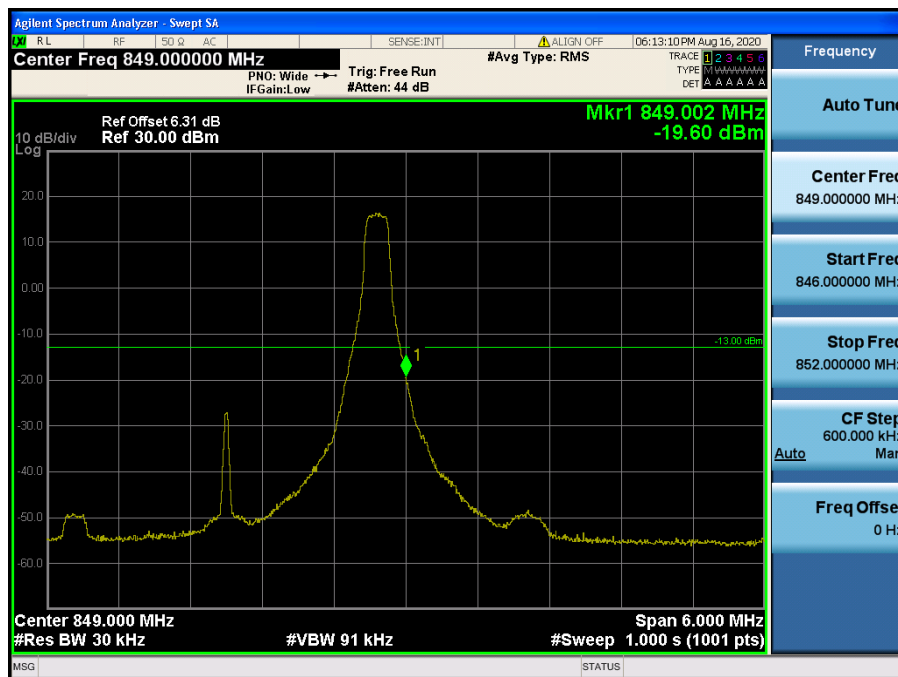
LTE Band 5 / 3 MHz / 64QAM - RB Size/Offset (1/14)
