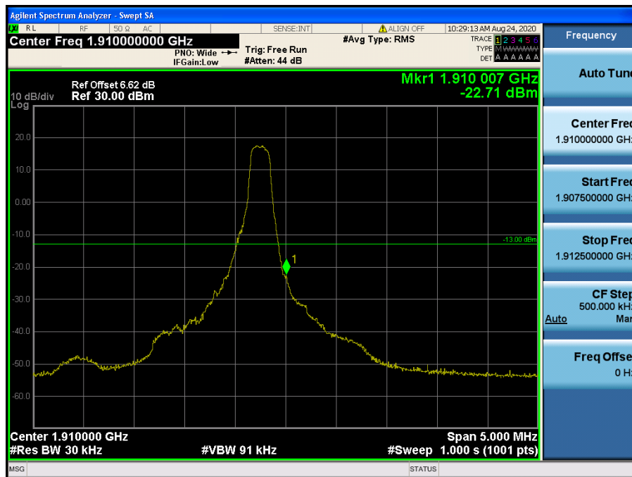
LTE Band 2 / 1.4 MHz / QPSK - RB Size/Offset (1/5)
