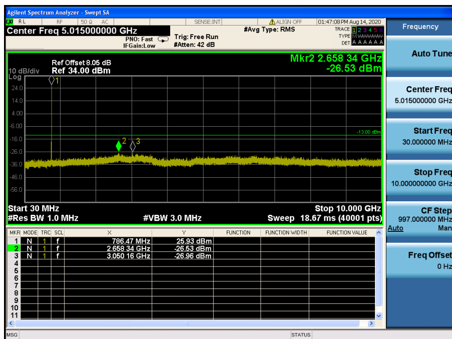
LTE Band 13 / 5 MHz / QPSK - RB Size/Offset (12/13) – High Channel
