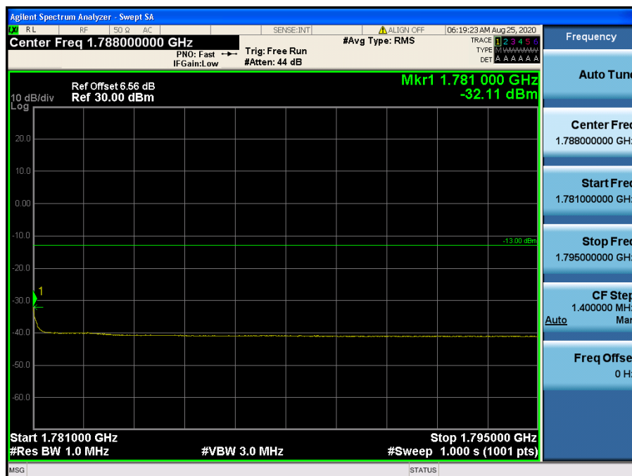
LTE Band 66, 4 / 15 MHz / QPSK - RB Size/Offset (1/74)
