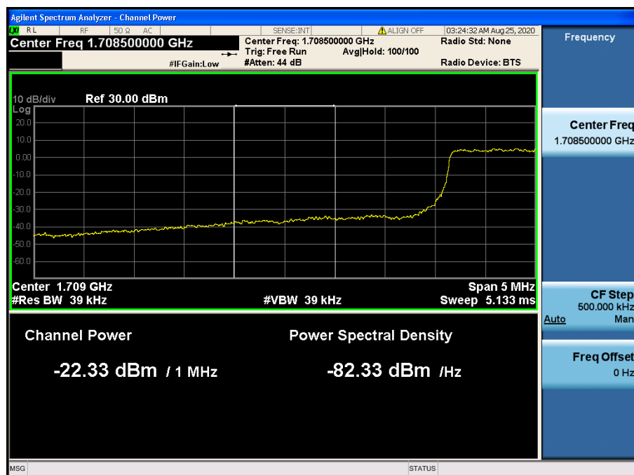
LTE Band 66, 4 / 3 MHz / QPSK - RB Size/Offset (15/0)
