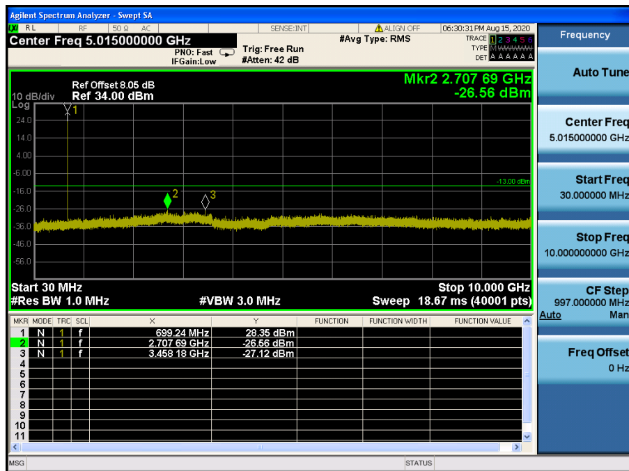
LTE Band 12 / 1.4 MHz / 64QAM - RB Size/Offset (1/0) – Low Channel
