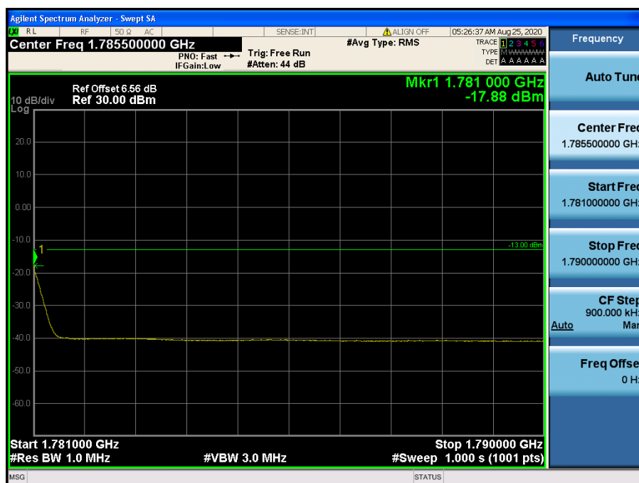
LTE Band 66, 4 / 10 MHz / QPSK - RB Size/Offset (1/49)
