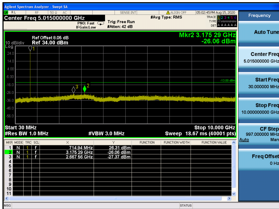
LTE Band 12 / 3 MHz / 16QAM - RB Size/Offset (8/4) – High Channel
