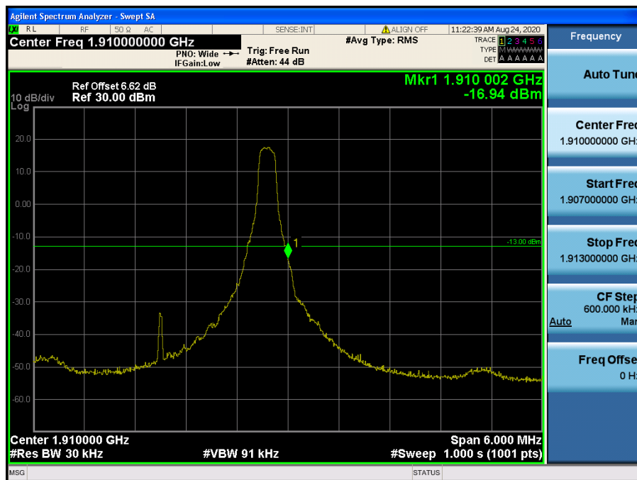
LTE Band 2 / 3 MHz / QPSK - RB Size/Offset (1/14)
