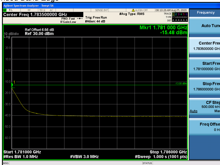
LTE Band 66, 4 / 1.4 MHz / 16QAM - RB Size/Offset (3/2)
