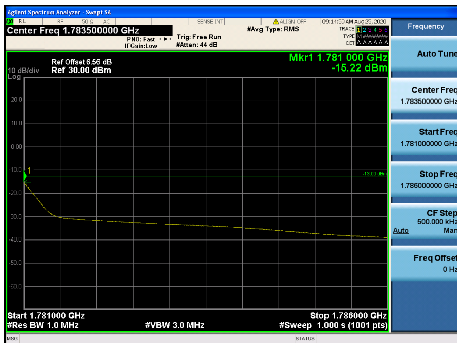
LTE Band 66, 4 / 3 MHz / 16QAM - RB Size/Offset (15/0)
