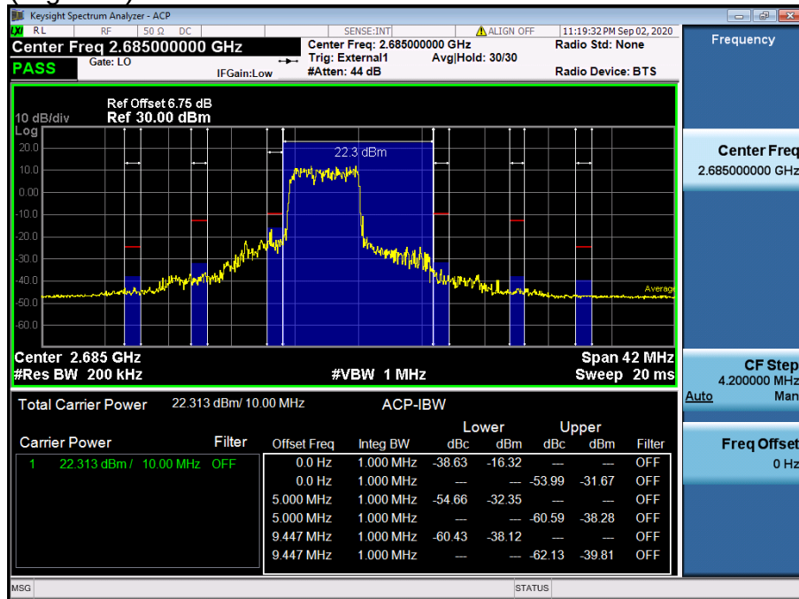
LTE Band 41 / 10MHz / QPSK - RB Size/Offset (25/0)
