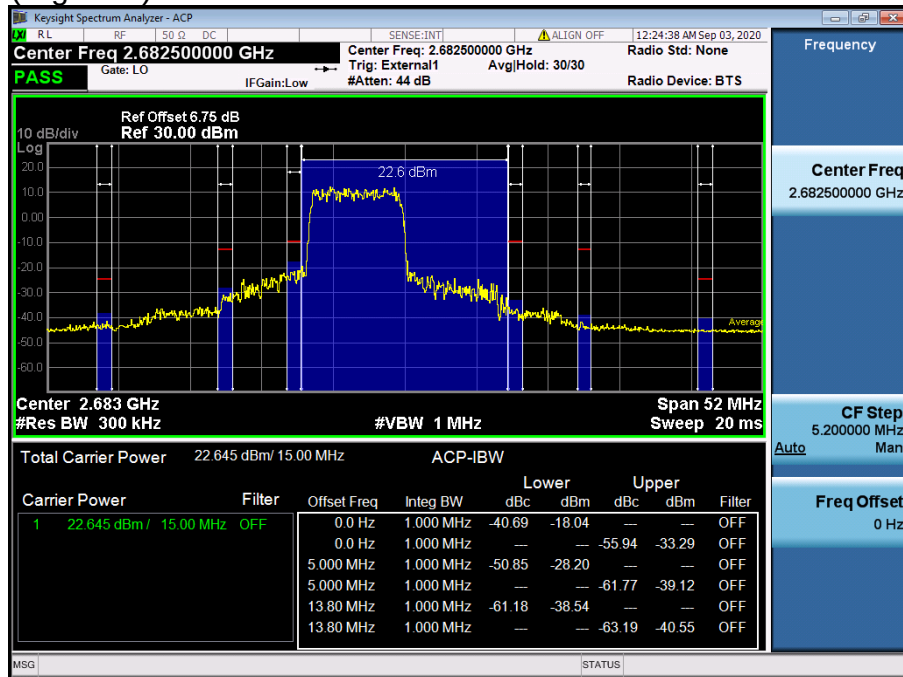
LTE Band 41 / 15 MHz / QPSK - RB Size/Offset (36/0)
