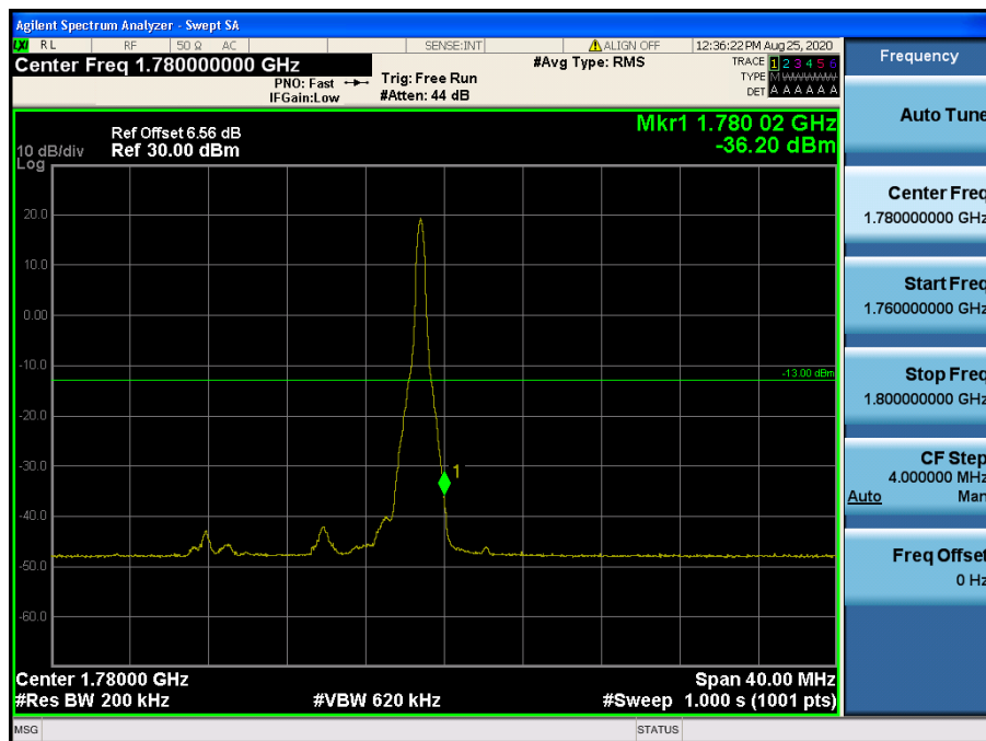
LTE Band 66, 4 / 20 MHz / 16QAM - RB Size/Offset (1/99)
