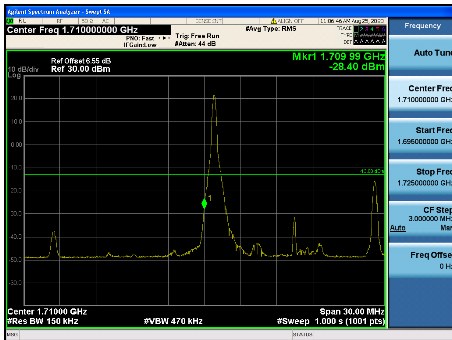
LTE Band 66, 4 / 15 MHz / 16QAM - RB Size/Offset (1/0)
