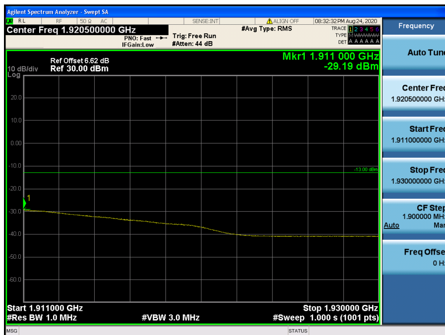
LTE Band 2 / 20 MHz / 16QAM - RB Size/Offset (50/50)
