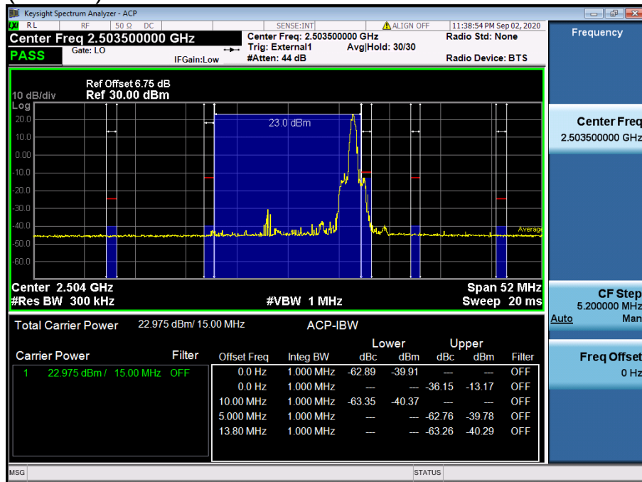
LTE Band 41 / 15 MHz / QPSK - RB Size/Offset (1/74)
