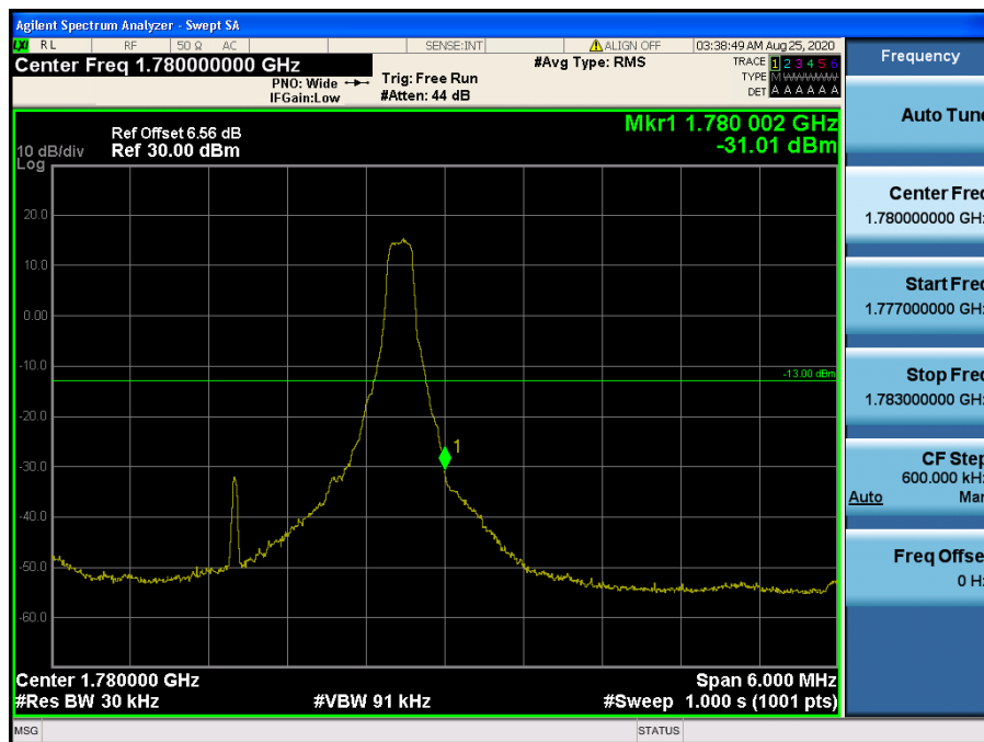
LTE Band 66, 4 / 3 MHz / QPSK - RB Size/Offset (1/14)
