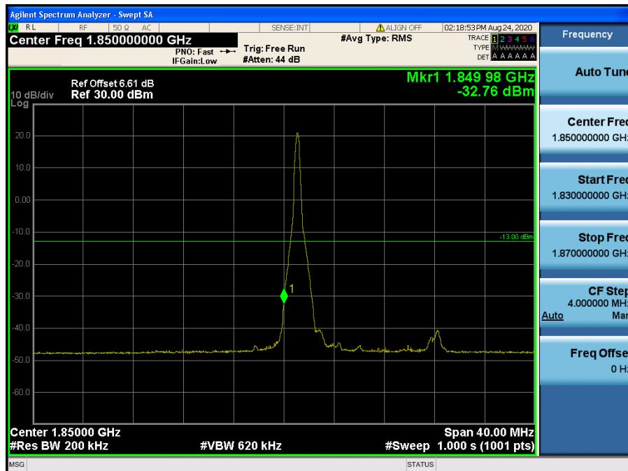
LTE Band 2 / 20 MHz / QPSK - RB Size/Offset (1/0)
