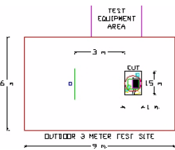
Figure 3-2. Dimensions of Outdoor Test Site
