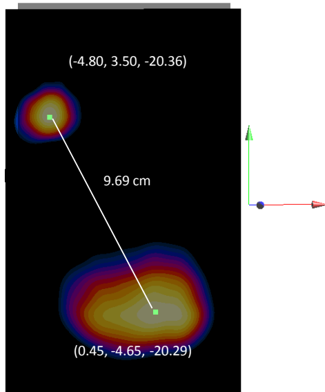
Figure 13-3 Peak SAR Location Plot of UMTS 1900 and 5 GHz WLAN
