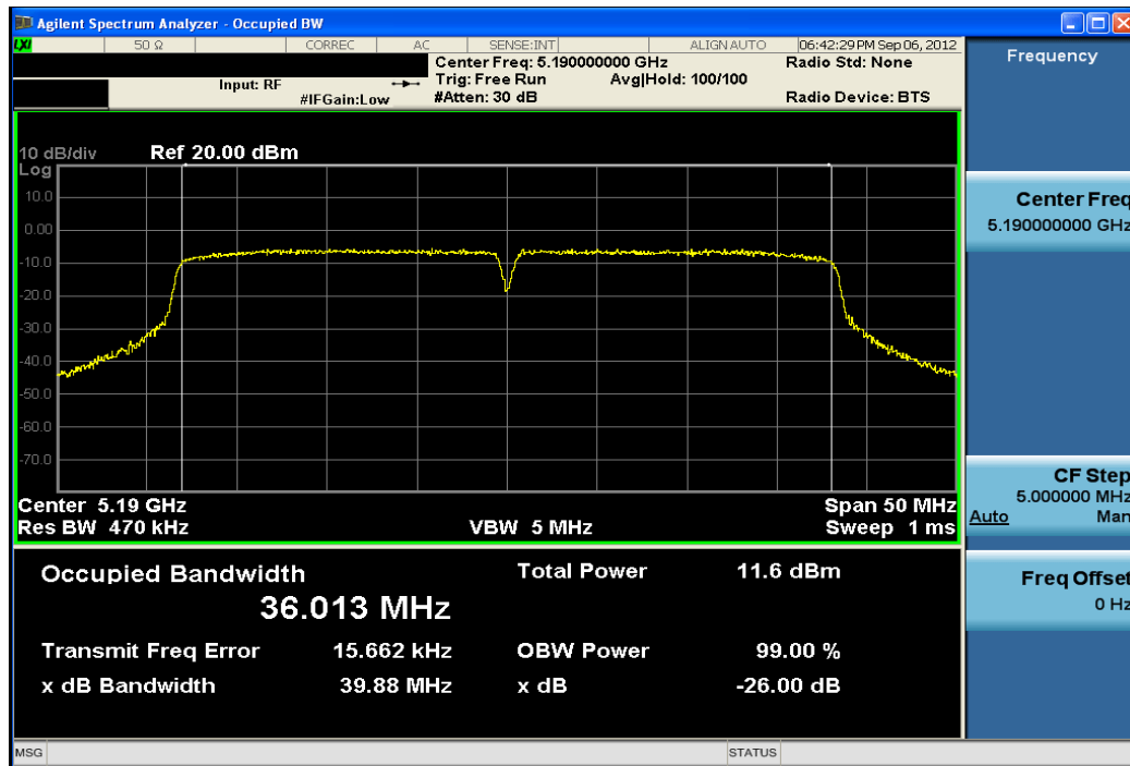
Plot 6-7. 26dB Bandwidth Plot (40MHz BW 802.11n (UNII Band 1) – Ch. 38)
