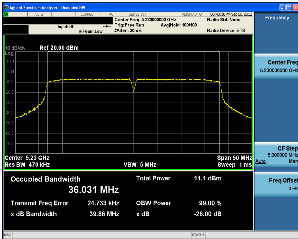
Plot 6-8. 26dB Bandwidth Plot (40MHz BW 802.11n (UNII Band 1) – Ch. 46)
