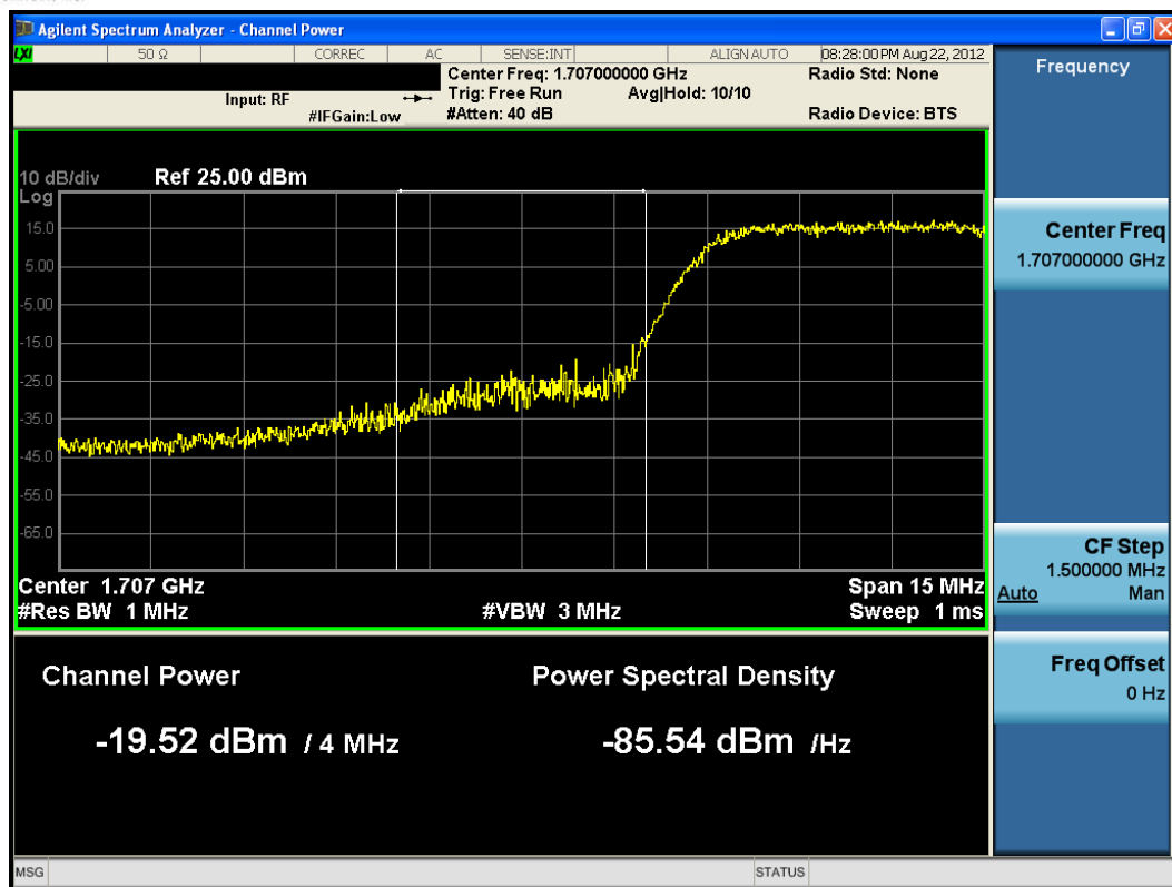
Plot 9-4. Lower Extended Band Edge Plot (5MHz QPSK– RB Size 25)
