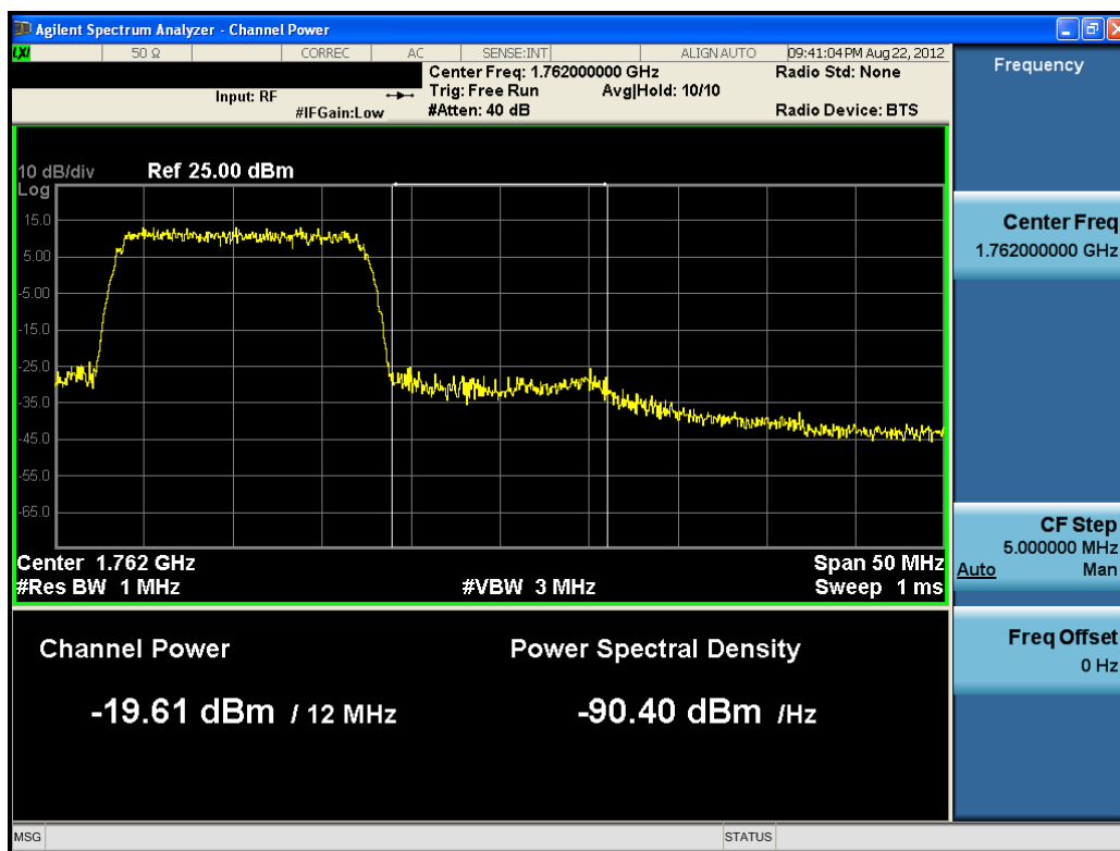
Plot 9-24. Upper Extended Band Edge Plot (15MHz QPSK– RB Size 75, Offset 0)
