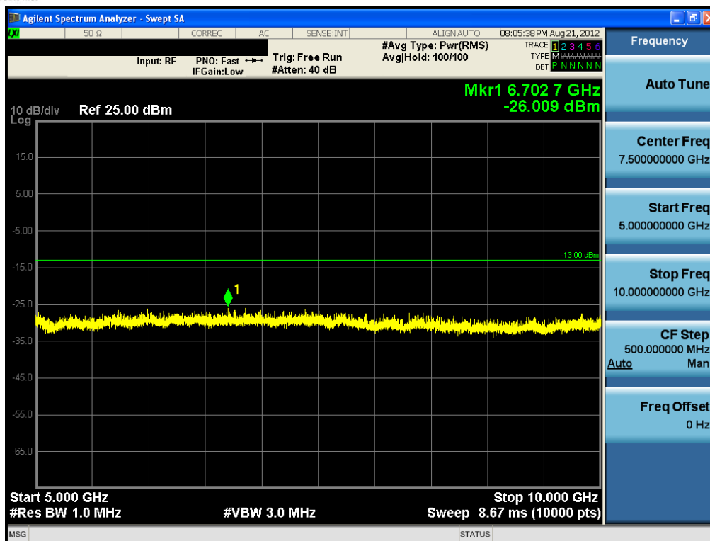
Plot 7-10. Conducted Spurious Plot (10MHz QPSK – RB Size 1, RB Offset 0 – Mid Channel)
