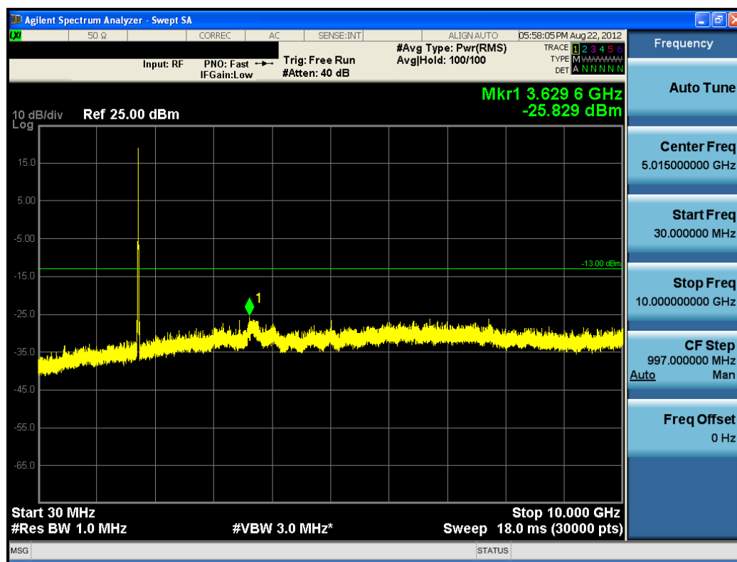
Plot 9-15. Conducted Spurious Plot (10MHz QPSK – RB Size 1, RB Offset 0 – Mid Channel)
