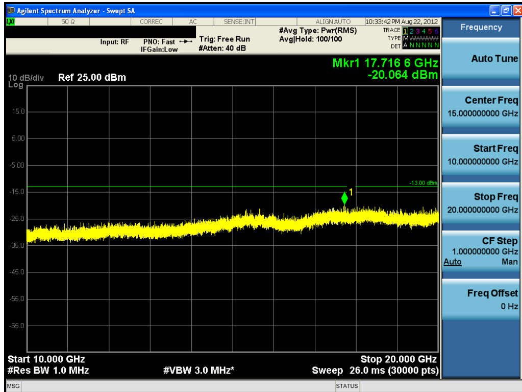
Plot 9-43. Conducted Spurious Plot (QPSK – RB Size 1, RB Offset 0 – High Channel)
