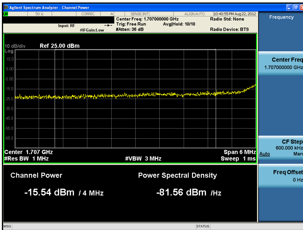
Plot 9-32. Lower Ext. Band Edge Plot (QPSK – RB Size 100)
