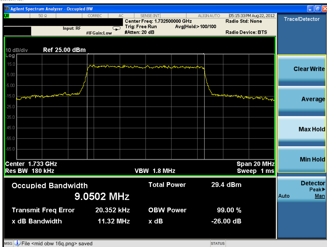
Plot 9-10. Occupied Bandwidth Plot (10MHz 16-QAM – RB Size 50)
