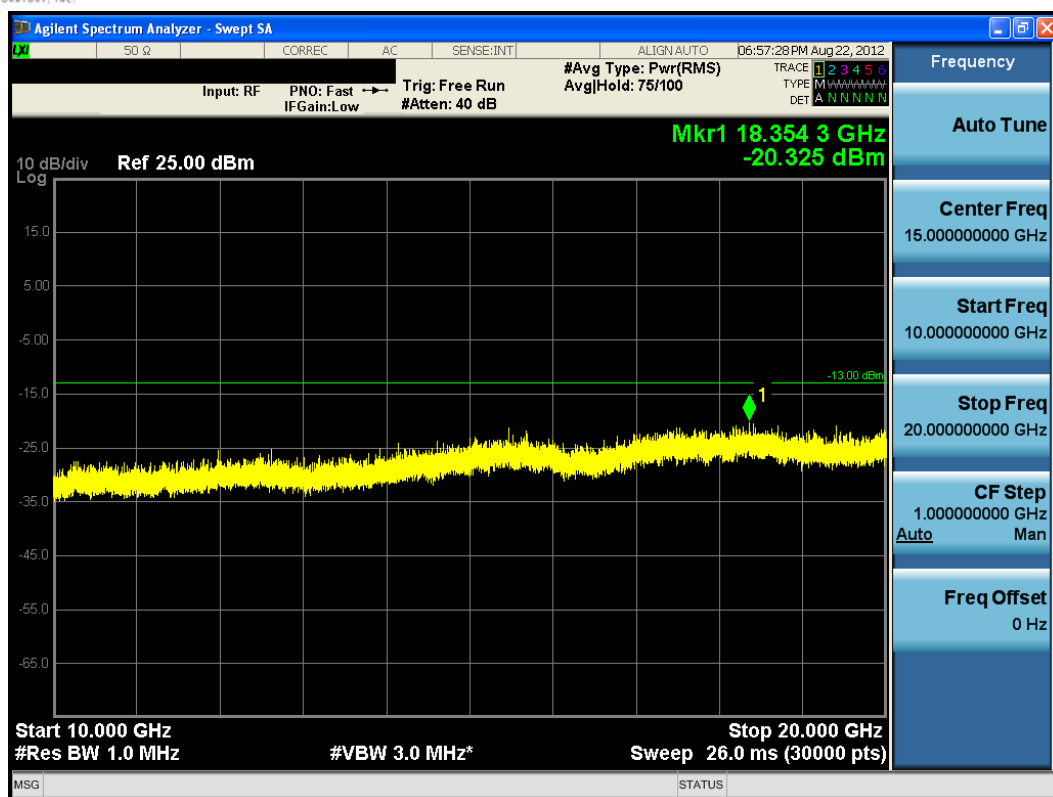
Plot 9-18. Conducted Spurious Plot (10MHz QPSK – RB Size 1, RB Offset 0 – High Channel)
