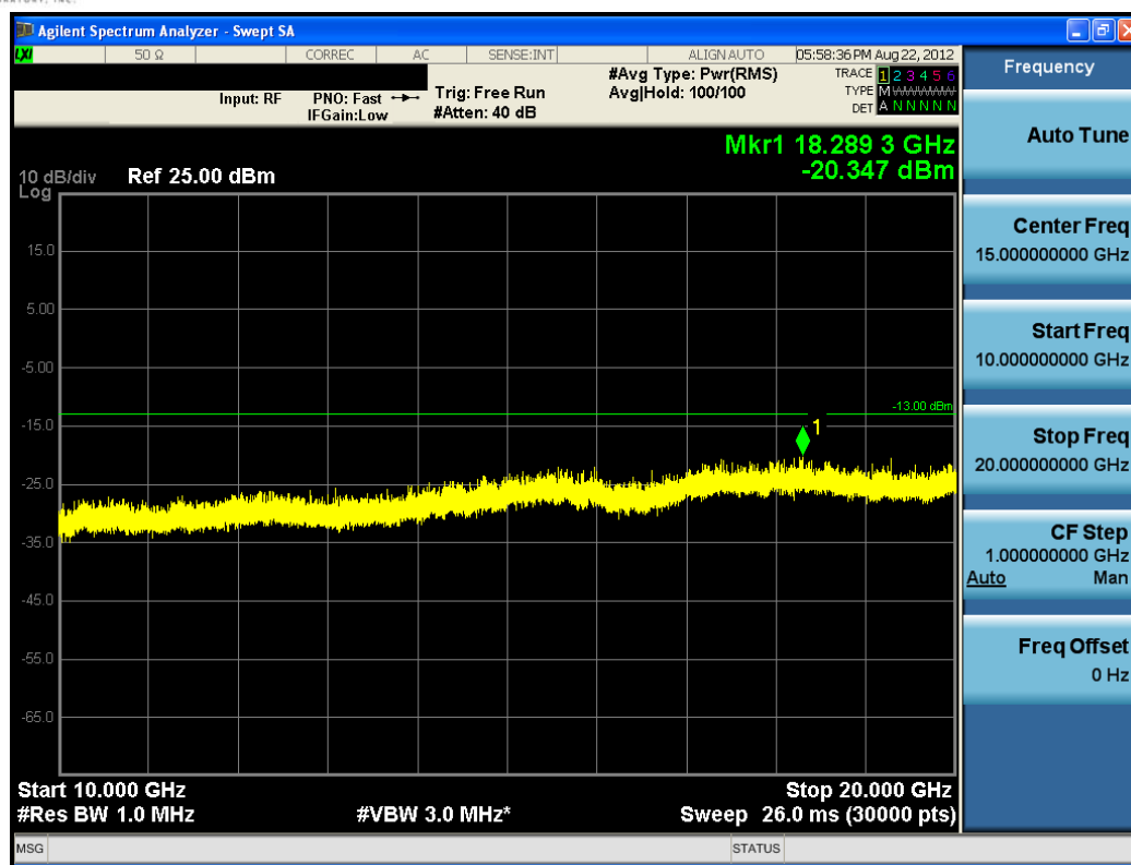
Plot 9-16. Conducted Spurious Plot (10MHz QPSK – RB Size 1, RB Offset 0 – Mid Channel)
