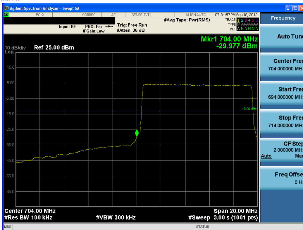
Plot 7-2. Lower Band Edge Plot (10MHz QPSK – RB Size 50)
