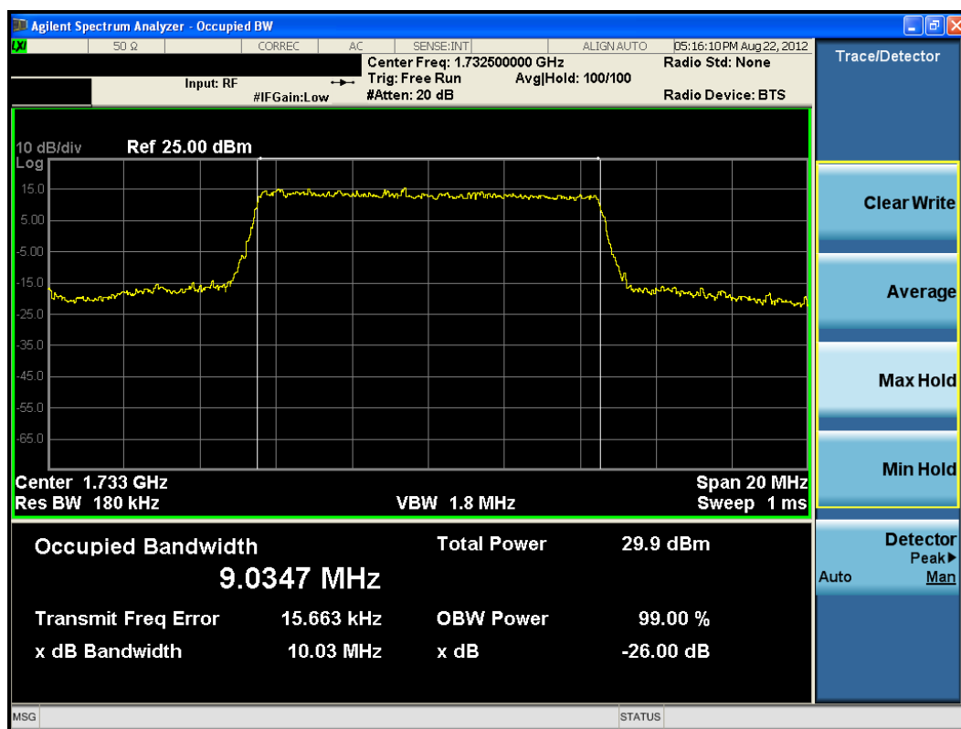
Plot 9-9. Occupied Bandwidth Plot (10MHz QPSK – RB Size 50)
