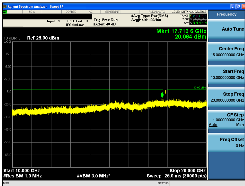
Plot 9-41. Conducted Spurious Plot (QPSK – RB Size 1, RB Offset 0 – Mid Channel)
