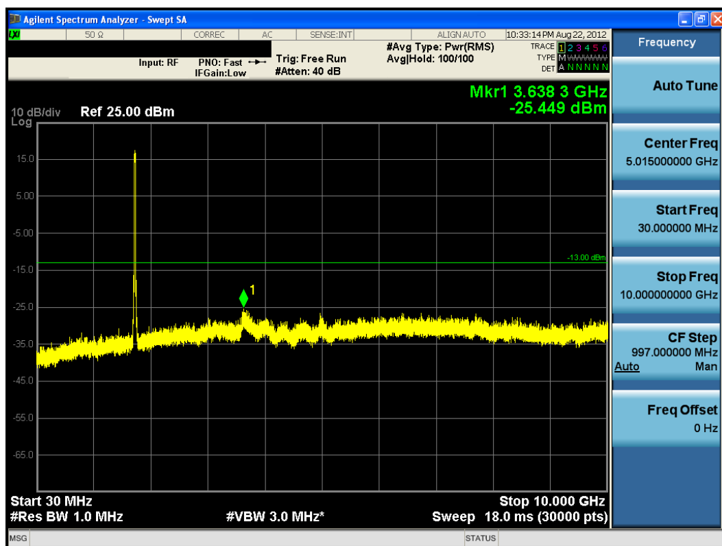
Plot 9-40. Conducted Spurious Plot (QPSK – RB Size 1, RB Offset 0 – Mid Channel)
