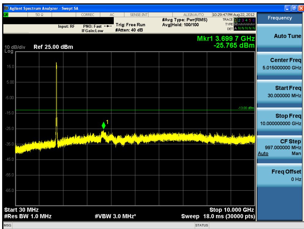
Plot 9-42. Conducted Spurious Plot (QPSK – RB Size 1, RB Offset 0 – High Channel)
