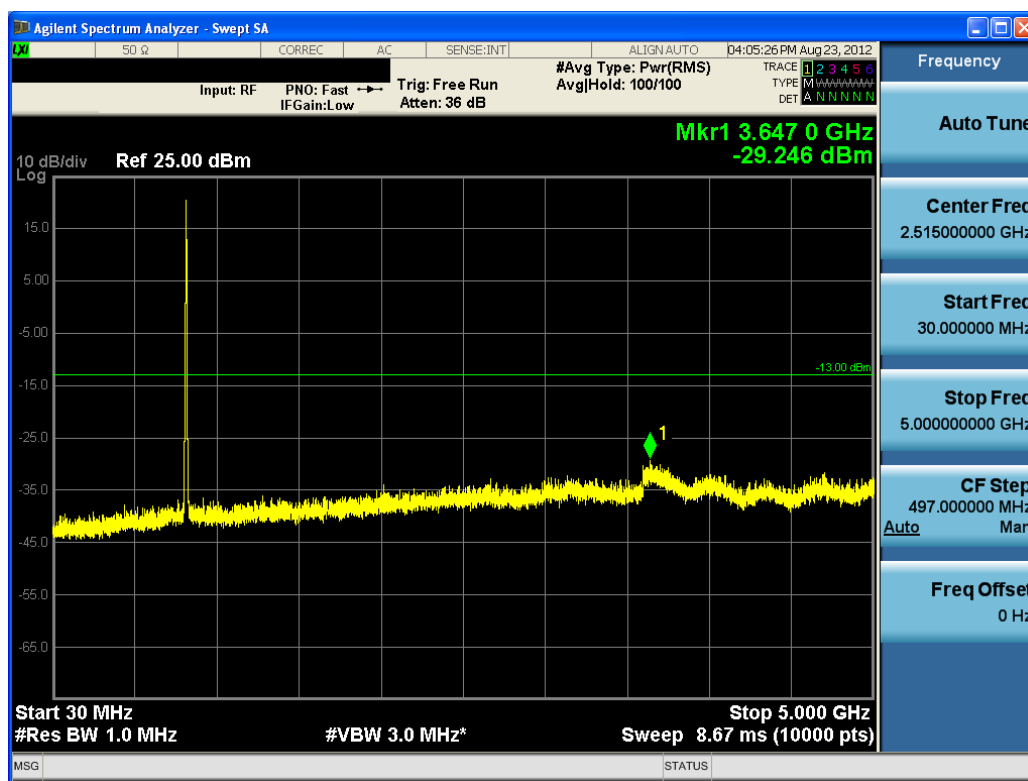
Plot 8-11. Conducted Spurious Plot (5MHz QPSK – RB Size 1, RB Offset 0 – Mid Channel)
