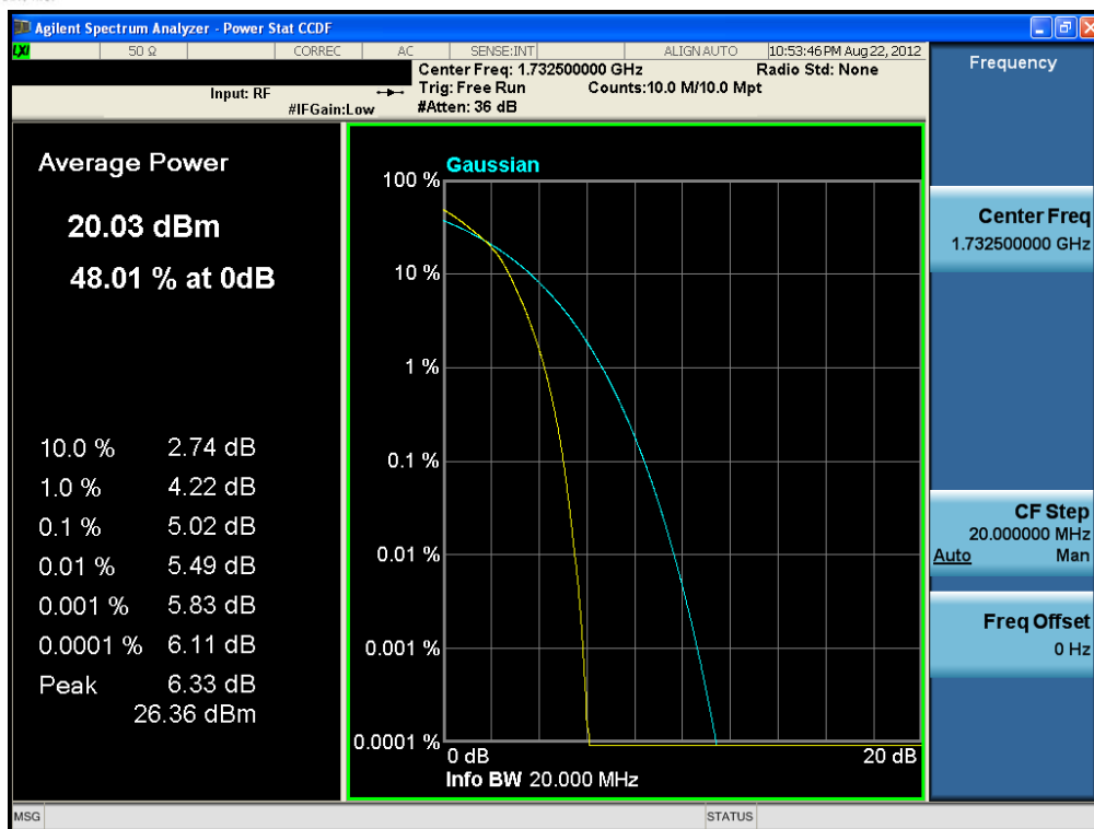
Plot 9-37. Peak to Average Ratio Plot (16QAM – RB Size 100)
