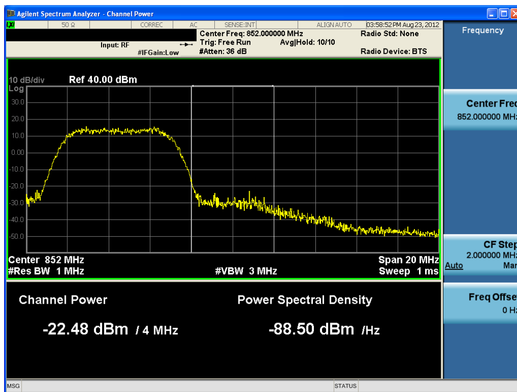
Plot 8-17. Upper Extended Band Edge Plot (5MHz QPSK – RB Size 25)
