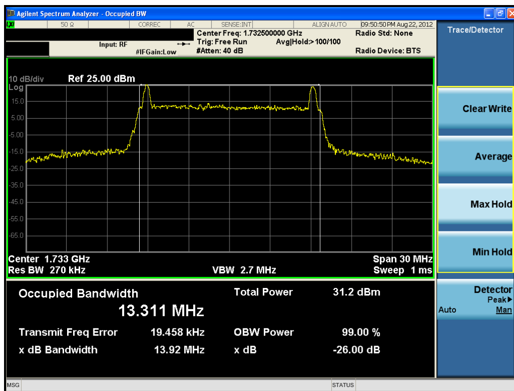
Plot 9-12. Occupied Bandwidth Plot (15MHz 16-QAM – RB Size 75)
