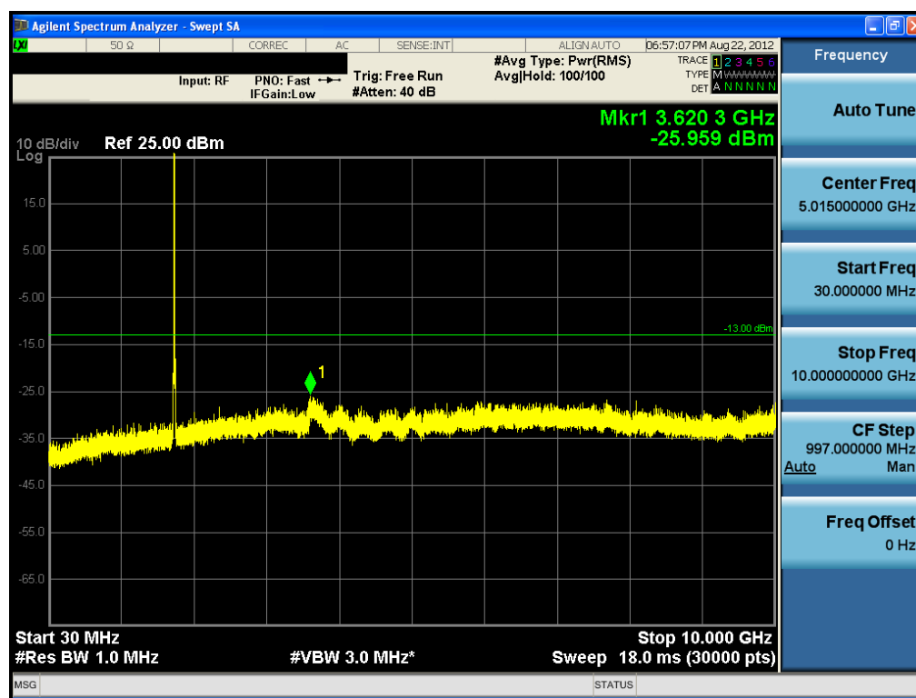
Plot 9-17. Conducted Spurious Plot (10MHz QPSK – RB Size 1, RB Offset 0 – High Channel)
