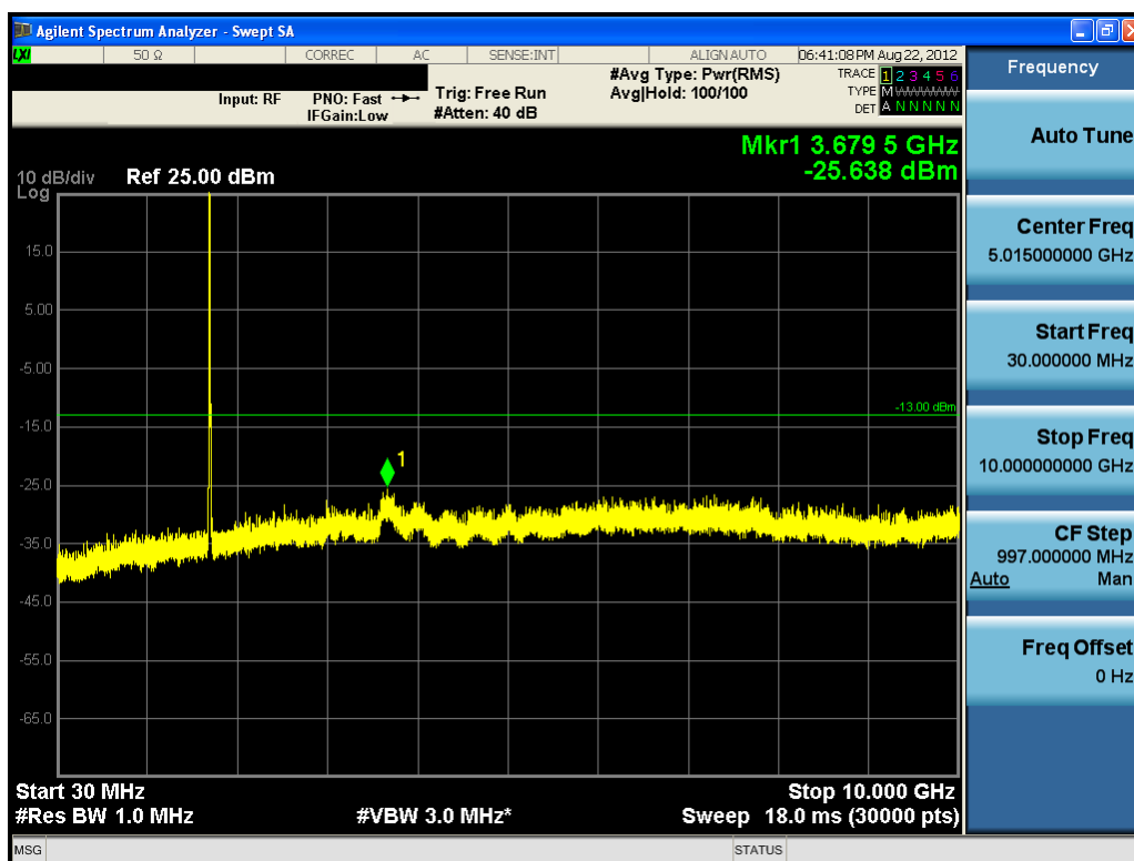
Plot 9-13. Conducted Spurious Plot (10MHz QPSK – RB Size 1, RB Offset 0 – Low Channel)
