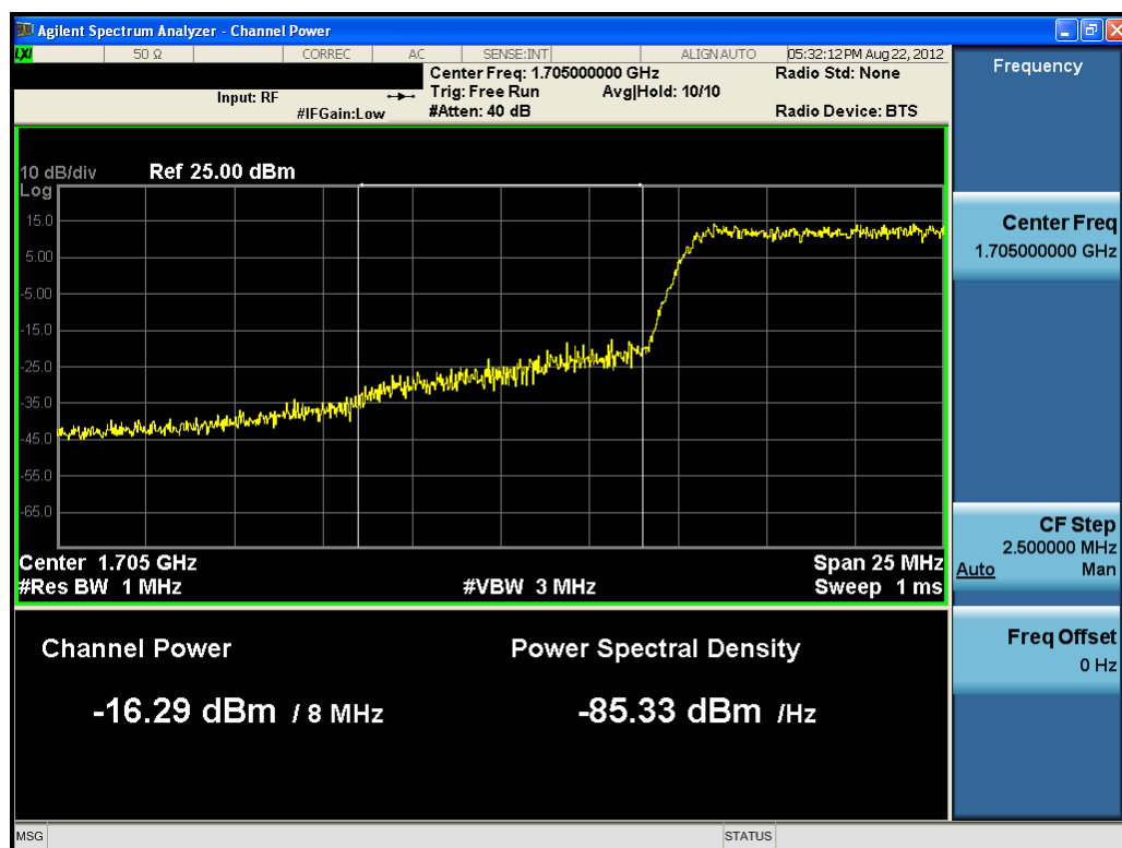
Plot 9-5. Lower Extended Band Edge Plot (10MHz QPSK– RB Size 50)
