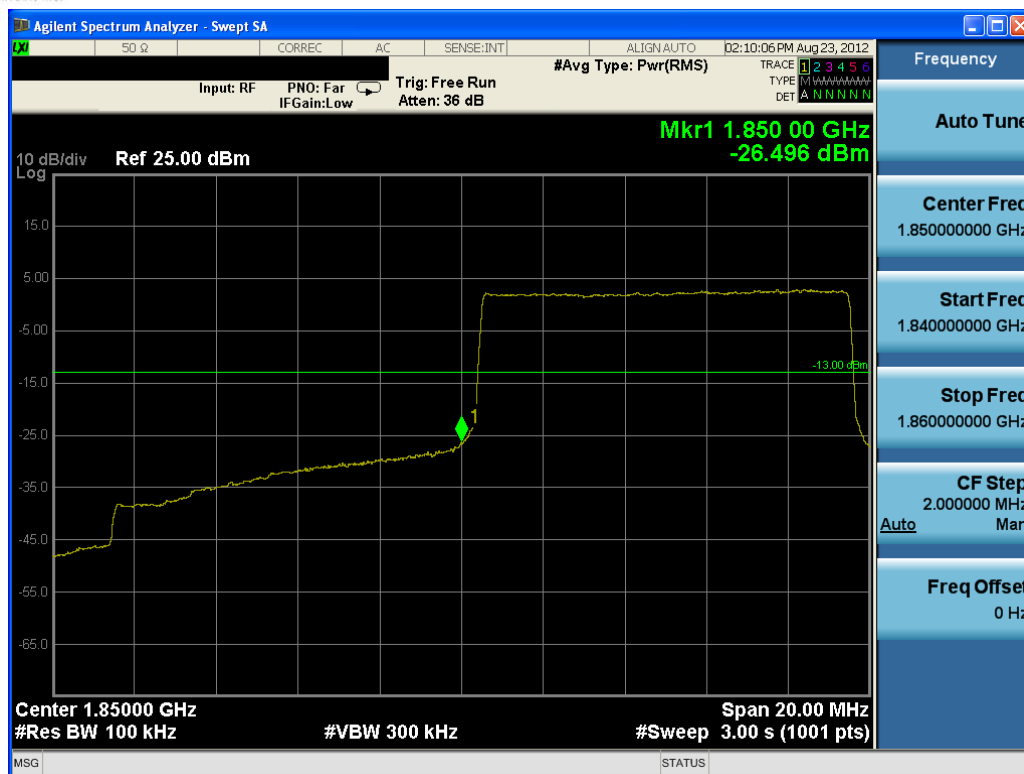
Plot 10-2. Lower Band Edge Plot (10MHz QPSK – RB Size 50)
