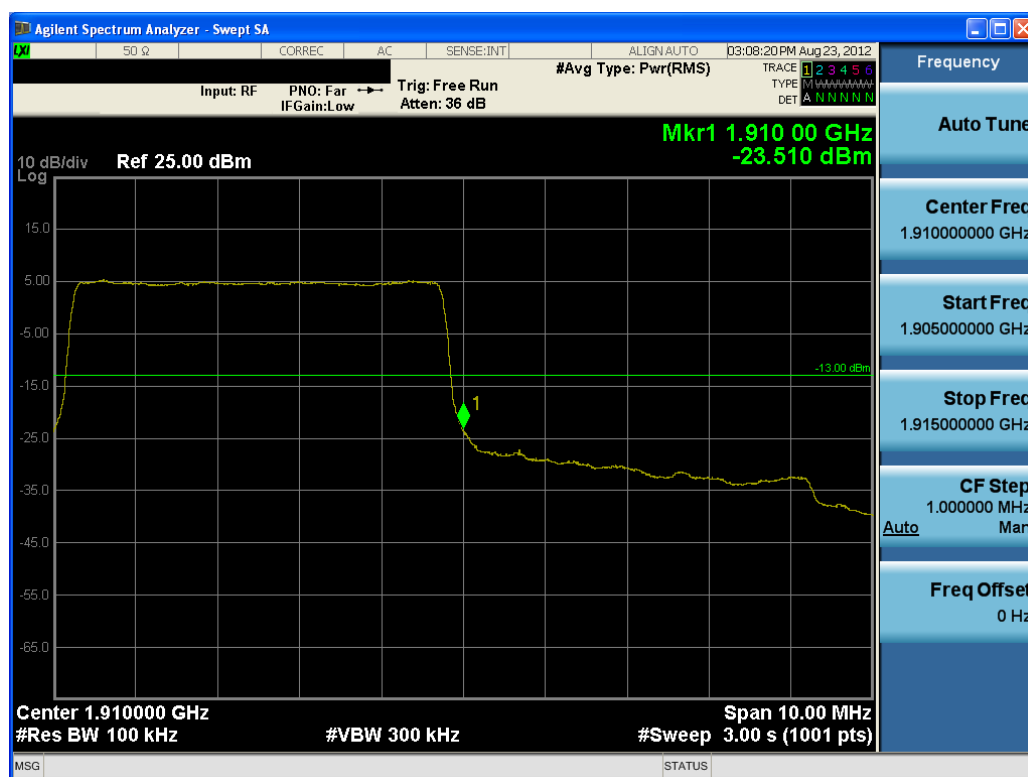
Plot 10-15. Upper Band Edge Plot (5MHz QPSK – RB Size 25)
