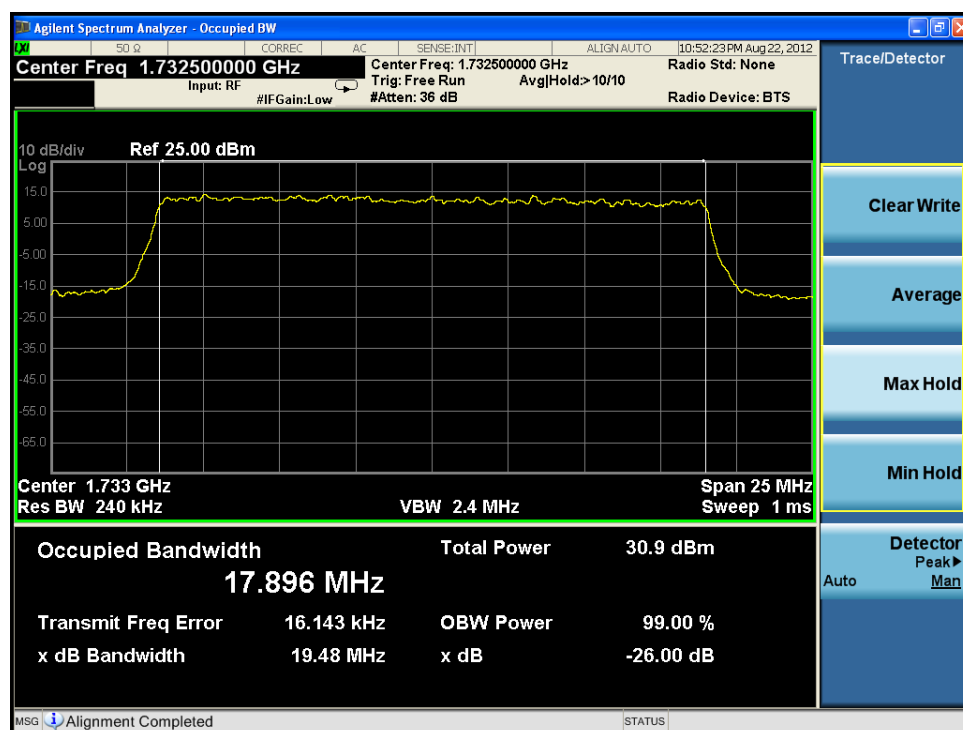
Plot 9-34. Occupied Bandwidth Plot (QPSK – RB Size 100)
