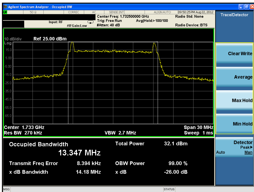
Plot 9-11. Occupied Bandwidth Plot (15MHz QPSK – RB Size 75)
