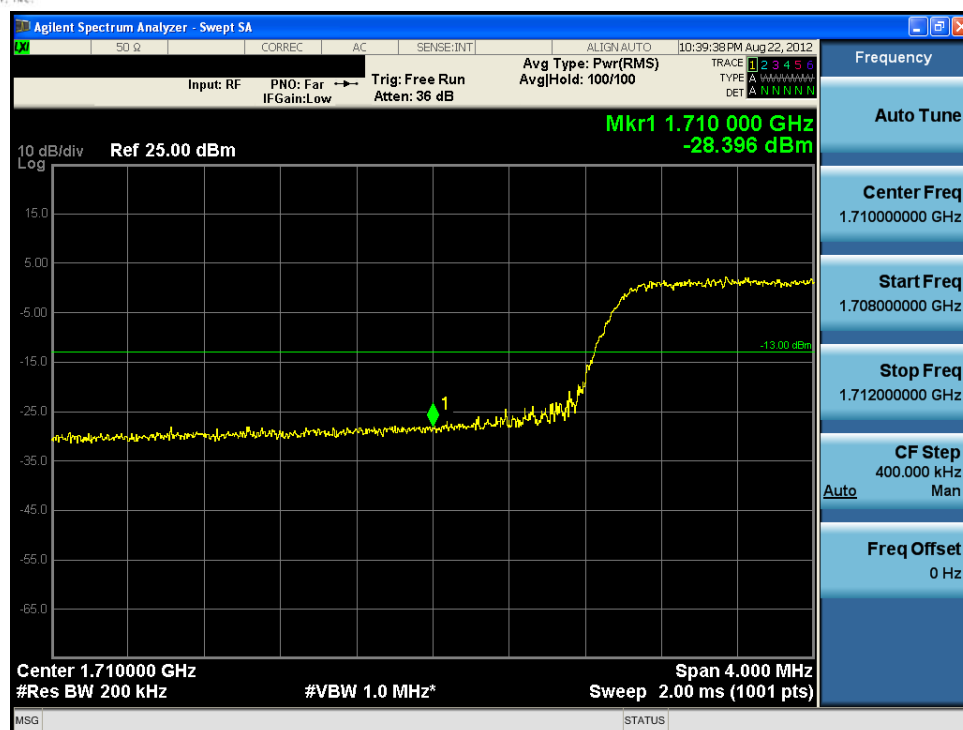
Plot 9-33. Lower Band Edge Plot (QPSK – RB Size 100)
