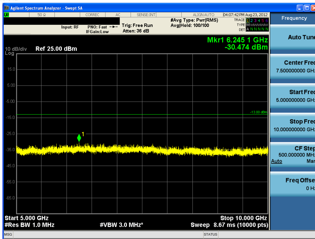
Plot 8-14. Conducted Spurious Plot (50MHz QPSK – RB Size 1, RB Offset 0 – High Channel)
