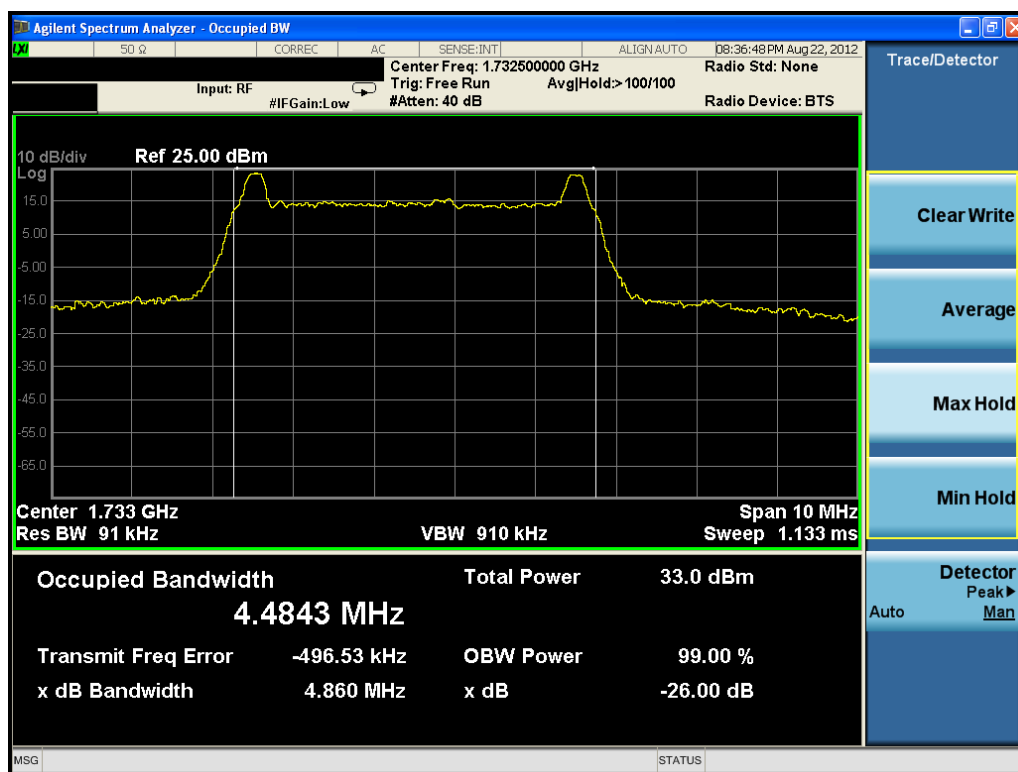
Plot 9-7. Occupied Bandwidth Plot (5MHz QPSK – RB Size 25)
