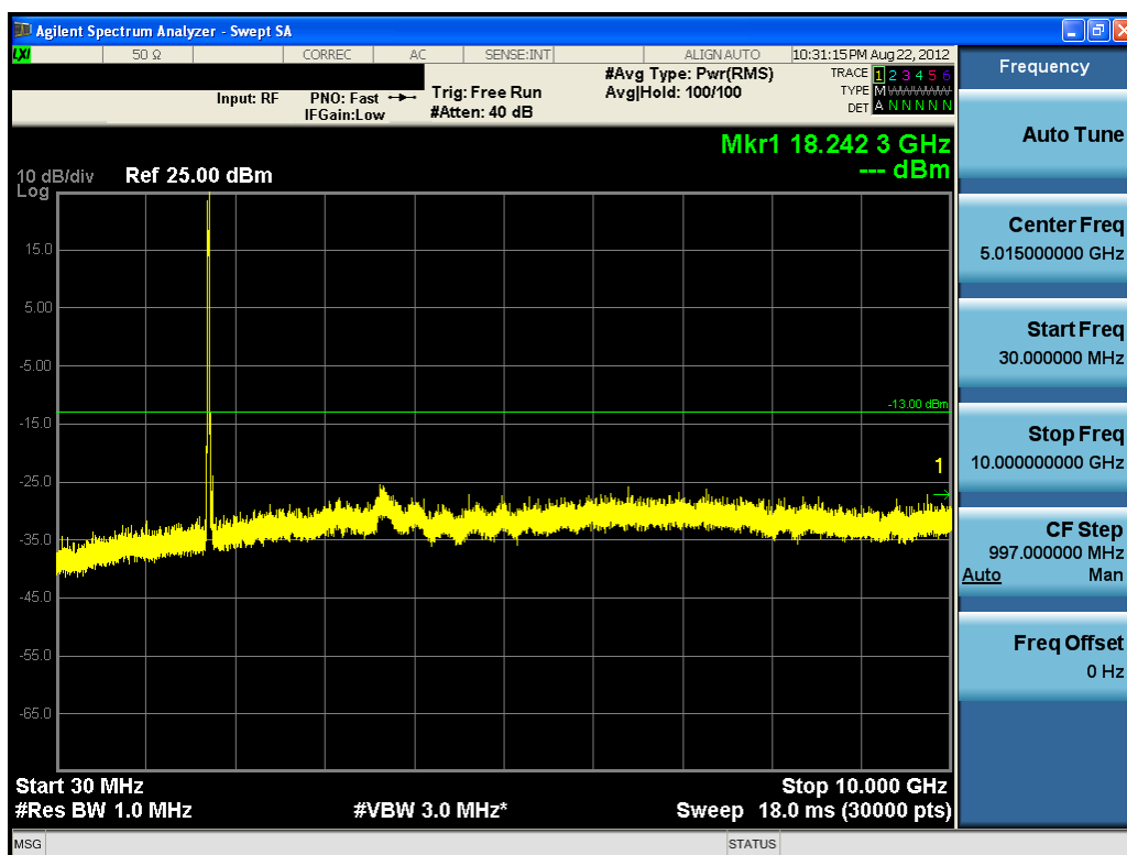
Plot 9-38. Conducted Spurious Plot (QPSK – RB Size 1, RB Offset 0 – Low Channel)
