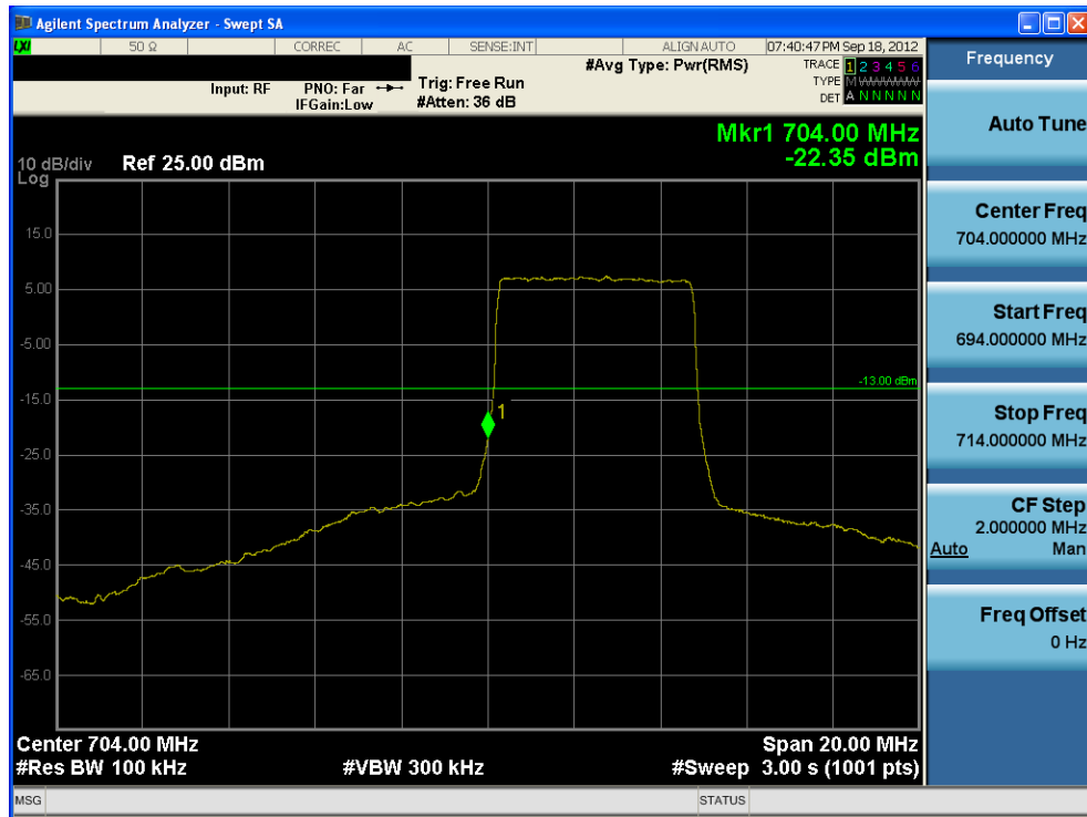
Plot 7-1. Lower Band Edge Plot (5MHz QPSK – RB Size 25)
