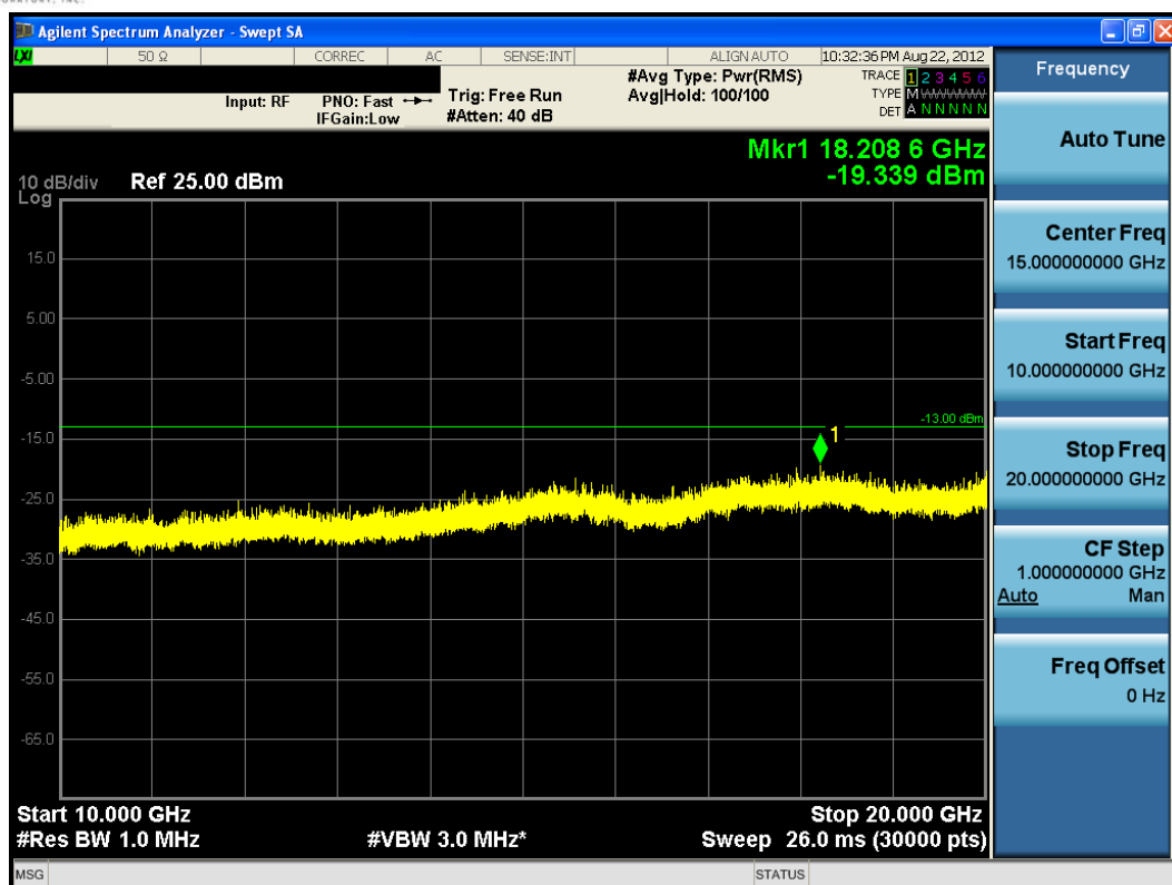
Plot 9-39. Conducted Spurious Plot (QPSK – RB Size 1, RB Offset 0 – Low Channel)
