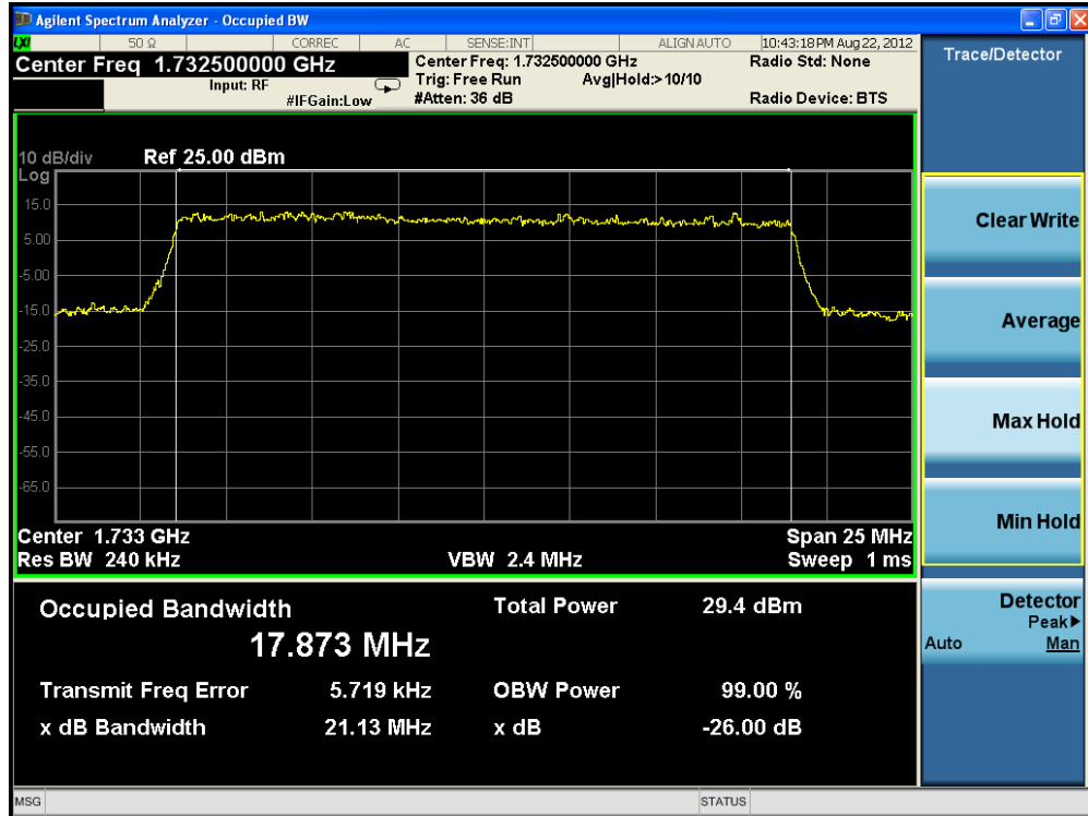
Plot 9-35. Occupied Bandwidth Plot (16-QAM – RB Size 100)
