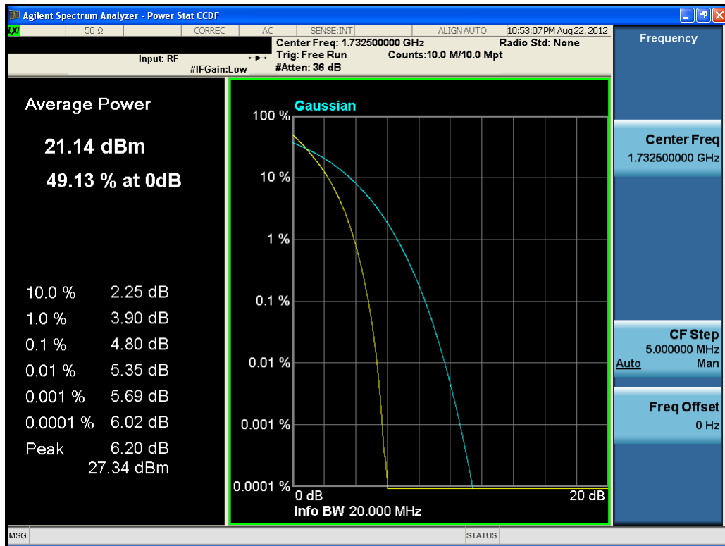
Plot 9-36. Peak to Average Ratio Plot (QPSK – RB Size 100)
