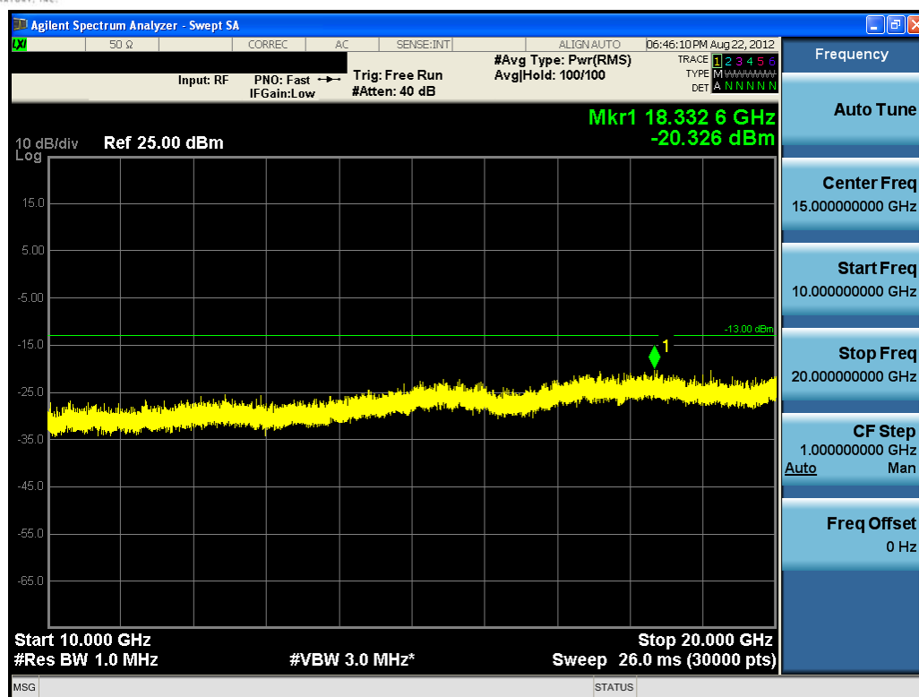
Plot 9-14. Conducted Spurious Plot (10MHz QPSK – RB Size 1, RB Offset 0 – Low Channel)
