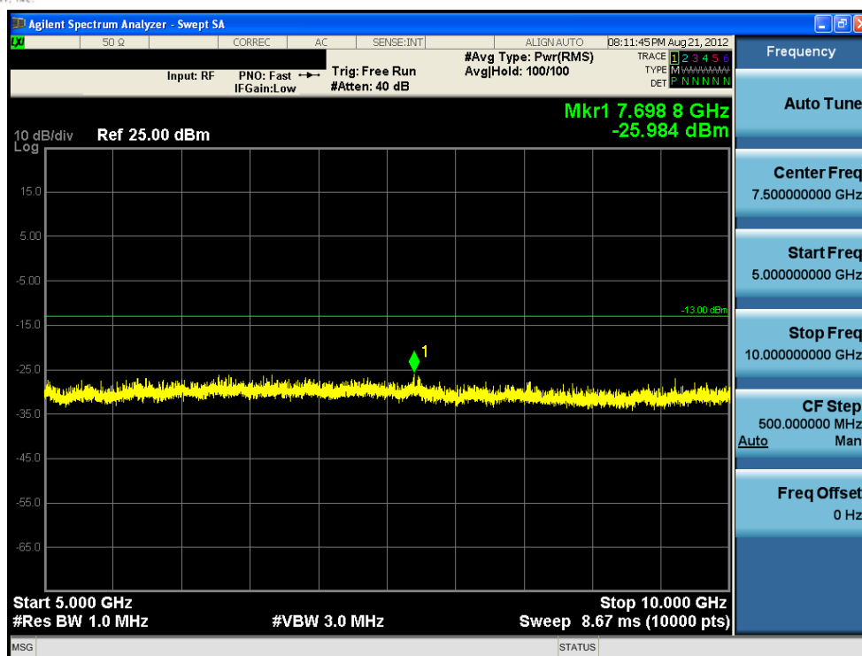
Plot 7-8. Conducted Spurious Plot (10MHz QPSK – RB Size 1, RB Offset 0 – Low Channel)
