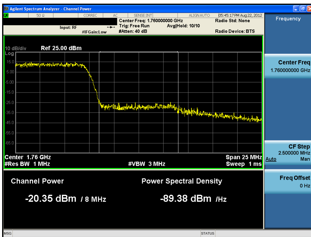
Plot 9-23. Upper Extended Band Edge Plot (10MHz QPSK- RB Size 50)
