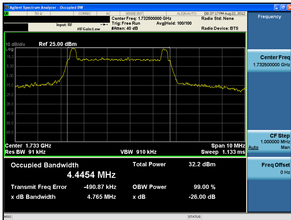
Plot 9-8. Occupied Bandwidth Plot (5MHz 16-QAM – RB Size 25)
