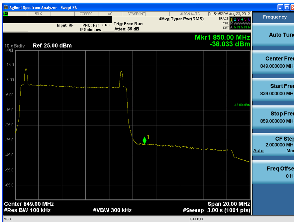
Plot 8-16. Upper Band Edge Plot (10MHz QPSK – RB Size 50)
