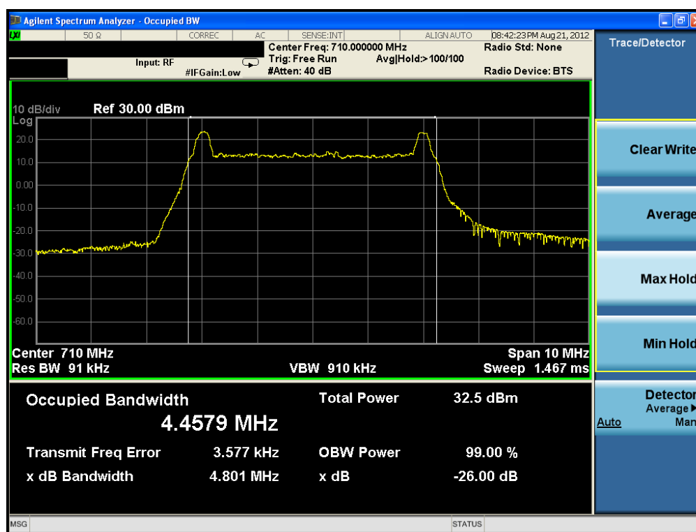
Plot 7-3. Occupied Bandwidth Plot (5MHz QPSK – RB Size 25)
