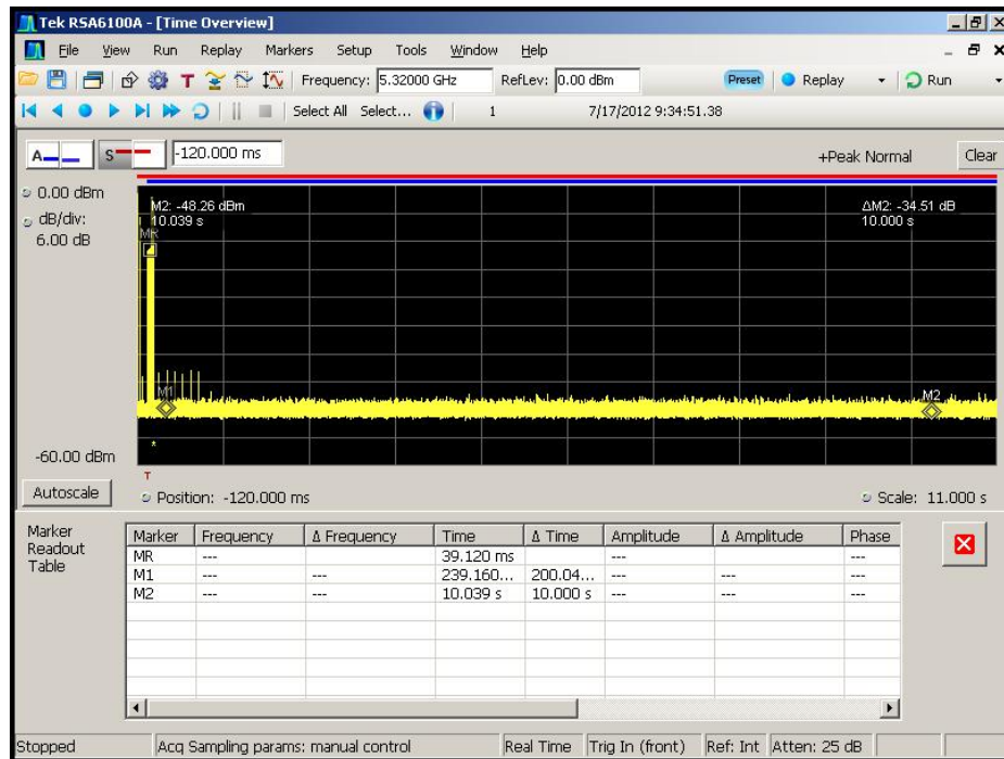
Figure 5-5. Channel Move Time (< 10sec)
