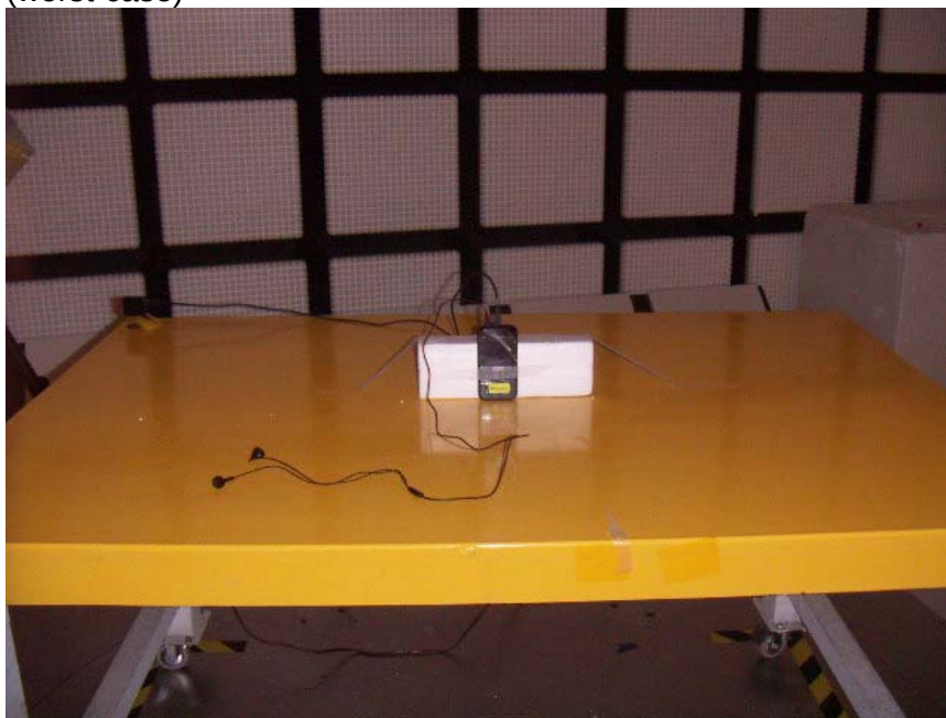
Y-AXIS WITH AC ADAPTER & EAR PHONE_ FRONT PHOTO (worst-case)
