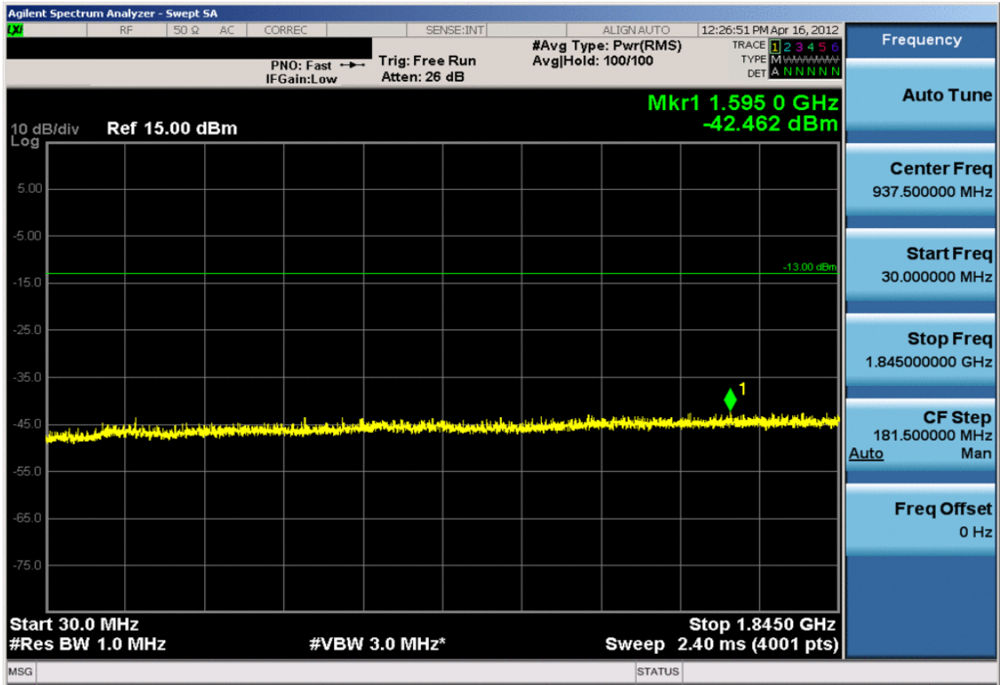
Plot 7-39. Conducted Spurious Plot (PCS WCDMA Mode – Ch. 9538)
