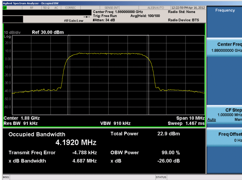
Plot 7-37. Occupied Bandwidth Plot (PCS WCDMA Mode – Ch. 9400)
