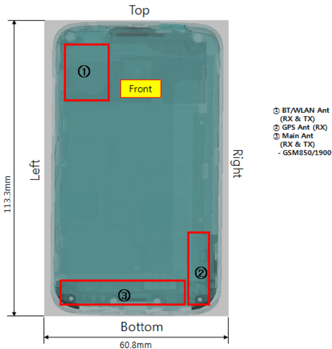
Figure 12.1 Identification of Sides for SAR Testing
