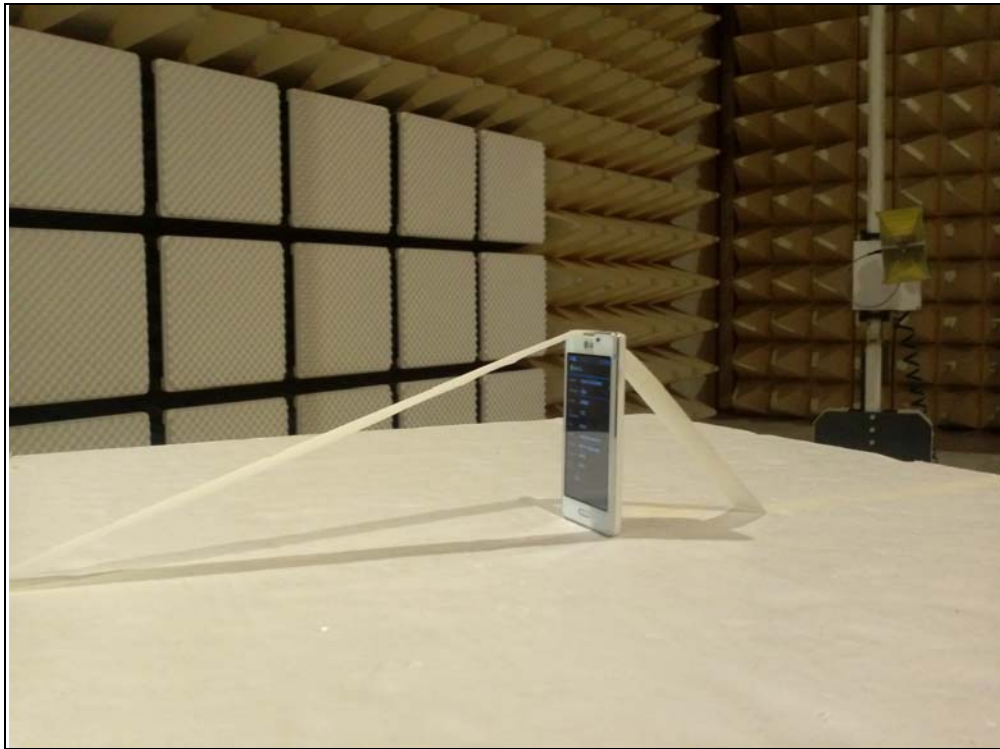
B. Photo of Radiated output power & Spurious Emission Test (BT)
