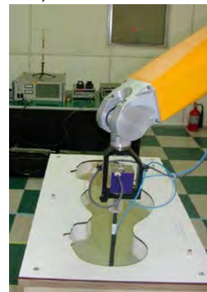
Figure 4.2 Photograph of the probe and the Phantom
