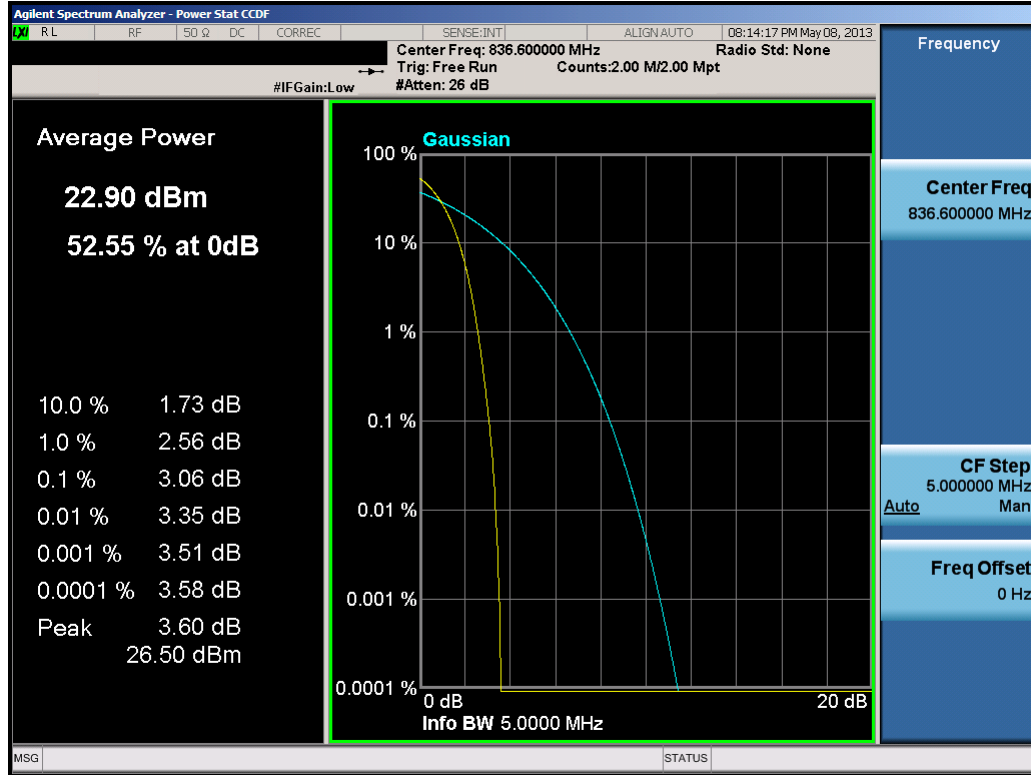
Plot 7-30. Peak-Average Ratio Plot (Cellular WCDMA Mode – Ch. 4183)
