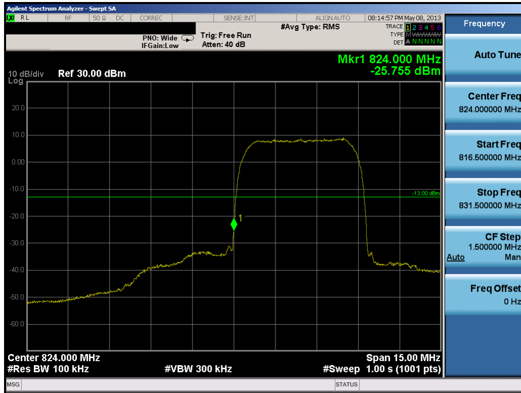
Plot 7-26. Band Edge Plot (Cellular WCDMA Mode – Ch. 4132)
