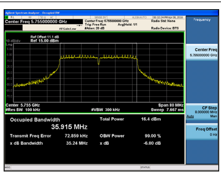
802.11ac_VHT40 BW UNII 3 BAND 6dB Bandwidth(CH.151)
