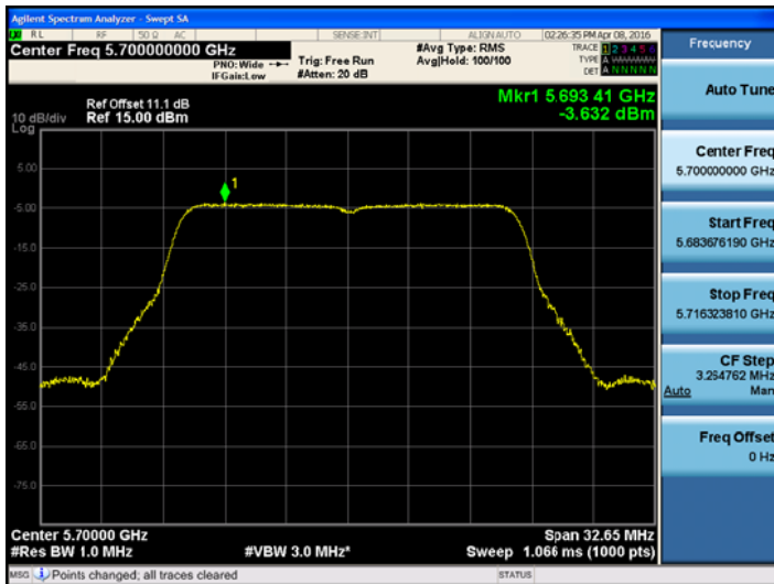
802.11n_HT20 BW UNII 2C BAND PSD CH 140
