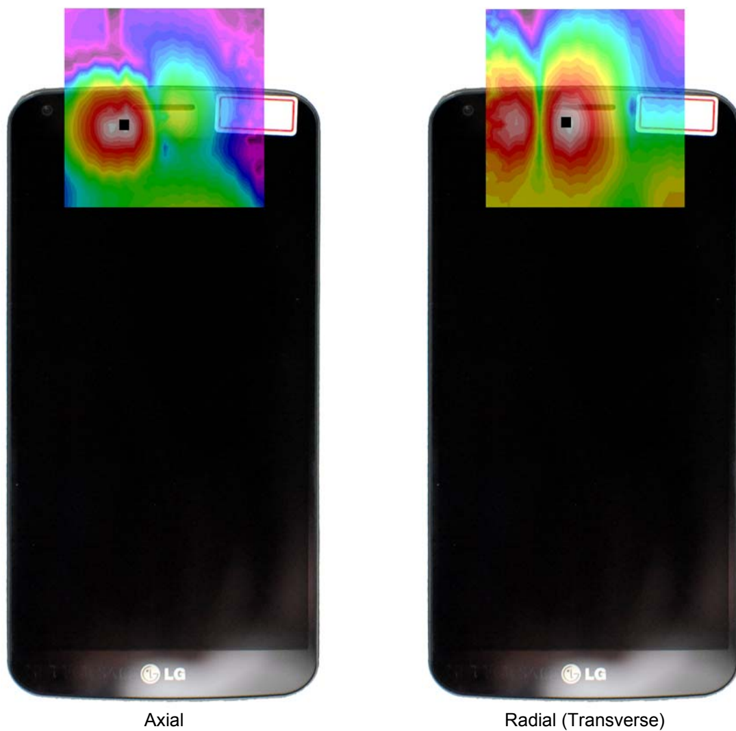
Figure 13-3 T-Coil Scan Overlay Magnetic Field Distributions
