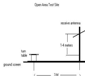
Figure 3-1. Diagram of 3-meter Test Range
