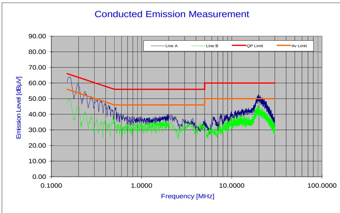
Plot 6-87. Line Conducted Plot with 802.11a UNII Band 4
