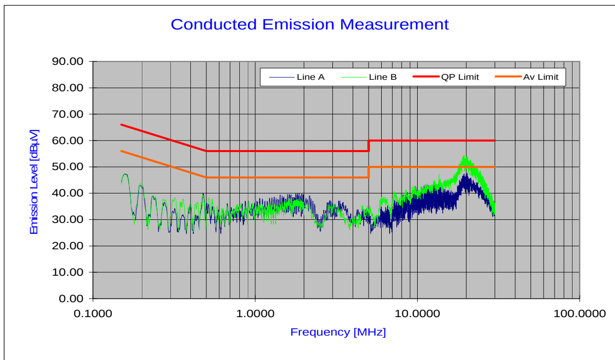
Plot 6-84. Line Conducted Plot with 802.11a UNII Band 2
