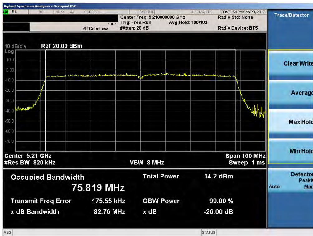
Plot 6-9. 26dB Bandwidth Plot (802.11ac (UNII Band 1) – Ch. 42)
