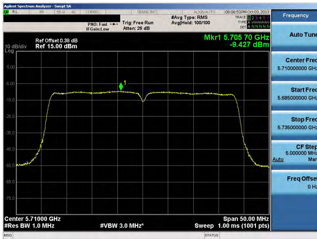
Plot 6-67. Peak Power Spectral Density Plot (40MHz BW 802.11n (UNII Band 3) – Ch. 142)
