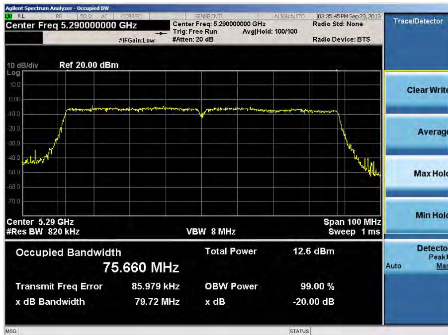
Plot 6-40 A. 20dB Bandwidth Plot (80MHz BW 802.11n (UNII Band 2) – Ch. 58)
