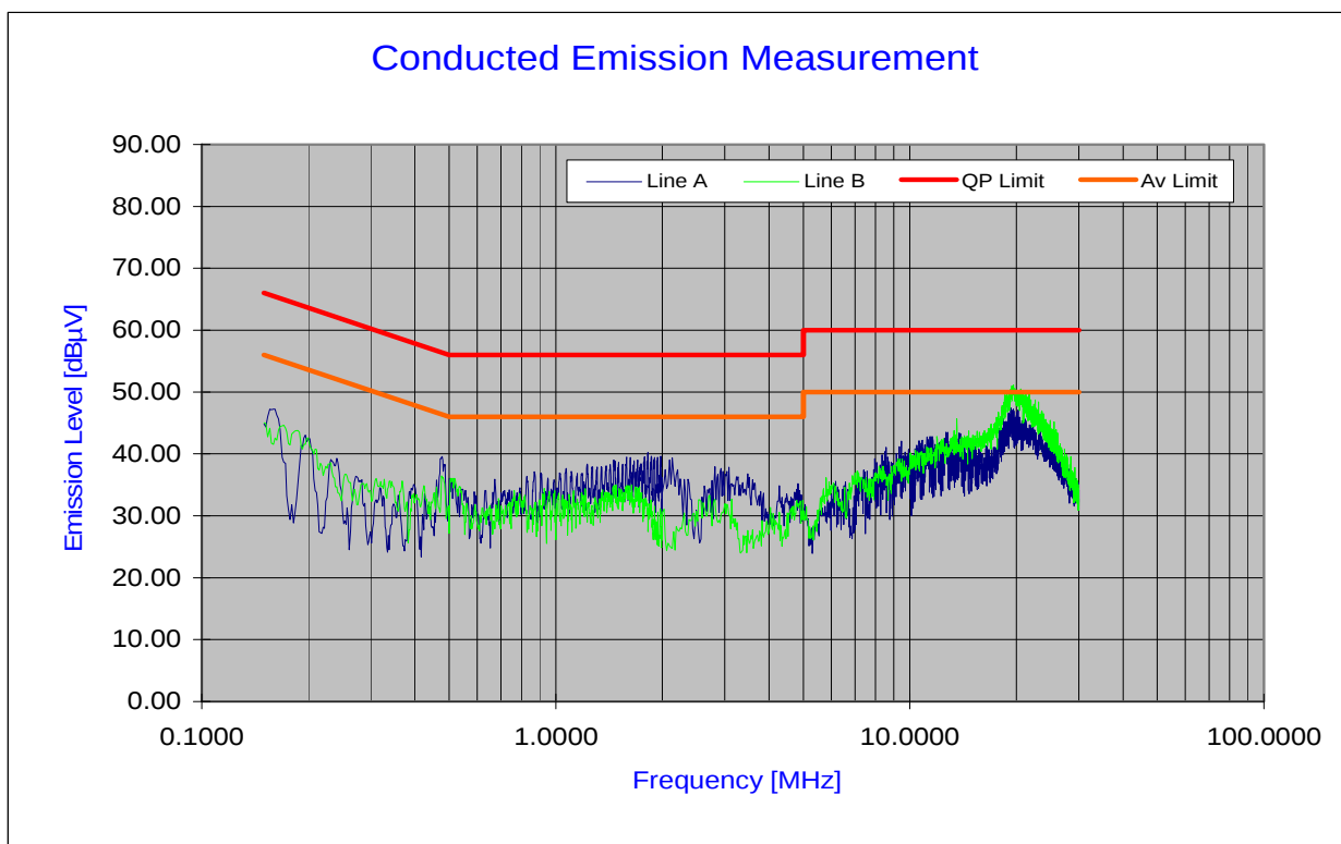
Plot 6-86. Line Conducted Plot with 802.11a UNII Band 3
