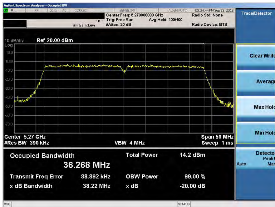
Plot 6-39. 20dB Bandwidth Plot (40MHz BW 802.11n (UNII Band 2) – Ch. 54)
