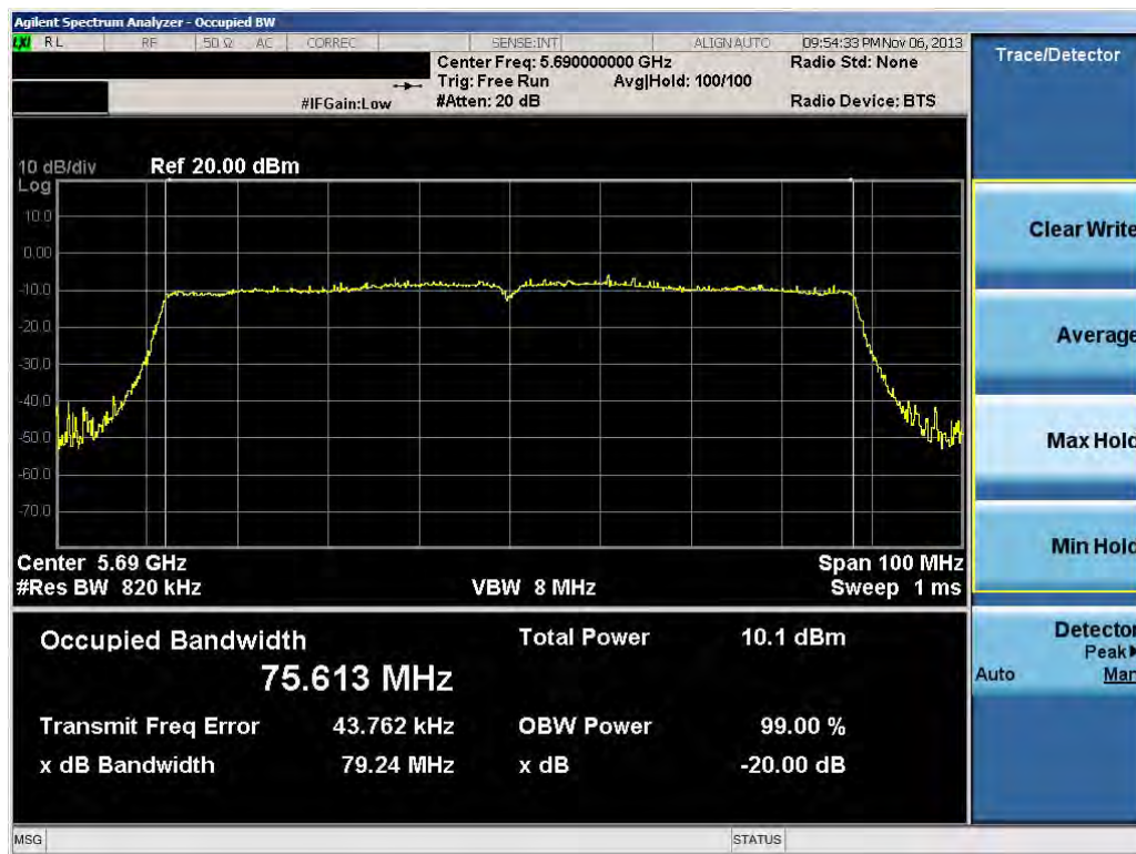
Plot 6-40 B. 20dB Bandwidth Plot (80MHz BW 802.11n (UNII Band 2) – Ch. 138)
