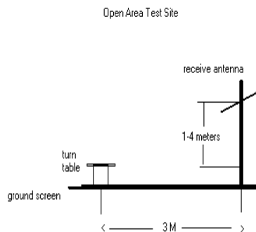
Figure 3-1. Diagram of 3-meter Test Range
