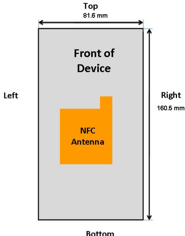
Bottom Figure 1-2 NFC Antenna Locations
