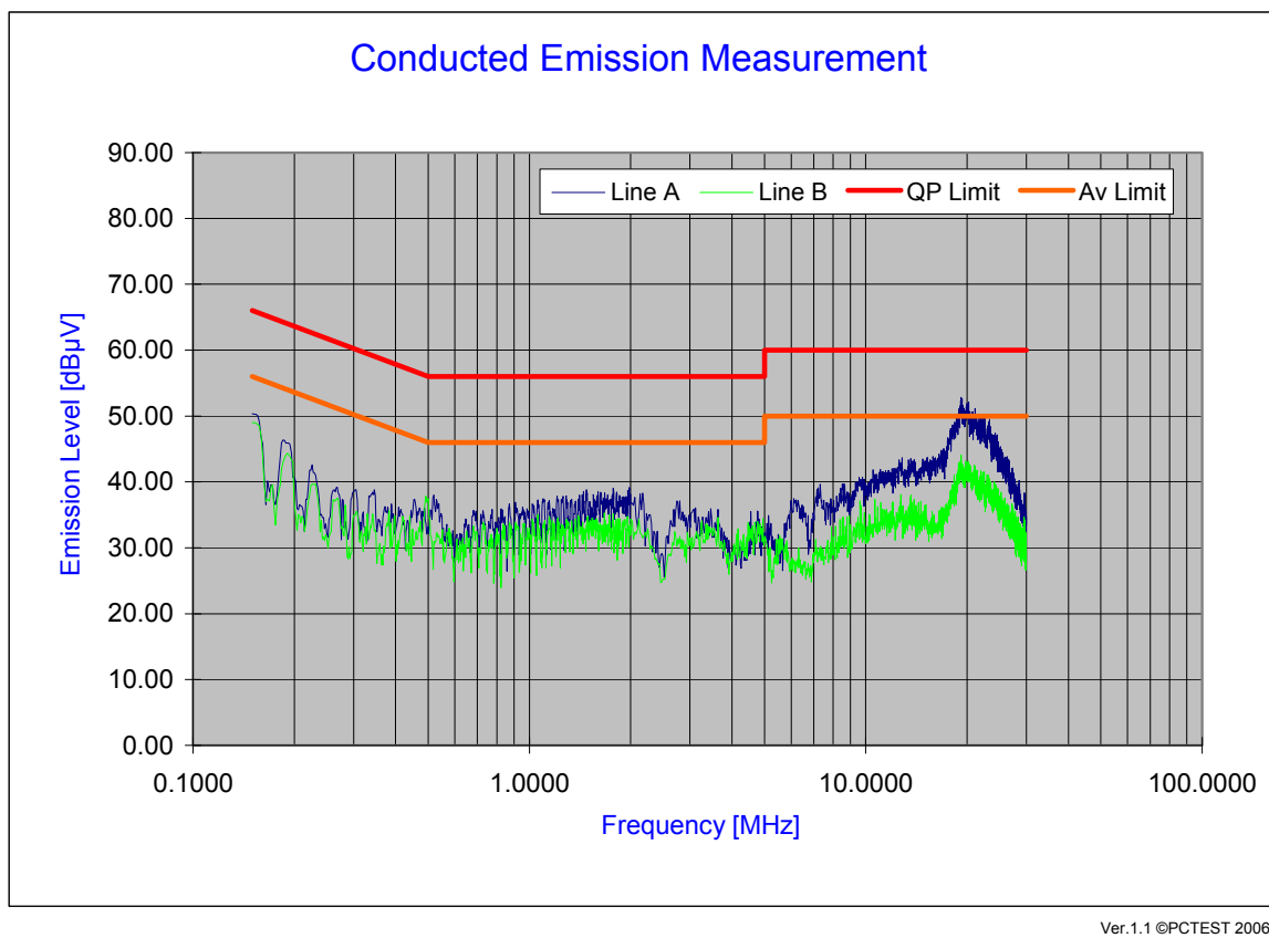
Plot 6-18. Line Conducted Plot with Bluetooth LE (L1)
