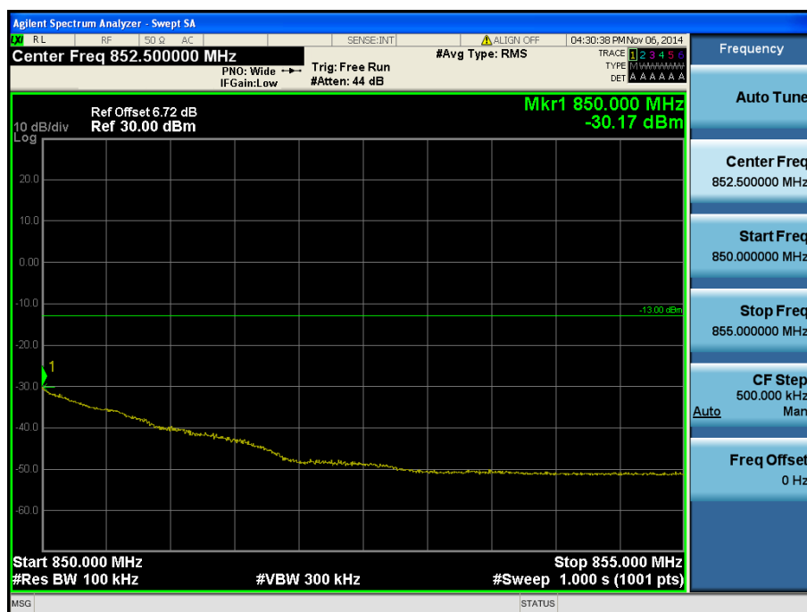
LTE Band 5 / 1.4MHz / QPSK - RB Offset/Size (0/6)
