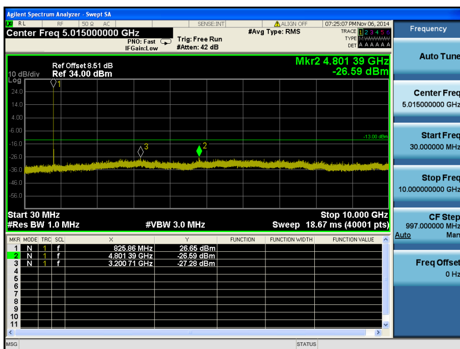
LTE Band 5 / 3MHz / 16QAM - RB Offset/Size (3/8) – Low Channel
