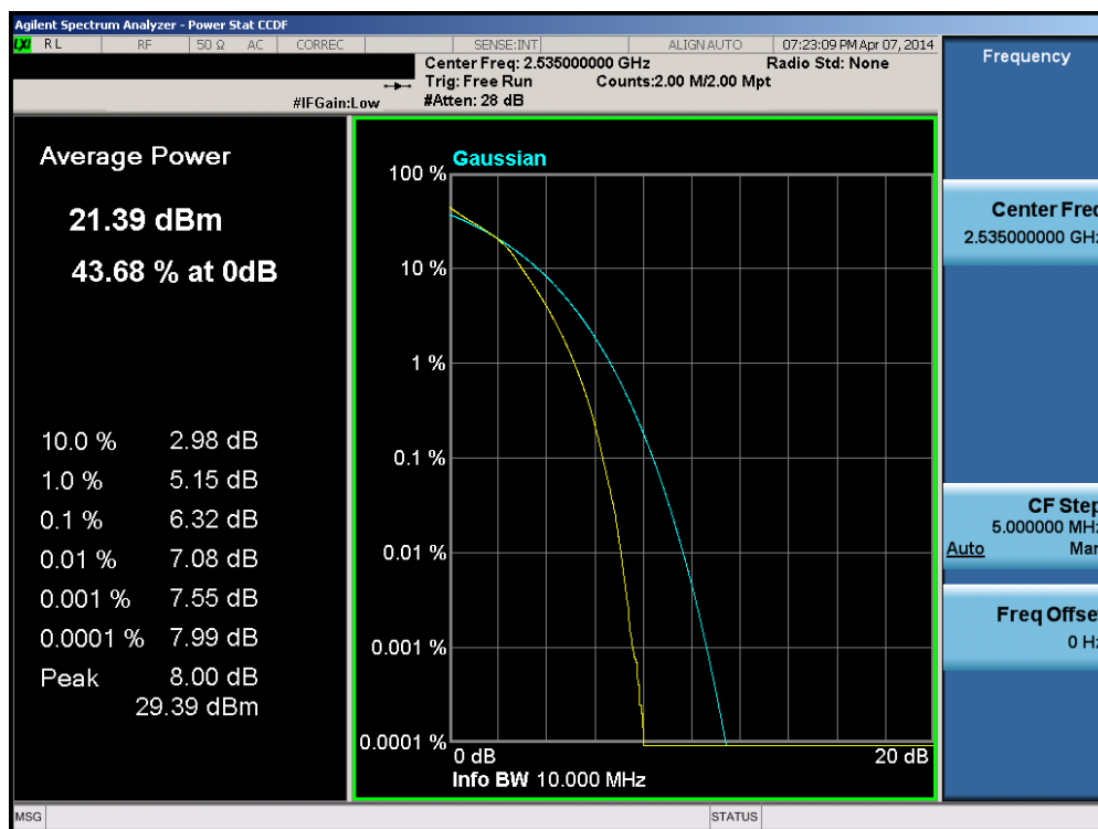
Plot 6-150. PAR Plot (Band 7 – 10.0MHz 16-QAM – RB Size 50)
