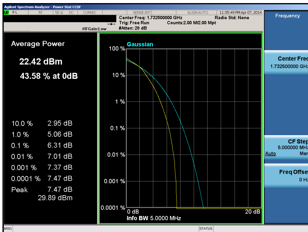
Plot 6-132. PAR Plot (Band 4 – 5.0MHz 16-QAM – RB Size 25)
