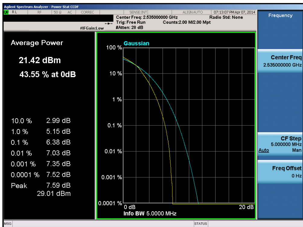
Plot 6-148. PAR Plot (Band 7 – 5.0MHz 16-QAM – RB Size 25)
