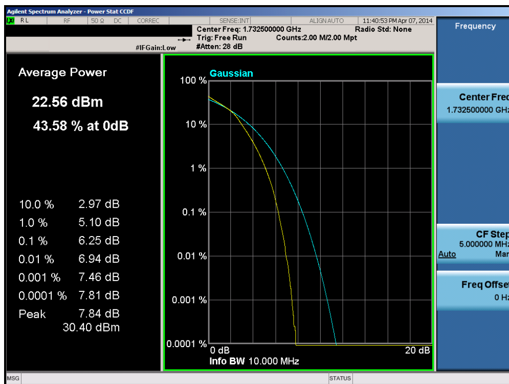
Plot 6-134. PAR Plot (Band 4 – 10.0MHz 16-QAM – RB Size 50)
