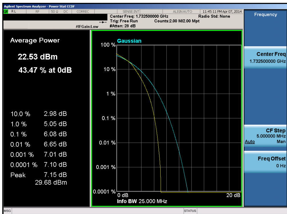
Plot 6-136. PAR Plot (Band 4 – 15.0MHz 16-QAM – RB Size 75)
