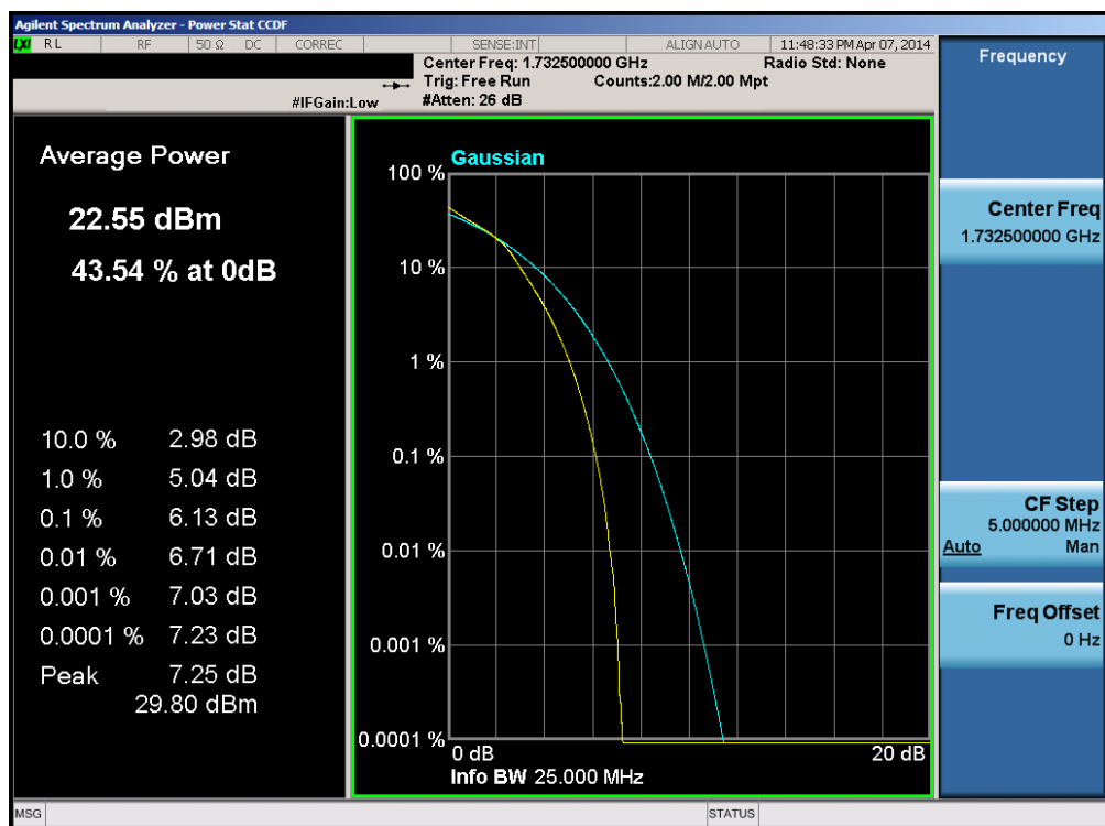
Plot 6-138. PAR Plot (Band 4 – 20.0MHz 16-QAM – RB Size 100)
