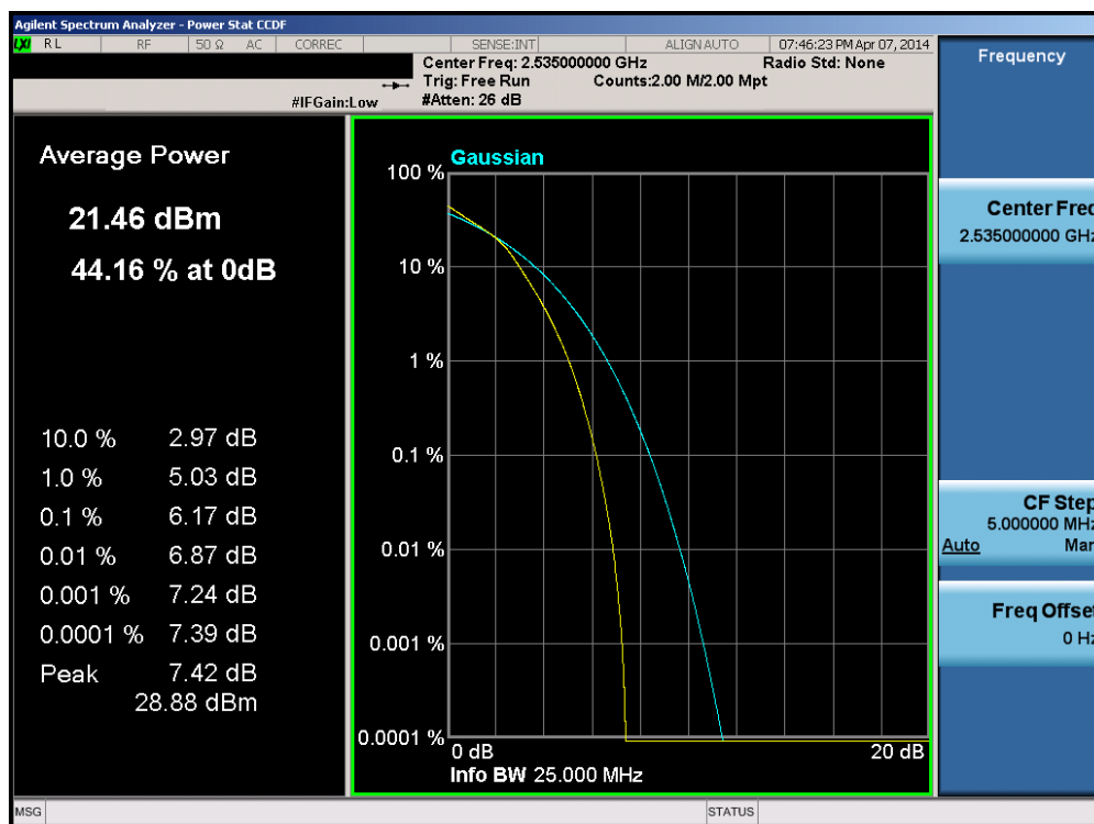
Plot 6-154. PAR Plot (Band 7 – 20.0MHz 16-QAM – RB Size 100)
